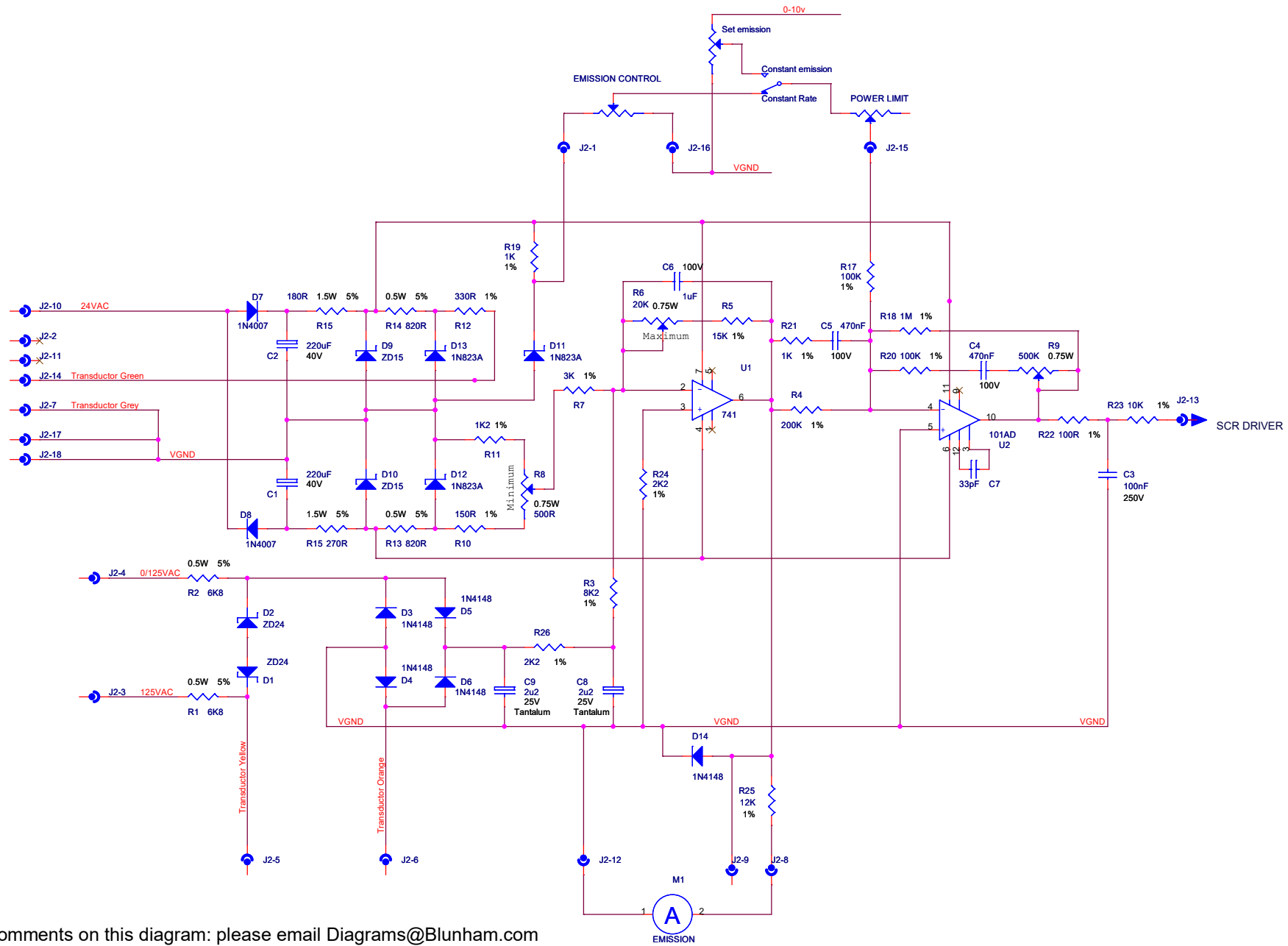
Emission Control board diagram with associated components for Balzers EKS110 system
