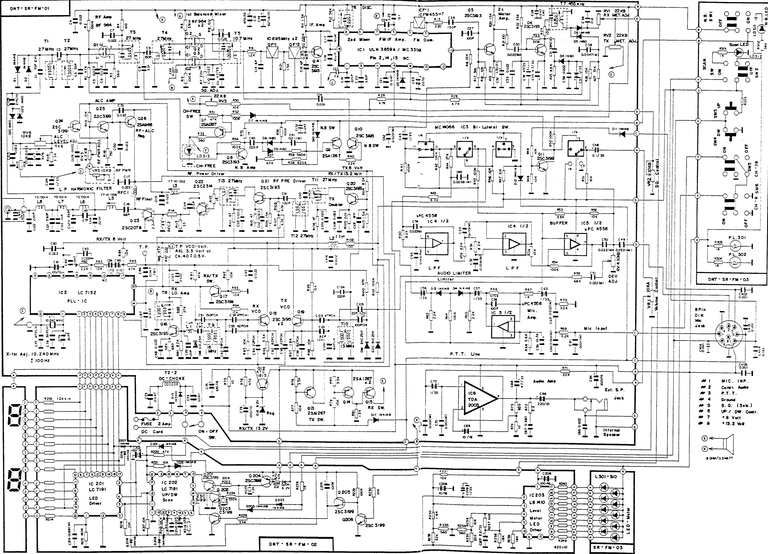
SCHEMATIC DIAGRAM SCANNER FM DNT
