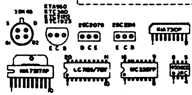
BOTTOM VIEW (PCT .TR)
