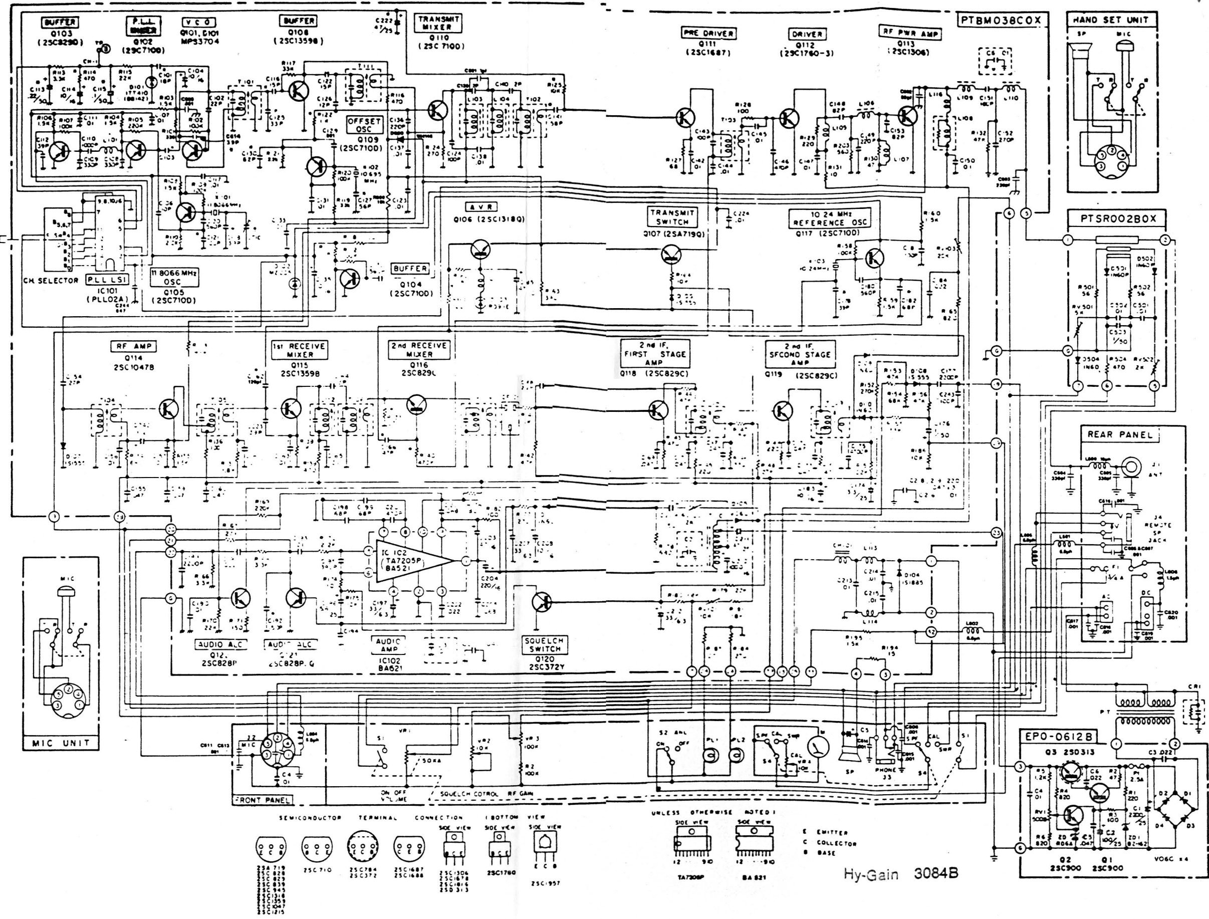
Fig. A-30. Hy-Gain's 3084B.
