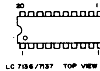
LC 7136/7137 TOP VIEW
