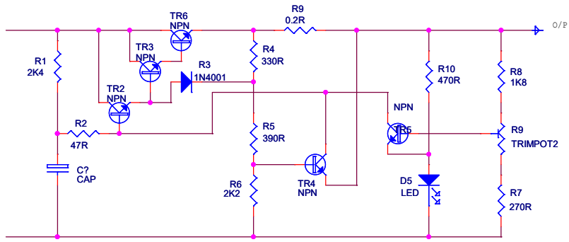
DELTA & CB MASTER PSU (3/5A)
