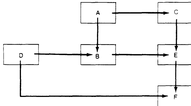
Dependency Diagram
