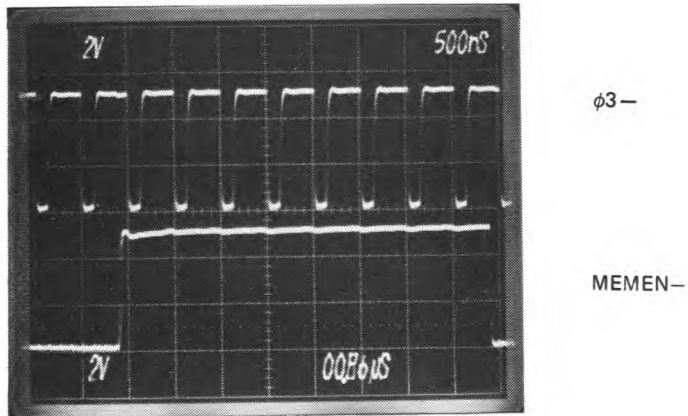
Figure 10-4. Clock Phase \phi 3- vs, MEMEN-
