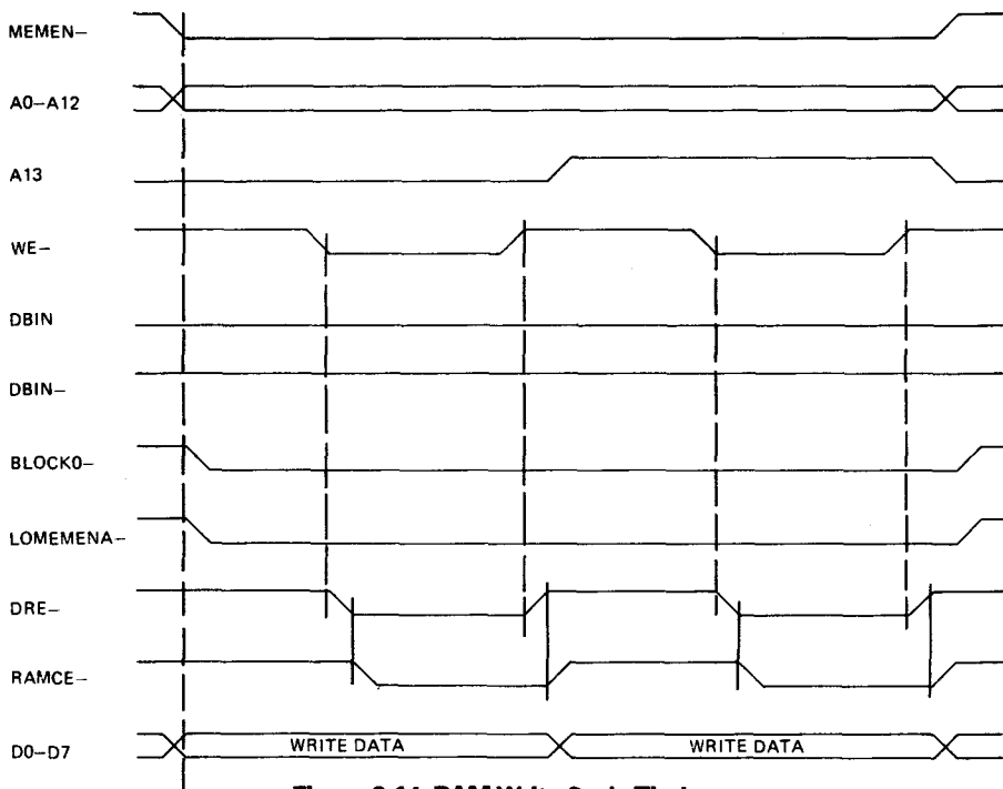
Figure 8-14. RAM Write Cycle Timing
