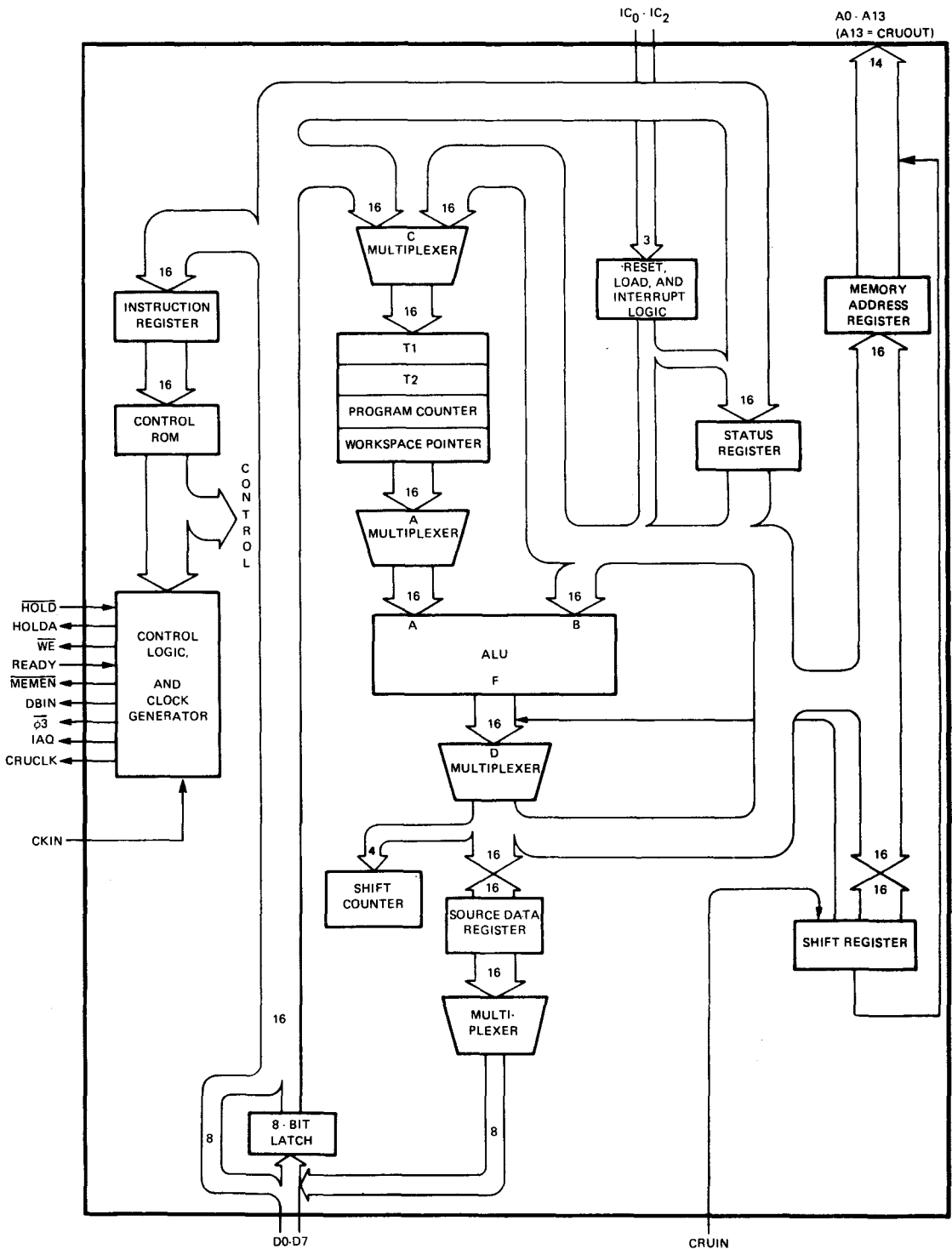
Figure 8-2. TMS 9980A Internal Architecture
