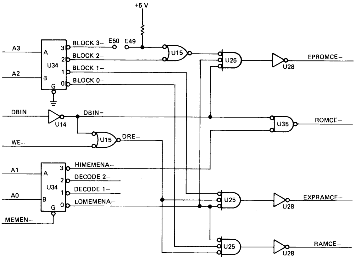
Figure 8-11. Memory Address Decoding
