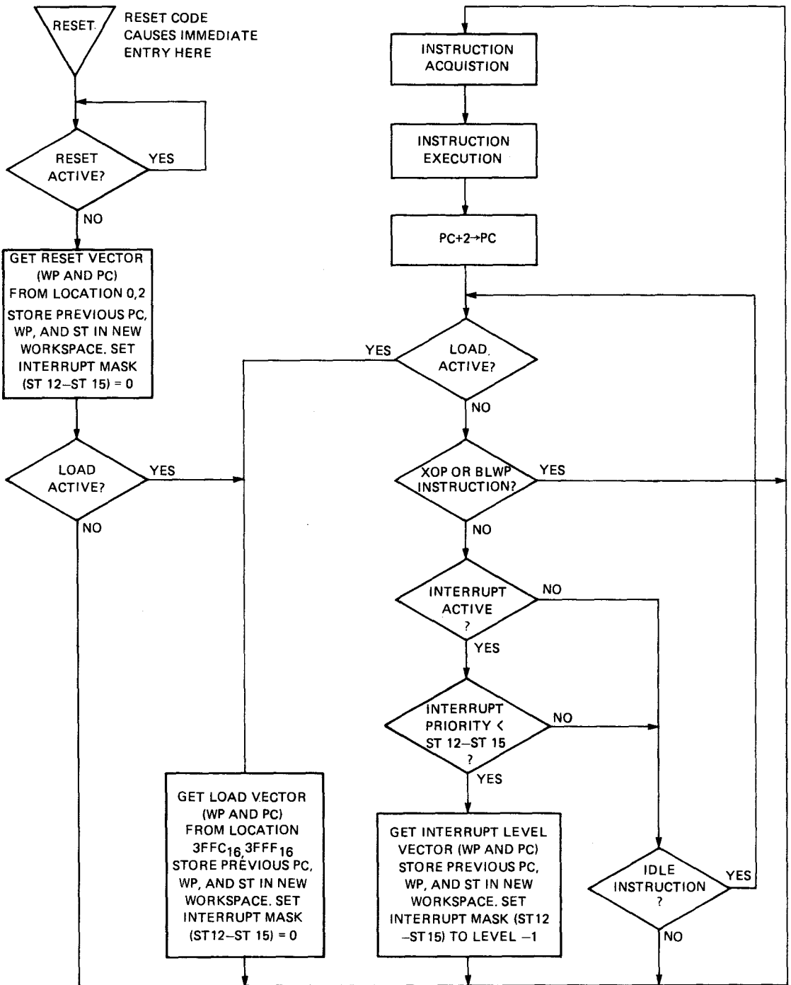
Figure 8-3. TMS 9980A CPU Flow Chart
