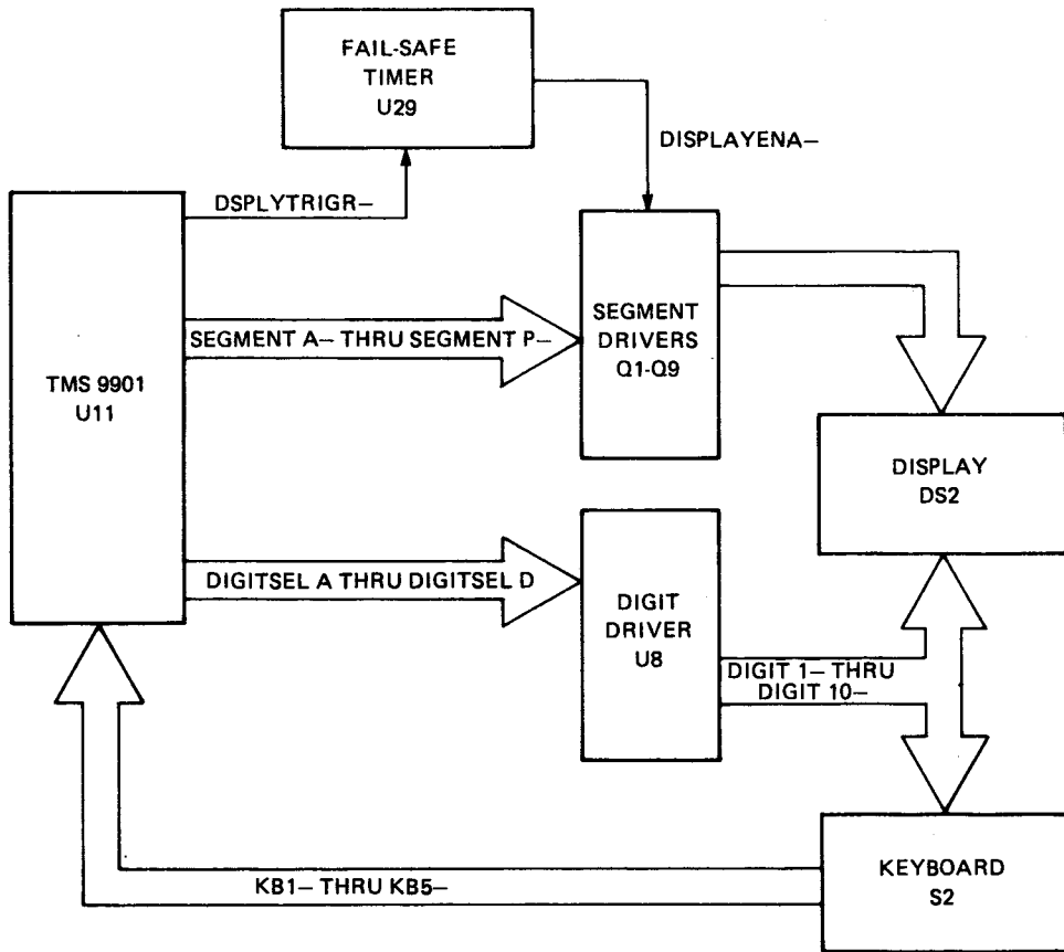
Figure 8-18. Keyboard and Display Interface Block Diagram
