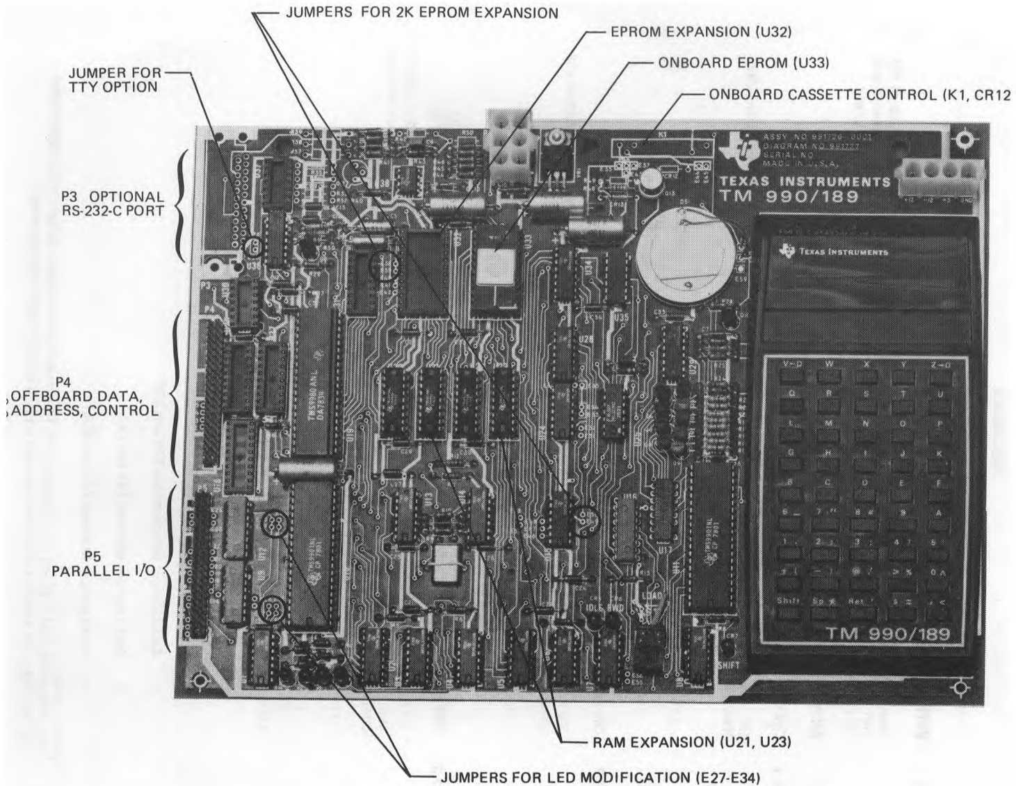
Figure 9-1. TM 990/189 Board Layout
