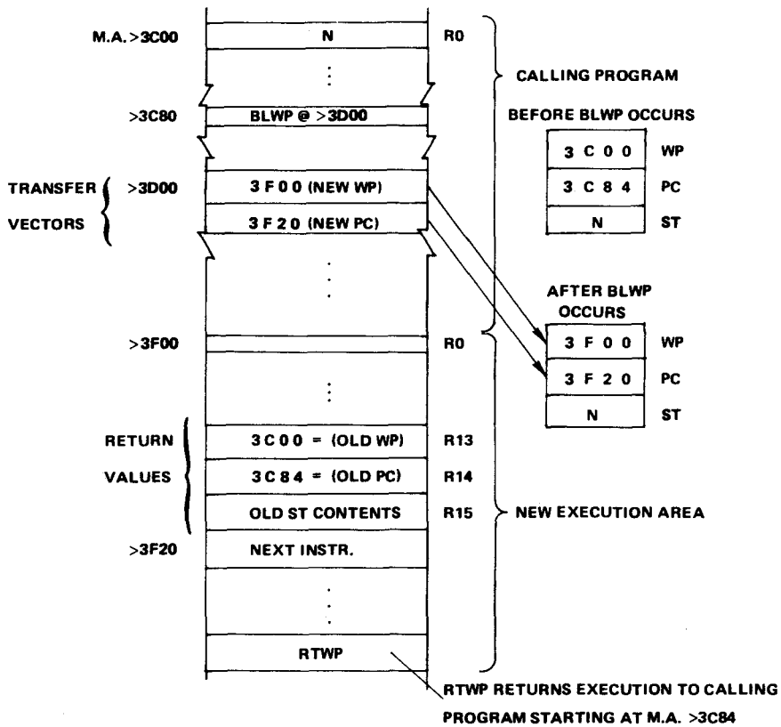
Figure 5-11. BLWP Example
