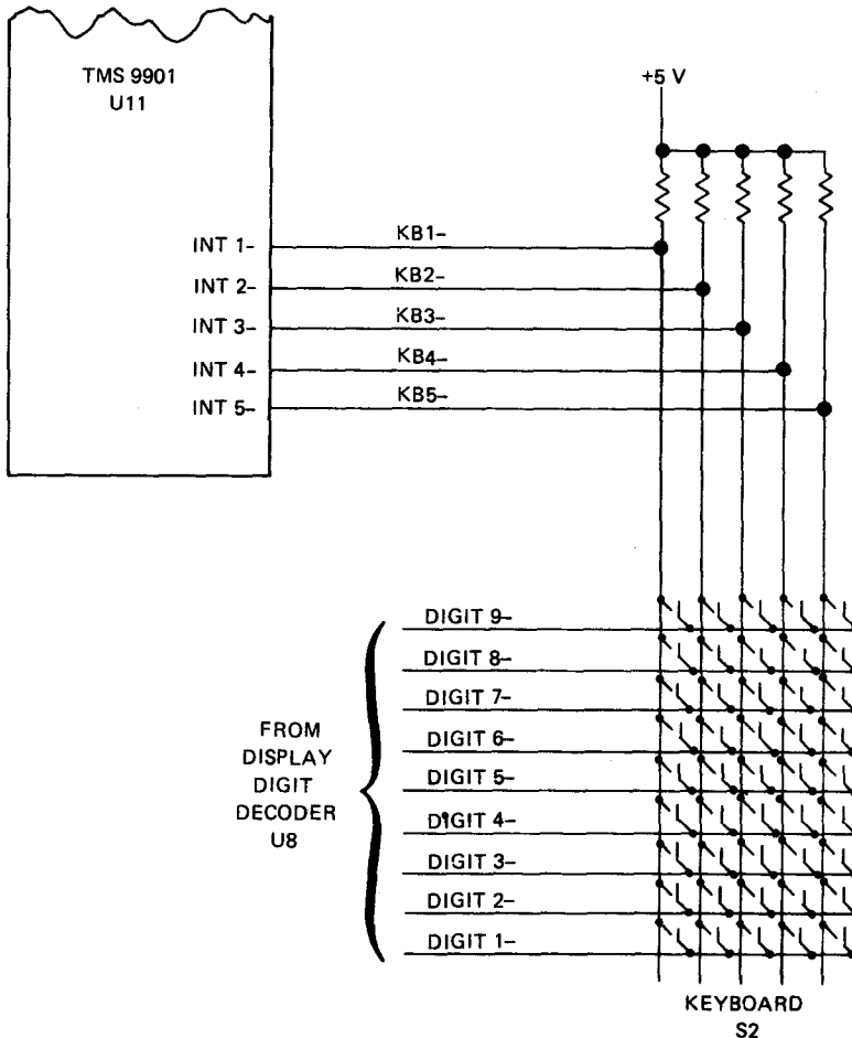
Figure 8-21. Keyboard Interface
