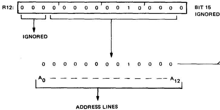
Figure 7-7. LDCR Word Execution to TMS 9901
