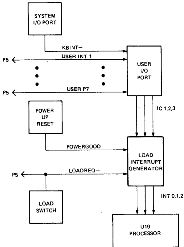
Figure 8-6. Interrupt Signal Flow
