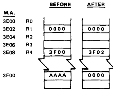
Figure 5-8. Indirect Register Autoincrement Addressing Example
