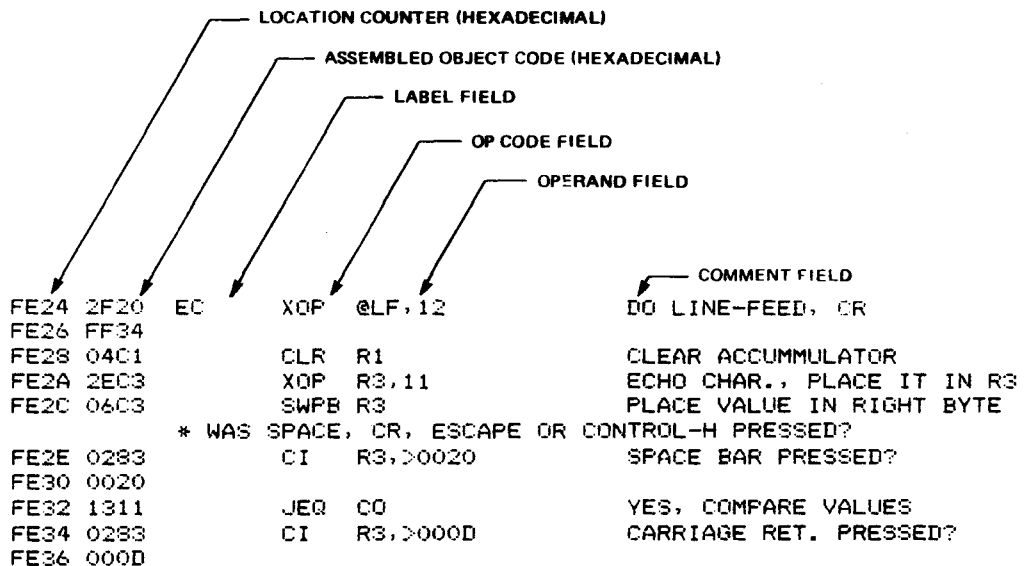
Figure 4-1. Listing and Source Statement Fields
