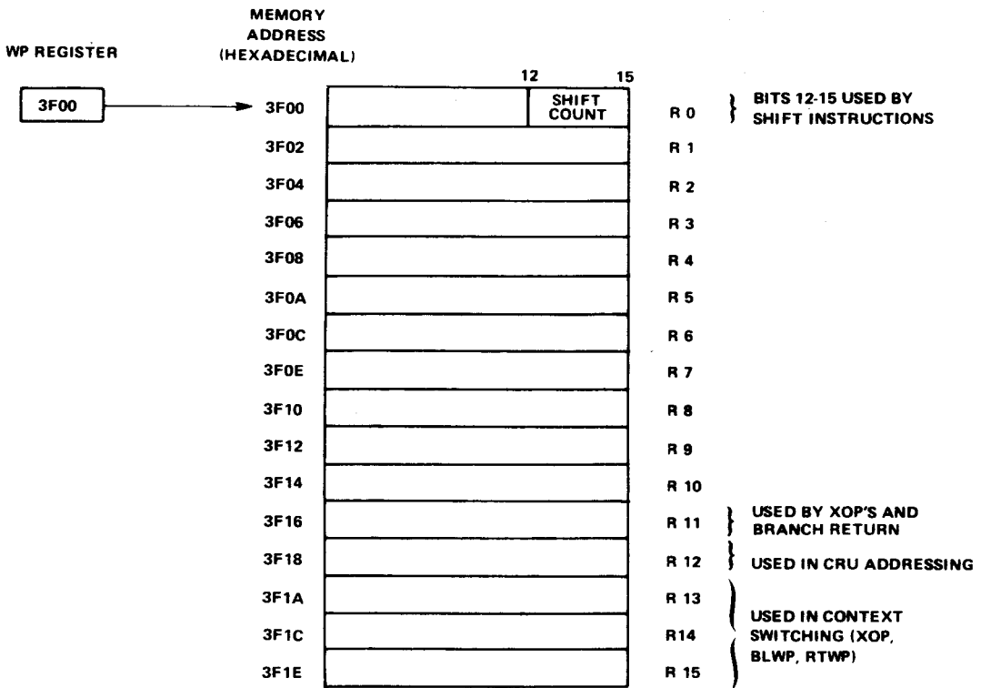
Figure 5-4. Workspace Example
