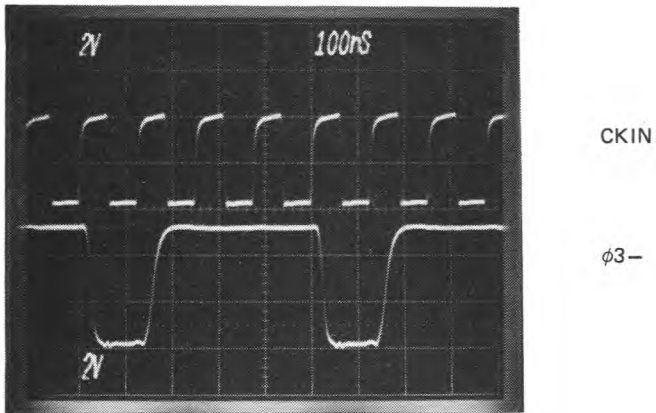
Figure 10-3. CKIN vs. Clock Phase \phi 3-
