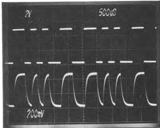
Figure 10-9. AUDIOIN vs. RDATA
