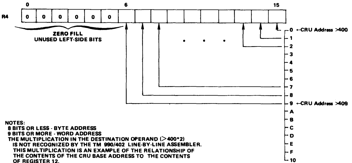
Figure 7-6. STCR Word Instruction
