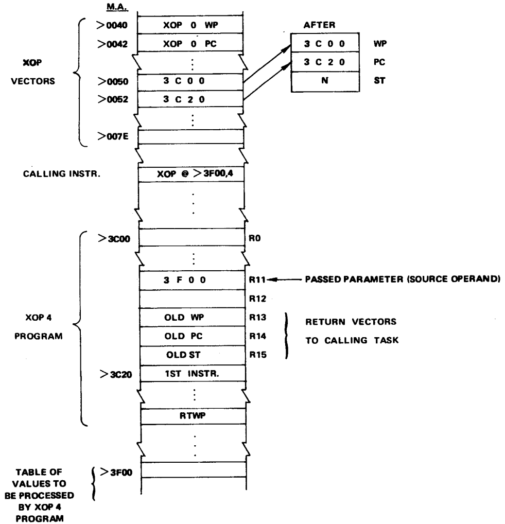
Figure 5-12. XOP Example
