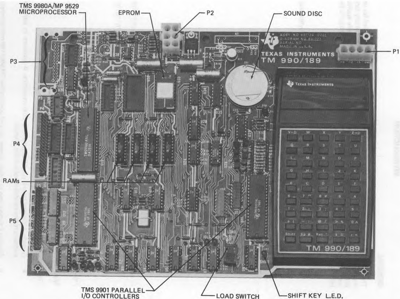
Figure 1-1. Principal TM 990/189 Components
