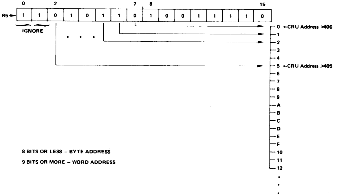
Figure 7-5. LDCR Byte Instruction
