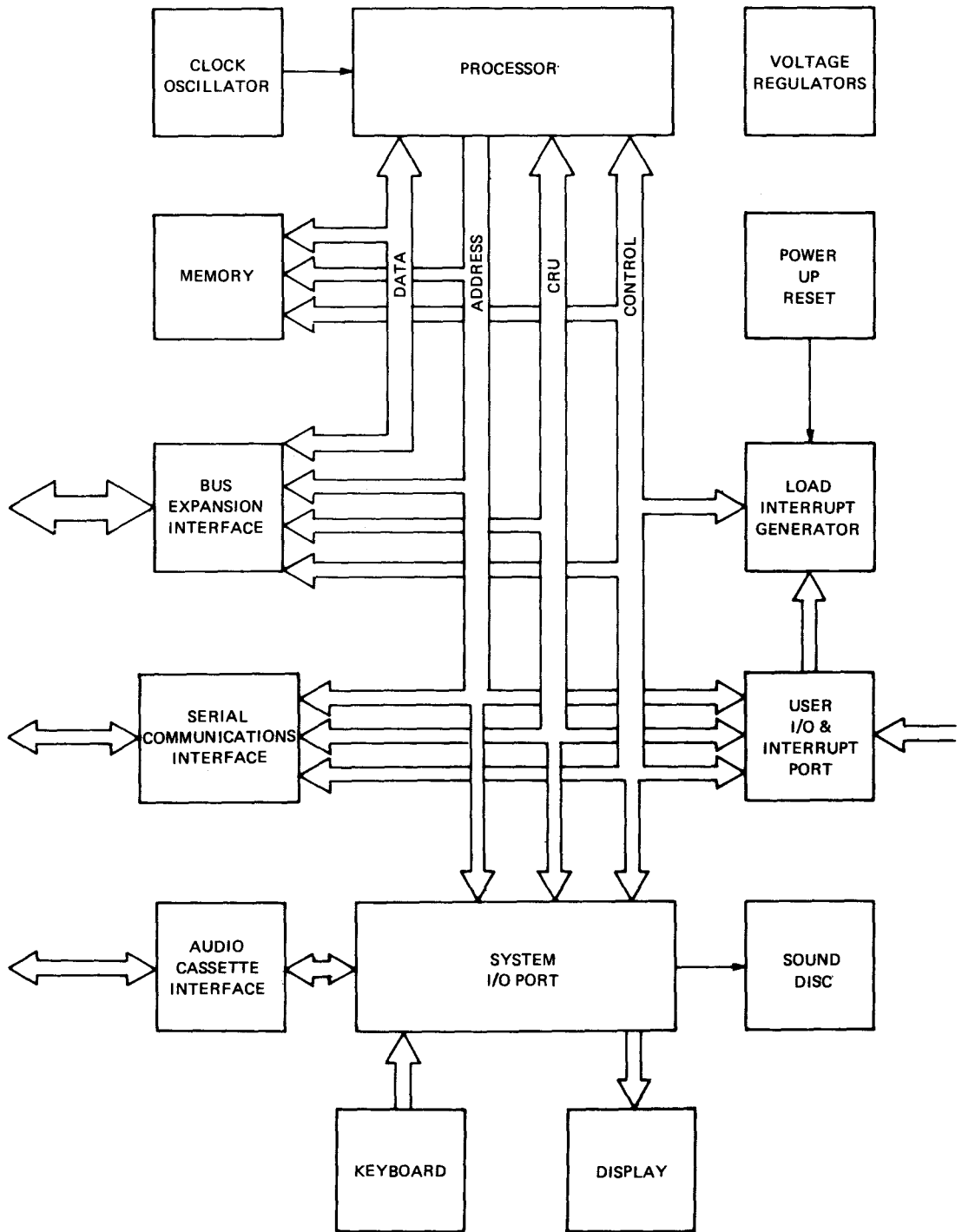
Figure 8-1. System Block Diagram
