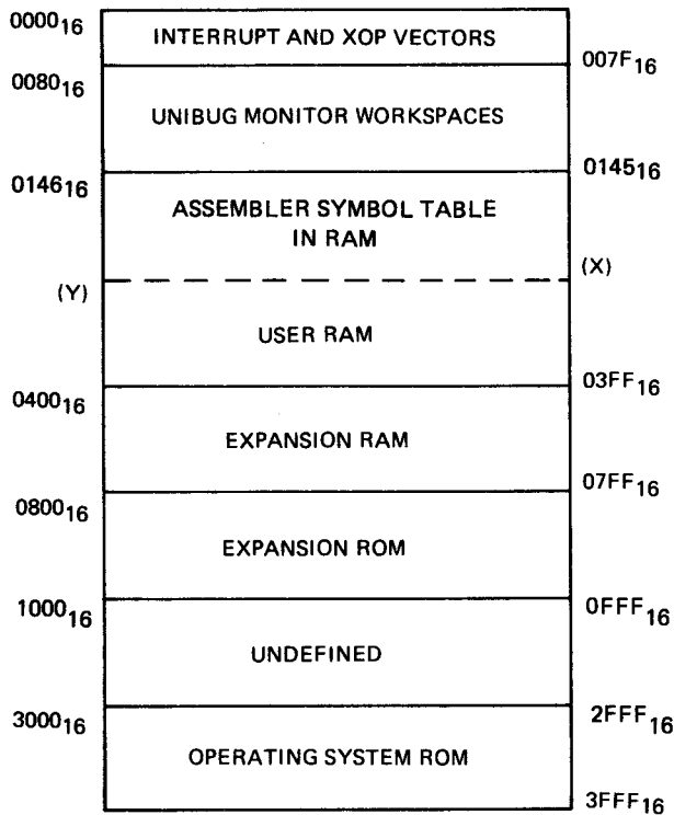
Figure 5-1. Memory Map
