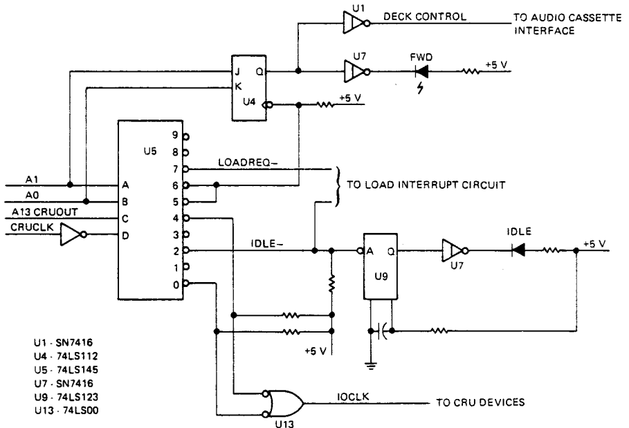
Figure 8-5. External Instruction Decode
