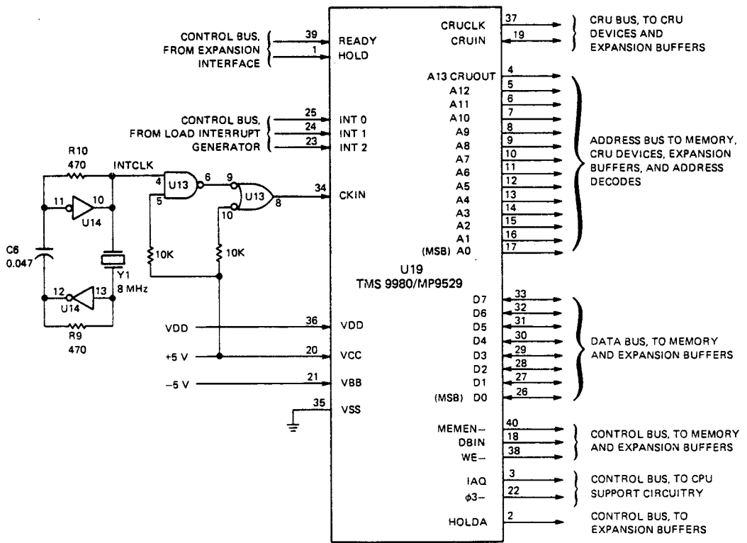
Figure 8-4. TMS 9980A Signals
