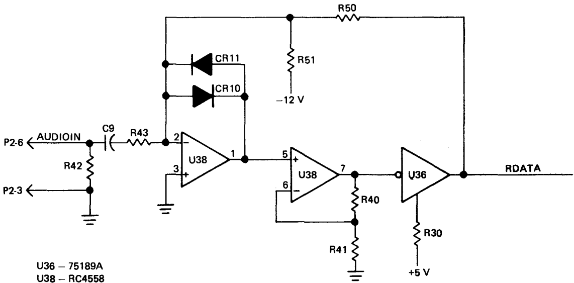
Figure 8-23. Cassette Read Circuit
