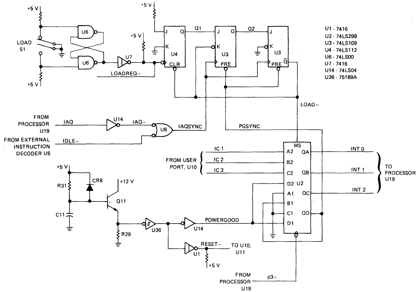
Figure 8-7. Load Interrupt Generator and Power Up Reset Circuit
