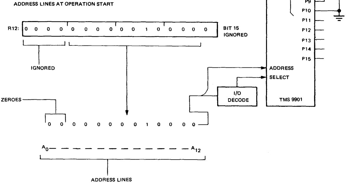
Figure 7-9. STCR Word Execution to TMS 9901
