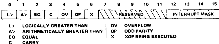
Figure 5-3. Status Register
