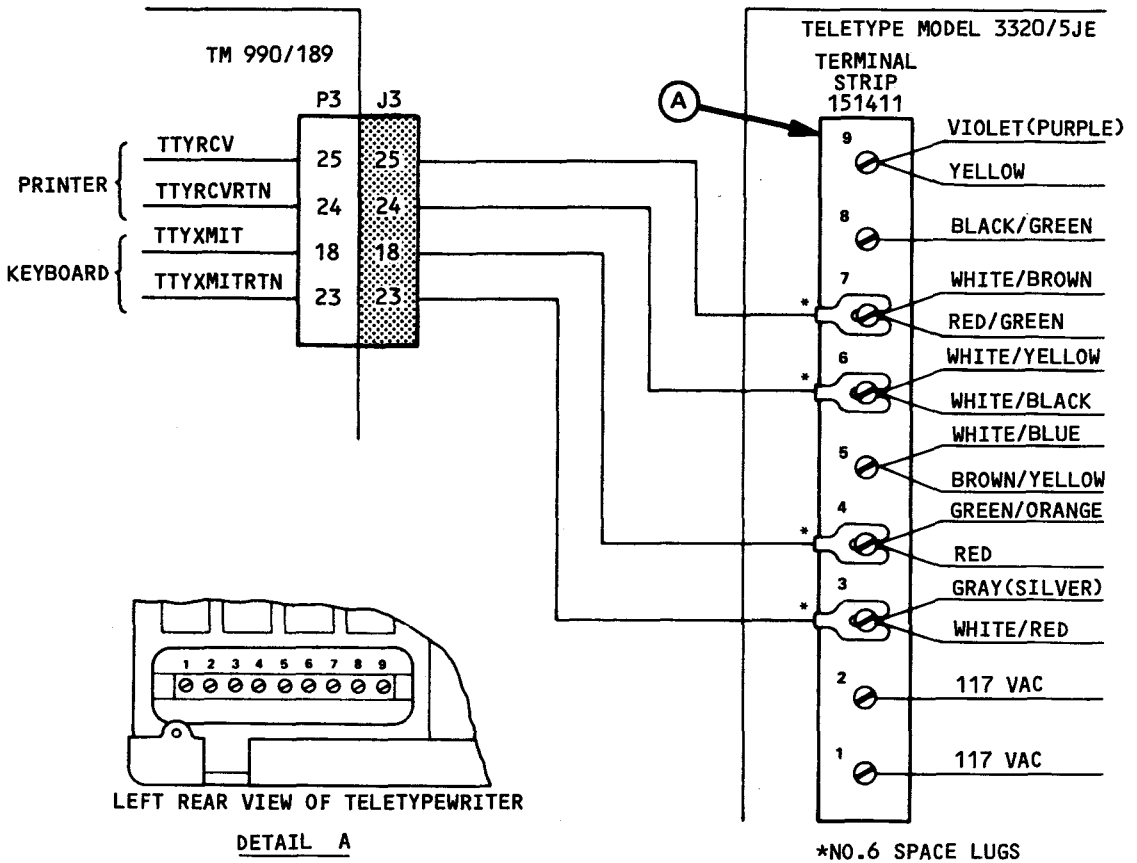
Figure I-1. Teletypewriter Terminal Strip Connections
