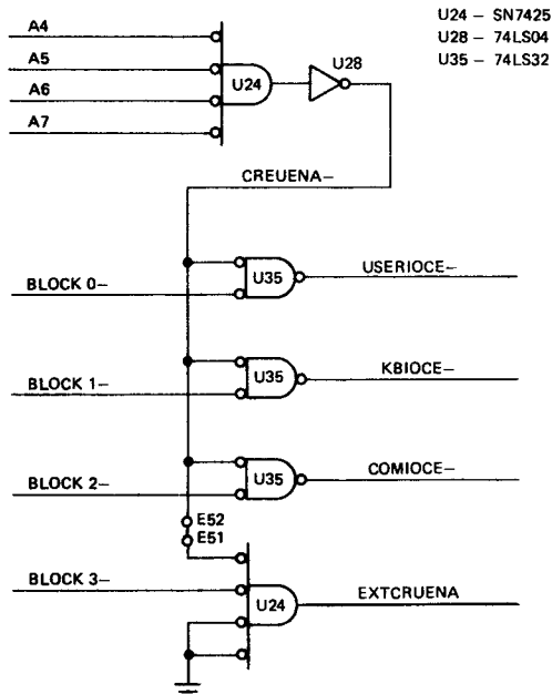
Figure 8-17. CRU Address Decoding Logic
