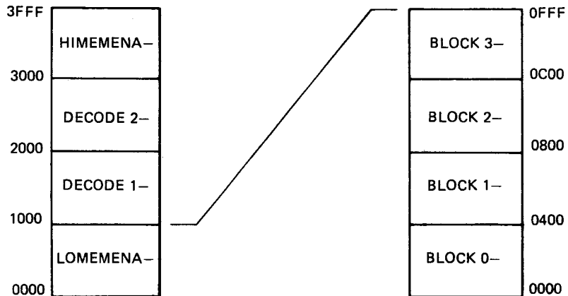
Figure 8-12. Memory Partitioning Signals
