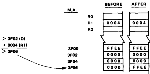
Figure 5-10. Symbolic Memory Addressing, Indexed Example
