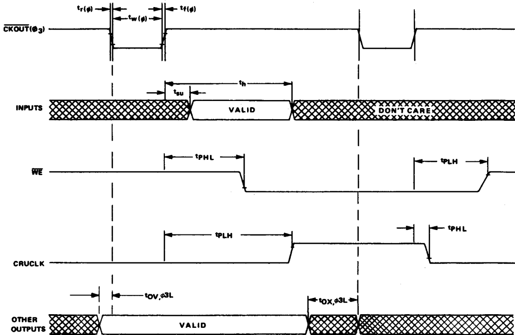
FIGURE 14 – EXTERNAL SIGNAL TIMING DIAGRAM
