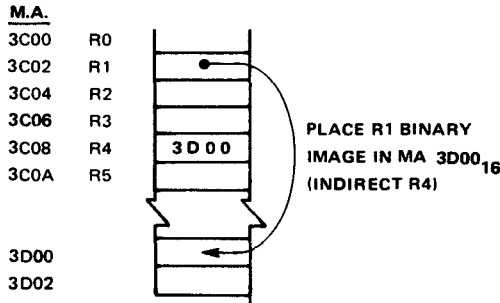
Figure 5-7. Indirect Register Addressing Example
