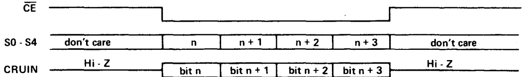
ACC DATA ACCESS SIGNAL TIMING
