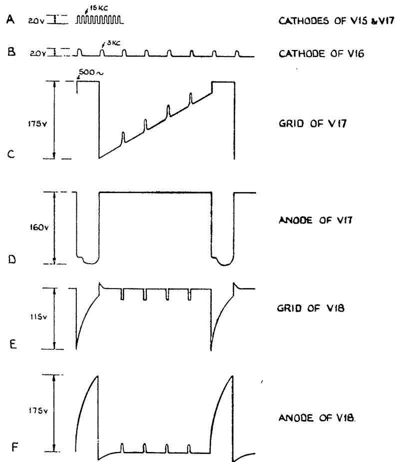
Fig. 36.—"A" strobe locking waveforms.
