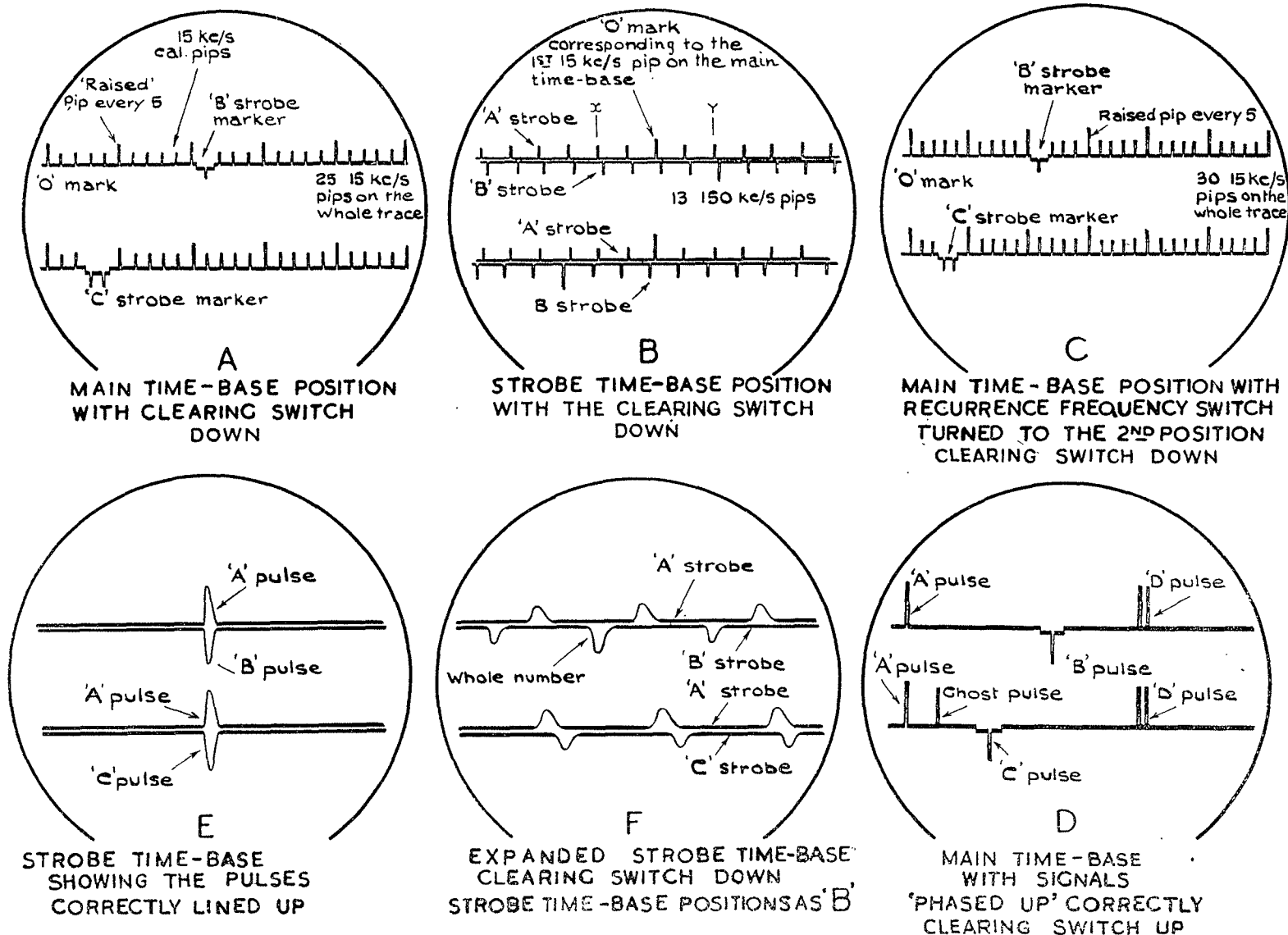
Fig. 6.—Screen indications.
