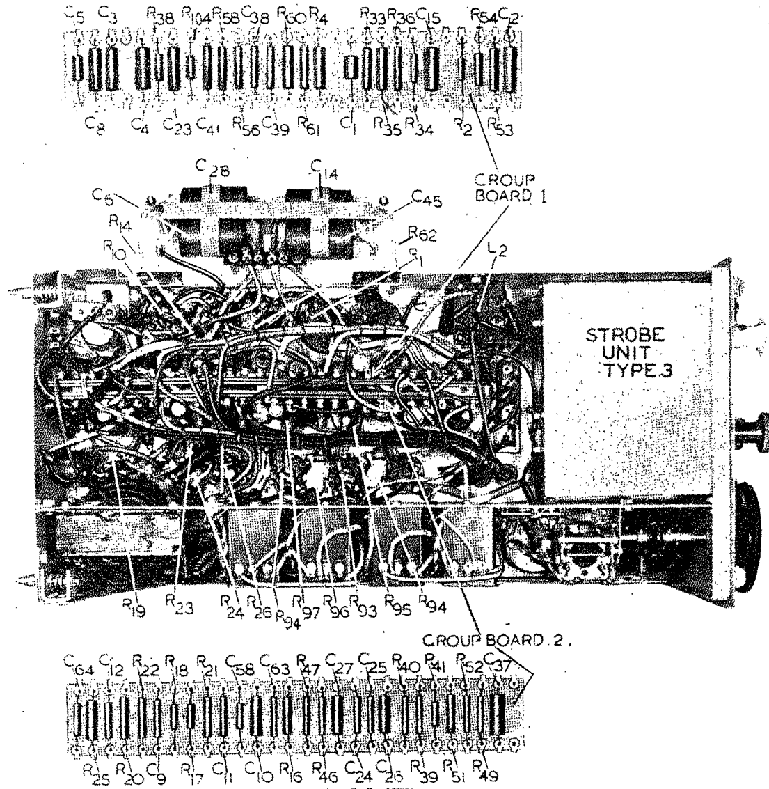
Fig. 31.—Indicator unit type 62, underside of chassis.
