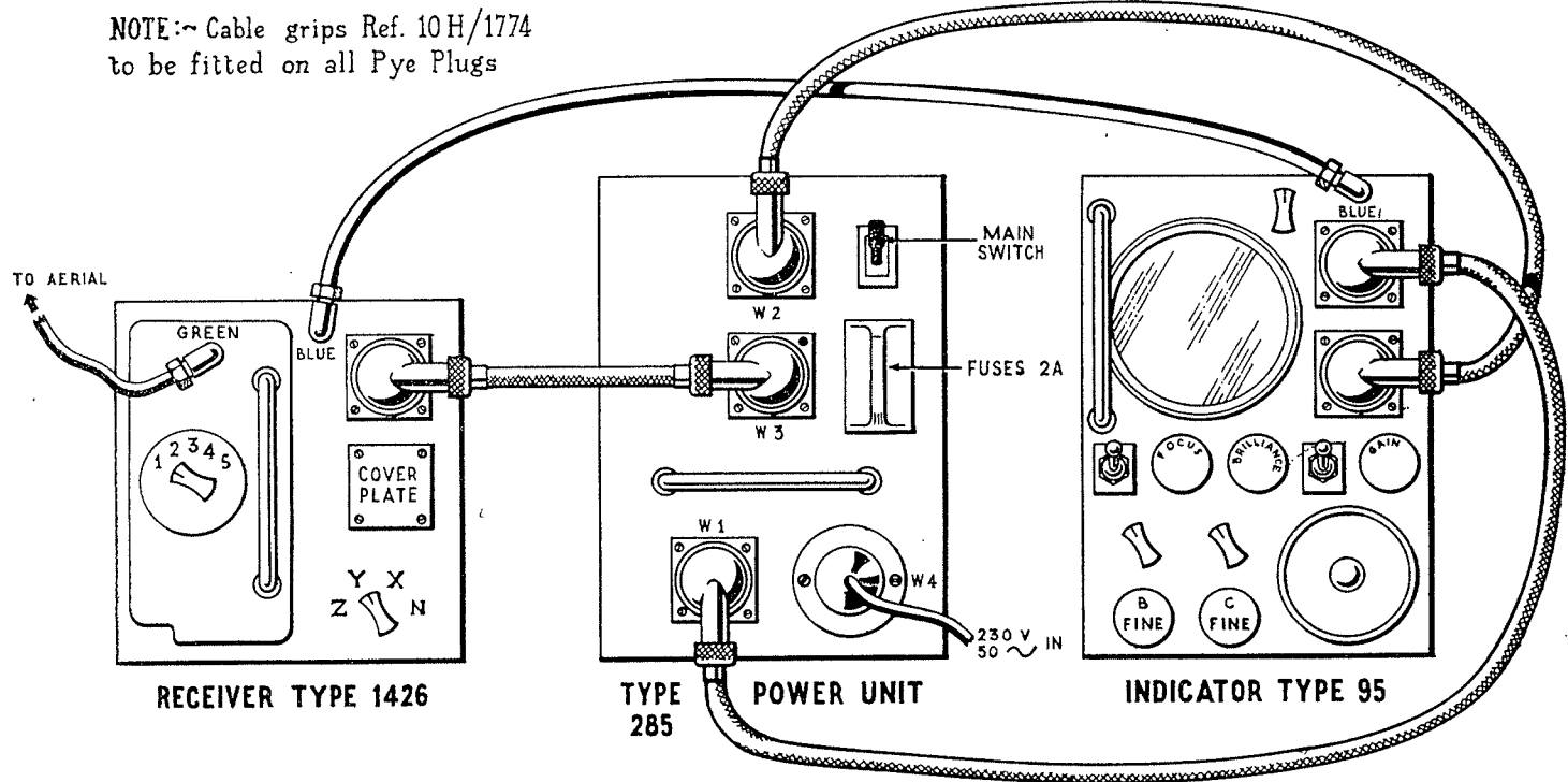
Fig. 34.—Interconnection—Kit type 30.
