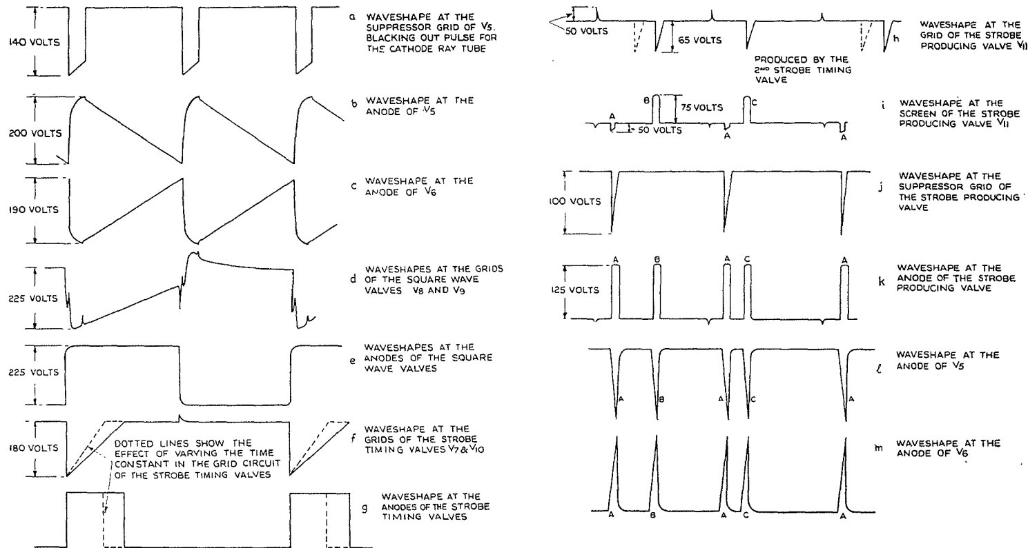
Fig. 28.—Waveforms [2].
