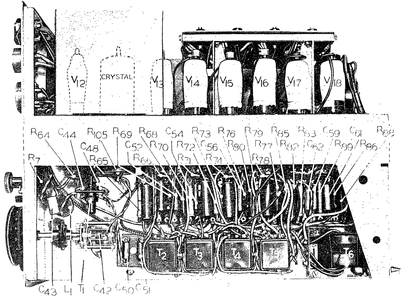
Fig. 29.—Indicator unit type 62, right-hand side of chassis.
