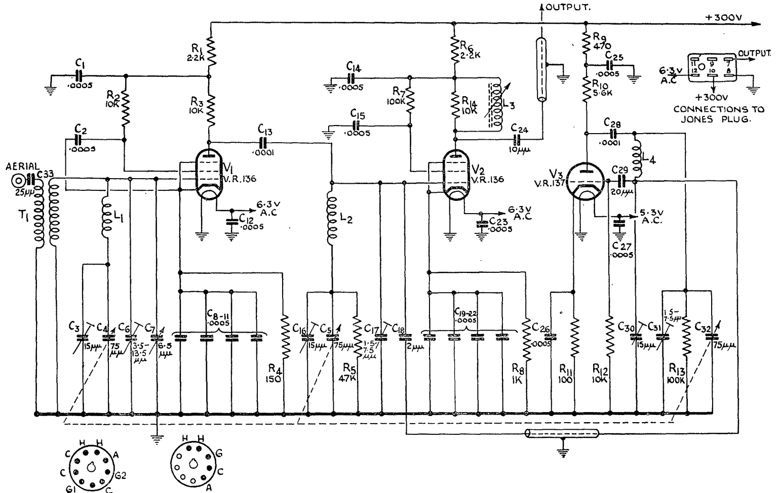
Fig. 19.—RF unit type 27, circuit.
