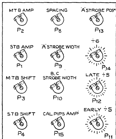
Fig. 32.—Indicator unit type 62, presets on top of chassis.
