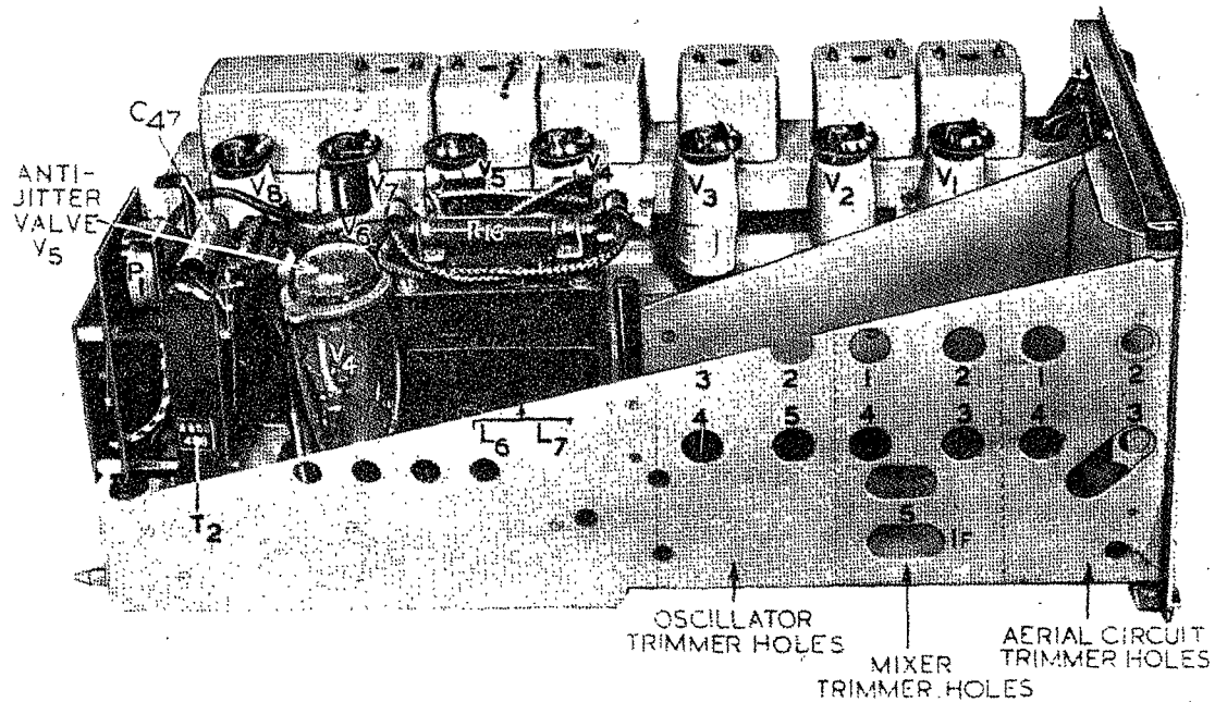
Fig. 24.—R.1355, top left-hand side of chassis.
