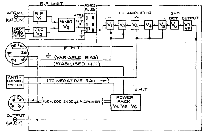
Fig. 3.—Receiver type R.1355, block schematic diagram.
