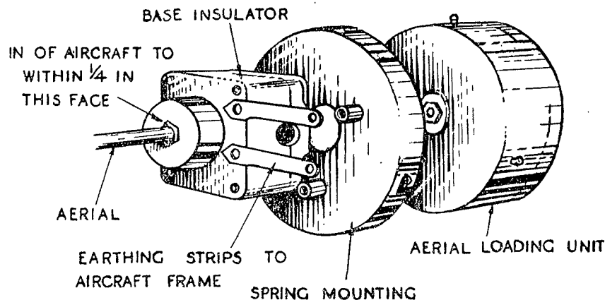
Fig. 9.—Exploded view illustrating attachment of loading unit to aerial.
