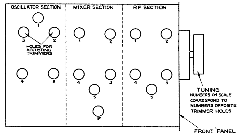
Fig. 12.—Positions of trimmers on RF units type 24 and 25.
