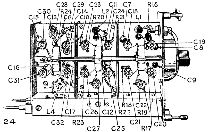
Fig. 14.—RF units types 24 and 25, side views.
