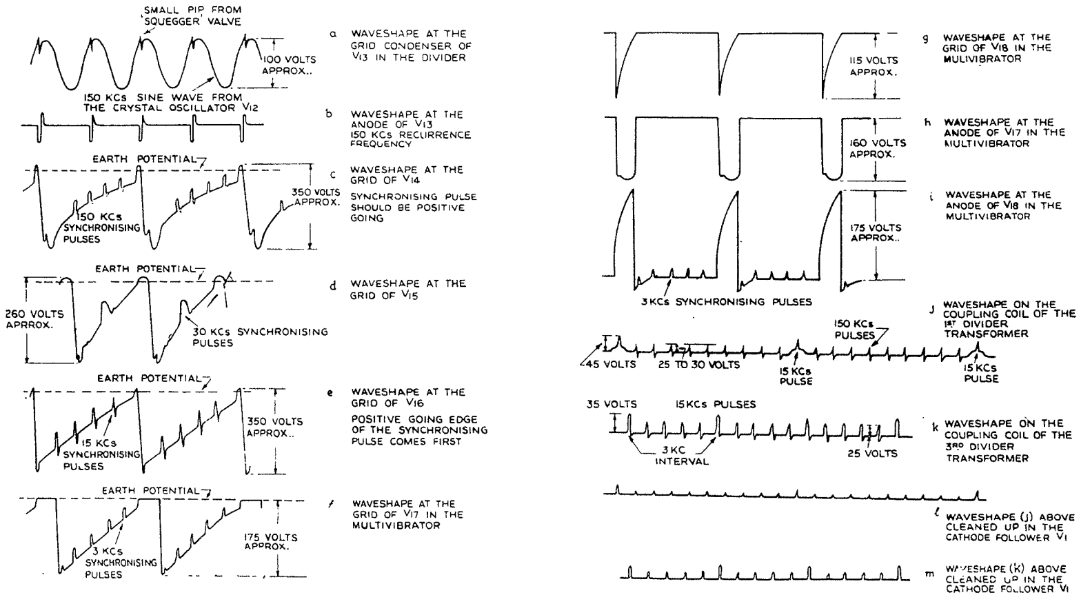
Fig.27.—Waveforms [1].
