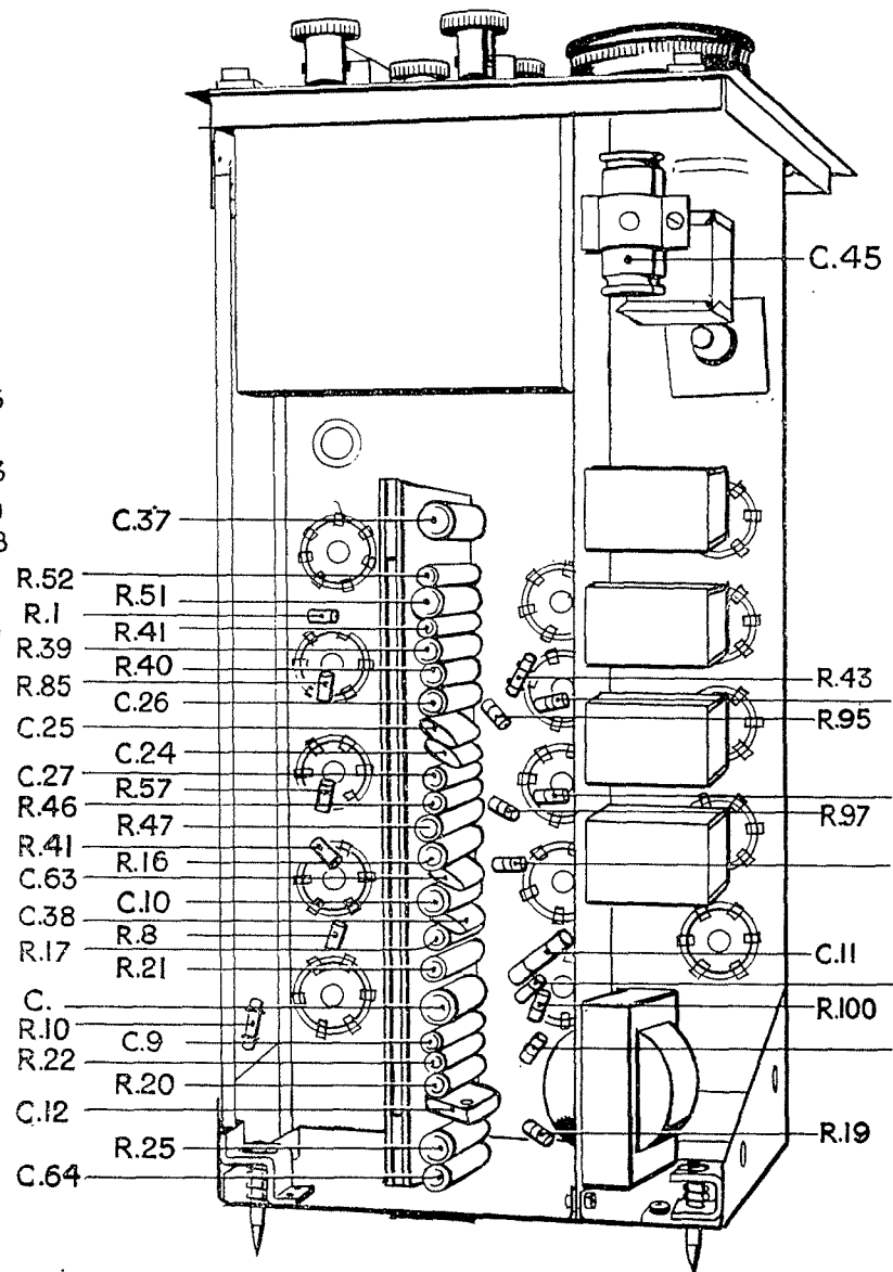
Fig. 41.—Indicator unit type 62A, underside of chassis.
