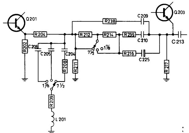
Fig. 5.3 Playback equalizing network.
