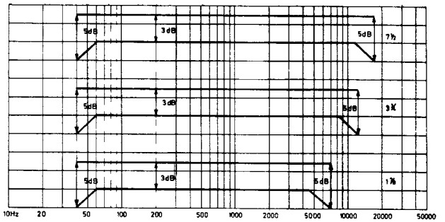
Fig. 8.3 DIN-curves for frequency range.
