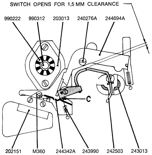
Fig. 4.37 End stop or tape break.
