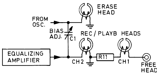
Fig. 5.8 Recording EXTRA.
