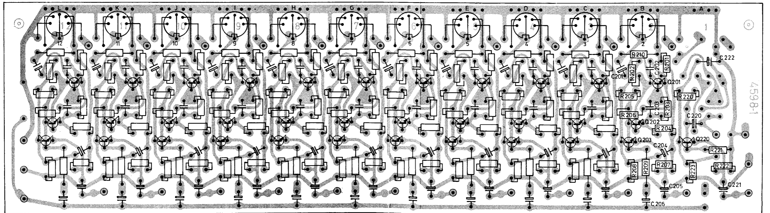
Board for input amplifiers, Model 15GT. Seen from print side.
