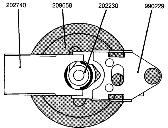
Fig. 4.10 Take-up friction disc with clutch levers.
