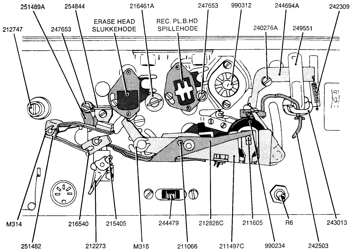
Fig. 4.4 Tape path.
