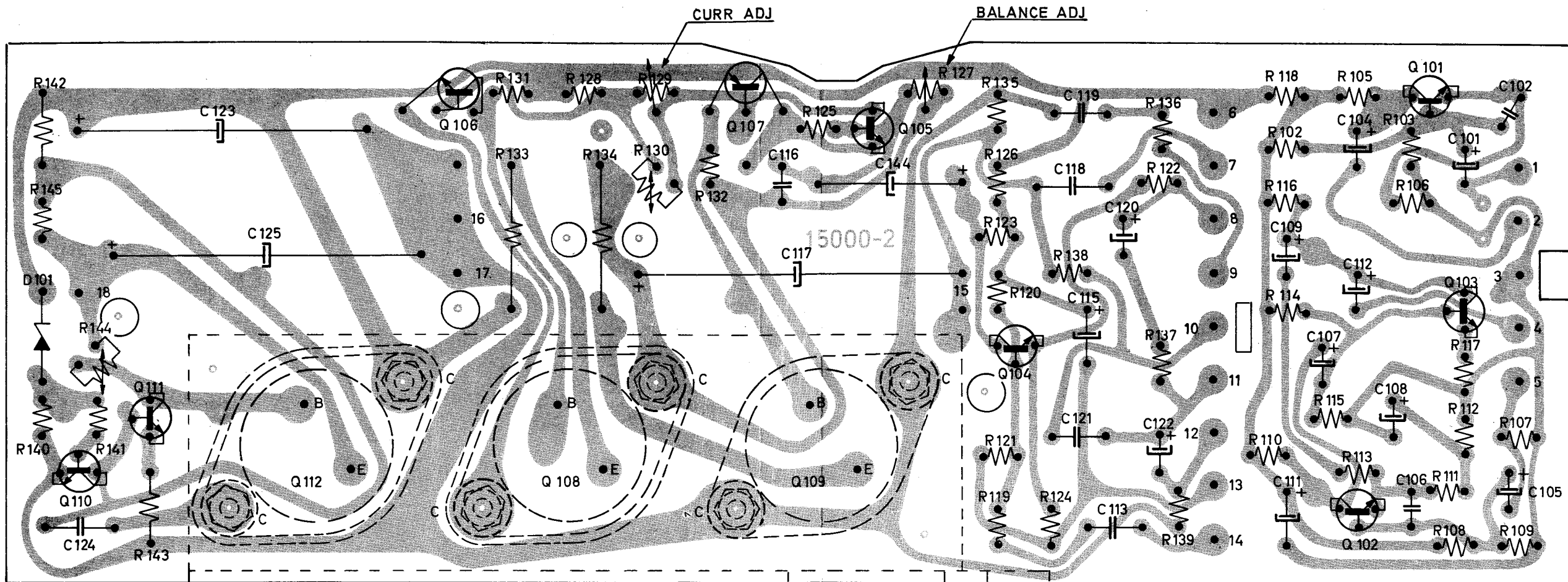
Board for line amplifier, microphone amplifier and voltage regulator, all models. Seen from print side.
