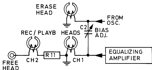
Fig. 5.6 Recording NORMAL.
