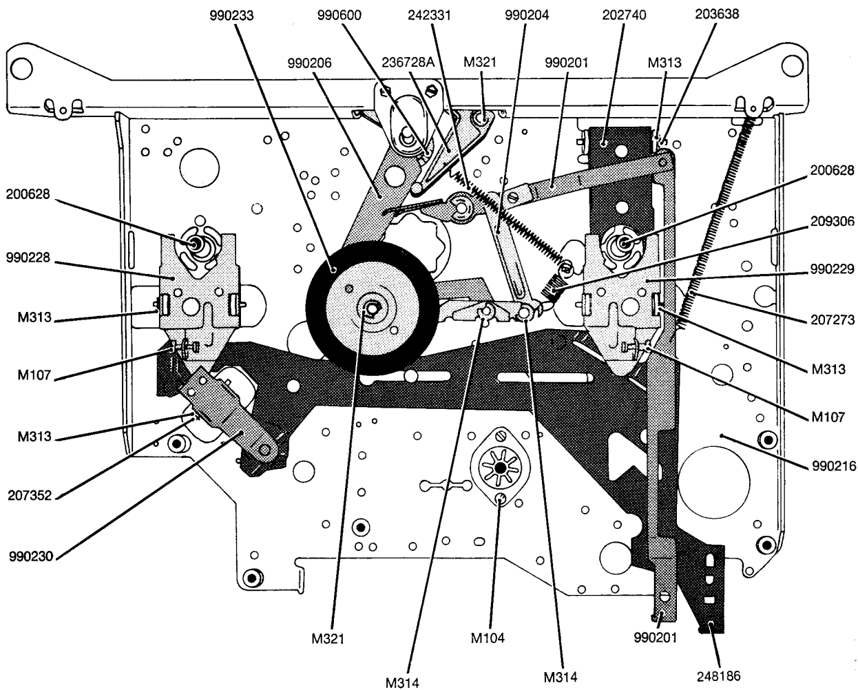
Fig. 4.5 Lower mounting plate with mechanical parts.
