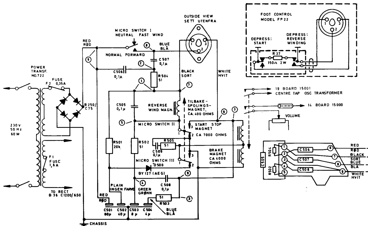
Schematic for remote control unit model 15F. Above serial no. 2 510 020.
