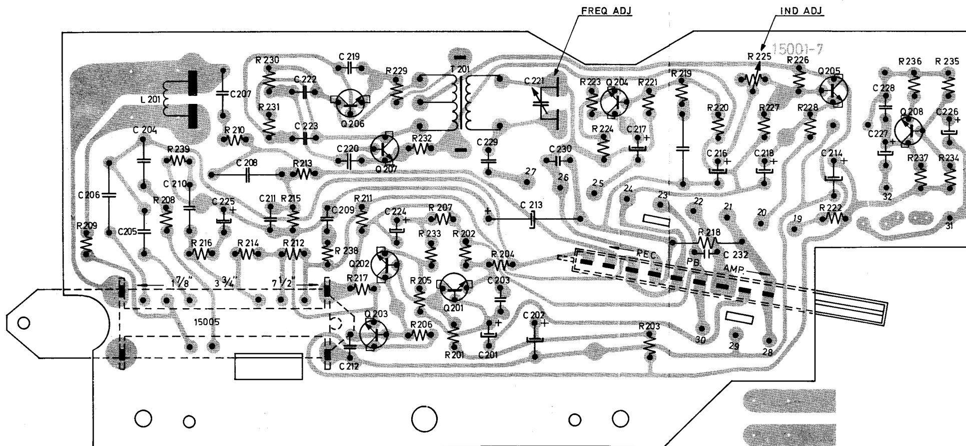
Board for record/playback amplifier, indicator amplifier and oscillator, all models. Seen from print side.
