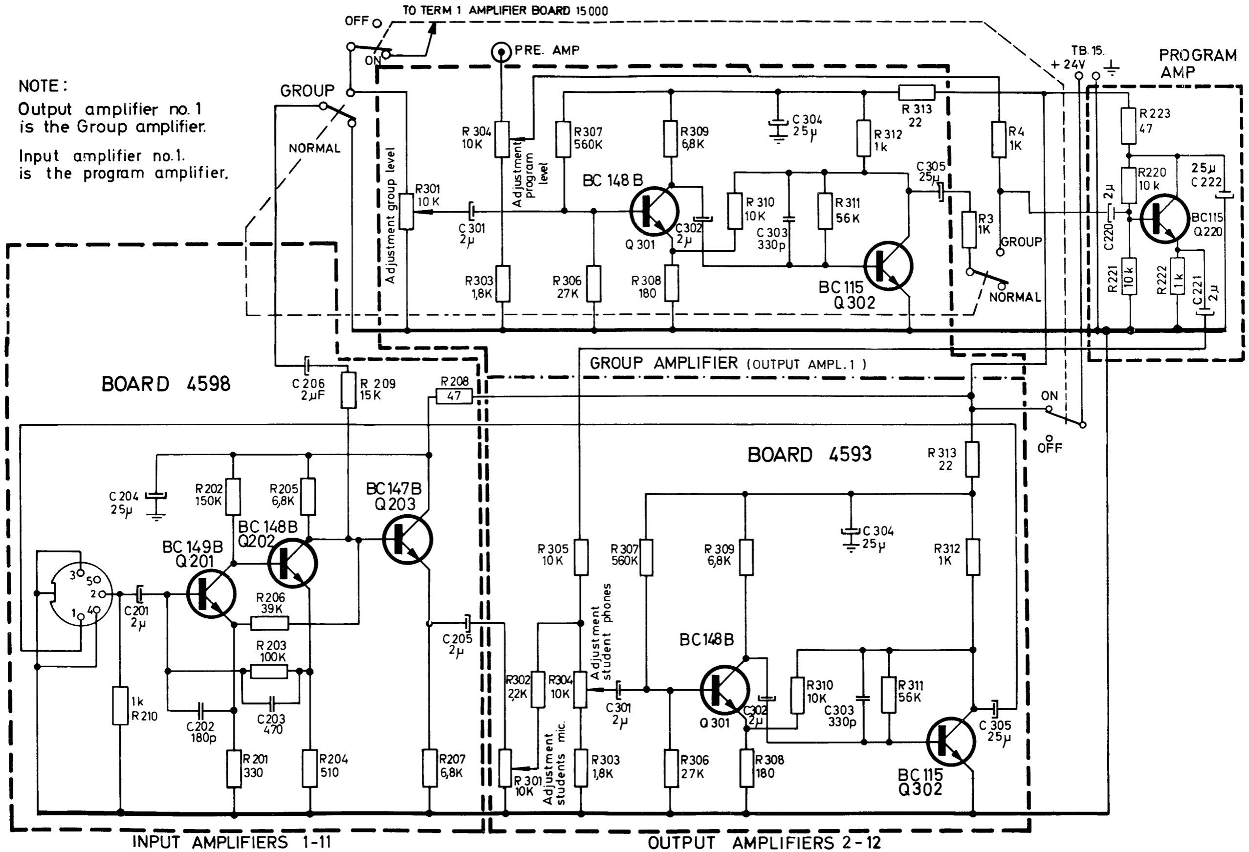
Schematic for additional amplifiers, Model 15GT.
