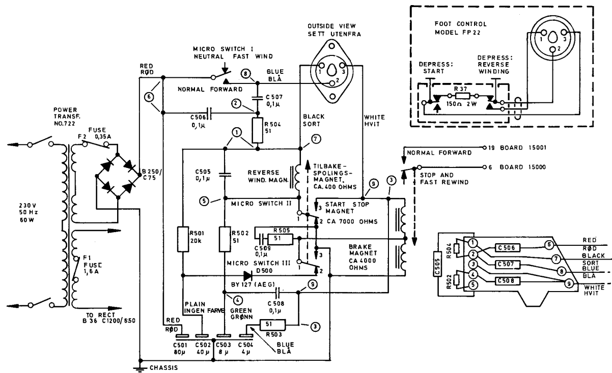
Schematic for remote control unit, model 15F. Below series no. 2 510 020.
