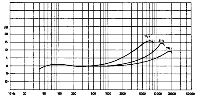
Fig. 5.2 a Record equalizing curves.
