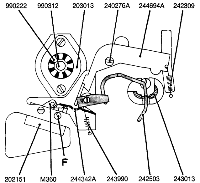
Fig. 4.39 Adjustment.
