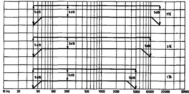
Fig. 1.1 DIN-specified frequency range with tolerances.
