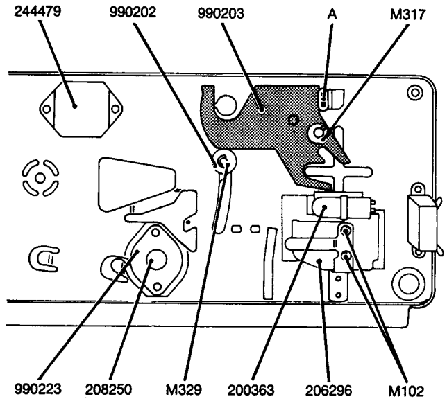
Fig. 4.2 Bottom view of upper mounting plate.
