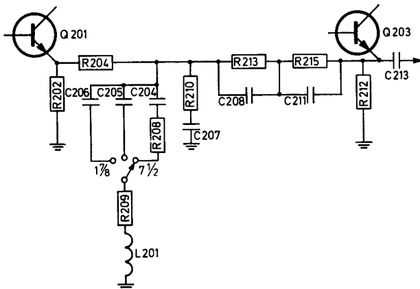
Fig. 5.1 Record equalizing network.
