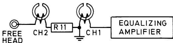
Fig. 5.5 Playback NORMAL.
