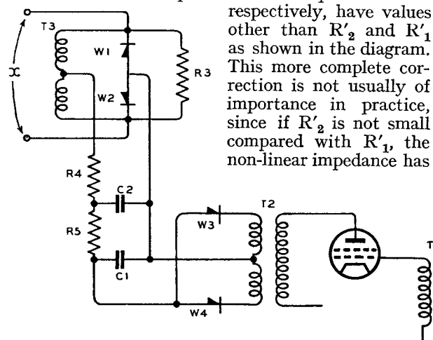
FIG. 2.—SCHEMATIC OF THE CONTROL CIRCUIT.
