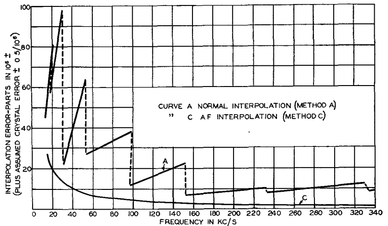
FIG. 5.—L.W. AND A.F. OSCILLATORS—INTERPOLATION ERROR (PLUS ASSUMED CRYSTAL ERROR OF \pm 0.5/10^6 ).
