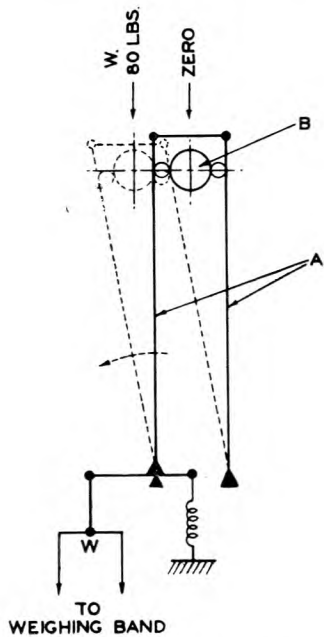
FIG. 8.—WEIGHING MECHANISM.
