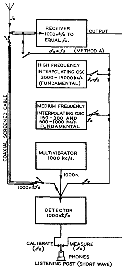
FIG. 9.—BLOCK SCHEMATIC SHOWING METHOD B.
