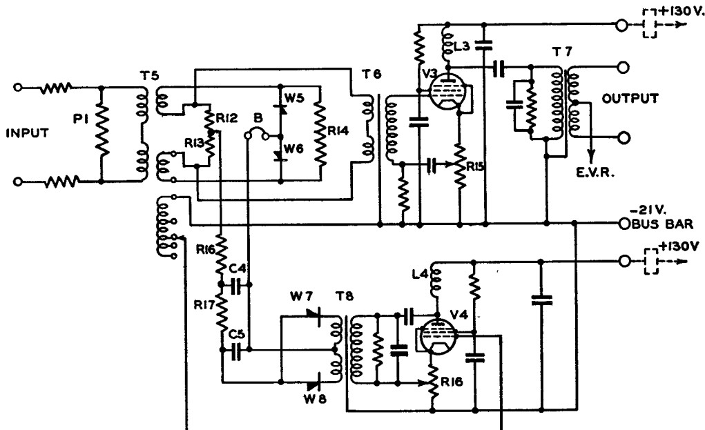
FIG. 5.—CIRCUIT OF THE EXPERIMENTAL EXPANDER UNIT.
