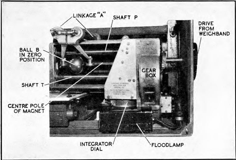
FIG. 6.—PLAN VIEW OF INTEGRATOR.
