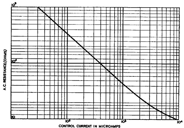
FIG. 3.—IMPEDANCE CHARACTERISTIC OF TYPICAL COPPER OXIDE RECTIFIER
