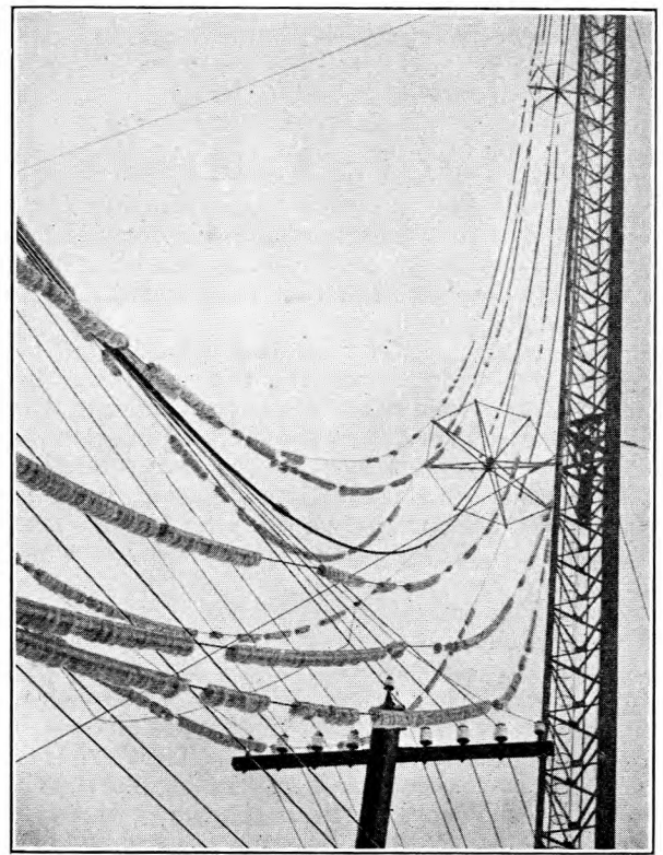
FIG. 5.—CLOSE-UP VIEW OF SUSPENDED AERIAL.
