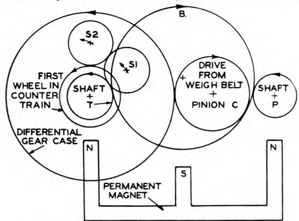
FIG. 7.—DIAGRAMMATIC VIEW OF INTEGRATOR.
