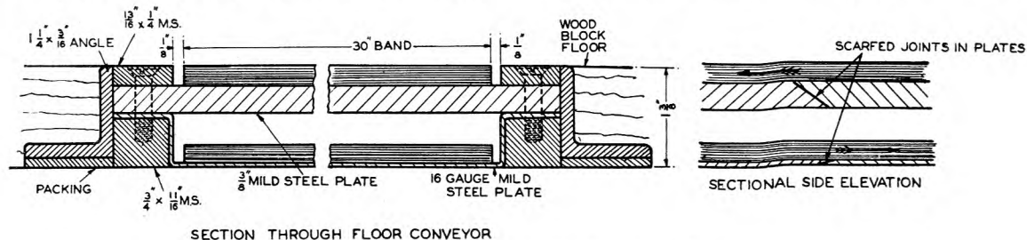
FIG. 3.—CONSTRUCTION OF THE CONVEYOR BED.
