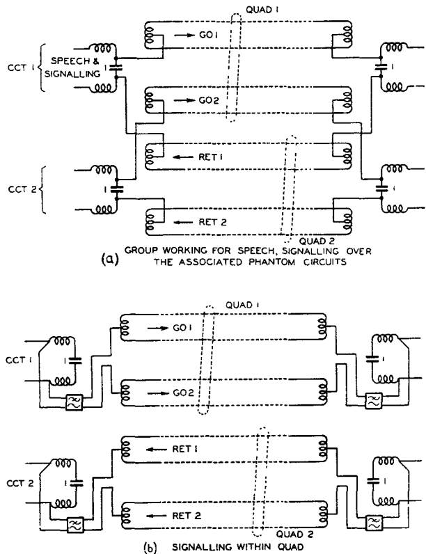
FIG. 3.—GROUP AND QUAD WORKING.
