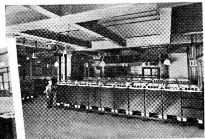
TWO BATTERIES OF HUW47 TYPE ALTON CELLS AT A LARGE CITY TELEPHONE EXCHANGE
