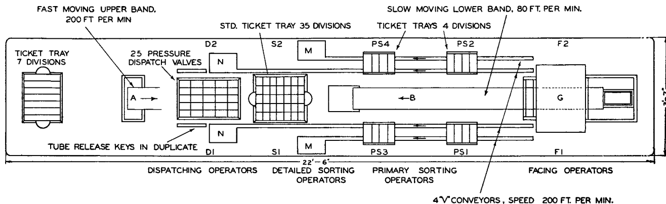
FIG. 8.—LAYOUT OF COMBINED PNEUMATIC DISTRIBUTION POSITION AND TICKET FILING POSITION.
