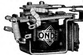
Midget Relay ML (for D.C.)
