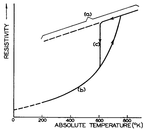
FIG. 8.—RESISTIVITY-TEMPERATURE CURVES FOR \beta -BRASS.
