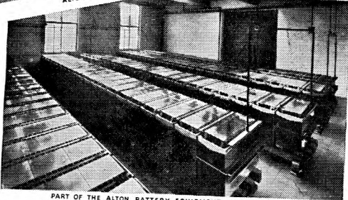
PART OF THE ALTON BATTERY EQUIPMENT INSTALLED AT A B.C. TRANSMITTING STATION
