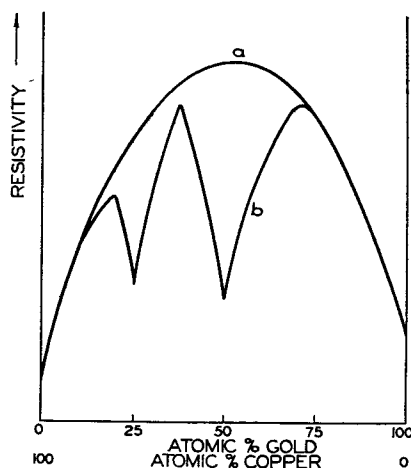
FIG. 7.—RESISTIVITY CURVES FOR COPPER-GOLD ALLOYS SUBJECTED TO HEAT-TREATMENT.
