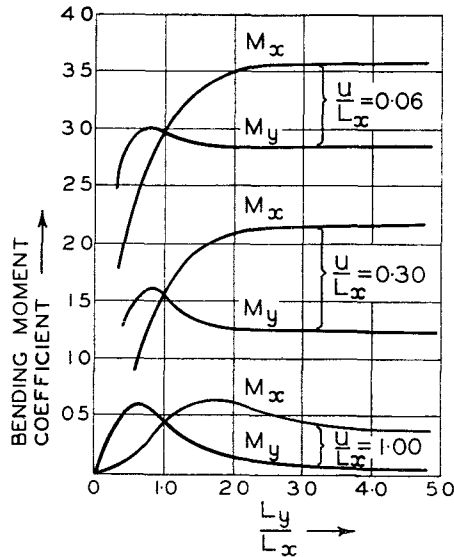
FIG. 9—BENDING MOMENT COEFFICIENTS FOR SLABS (CONCENTRATED LOADS).
