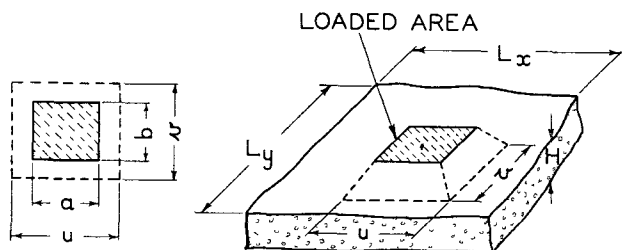
FIG. 8.—SPREAD OF A CONCENTRATED LOAD.
