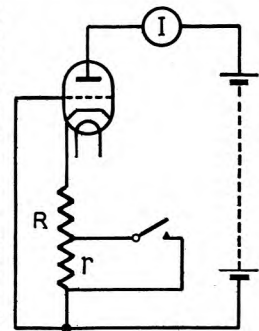
FIG. 7.—PRINCIPLE OF VALVE TEST.
