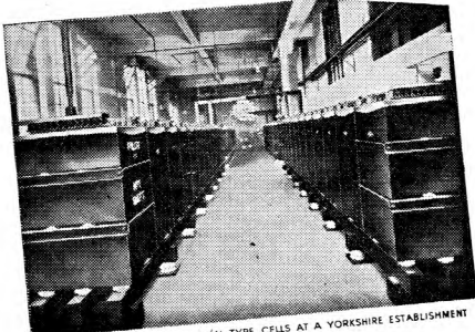
TWO ALTON BATTERIES OF JUN27/41 TYPE CELLS AT A YORKSHIRE ESTABLISHMENT
