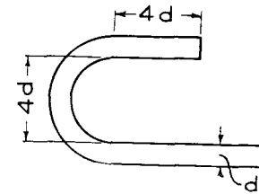
FIG. 5—HOOK FOR ADDITIONAL ANCHORAGE
