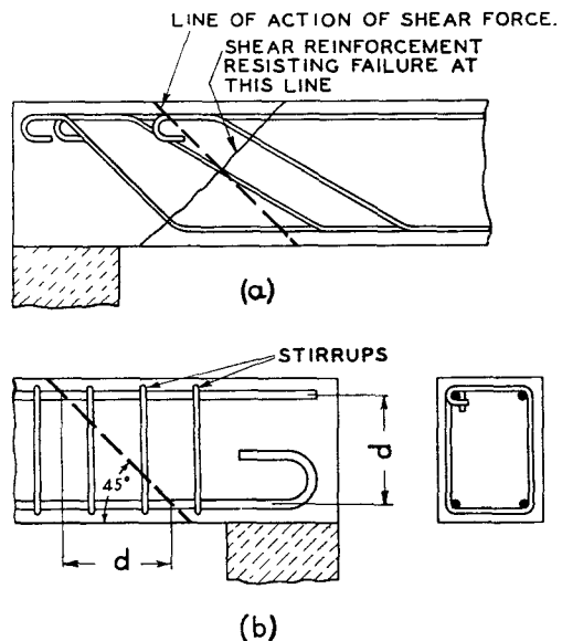
FIG. 4.—SHEAR REINFORCEMENT.
