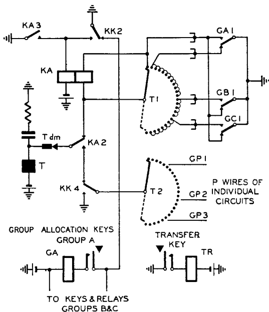
FIG. 7.—PART OF CONNECTING CIRCUIT, DIRECTORY ENQUIRY BUREAU.
