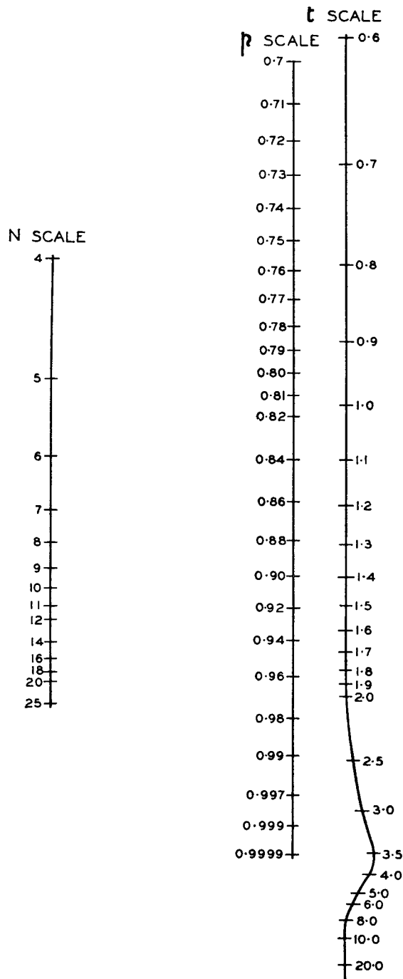
FIG. 2.—PROBABILITY CHART FOR "t" TEST.
