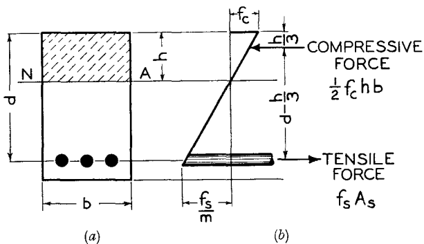
FIG. 1.—STRESS DIAGRAM.
