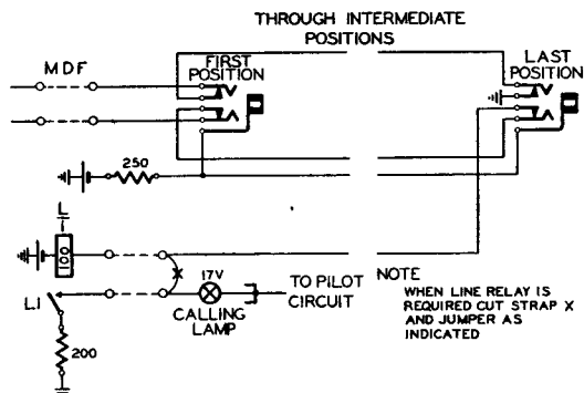
FIG. 5.—EXTENSION LINE CIRCUIT.
