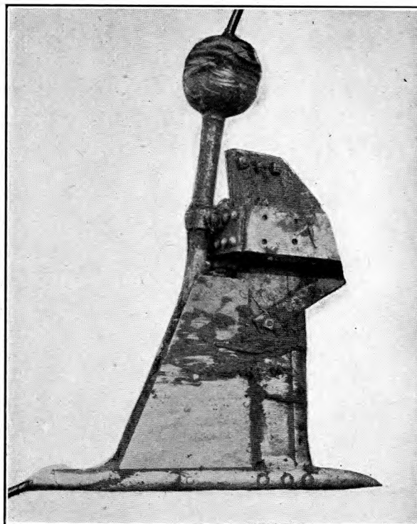
FIG. 1.—MOLEDRAINER MODIFIED FOR CABLING WORK.
