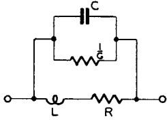
FIG. 1.—EQUIVALENT CIRCUIT OF IRON-CORED INDUCTANCE.
