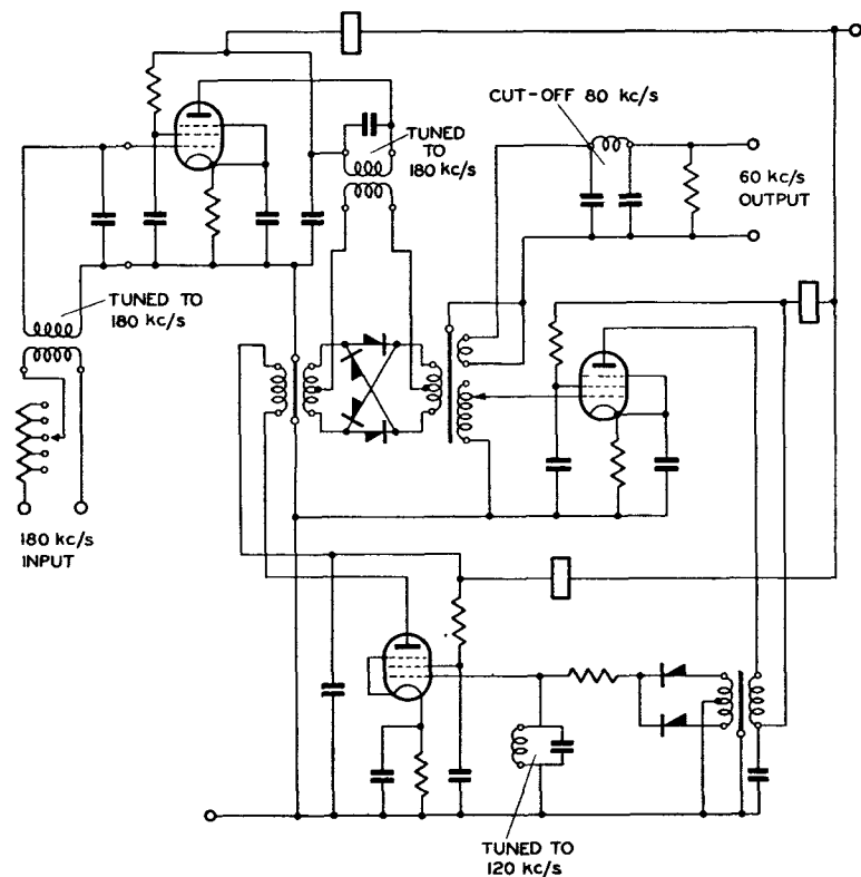
FIG. 3.—180 TO 60 KC/S FREQUENCY DIVIDER.
