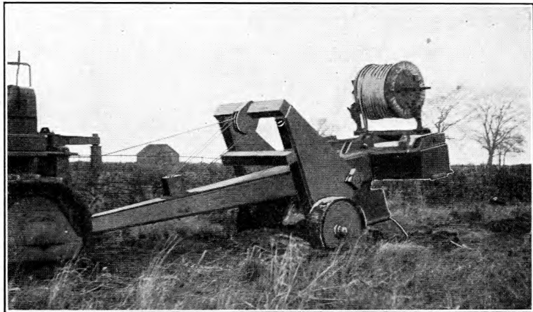
FIG. 4.—RIPPER PLOUGH.
