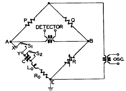
FIG. 4.—SIMPLE RESONANCE BRIDGE.
