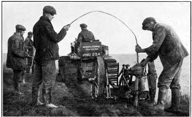
FIG. 2.—CABLE-LAYING WITH MOLEDRAINER.
