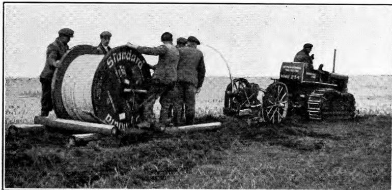
FIG. 3.—CABLE-LAYING WITH MOLEDRAINER AND SLEDGE.
