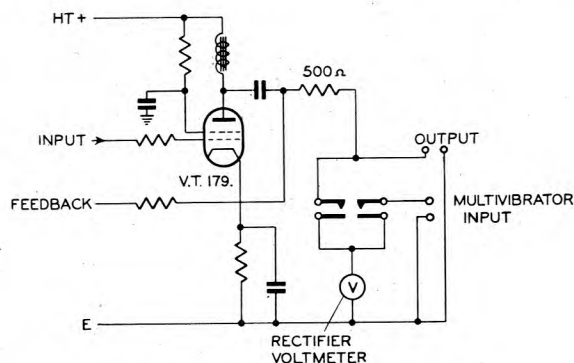
FIG. 4.—OUTPUT CIRCUIT SCHEMATIC.
