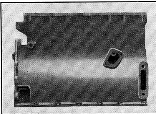
FIG. 3.—REPAIR OF MOTOR VEHICLE CYLINDER BLOCK.
