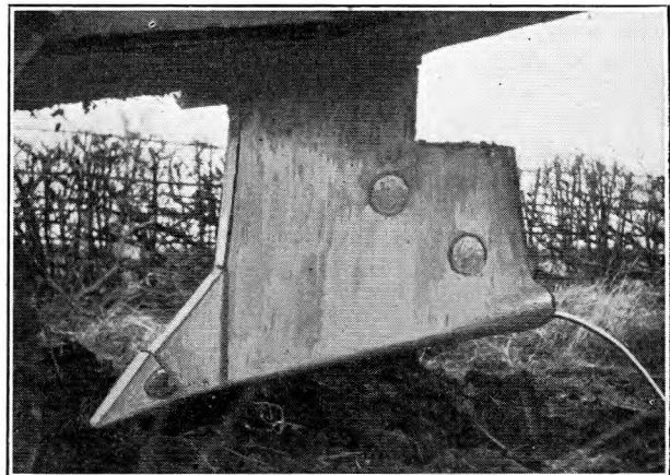
FIG. 5.—RIPPER BLADE WITH CABLE-LAYING MODIFICATION.
