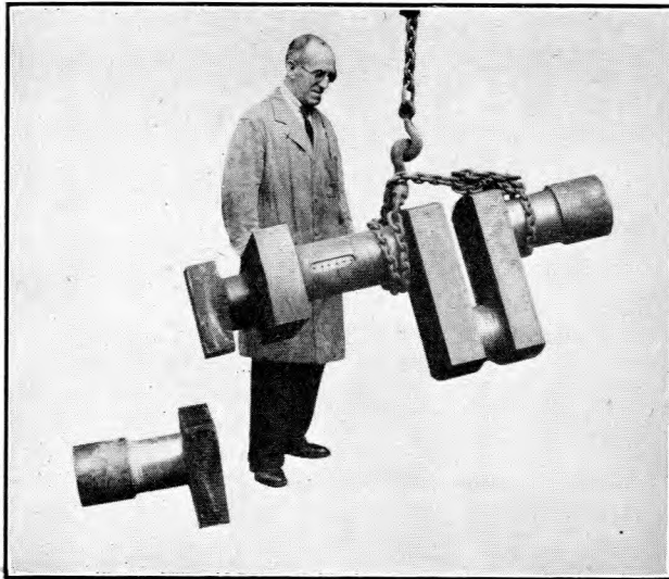
FIG. 2.—REPAIR OF 1\frac{1}{2} TON LOCOMOTIVE CRANKSHAFT.
