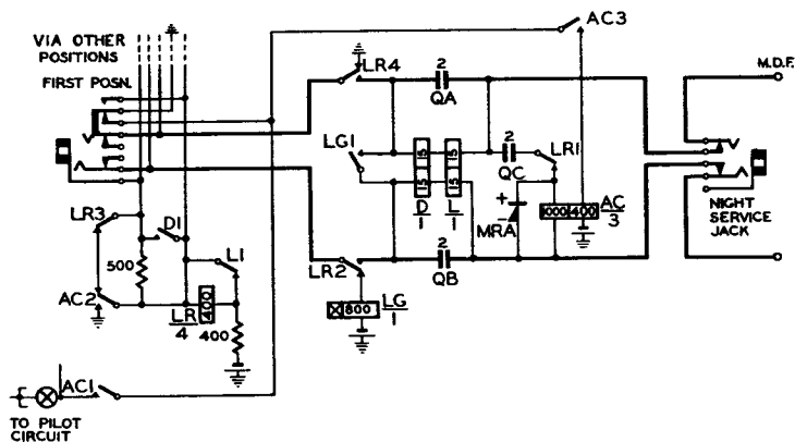
FIG. 7.—EXCHANGE LINE CIRCUIT.
