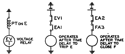
FIG. 4.—BASIC CIRCUITS OF REDESIGNED CHANGE-OVER EQUIPMENT.
