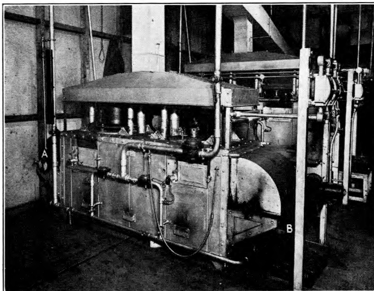
FIG. 3.—CONVEYORISING FURNACE.
