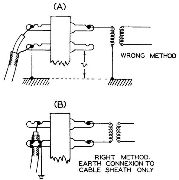
FIG. 7.—TERMINATING COAXIAL CABLES ON PANEL TAG BLOCKS.
