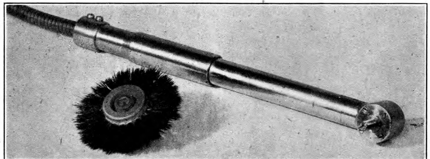
FIG. 3.—BANK CLEANING BRUSH AND TOOL.
