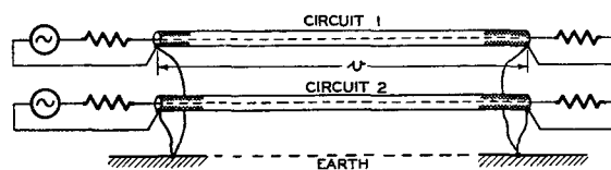
FIG. 2.—CABLE SHEATHS EARTHED DIRECT.
