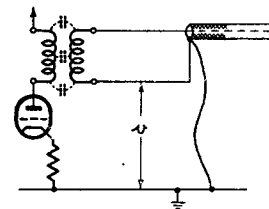
Fig. 5.—CIRCUIT CONDITION LIKELY TO GIVE RISE TO CROSSTALK.
