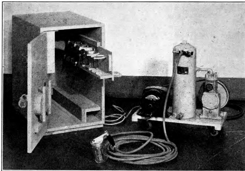
FIG. 1.—DEKALIN SPRAY CLEANING APPARATUS.
