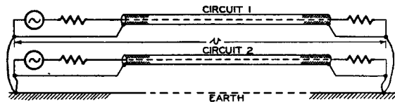
FIG. 3.—CABLE SHEATHS EARTHED VIA SERIES IMPEDANCES.
