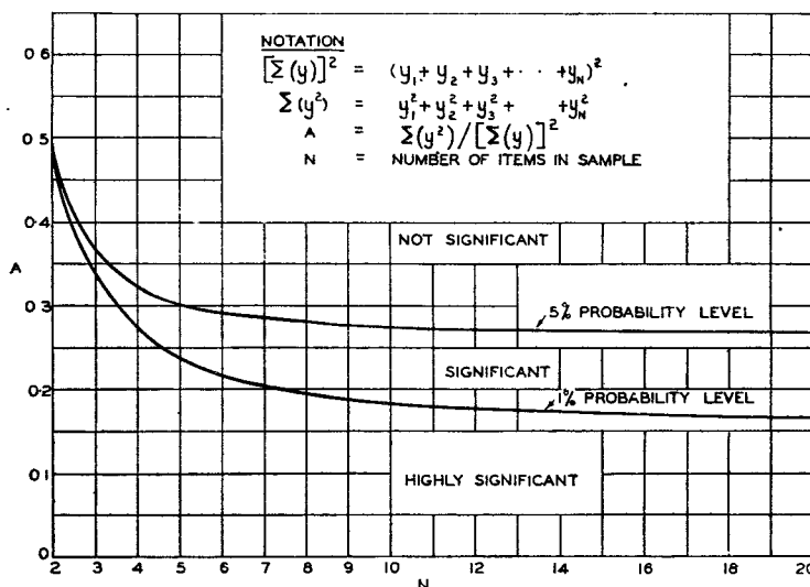
FIG. 1.—SINGLE MEAN "t" TEST PROBABILITY CHART FOR 5% AND 1% LEVELS
