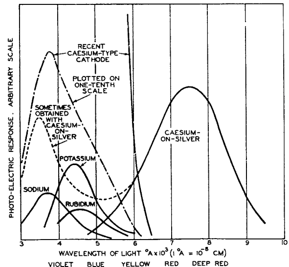
FIG. 3.—COLOUR CHARACTERISTICS OF VARIOUS CATHODES.
