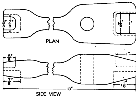
FIG. 6.—LAG WRENCH
