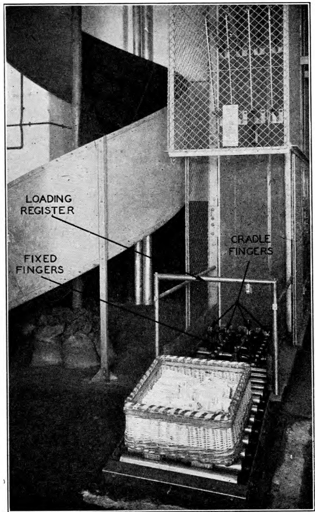
FIG. 5.—LOADING PLATFORM.
