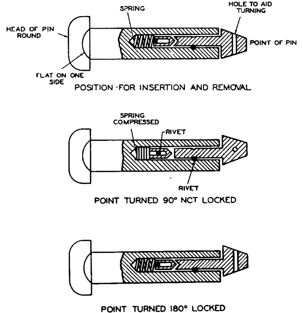
FIG. 7.—ECCENTRIC POINT CONNECTING PIN
