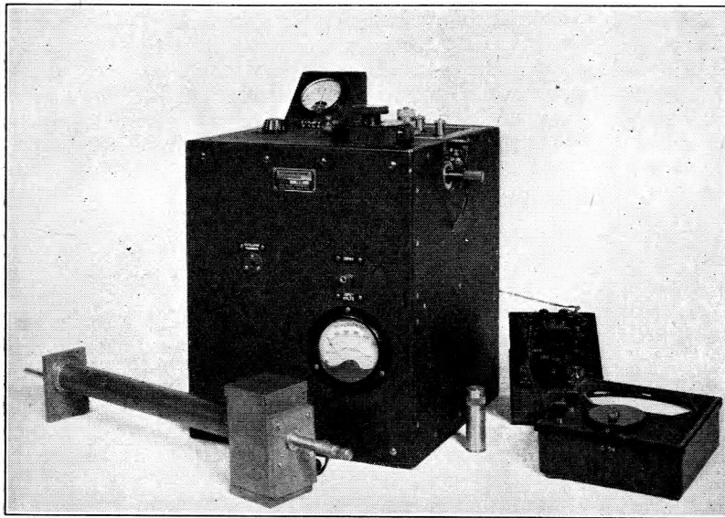
FIG. 6.—REACTANCE VARIATION APPARATUS. 5-50 Mc/s AND 50-250 Mc/s.
