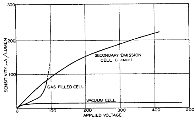
FIG. 2.—VARIATION OF SENSITIVITY WITH APPLIED VOLTAGE.
