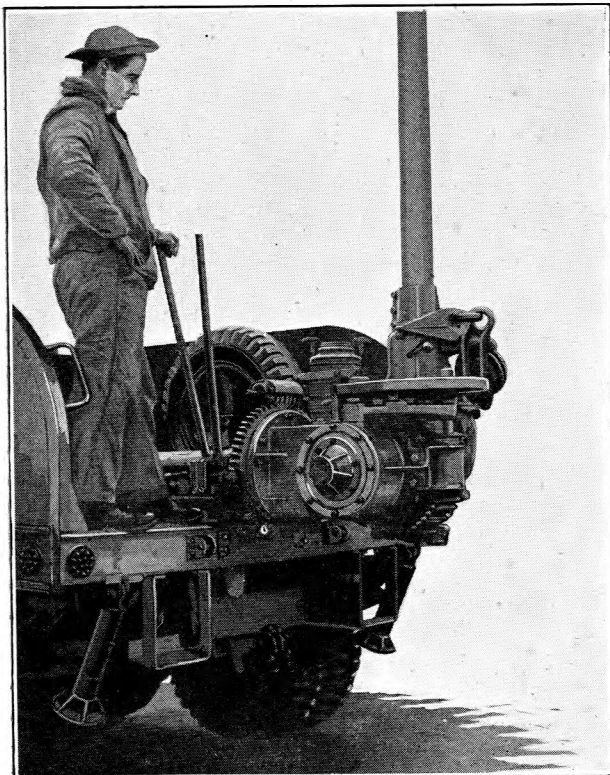
FIG. 1.—EARTH BORING MACHINE
