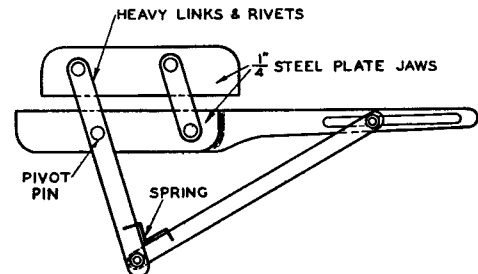
FIG. 8.—WIRE TENSIONING TONGS.
