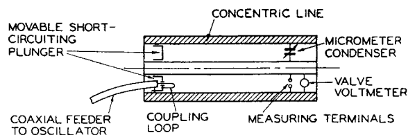
FIG. 7.—REACTANCE VARIATION CIRCUIT. 50-250 Mc/s.
