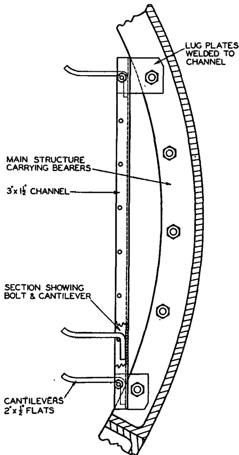
FIG. 4.—CABLE BEARER.
