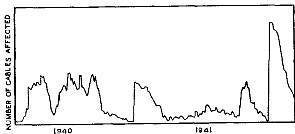
FIG. 1.—GRAPH ILLUSTRATING INCIDENCE OF CABLE FAULTS.
