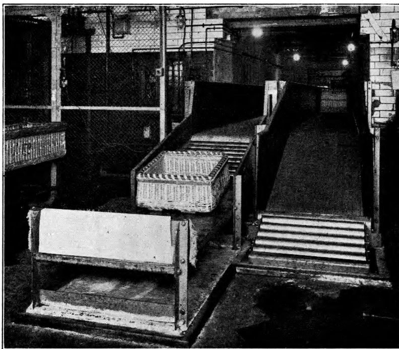
FIG. 2.—HORIZONTAL CONVEYOR BANDS SEEN FROM WEST BUILDING.
