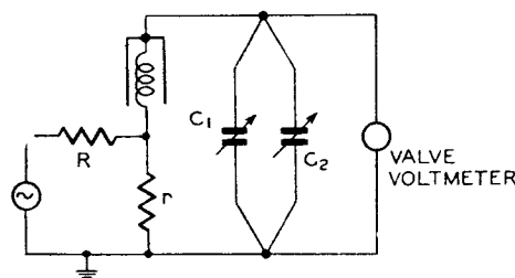
FIG. 5.—REACTANCE VARIATION CIRCUIT, 5-50 Mc s.
