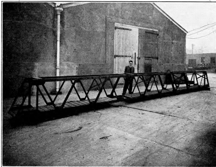
FIG. 6.—3-SECTION EMERGENCY CABLE BRIDGE.
