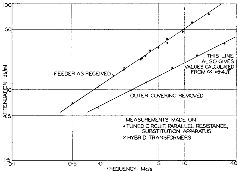
FIG. 4.—UNSCREENED TWIN FEEDER ATTENUATION CHARACTERISTICS.
