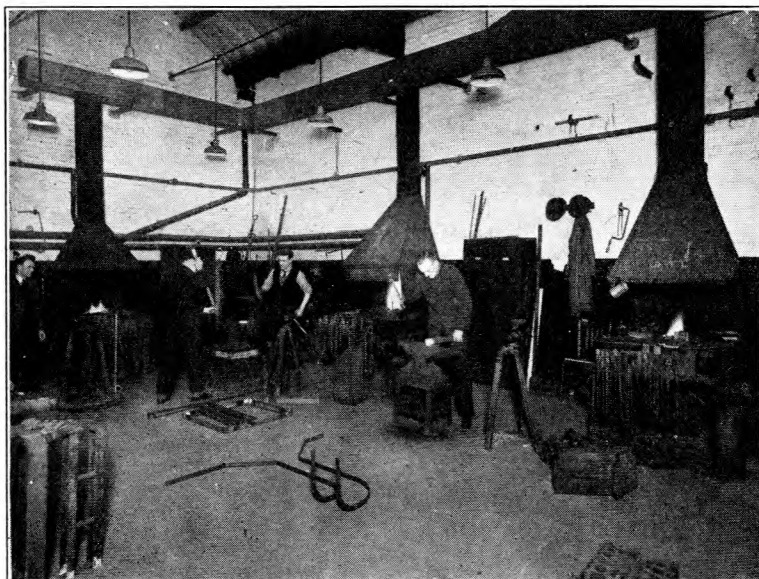
FIG. 1.—BLACKSMITH'S SHOP.
