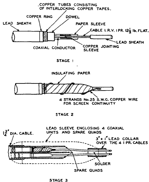
FIG. 2.—TEMPORARY REPAIR TO COAXIAL CABLE.
