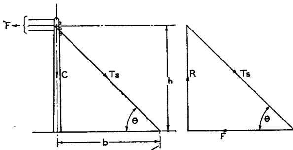
FIG. 1.—FORCES ACTING ON STAYED POLE.
