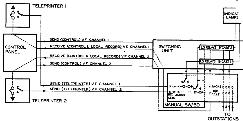
FIG. 3.—SCHEMATIC DIAGRAM OF TELEPRINTER BROADCAST SYSTEM.
