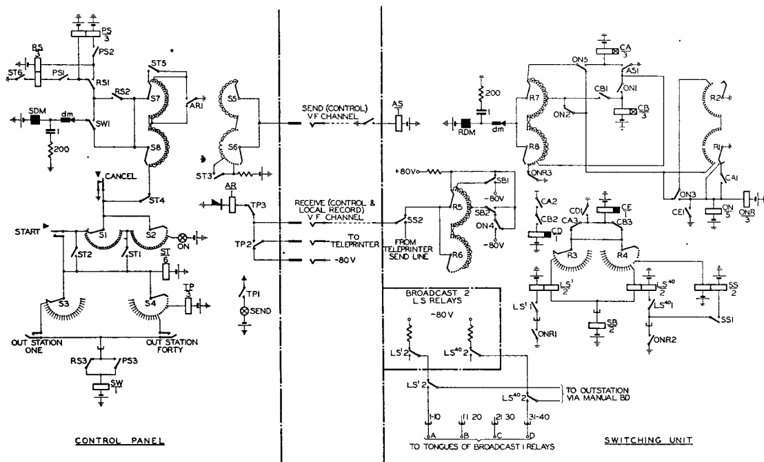
FIG. 4.—CIRCUIT ELEMENTS ASSOCIATED WITH BROADCAST 1.
