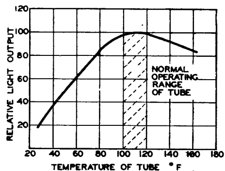
FIG. 6.—GRAPH ILLUSTRATING EFFECT OF TUBE TEMPERATURE ON EFFICIENCY.
