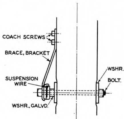
FIG. 4.—METHOD OF ATTACHMENT FOR SUSPENSION WIRE.
