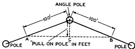
FIG. 2.—"PULL-ON-POLE" MEASUREMENT.
