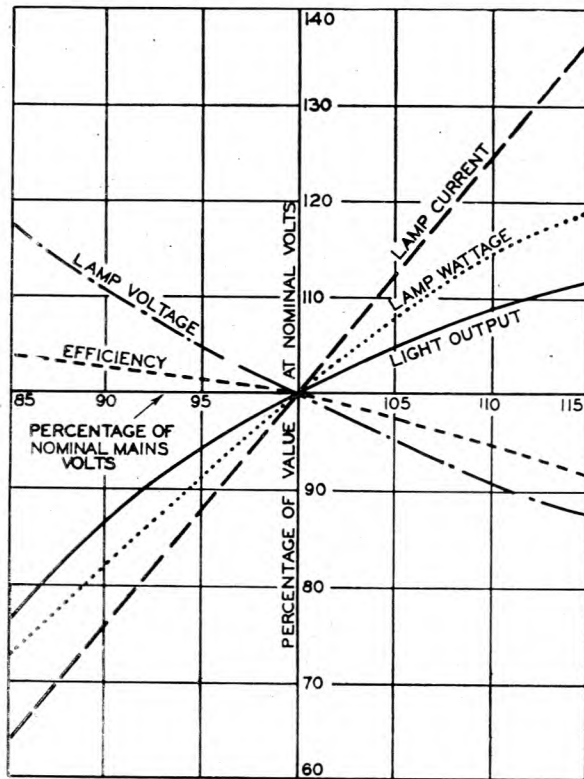
FIG. 7.—GRAPH ILLUSTRATING EFFECT OF SUPPLY VOLTAGE VARIATIONS.
