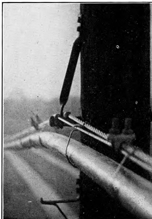
FIG. 5.—CABLE SUPPORTED BY MAIN AND AUXILIARY SUSPENSION WIRES.
