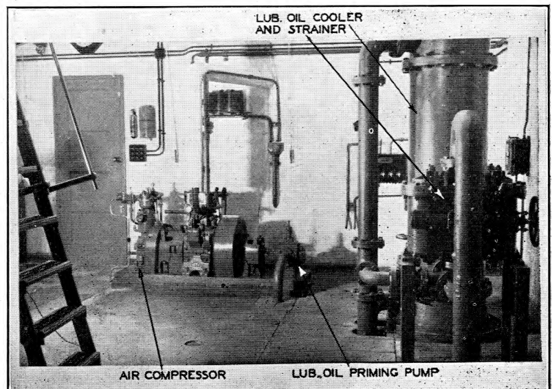
FIG. 5. AUXILIARY EQUIPMENT.
