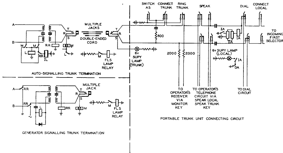
FIG. 5.—CIRCUIT ARRANGEMENTS FOR SLEEVE CONTROL NON-DIRECTOR EXCHANGE UNIT.
