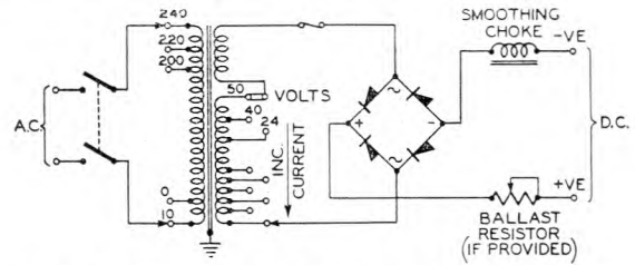
FIG. 4.—CIRCUIT ARRANGEMENT OF RECTIFIER UNIT.
