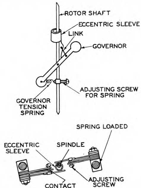
FIG. 2.—GOVERNOR DETAILS. WALLACE AND TIERNAN MOTOR.
