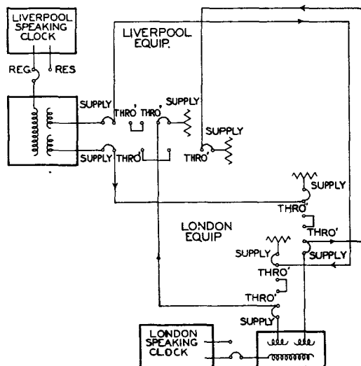
FIG. 2.—OMNIBUS TRUNK CIRCUIT CONNECTIONS AT REPEATER STATIONS.
