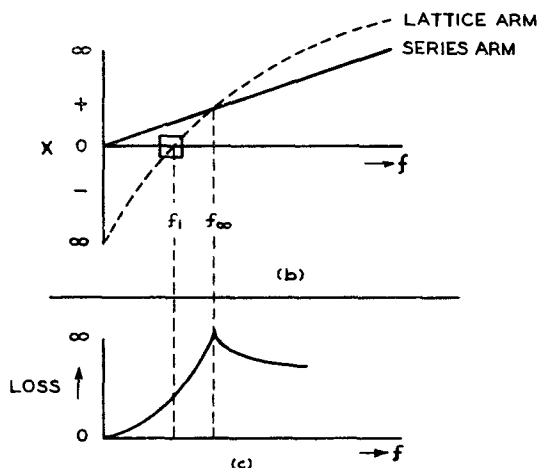
FIG. 2.—REACTANCE AND LOSS CURVES FOR A SIMPLE LOW-PASS LATTICE FILTER NETWORK.
