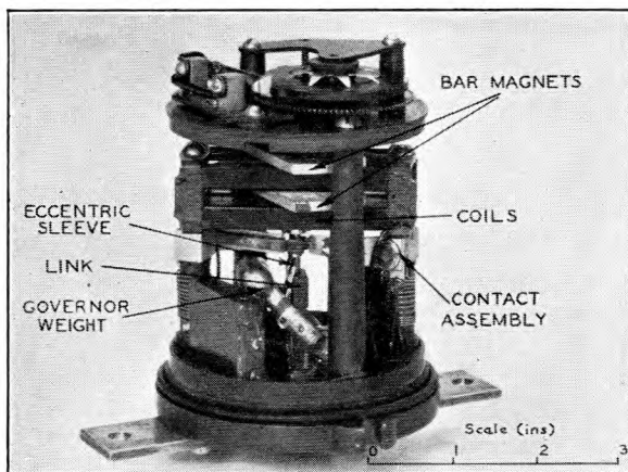
FIG. 1.—WALLACE AND TIERNAN IMPULSE MOTOR.
