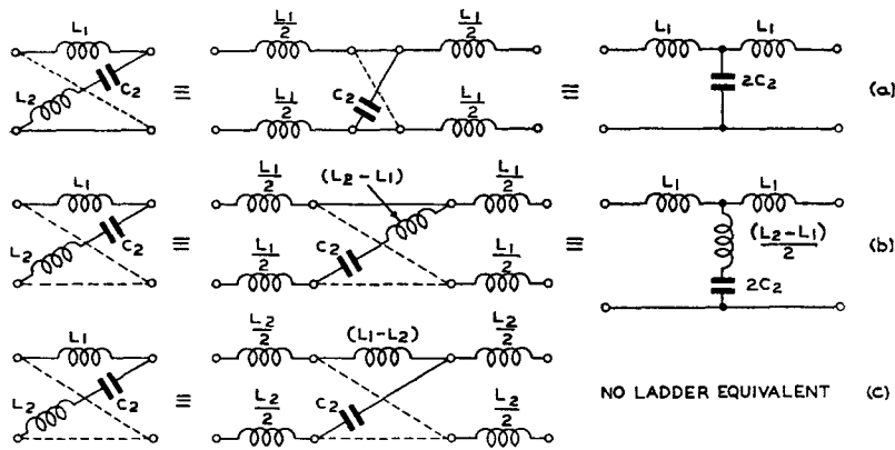
FIG. 4.—EQUIVALENT LATTICE AND LADDER NETWORKS.
