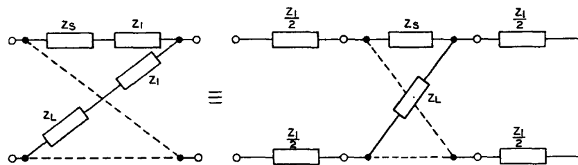
FIG. 3.—LATTICE NETWORK WITH COMMON SERIES ELEMENT AND EQUIVALENT.
