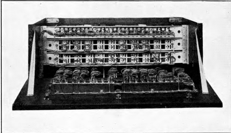
FIG. 3.—FRONT VIEW OF UNIT—TOP REMOVED AND FRONT OPEN.
