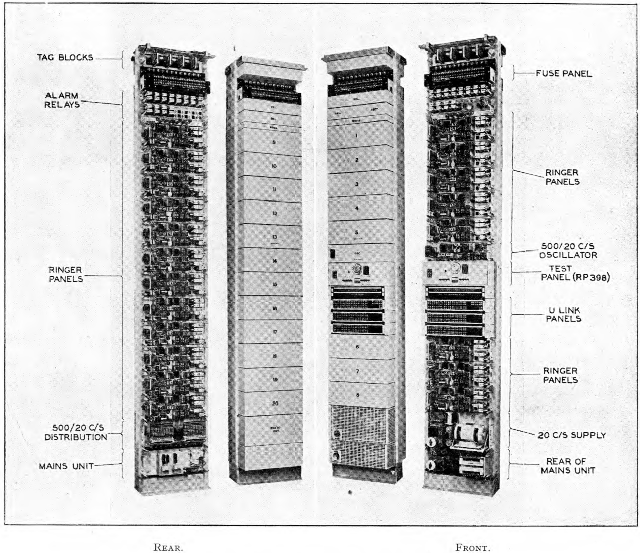
FIG. 6.—REAR AND FRONT VIEWS OF COMPLETE BAY.
