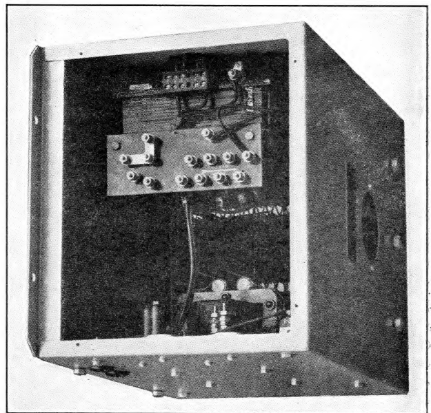
FIG. 2.—RECTIFIER WITH TOP COVER REMOVED.
