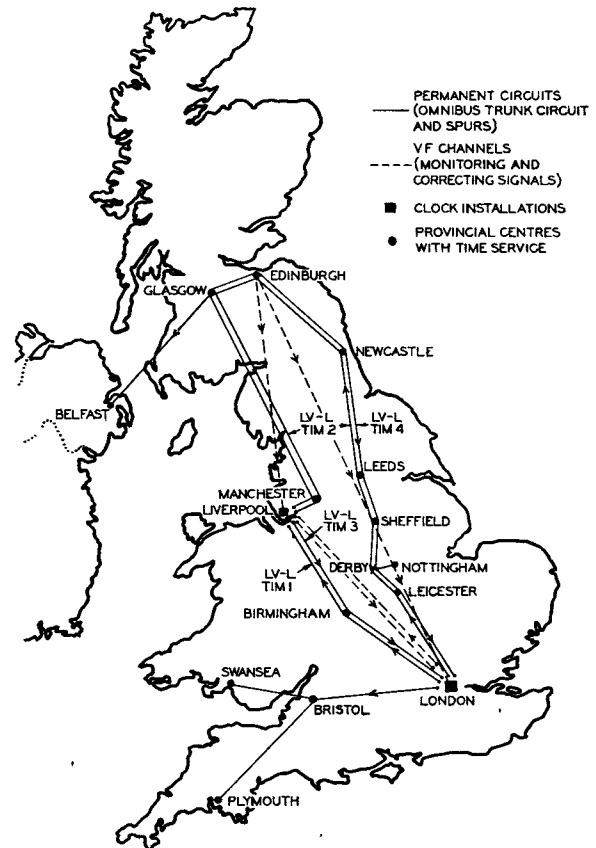
FIG. 1.—DISTRIBUTION CIRCUITS.
