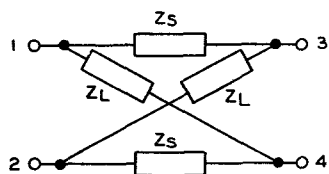
FIG. 1.—SYMMETRICAL LATTICE NETWORK.
