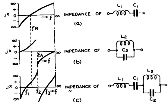
FIG. 5.—IMPEDANCE CURVES OF REACTIVE CIRCUITS.
