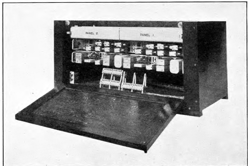
FIG. 2.—REAR VIEW OF UNIT—TOP REMOVED AND BACK OPEN.
