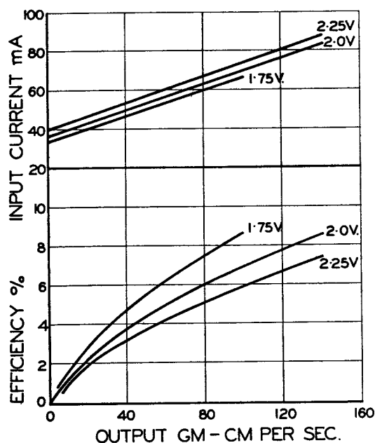
FIG. 7.—PERFORMANCE CURVES OF EXPERIMENTAL MOTOR.
