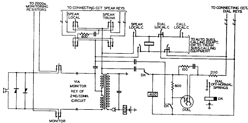
FIG. 6.—OPERATOR'S CIRCUIT.
