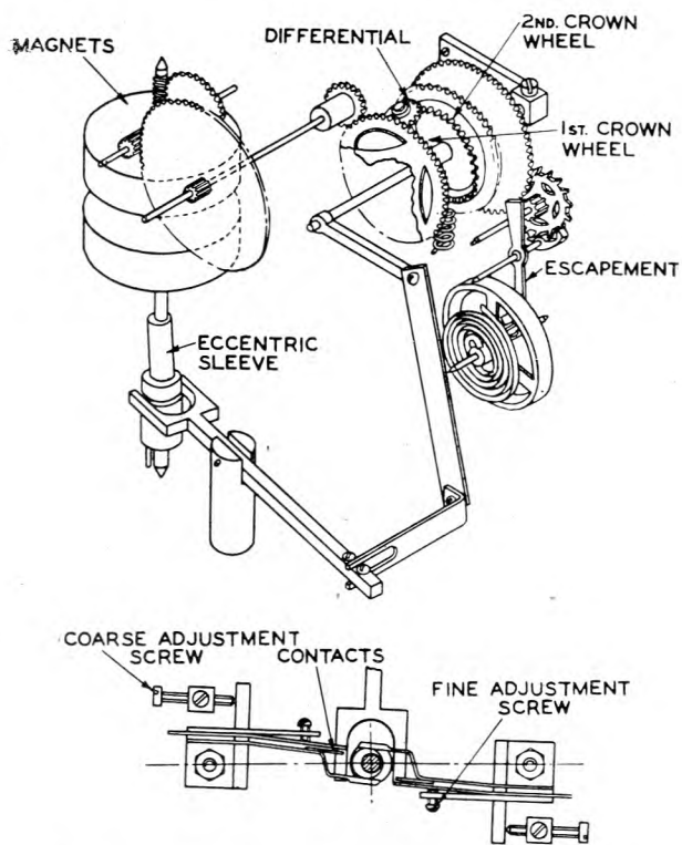
FIG. 6.—CONSTRUCTIONAL DETAILS OF EXPERIMENTAL MOTOR.
