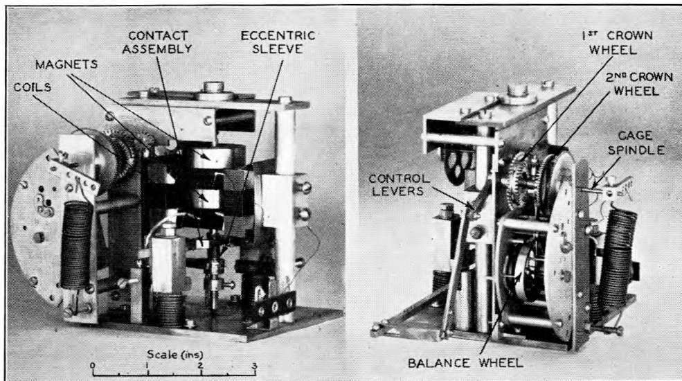
FIG. 5.—EXPERIMENTAL IMPULSE MOTOR.
