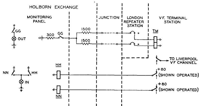
FIG. 4.—MONITORING CIRCUIT
