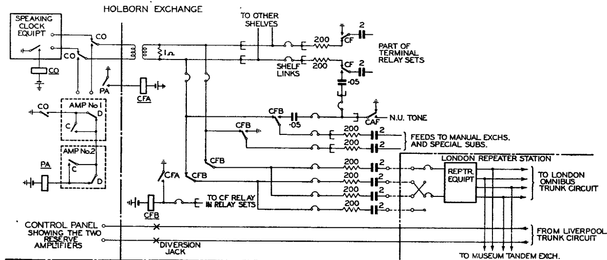
FIG. 3.—TIM DISTRIBUTION (LONDON).
