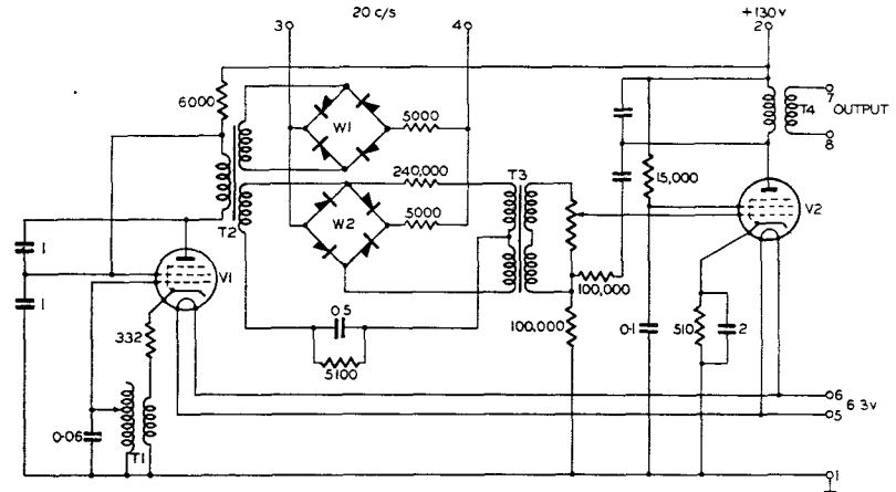
FIG. 4.—500 c/s OSCILLATOR WITH STATIC "CHOPPER."
