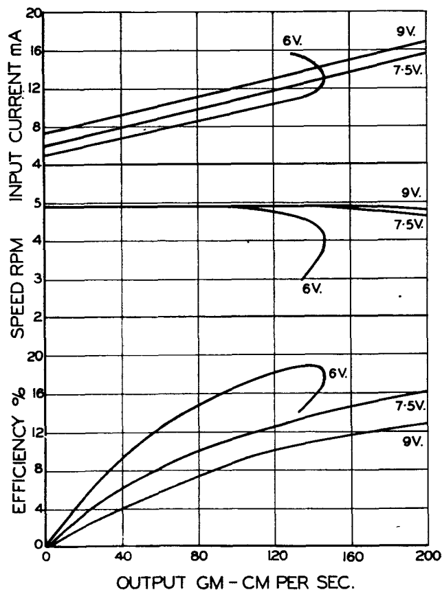
FIG. 4.—PERFORMANCE CURVES OF WALLACE AND TIERNAN MOTOR.
