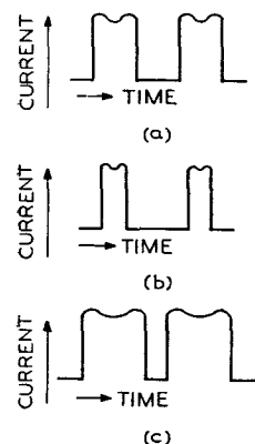
FIG. 3.—WAVE SHAPE OF MOTOR CURRENT IMPULSES.
