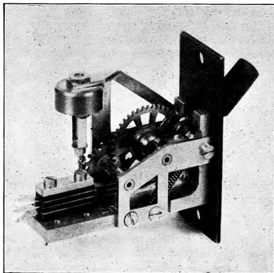
FIG. 1.—MECHANISM OF DELAYED ACTION KEY.
