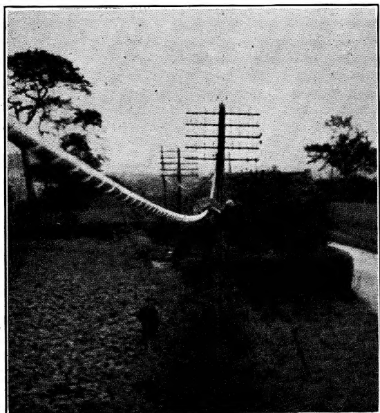
FIG. 4. CABLE SPAN PARTLY COMPLETED.
