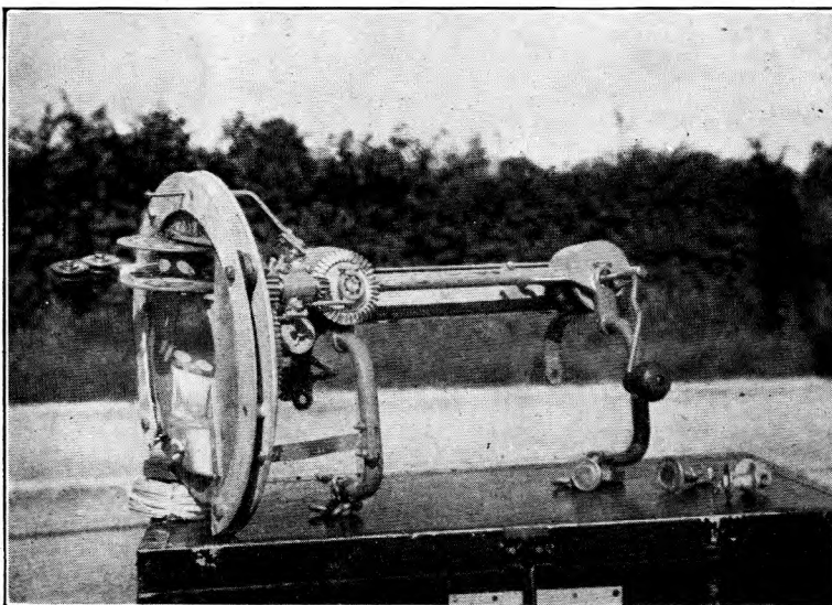
FIG. 2. THE NEALE SPINNER (SHOWING TENSIONING WHEELS).
