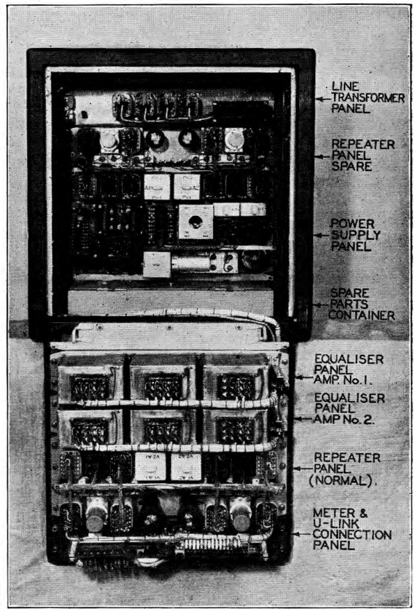
FIG. 4.—REPEATER C.T. No. 3.
