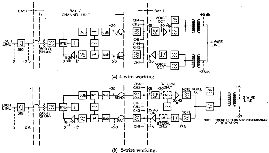
FIG. 1.—BLOCK SCHEMATIC OF ONE TERMINAL.
