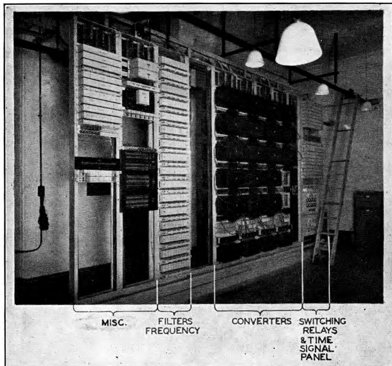
FIG. 6.—PART OF APPARATUS ROOM.
