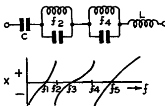
FIG. 4.—EXAMPLE FOR FOSTER'S THEOREM.
