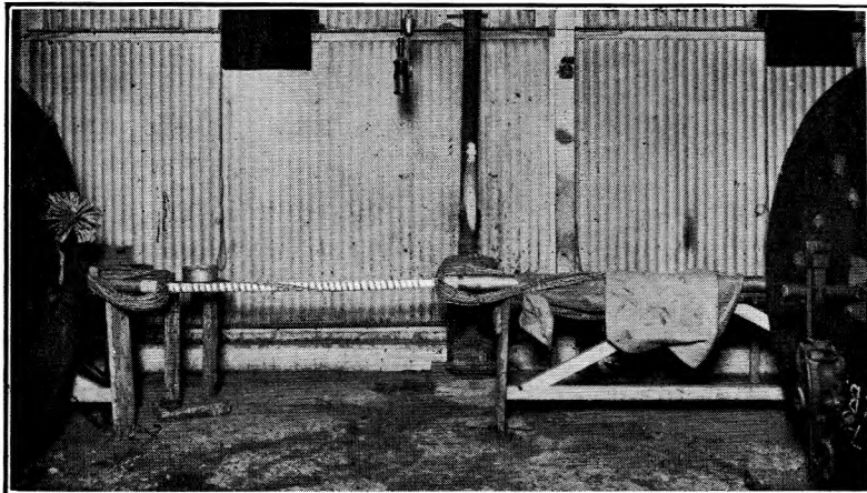
FIG. 3.—“UNIDIAMETER” JOINT PARTIALLY COMPLETED.
