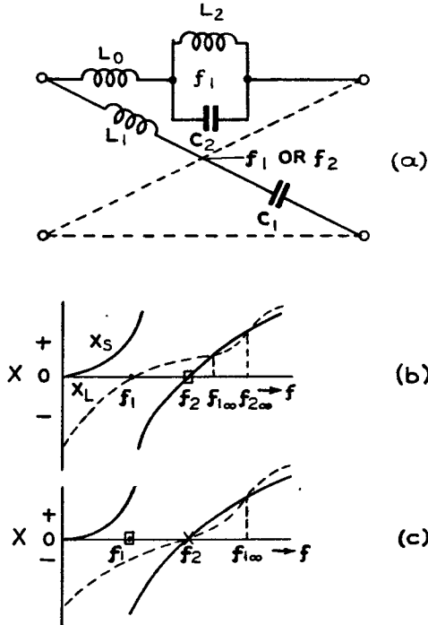
FIG. 5.—LOW PASS FILTER WITH ALTERNATIVE CHARACTERISTICS.
