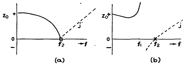
FIG. 6.—ALTERNATIVE IMPEDANCES.
