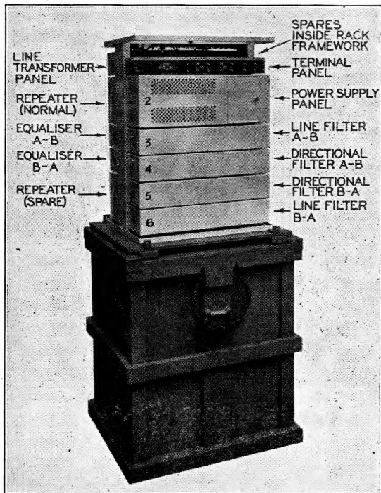
FIG. 3.—REPEATER C.T. No. 1, Mk.1.
