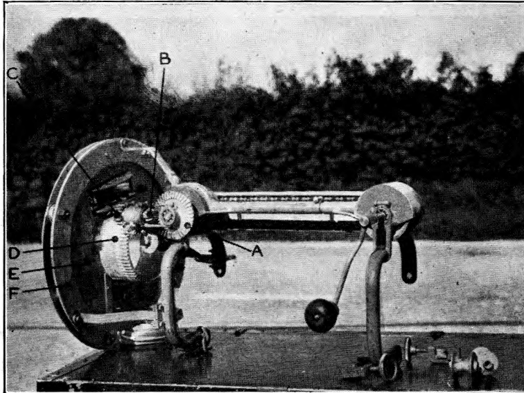
FIG. 1. THE NEALE SPINNER.
