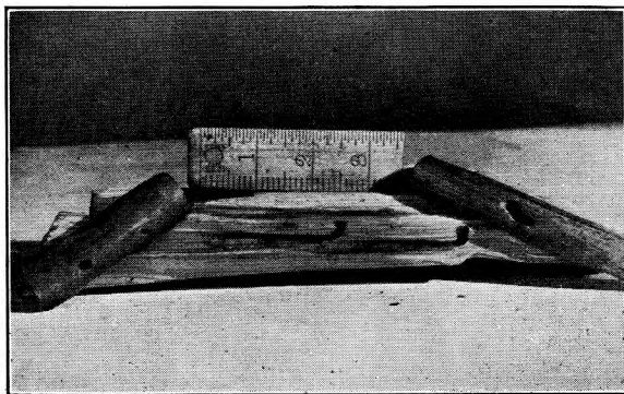
FIG. 2.—EFFECT OF LARVA ON LEAD.
