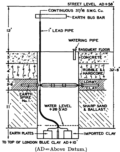
FIG. 7.—C.T.O. MAIN EARTH.
