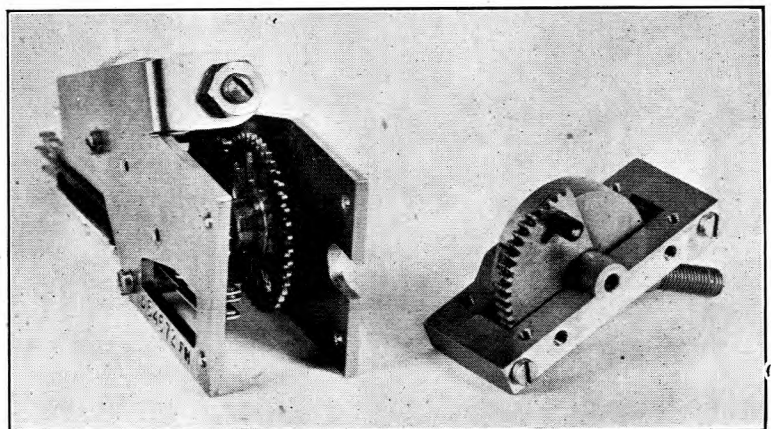
FIG. 5.—GOVERNOR AND HANDLE UNITS.
