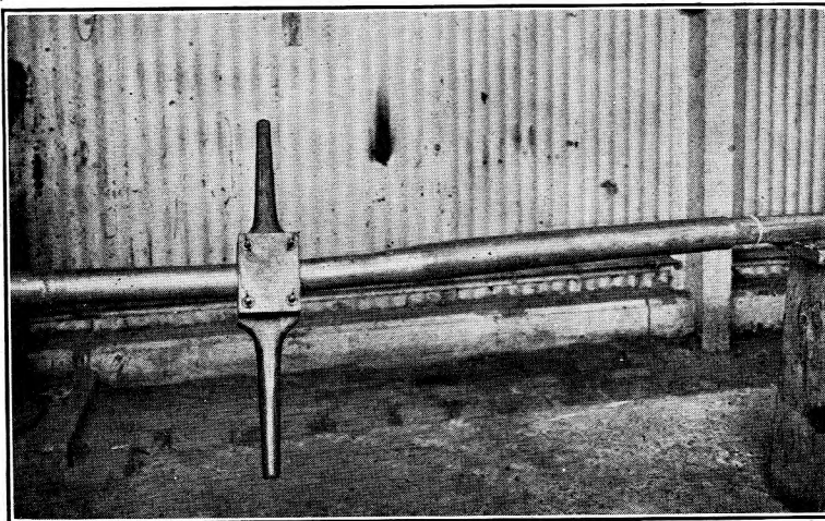
FIG. 5.—SWAGE CLAMPED TO CABLE.
