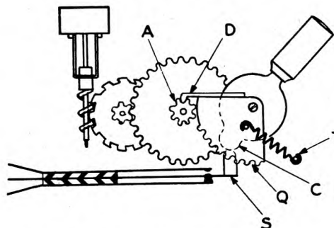
FIG. 2.—ESSENTIAL FEATURES OF KEY.
