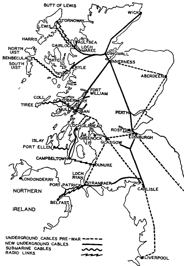
FIG. 3.—ILLUSTRATING WARTIME GROWTH OF UNDERGROUND CABLE NETWORK IN SCOTLAND.
