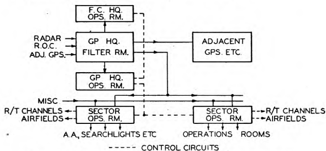
FIG. 3.—DISTRIBUTION OF PLOTTING INFORMATION.
