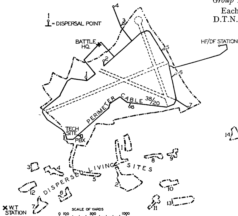
FIG. 1.—LAYOUT OF TYPICAL BOMBER AIRFIELD.
