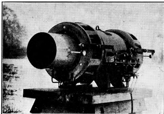
FIG. 3.—SIREN WITH "CUCKOO" ATTACHMENT.
