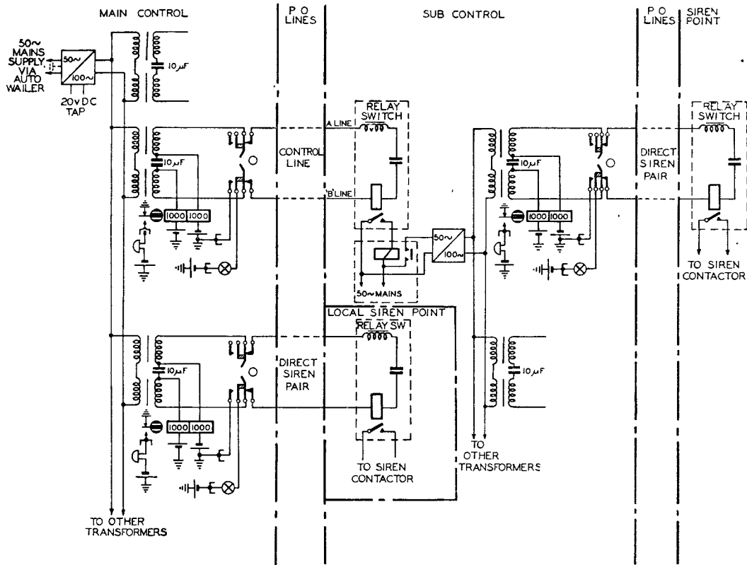
FIG. 5.—CIRCUIT ARRANGEMENTS FOR REMOTE CONTROL OF SIRENS.
