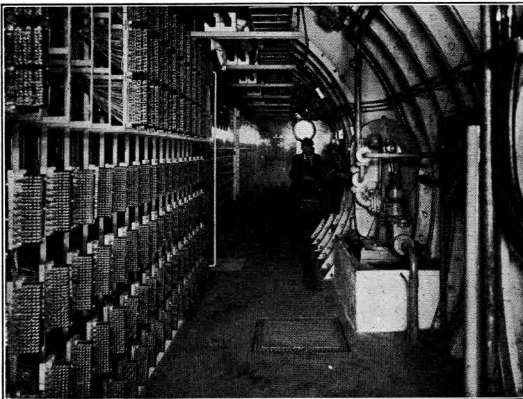
FIG. 5.—M.D.F. AND REPEATER EQUIPMENT IN DEEP-LEVEL PROTECTION.
