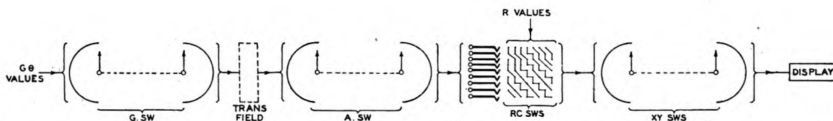
FIG. 2.—CIRCUIT PRINCIPLES OF THE CALCULATOR.
