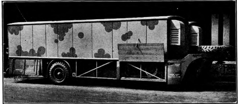
FIG. 2.—VEHICLE FOR 12-CIRCUIT CARRIER EQUIPMENT.
