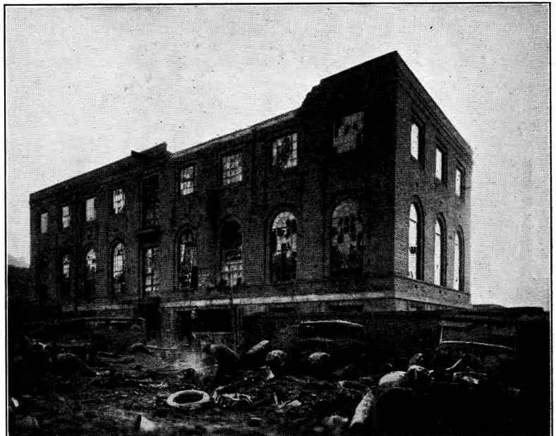
FIG. 3.—DAMAGE TO AN AUTOMATIC EXCHANGE (VICTORIA EXCHANGE, BIRMINGHAM).
