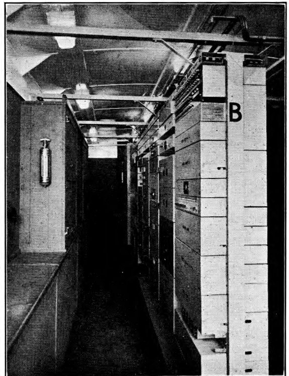
FIG. 3.—INTERIOR OF VEHICLE FITTED WITH 12-CIRCUIT CARRIER EQUIPMENT.
