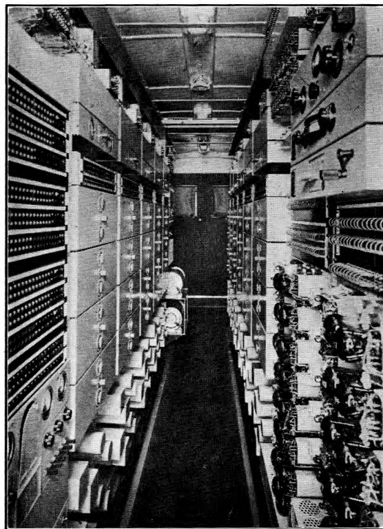
FIG. 5.—D.T.N. MOBILE TELEGRAPH TERMINAL (VIEWED FROM FRONT).
