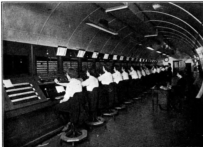
FIG. 1.—TELEPRINTER SWITCHING CENTRE.
