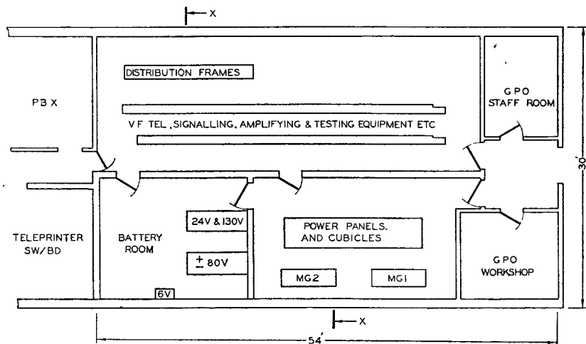
FIG. 2.—TYPICAL LAYOUT OF D.T.N. EQUIPMENT IN NISSEN HUT.
