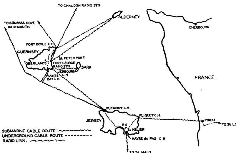
FIG. 1.—CHANNEL ISLANDS COMMUNICATIONS.
