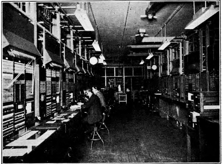
FIG. 3.—TRUNK TEST RACKS IN CITADEL.
