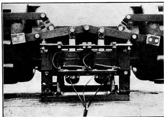
FIG. 4.—OPERATING LINKAGE OF "CUCKOO" ATTACHMENT.
