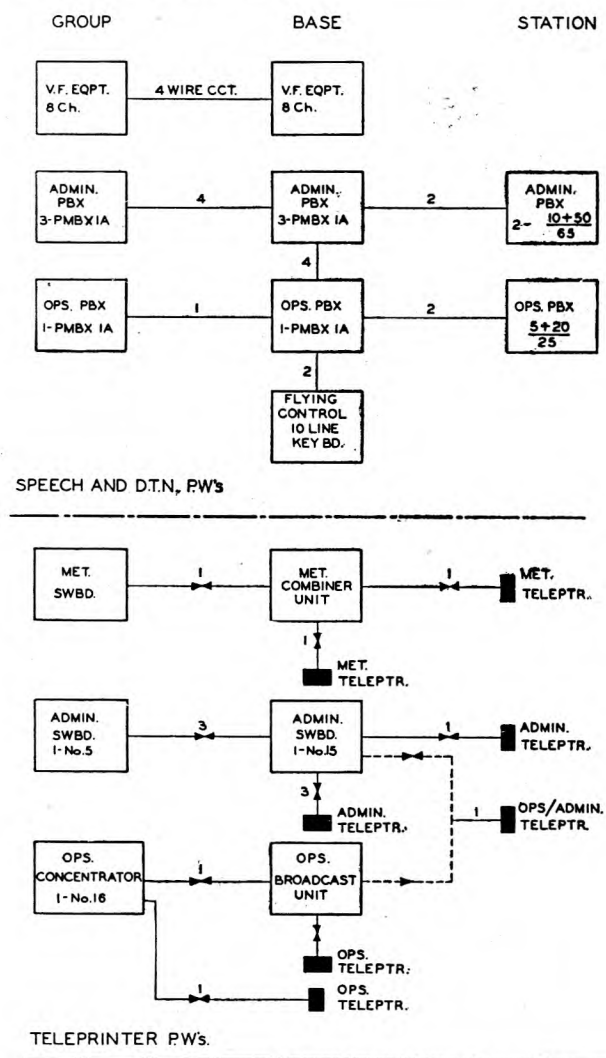
FIG. 3.—PRIVATE WIRE FACILITIES FOR BASE ORGANISATION.
