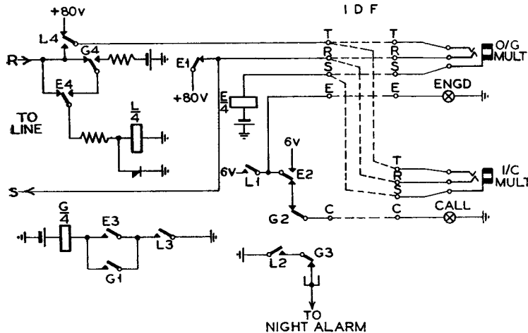
FIG. 4.—CIRCUIT SCHEMATIC OF MANUAL LINE EQUIPMENT.
