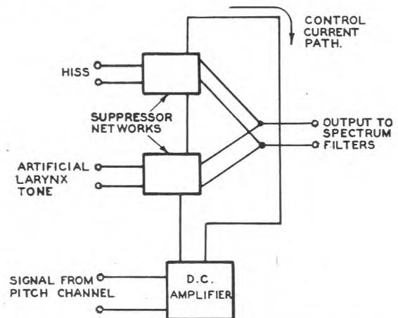
FIG. 8.—PRINCIPLE OF THE SWITCHING CIRCUIT.
