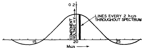
FIG. 9.—SPECTRUM OF FREQUENCIES TRANSMITTED FOR THE MEASUREMENT OF CABLE IRREGULARITIES.
