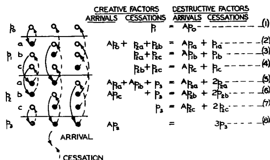
FIG. 6.—BASIC EQUATIONS FOR GROUP OF THREE CHANNELS, FULL AVAILABILITY.
