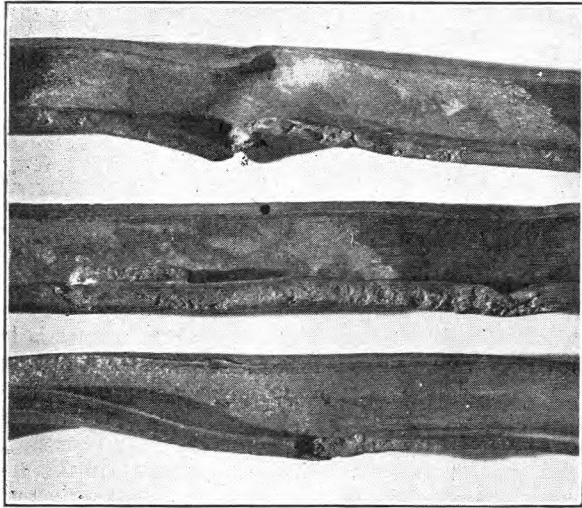
FIG. 4.—EXAMPLE OF RED LEAD EXTRUDED IN THE SHEATH OF A CABLE.
