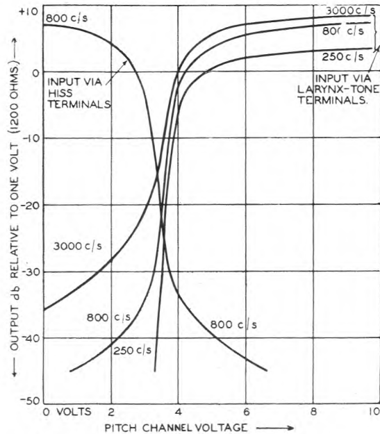
FIG. 9.—TYPICAL SWITCHING CIRCUIT CHARACTERISTIC.
