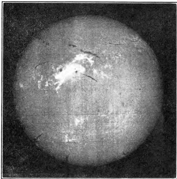
FIG. 5.—THE GREAT SOLAR FLARE OF 25TH JULY, 1946.
