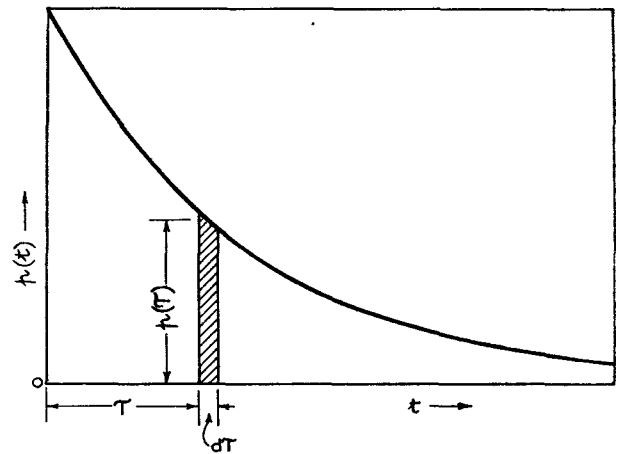
FIG. 2.—EXPONENTIAL DISTRIBUTION.
