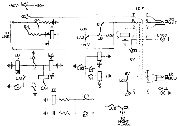
FIG. 5.—CIRCUIT SCHEMATIC OF AUTO-MANUAL LINE EQUIPMENT.
