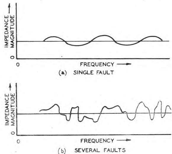
FIG. 1.—TYPICAL IMPEDANCE/FREQUENCY CHARACTERISTICS
