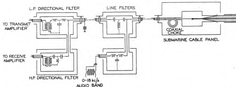
FIG. 11.—EARTHING AND SCREENING ARRANGEMENTS AT ALDEBURGH.
