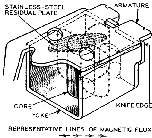
FIG. 3.—MAGNETIC CIRCUIT.
