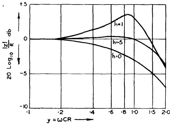
FIG. 4.—ANODE LOAD INCLUDING REACTANCES.
