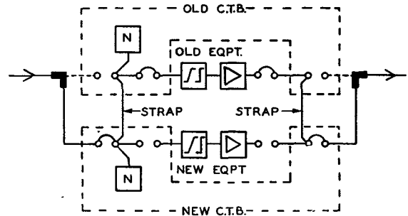
FIG. 2.—CONNECTIONS AT EXISTING STATION BEFORE NEW EQUIPMENT IS CUT IN.
