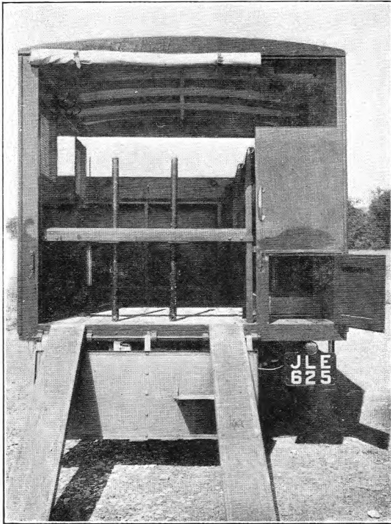
FIG. 4.—REAR VIEW.
