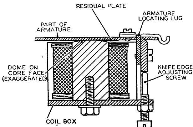
FIG. 4.—CROSS-SECTION OF COIL BOX AND ARMATURE.
