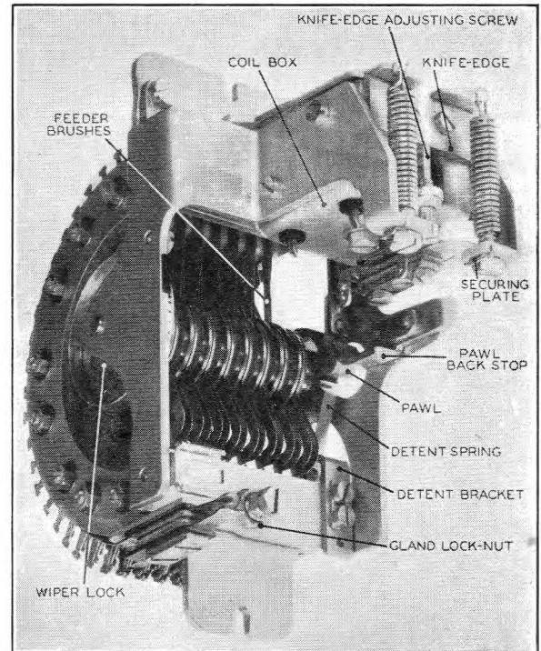
FIG. 2.—P.O. UNISELECTOR TYPE 2—8 LEVEL.
