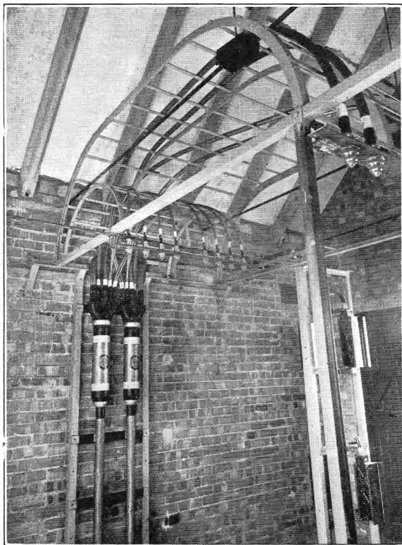
FIG. 7.—CABLE TERMINATIONS.
