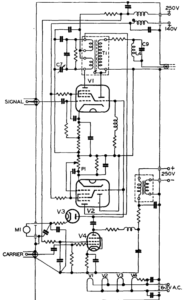
FIG. 5.—FREQUENCY CHANGER CIRCUIT.
