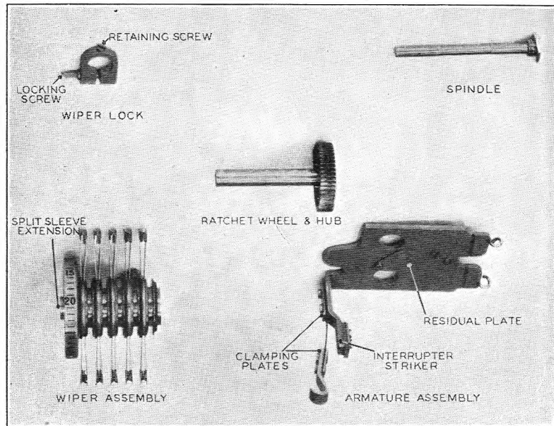
FIG. 6.—PARTS OF UNISELECTOR TYPE 2.
