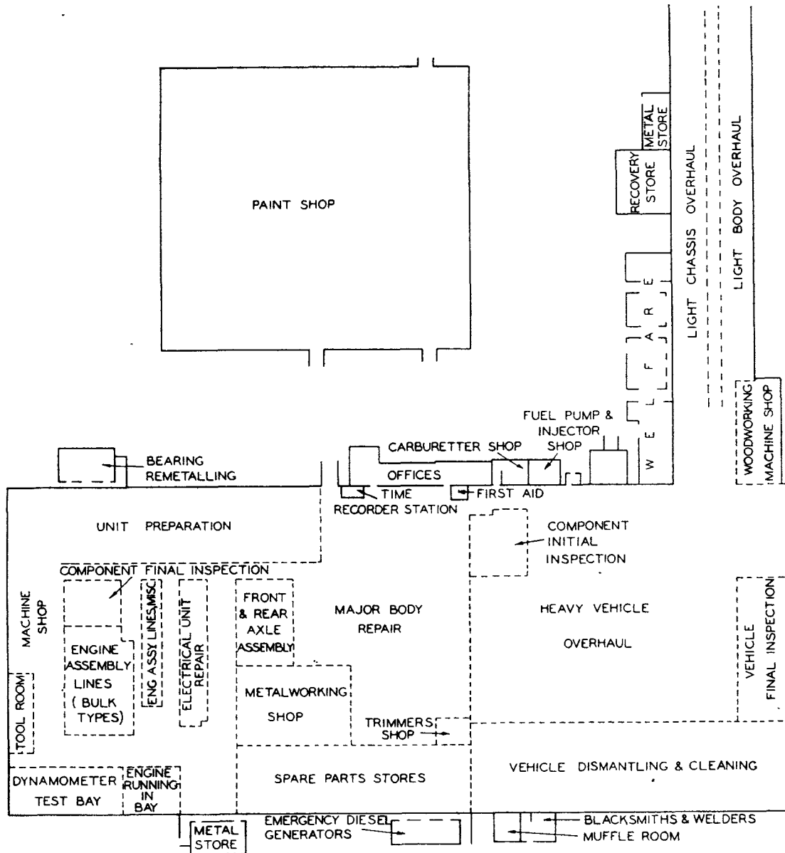
FIG. 1.—LAYOUT OF YEADING REPAIR DEPOT.
