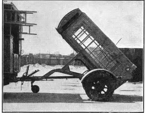
LOADED KIOSK TRAILER IN TOWING POSITION.
