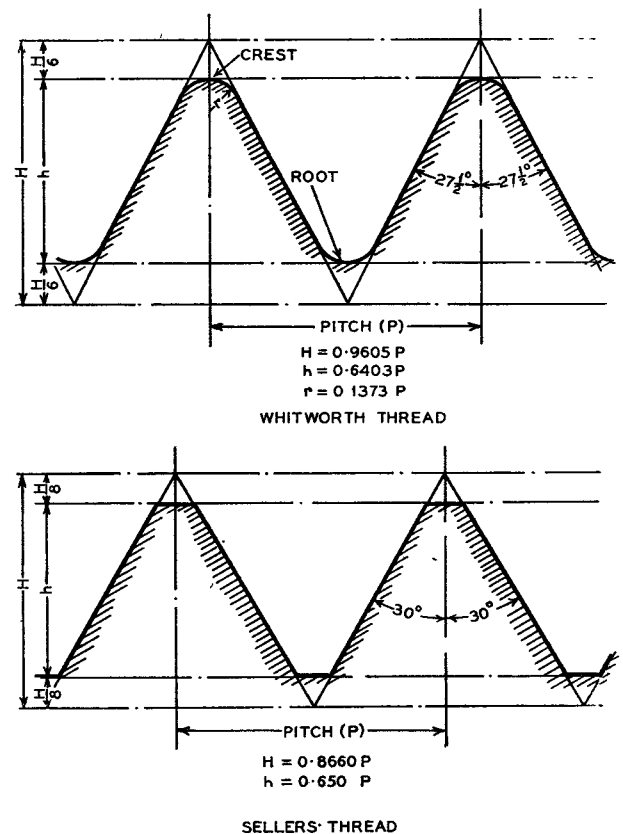
FIG. 1.—COMPARATIVE SHAPES OF WHITWORTH AND SELLERS THREADS.
