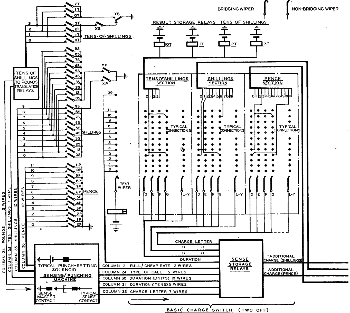
FIG. 6.—SCHEMATIC CIRCUIT
