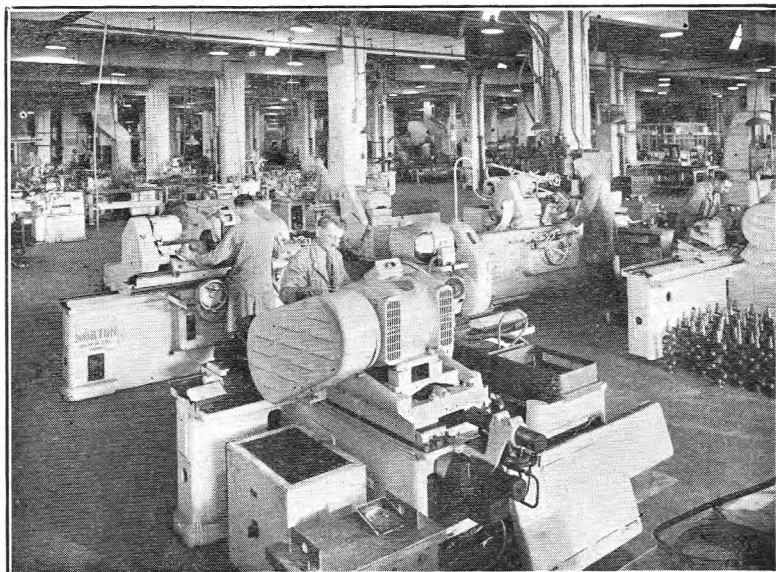
FIG. 3.—CRANKSHAFT GRINDERS.
