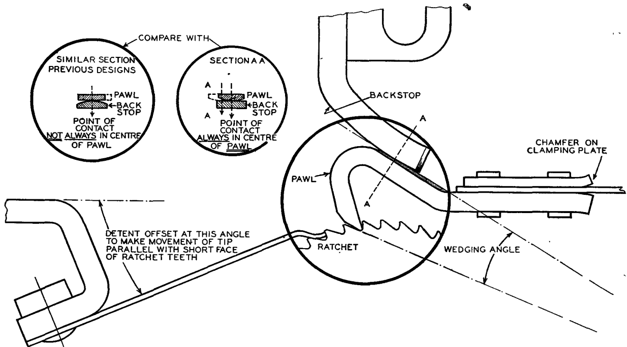
FIG. 5.—MAIN FEATURES OF DRIVING MECHANISM.
