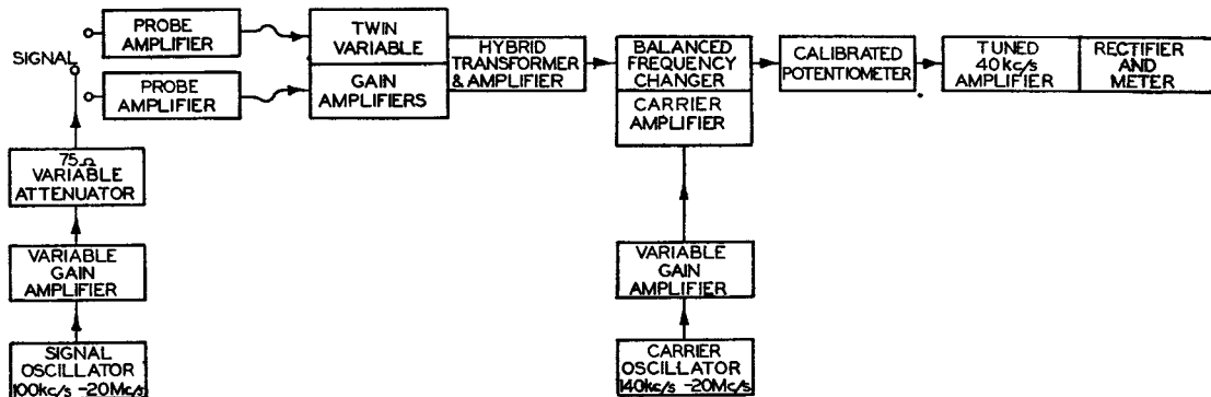
FIG. 1.—BLOCK SCHEMATIC DIAGRAM OF PHASE METER.
