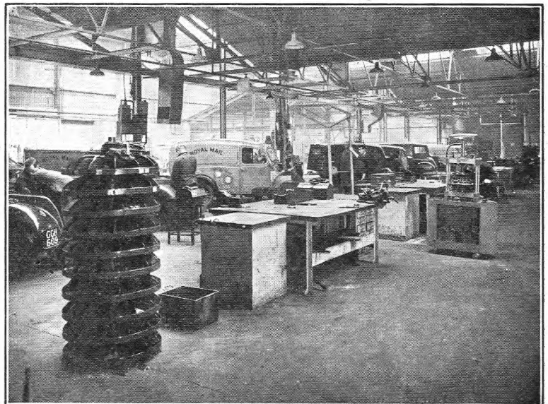
FIG. 8.—LIGHT VAN BODY SHOP.
