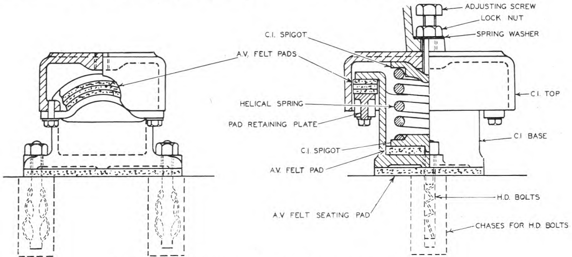
FIG. 4.—CONSTRUCTION OF A TYPICAL PEDESTAL-TYPE ANTI-VIBRATOR.
