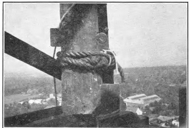
FIG. 3.—LASHING AT BUTT OF DERRICK.
