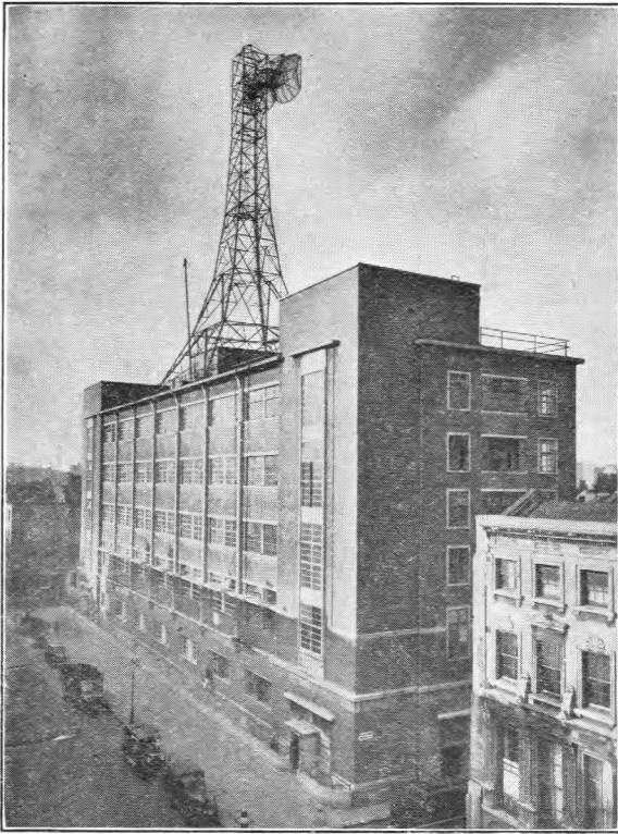
FIG. 7.—THE TOWER AT MUSEUM EXCHANGE, LONDON.
