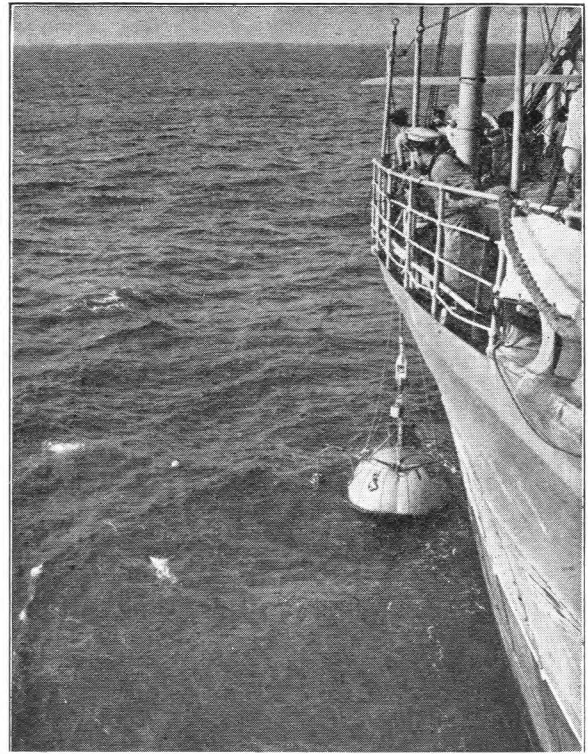
FIG. 3.—VIEW, LOOKING AFT, OF BUOY COMING IN ALONGSIDE SHIP AND SEAMEN HOOKING "TAIL" WITH GRAPNELS.
