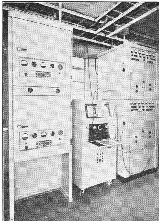
FIG. 11.—RECEIVERS, MONITORS AND TRANSMITTERS AT MUSEUM TERMINAL.
