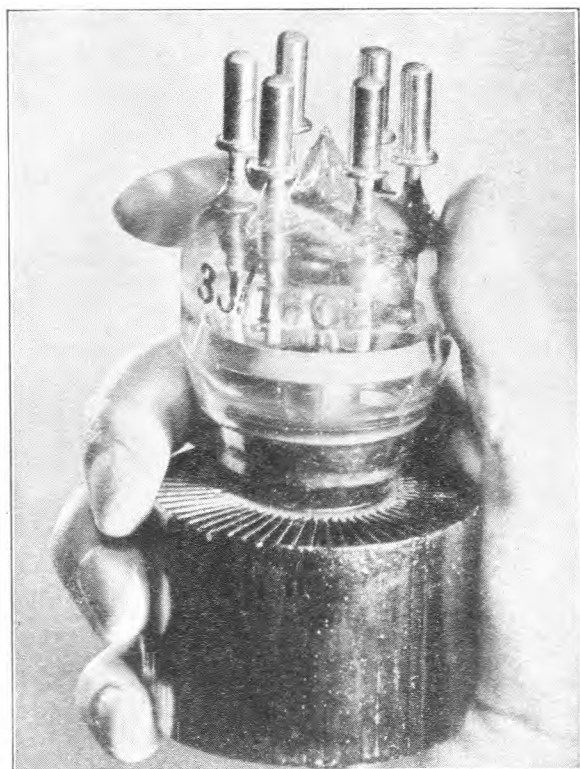
FIG. 7.—FORCED-AIR-COOLED TRIODE, 1 KW ANODE DISSIPATION.
