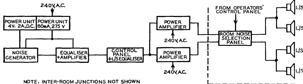
FIG. 2.—ARAEN; BLOCK SCHEMATIC DIAGRAM OF NOISE GENERATION EQUIPMENT.
