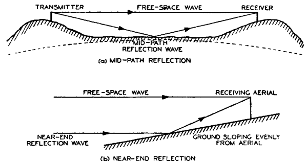
FIG. 2.—PROPAGATION OF FREE-SPACE AND REFLECTED WAVES.
