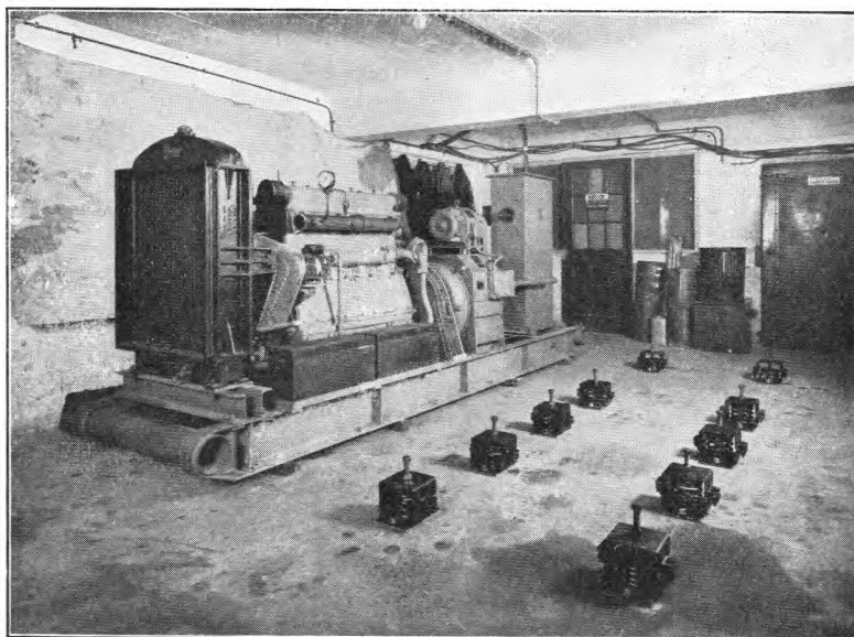
FIG. 7.—DAVEY PAXMAN 65-KVA SET WITH ANTI-VIBRATORS AT CLERKENWELL EXCHANGE.
