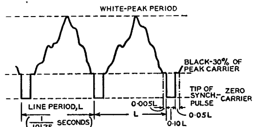
FIG. 1.—405-LINE SIGNALS, U.K. TELEVISION STANDARD TYPICAL LINE SIGNALS DURING FRAMES.
