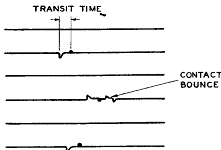
FIG. 5.—C.R.T. DISPLAY SHOWING TRANSIT TIME.
