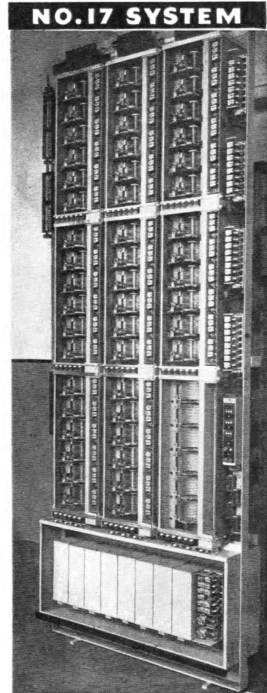
Rack of First Selectors with Covers removed (1950)
