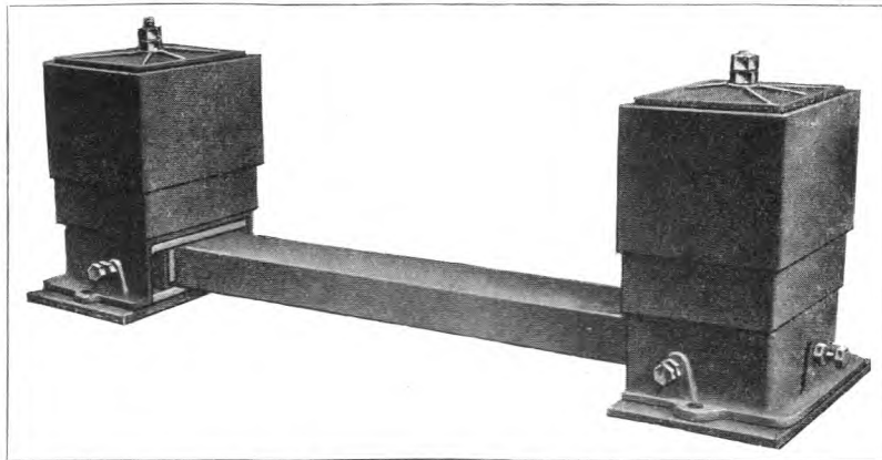
FIG. 6.—BRIDGE-TYPE ANTI-VIBRATOR.
