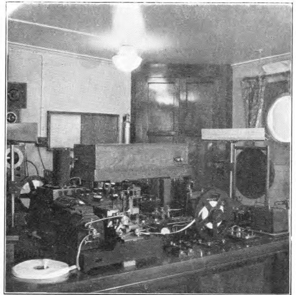
FIG. 2.—THE MAIN TEST TABLE, SHOWING SYPHON RECORDER AND D.R. TEST SET.
