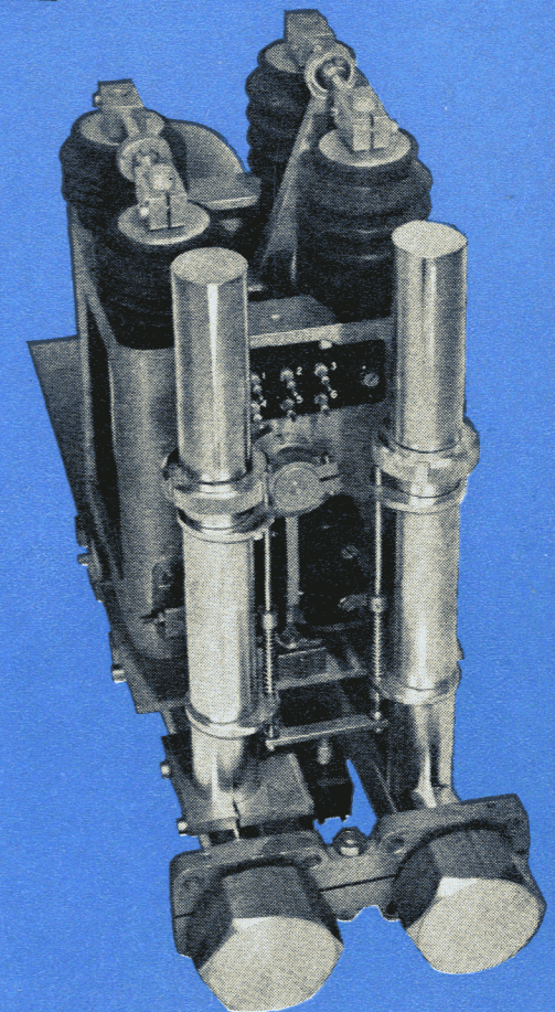
A radio-frequency contactless aerial switch.
