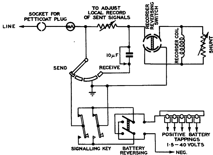
FIG. 6.—CIRCUIT DIAGRAM OF THE LONG-DISTANCE RECORDER.
