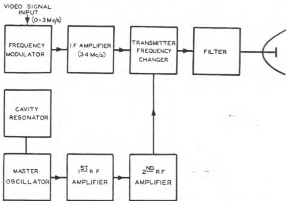
FIG. 8.—BLOCK SCHEMATIC OF TERMINAL TRANSMITTER.
