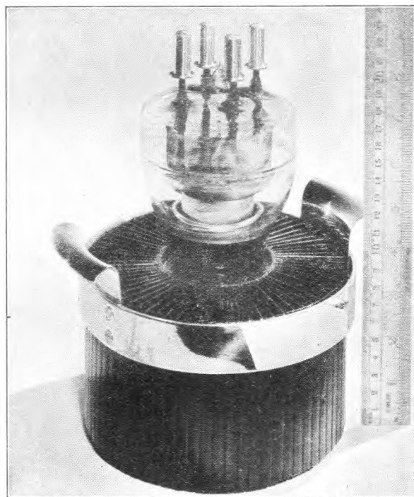
FIG. 6.—FORCED-AIR-COOLED TRIODE, 4.5 kW ANODE DISSIPATION.
