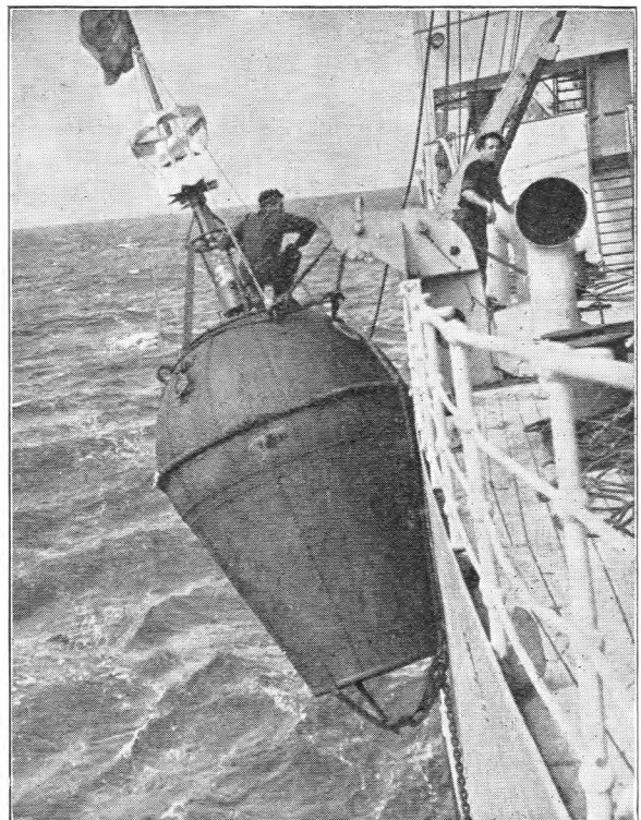
FIG. 5.—BUOY HOISTED TO DECK LEVEL ON SPECIAL SHEAVE.
