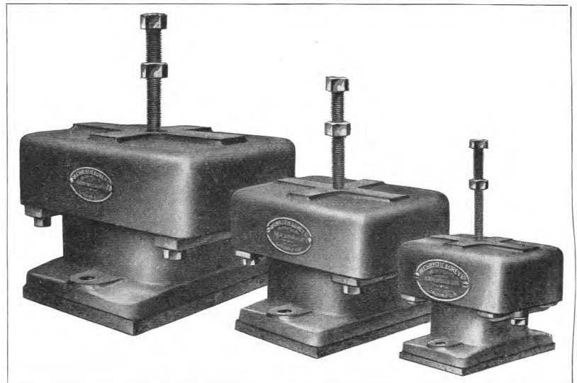
FIG. 5.—PEDESTAL-TYPE ANTI-VIBRATORS.
