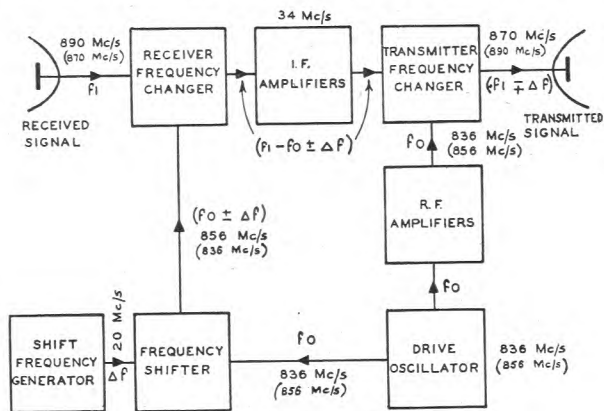
FIG. 12.—ARRANGEMENT OF FREQUENCIES AT A REPEATER STATION (FREQUENCIES IN SMALLER PRINT, IN BRACKETS, ARE ALTERNATIVES).
