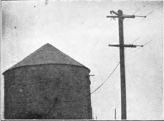
DIPOLE WITH REFLECTOR AT CALDY.
