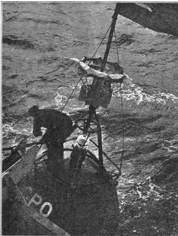
FIG. 4.—SEAMAN SHACKLING 6 \times 3 ROPE FROM BOW SHEAVE BEFORE MOORINGS ARE SLIPPED FROM BUOY AT SIDE SHEAVE.
