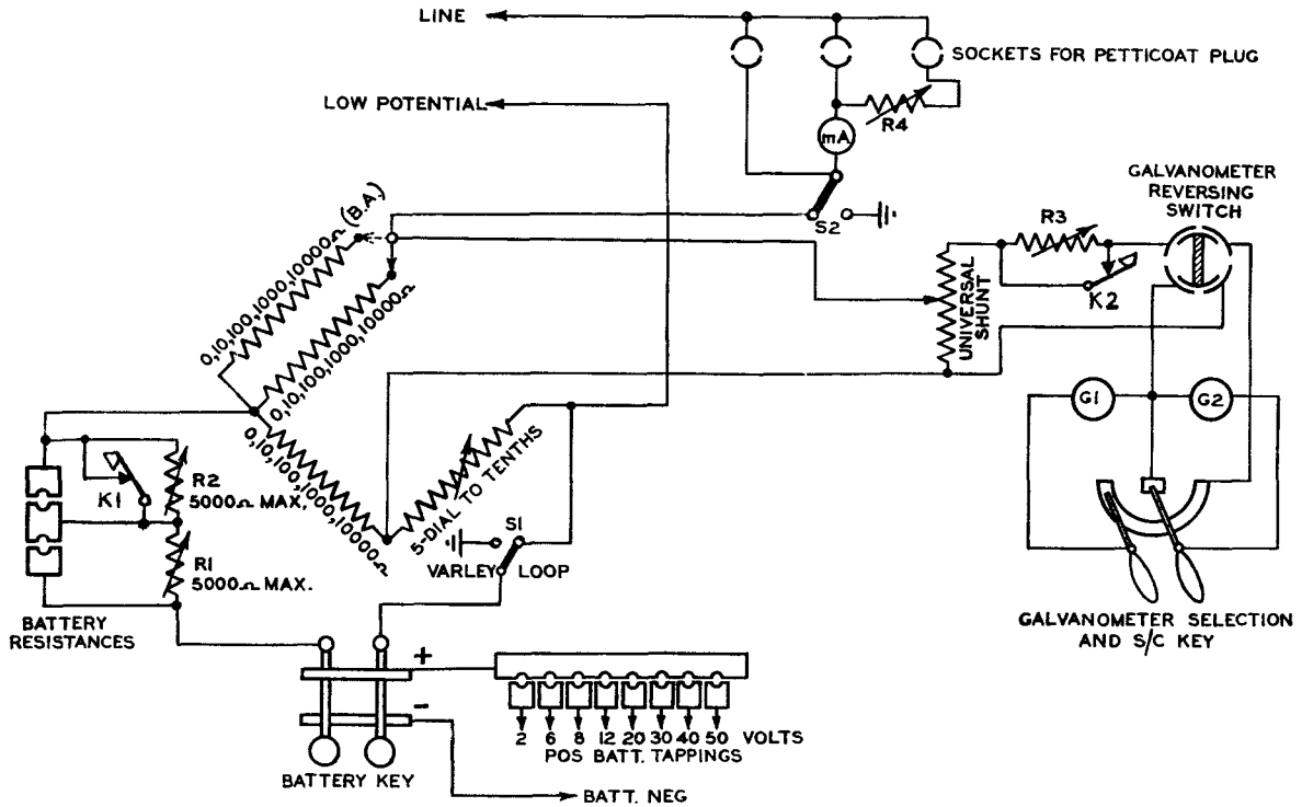
FIG. 3.—CIRCUIT DIAGRAM OF THE CONDUCTOR RESISTANCE TEST SET.
