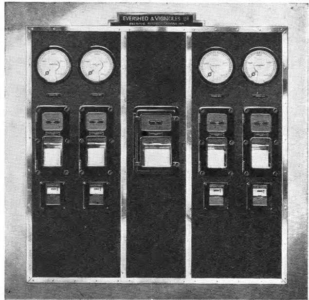
Evershed Recorder Panel for distant indication and recording of electrical loads in a modern film studio.
