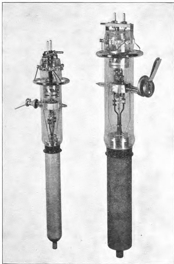
FIG. 5.—18-KW TRIODE (RIGHT) AND 12-KW TRIODE, WITH SIDE-ENTRY GRID SEALS.
