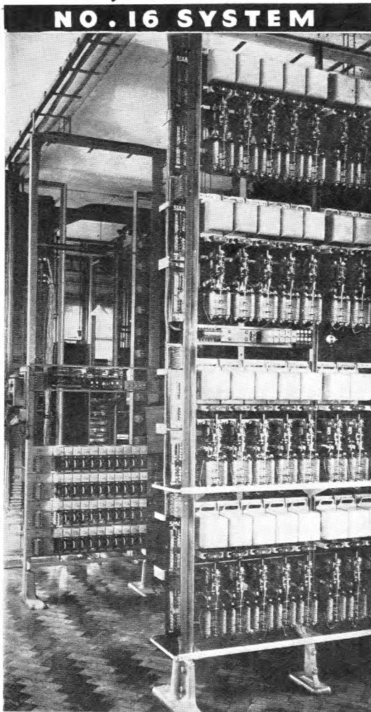
Automatic racks, Preston Exchange, Brighton (1927)
