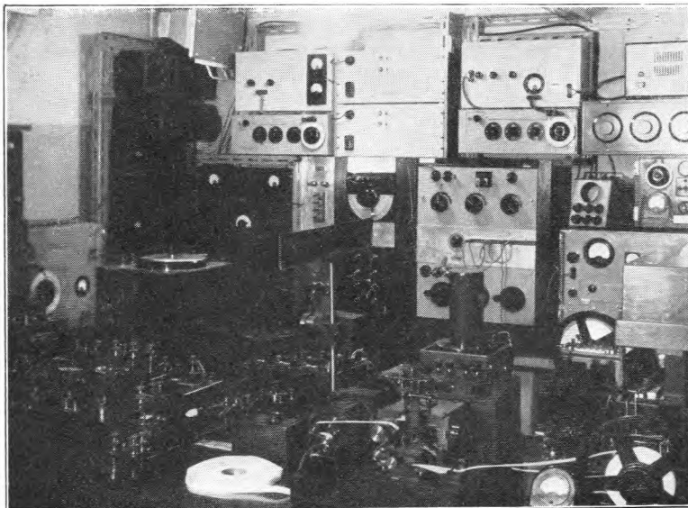
FIG. 1.—GENERAL VIEW OF THE TESTING ROOM.
