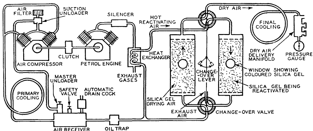
FIG. 1.—SCHEMATIC ARRANGEMENT OF DESICCATOR.
