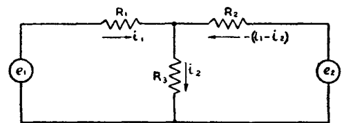
(b) EQUIVALENT CIRCUIT FOR (a)
