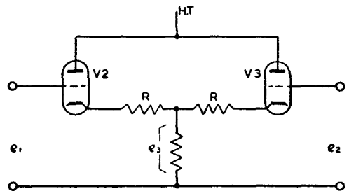
(a) ADDITION CIRCUIT
