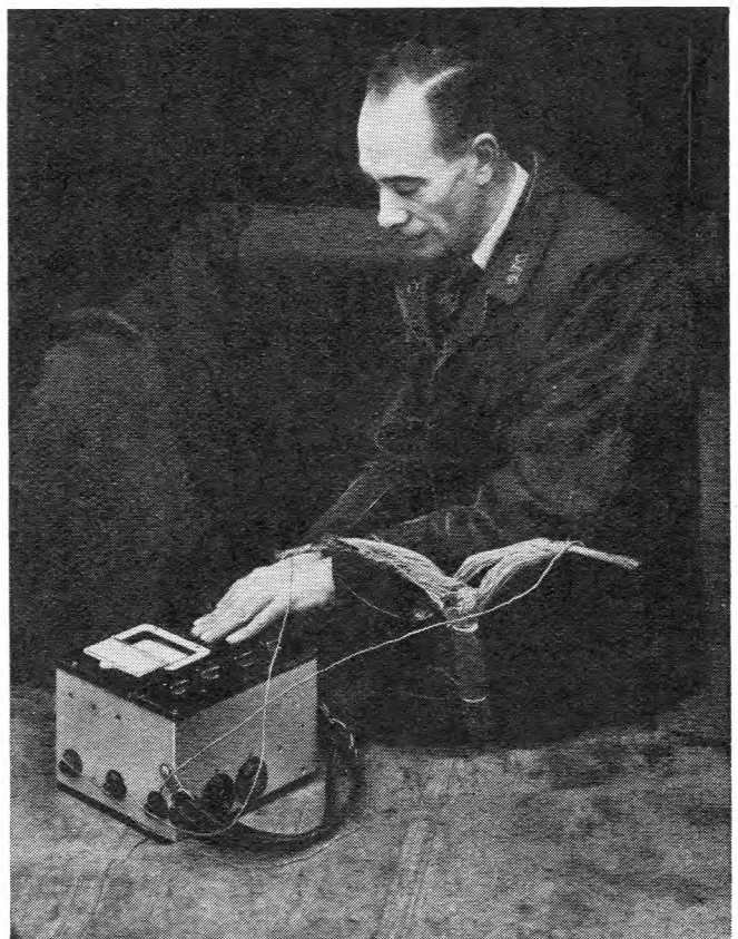
A Bridge-Megger Tester, Series 2, in use by the Post Office Engineering Department. The engineer is shown testing the insulation of 300 pair 6½ lb. P.C.U.T. cable at a pavement box.
