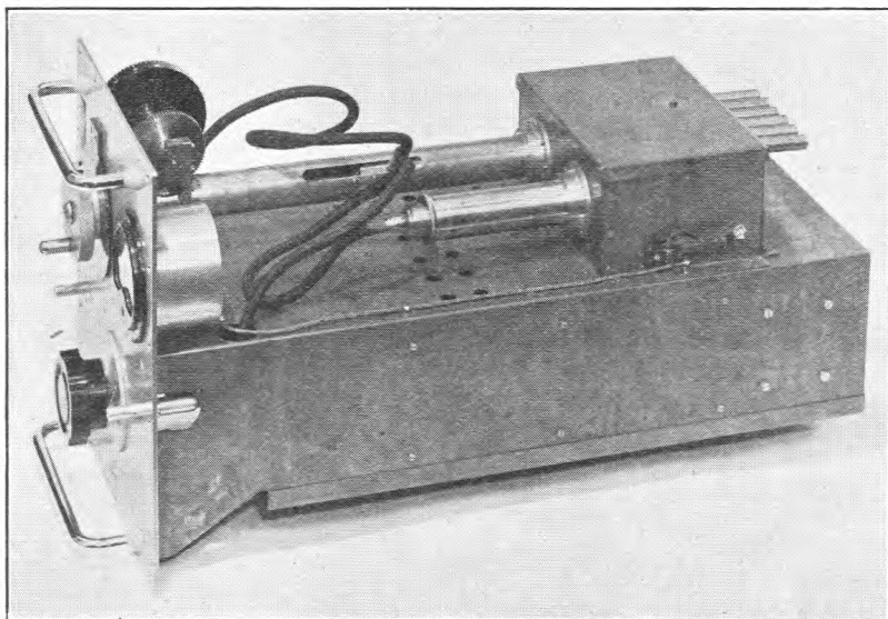
FIG. 5.—THE SIGNAL GENERATOR WITH COVER REMOVED.
