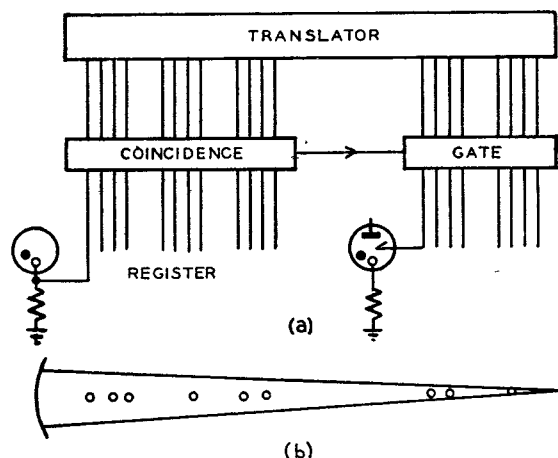
FIG. 7.—THE ELEMENTS OF A STATIC REGISTER-PULSE TRANSLATOR.
