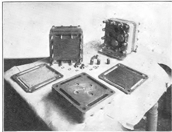
FIG. 5.—THE HEAT-EXCHANGER COMPONENTS AND ASSEMBLY.
