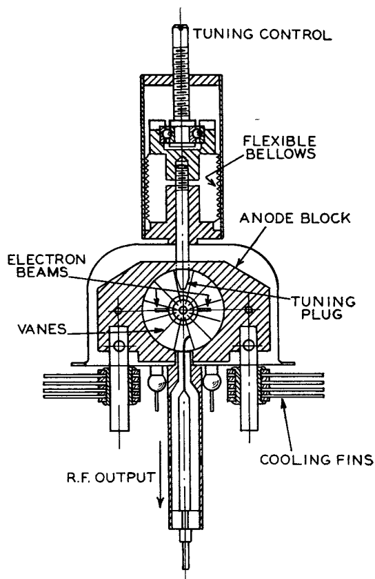
FIG. 14.—C.W. MAGNETRON, ARRANGED FOR FREQUENCY MODULATION BY ELECTRON BEAMS.
