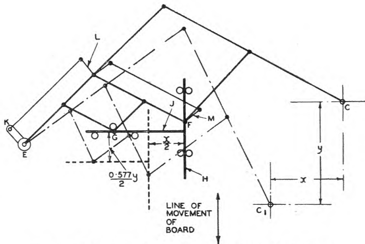
FIG. 4.—SCHEMATIC DRAWING OF PARALLEL PERSPECTOR.
