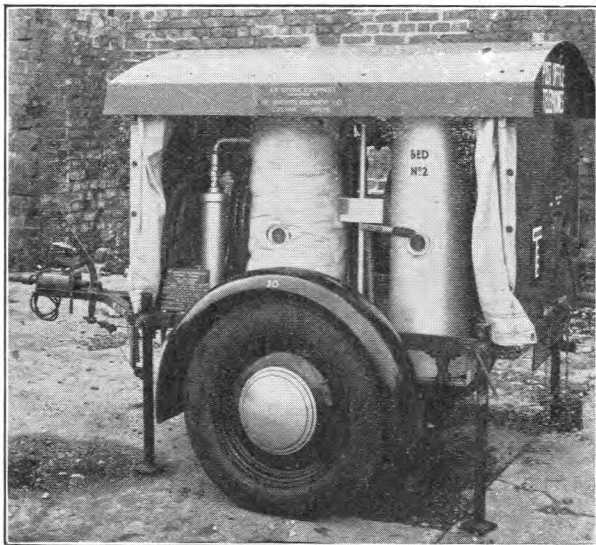
FIG. 3.—SILICA-GEL BEDS SIDE OF THE DESICCATOR.
