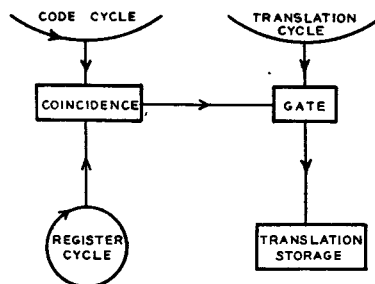
FIG. 8.—THE ELEMENTS OF A PULSE REGISTER-PULSE TRANSLATOR.
