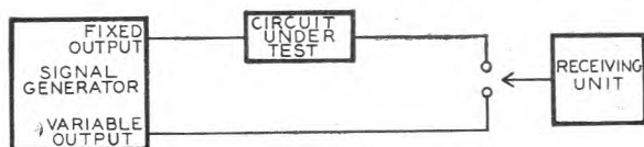
FIG. 2.—ARRANGEMENT FOR MEASURING INSERTION LOSS.
