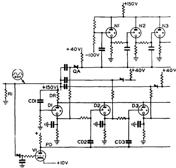
FIG. 1.—A DIALLED IMPULSE REGISTER.
