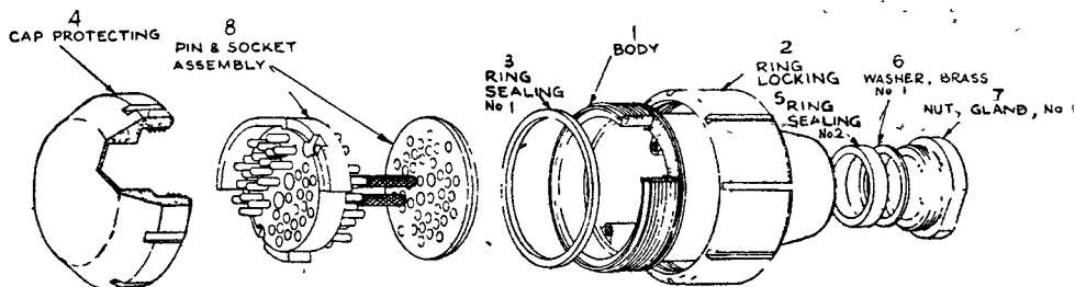
FIG. 6.—EXPLODED VIEW OF A CABLE CONNECTOR PRODUCED ON THE PARALLEL PERSPECTER.
