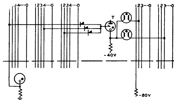
FIG. 6.—THE ELEMENTS OF A STATIC REGISTER-STATIC TRANSLATOR.
