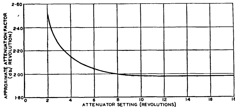
FIG. 7.—VARIATION OF ATTENUATION FACTOR WITH SETTING OF MAIN ATTENUATOR.
