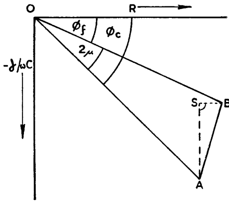
FIG. 2.—VECTORIAL REPRESENTATION OF OPEN AND CLOSED IMPEDANCES.
