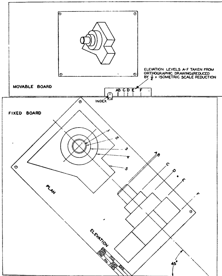
FIG. 5.—SIMPLE EXAMPLE OF THE METHOD OF CONSTRUCTION.
