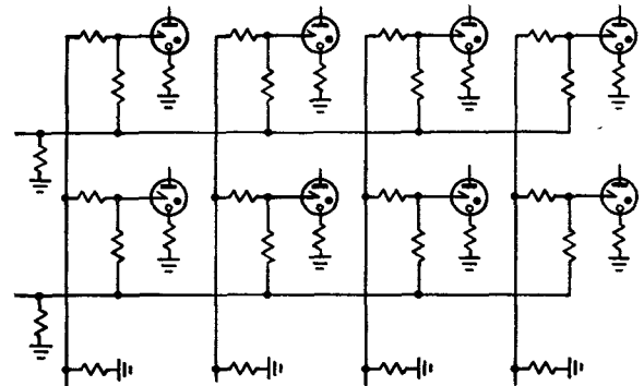
FIG. 2.—A CODED IMPULSE REGISTER.
