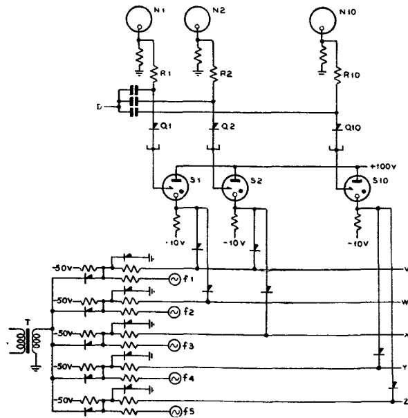
FIG. 9.—THE ELEMENTS OF A SENDER.
