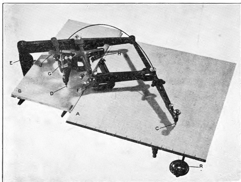
FIG. 3.—GENERAL VIEW OF THE PARALLEL PERSPECTOR.
