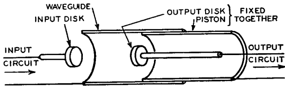
FIG. 1.—BASIC FEATURES OF AN E_{0,1} PISTON ATTENUATOR.
