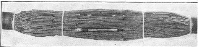
FIG. 4.—EXPERIMENTAL JOINT WITH COAXIAL PAIRS BROUGHT TO THE OUTSIDE.
