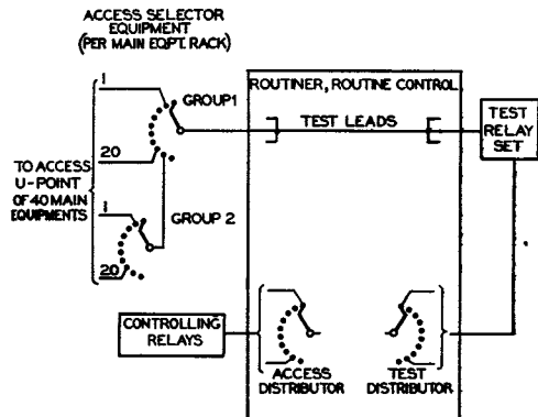
FIG. 1.—SIMPLIFIED BLOCK SCHEMATIC DIAGRAM OF NEW-TYPE ROUTER.
