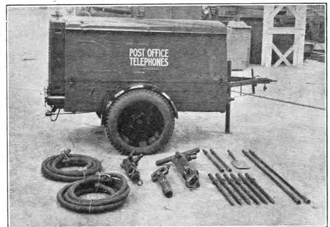
FIG. 6.—SINGLE-TOOL TRAILER AIR-COMPRESSOR AND TOOL EQUIPMENT.
