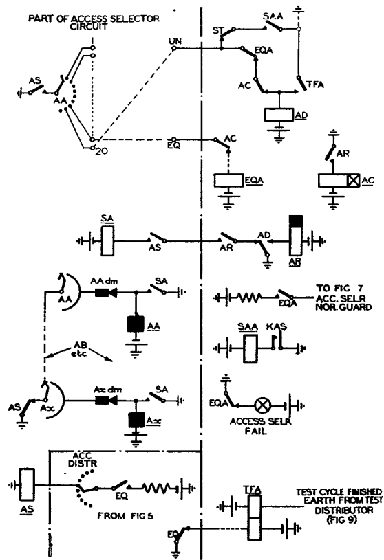
FIG. 6.—ACCESS SELECTOR STEPPING.
