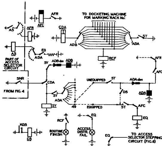
FIG. 5.—ACCESS DISTRIBUTOR STEPPING.
