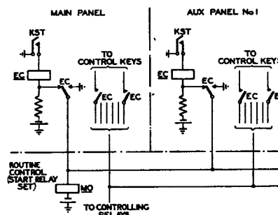
FIG. 10.—MAIN AND AUXILIARY CONTROL PANELS.
