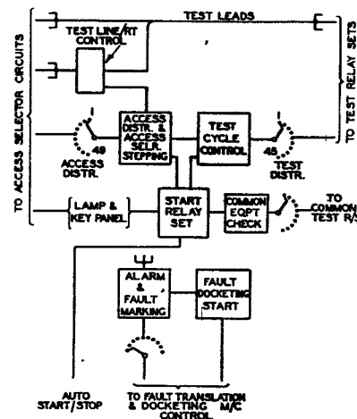
FIG. 2.—BLOCK SCHEMATIC DIAGRAM OF ROUTINE CONTROL.
