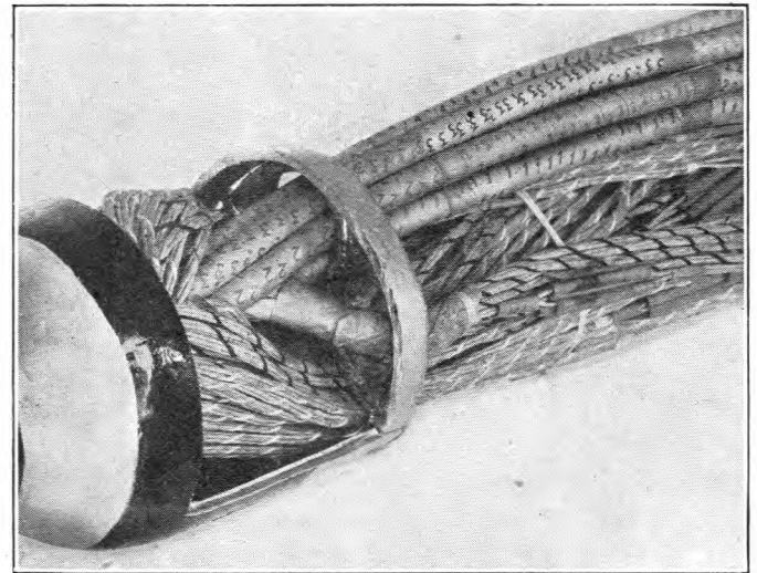
(b) SECTIONAL VIEW OF LEAD PLUG.
