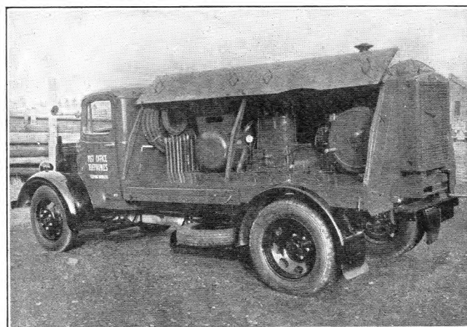
FIG. 2.—SELF-MOBILE AIR-COMPRESSOR WITH SIDE CANOPY OPEN.
