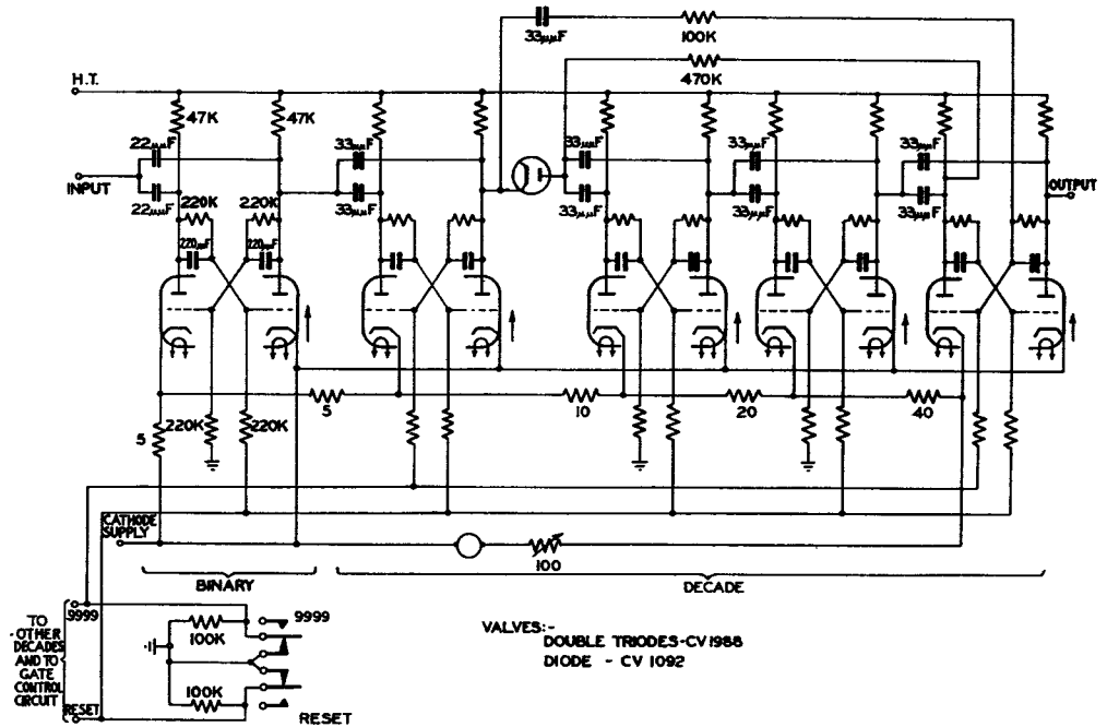
FIG. 5.—THE COUNTER CIRCUIT.
