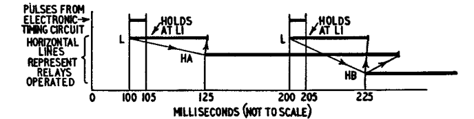
FIG. 6.—METHOD OF LIGHTING 1 V.F. “HUNDREDS OF MILLISECONDS” LAMPS.
