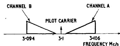
FIG. 2.—INDEPENDENT-SIDEBAND SIGNAL PRODUCED BY DRIVE EQUIPMENT.
