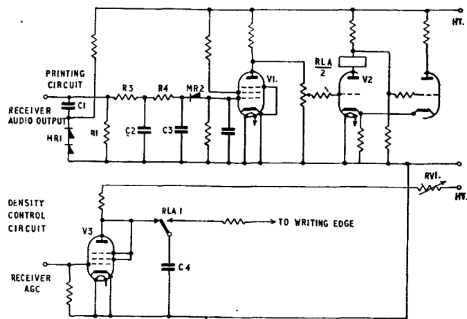
FIG. 5.—CIRCUIT DIAGRAM OF RECORDER.
