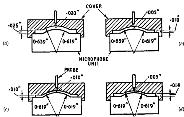
FIG. 3.—CAVITY SHAPES (NOT TO SCALE).
