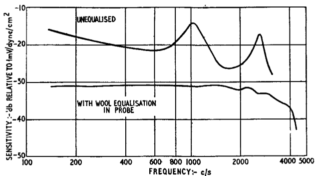
FIG. 4.—SENSITIVITY OF LABORATORY PROBE MICROPHONE WITH INPUT TRANSFORMER.
