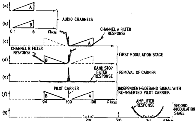
FIG. 4.—GENERATION OF INDEPENDENT-SIDEBAND SIGNAL.
