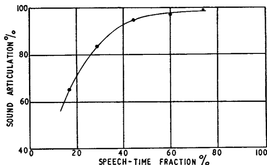
FIG. 3.—SOUND ARTICULATION AS A FUNCTION OF SPEECH-TIME FRACTION.
