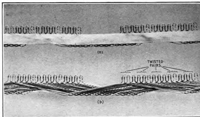
FIG. 6.—RIBBON CABLE USED FOR BANK MULTIPLE.
