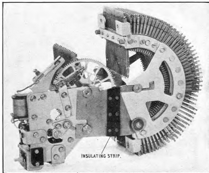
FIG. 5.—MECHANISM FITTED IN OUTRIGGER.
