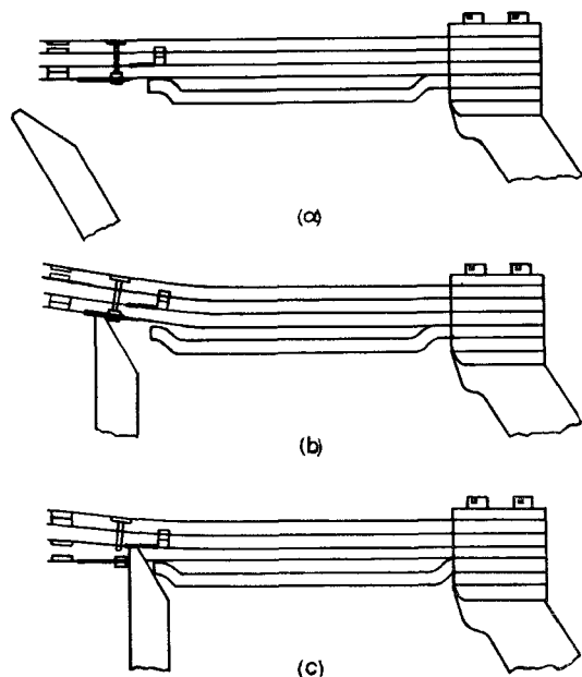
FIG. 9.—STAGES IN OPERATION OF CAM SPRINGSET.
