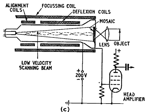
FIG. 5.—CAMERA TUBES. (a) ICONOSCOPE TUBE, (b) IMAGE ICONOSCOPE TUBE, (c) ORTHICON.
