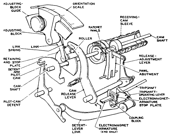
FIG. 4.—ORIENTATION MECHANISM.
