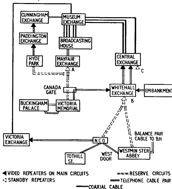
FIG. 11.—TELEVISION CIRCUITS.
