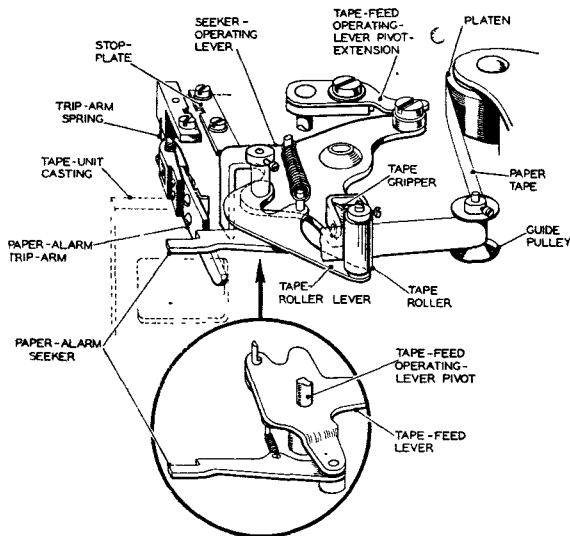
FIG. 8.—PAPER-FAILURE ALARM MECHANISM.
