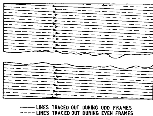
F.G. 3.—INTERLACED SCANNING.
