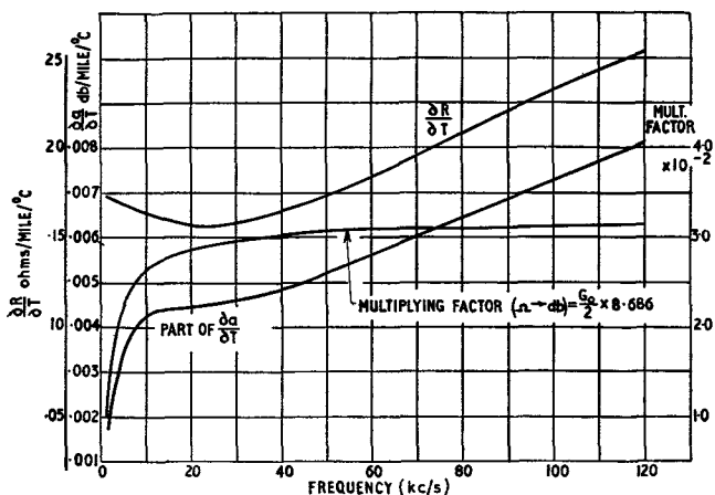
FIG. 10.—COMPOSITION OF COMPONENT OF \frac{\partial a}{\partial T} DUE TO VARIATION OF RESISTANCE WITH TEMPERATURE SHOWN IN FIG. 9.
