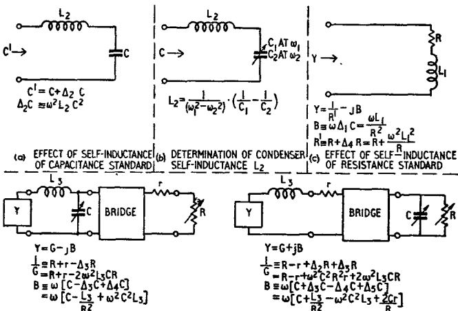
FIG. 1.—CORRECTIONS FOR RESIDUALS IN STANDARDS AND IN BRIDGE.
