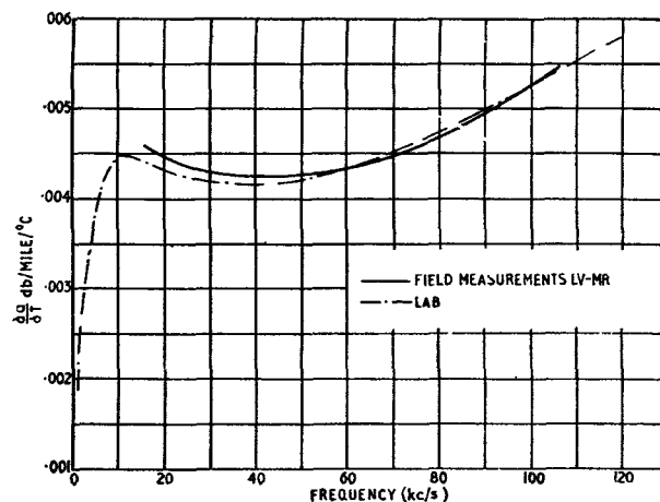
FIG. 12.—COMPARISON OF RESULTS OF FIELD AND LABORATORY MEASUREMENTS OF VARIATION OF ATTENUATION WITH TEMPERATURE, FOR SIDE CIRCUITS.
