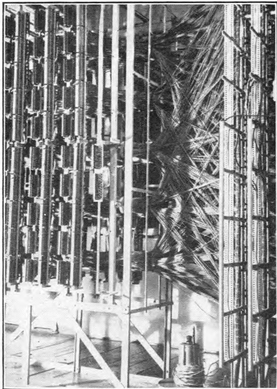
FRAMEWORK CONSTRUCTED FOR TRANSFER AT GREENOCK EXCHANGE.
