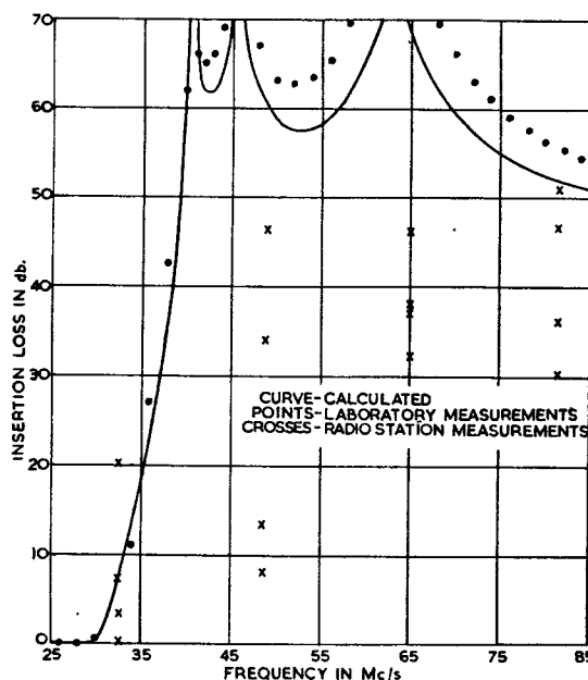
FIG. 2.—INSERTION LOSS/FREQUENCY BEHAVIOUR OF THE FILTER
