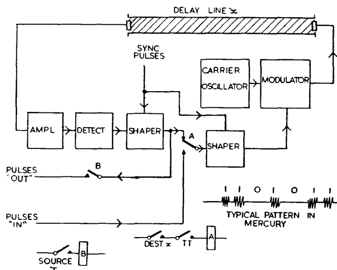
FIG. 1.—BLOCK SCHEMATIC DIAGRAM OF MERCURY DELAY-LINE SWITCHING CIRCUITS.
