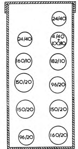
FIG. 13.—SECTION THROUGH TROUGHING SHOWING CHANGED POSITION OF CABLES APPROACHING SLACK BOXES.
