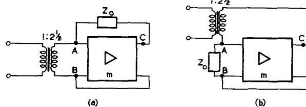
FIG. 7—ADDITION OF COUPLING TRANSFORMERS TO TWO NEGATIVE IMPEDANCES.
