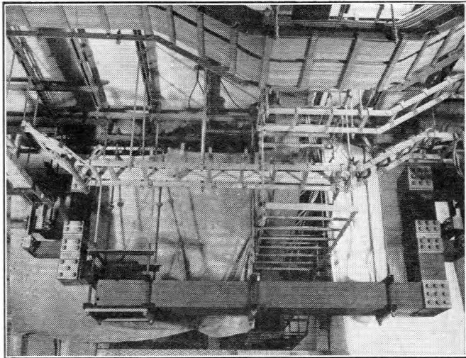
FIG. 9.—POWER DISTRIBUTION BUSBARS AND CABLE RACKING.
