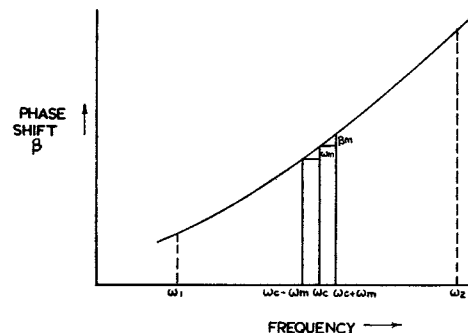
FIG. 1.—MEASUREMENT OF THE SLOPE OF A PHASE/FREQUENCY CHARACTERISTIC.
