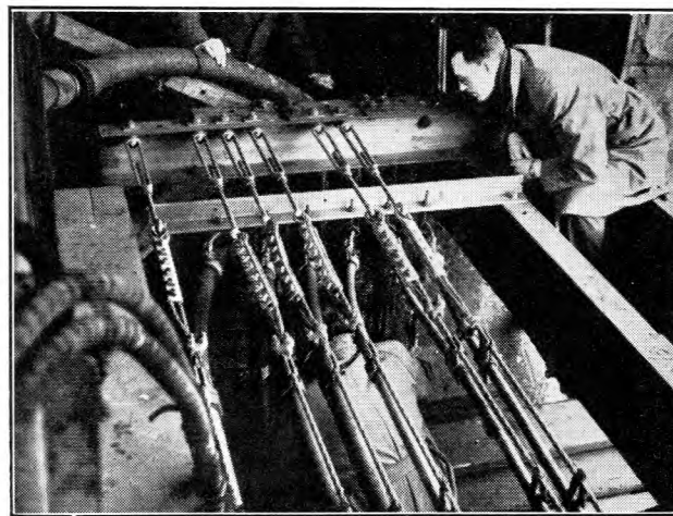
FIG. 5.—TERMINATION OF CABLE SUSPENSION WIRES.
