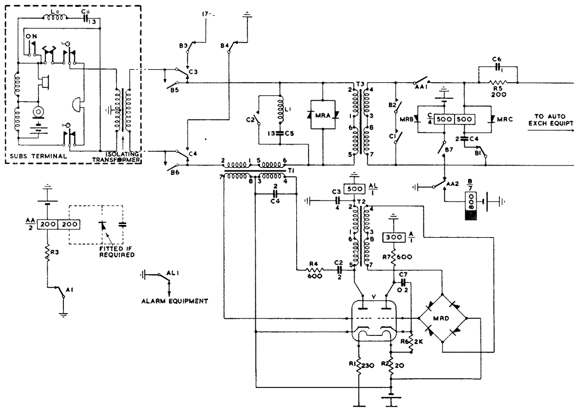
FIG. 1.—SIMPLIFIED CIRCUIT OF IMPEDANCE DIALLING SYSTEM.
