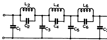
FIG. 1.—THE LOW-PASS FILTER CIRCUIT.
