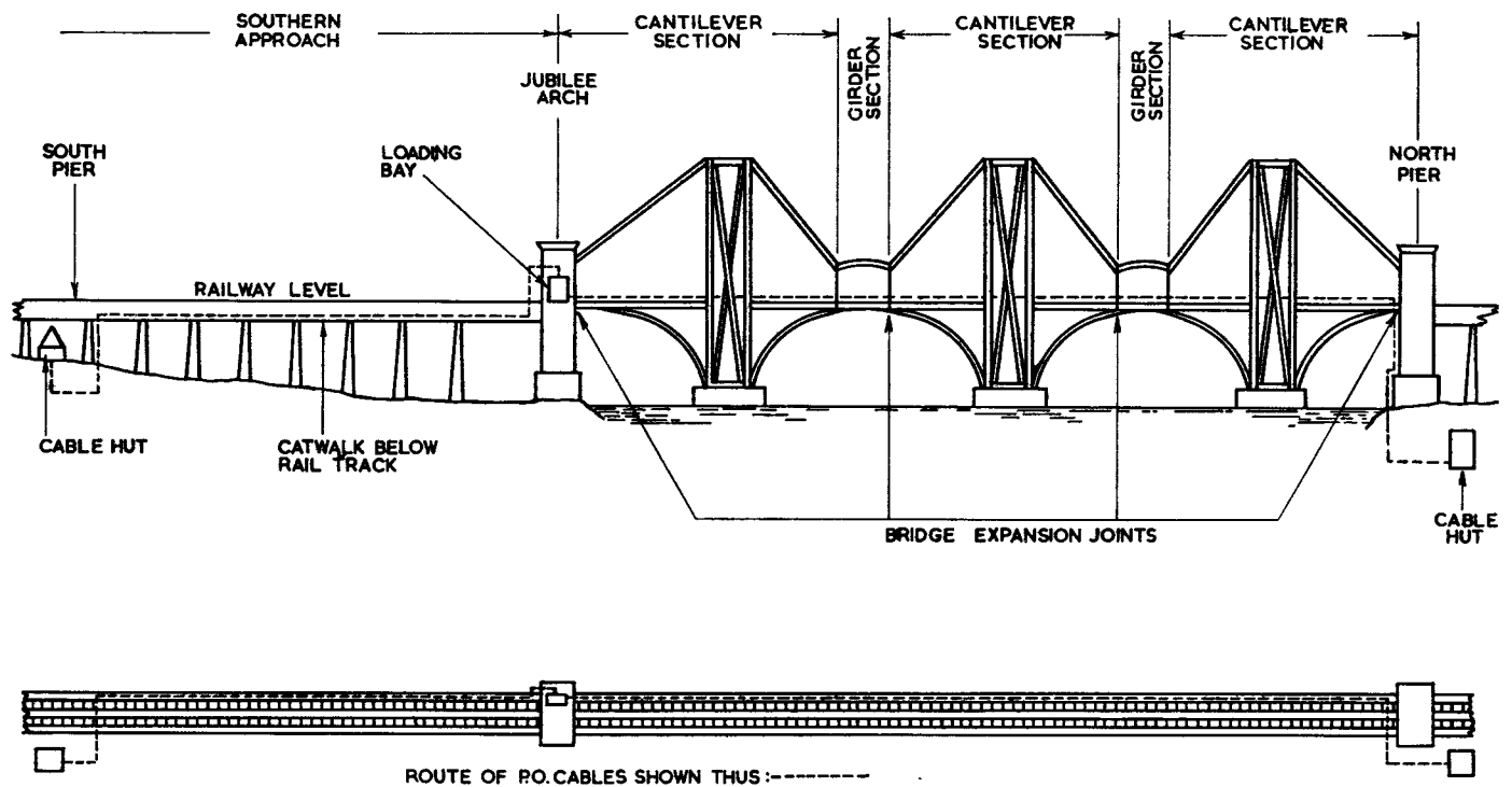
FIG. 2.—DIAGRAM OF BRIDGE SHOWING POSITION OF CABLES.
