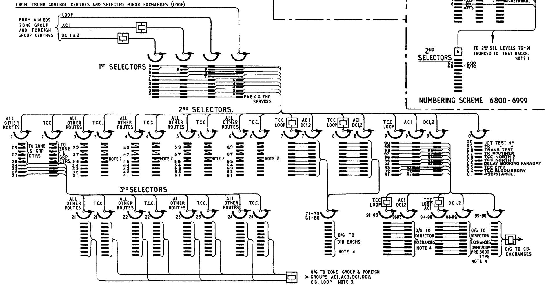
FIG. 1.—TRUNKING PRINCIPLES.
