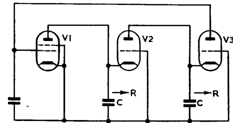
FIG. 1.—SIMPLIFIED CIRCUIT OF MODULATOR.
