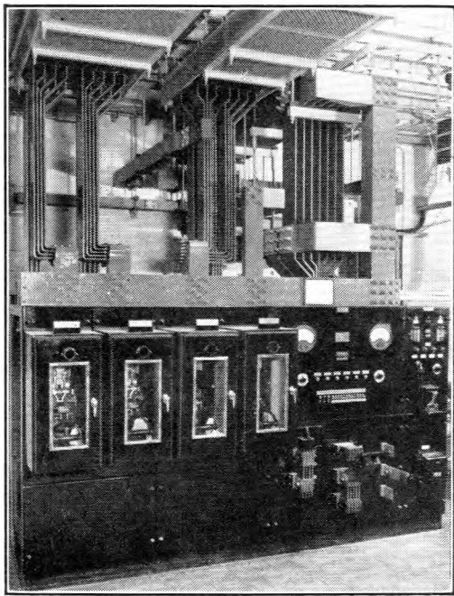
FIG. 8.—POWER-DISTRIBUTION BOARD.
