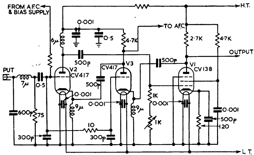
FIG. 2.—TYPICAL MODULATOR CIRCUIT.
