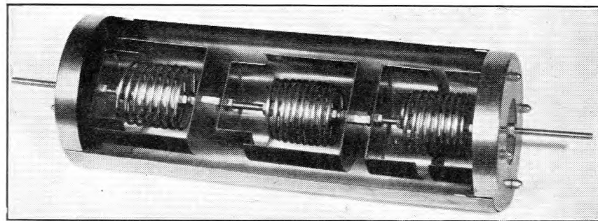
FIG. 3.—SECTIONAL MODEL OF 300-OHM FILTER.
