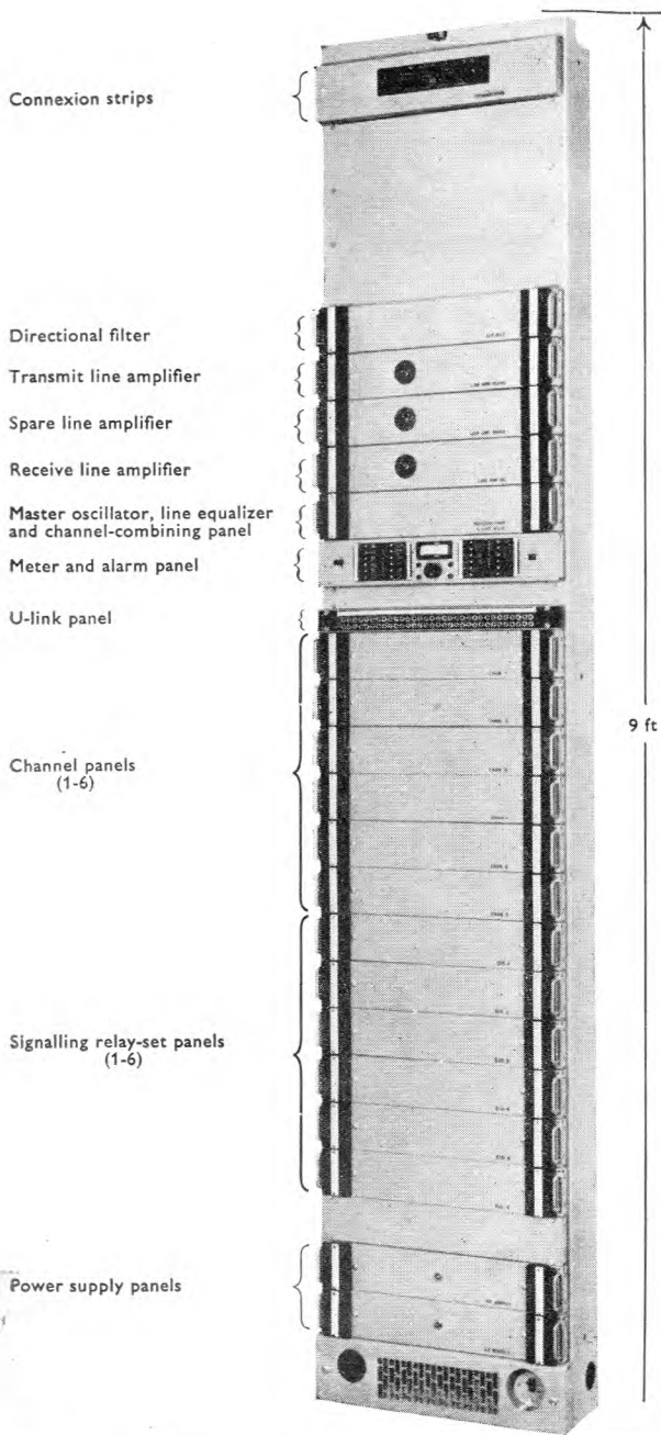
FIG. 9.—“Q” SYSTEM CARRIER TERMINAL EQUIPMENT.
