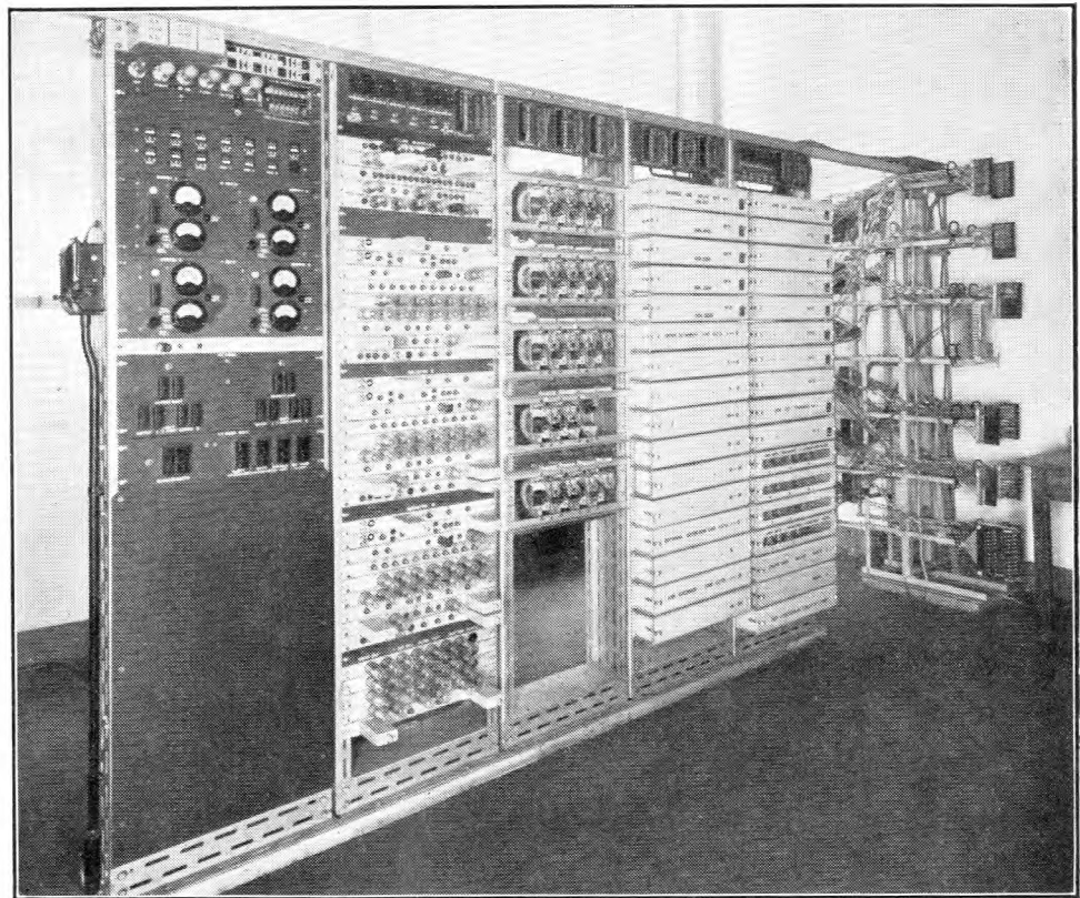
FIG. 10.—GENERAL VIEW OF THE EXPERIMENTAL ELECTRONICALLY-CONTROLLED P.A.B.X.
