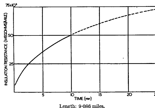
FIG. 19.—INSULATION RESISTANCE OF THE CABLE.
