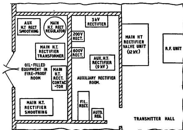
FIG. 2.—TYPICAL LAYOUT OF HIGH-POWER H.F. TRANSMITTER.
