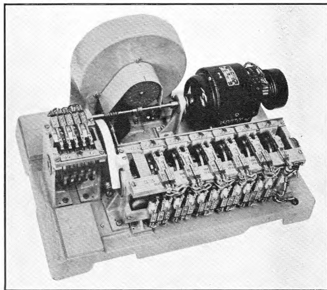
FIG. 6.—TELEGRAPH SIGNAL GENERATOR.
