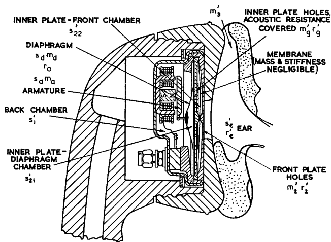
FIG. 6.—SECTIONAL VIEW OF THE 4T RECEIVER INSET (IN THE NEW HANDSET) HELD AGAINST THE EAR, SHOWING MECHANICAL-ACOUSTICAL SYSTEM.
