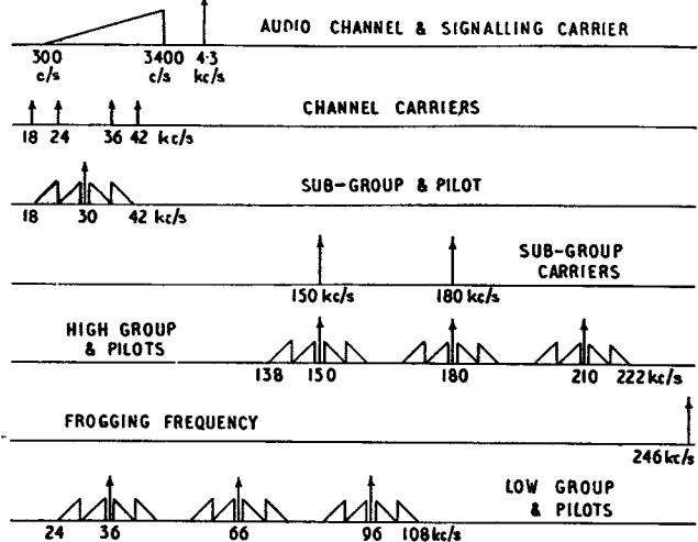
FIG. 6.—FREQUENCY ALLOCATION OF 12-CIRCUIT CARRIER SYSTEM FOR USE ON UNLOADED CABLE.
