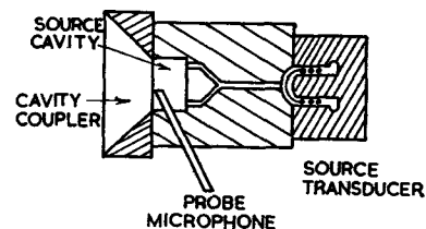
FIG. 5.—SOUND SOURCE AND CAVITY COUPLER.
