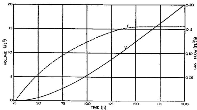
FIG. 13.—RELATIONSHIP BETWEEN RECEIVED VOLUME OF GAS (V), GAS FLOW (F) AND TIME.
