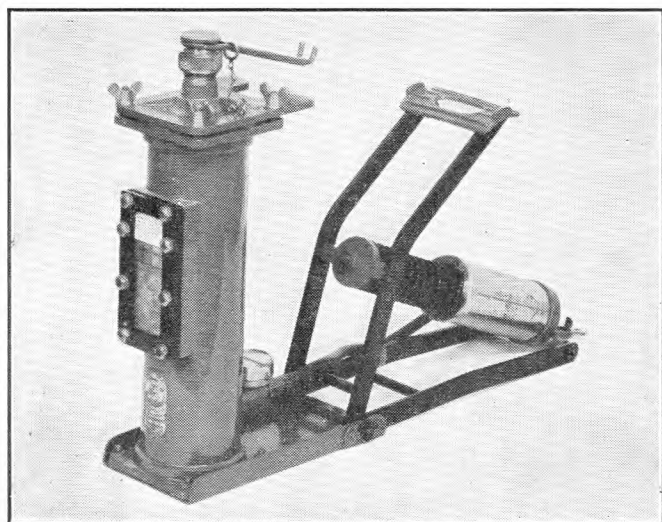
FIG. 1.—THE DESICCATOR, READY FOR USE.
