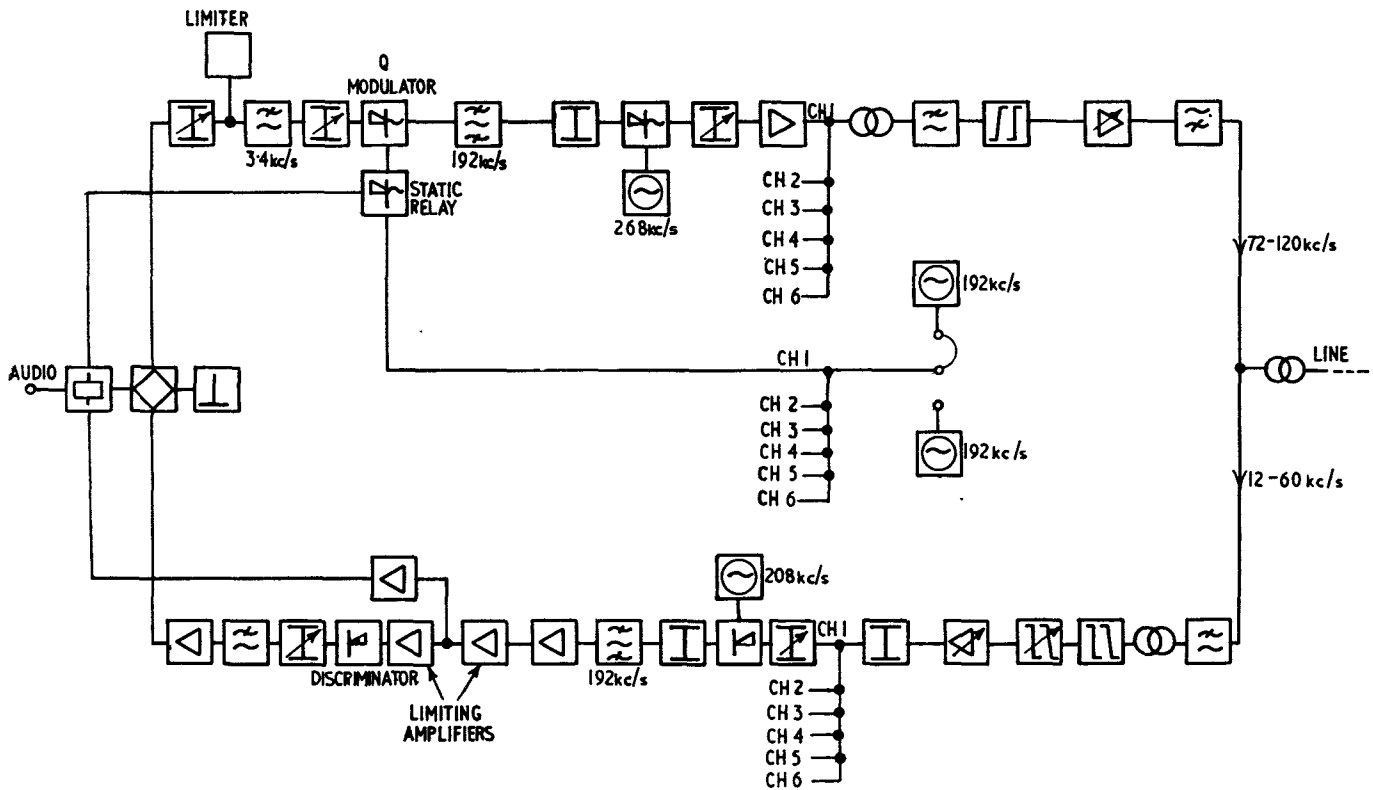
FIG. 8.—A-TYPE TERMINAL OF THE "Q" CARRIER TELEPHONE SYSTEM.
