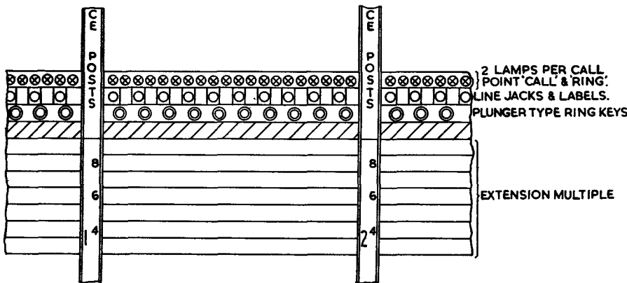
FIG. 2.—ARRANGEMENT OF CALL-POINT CIRCUITS ON THE SWITCHBOARD.
