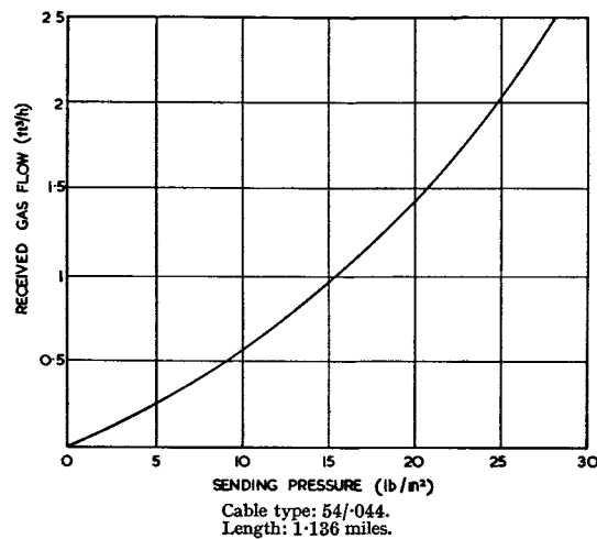
FIG. 14.—RELATIONSHIP BETWEEN SENDING PRESSURE AND RECEIVED GAS FLOW.
