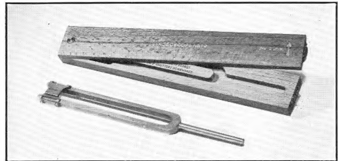
FIG. 1.—TUNING-FORK STROBOSCOPE.
