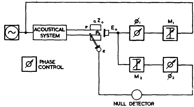
FIG. 4.—COMMON ELECTRICAL CONTROL CIRCUIT (SHOWN WITH ACOUSTICAL EQUIPMENT).
