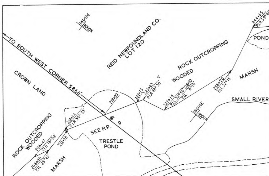
P.I.R.—Point of Interception Right. P.I.L.—Point of Interception Left. 206+47—20,647 ft from commencement of Section of Survey (in this Example from Black River).
