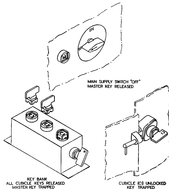
FIG. 1.—TYPICAL ARRANGEMENT OF CODED LOCKS AND KEYS.
