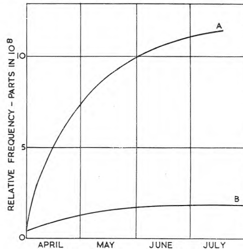
A—Oscillator operating at about 50^\circ\text{C} . B—Resonator operating underground at 11.5^\circ\text{C} . FIG. 4.—FREQUENCY-TIME PERFORMANCE OF QUARTZ-CRYSTAL OSCILLATOR AND RESONATOR.
