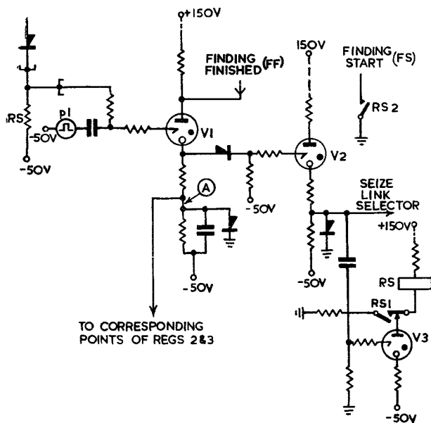
FIG. 3.—REGISTER SEIZE AND BARRING CIRCUIT.
