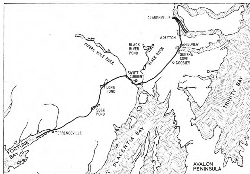
FIG. 1.—ROUTE OF THE CABLE ACROSS NEWFOUNDLAND.
