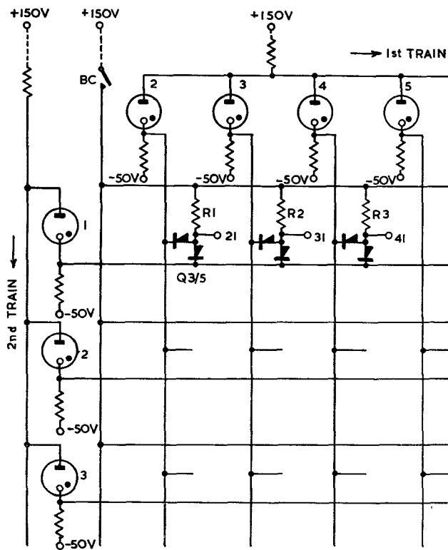
FIG. 6.—REGISTER COINCIDENCE FIELD.
