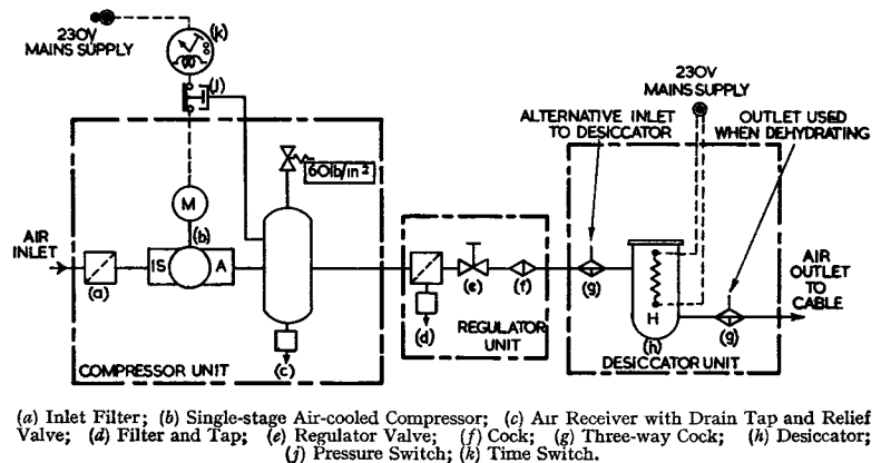
FIG. 15.—BLOCK SCHEMATIC DIAGRAM OF AIR-COMPRESSING AND DRYING PLANT.
