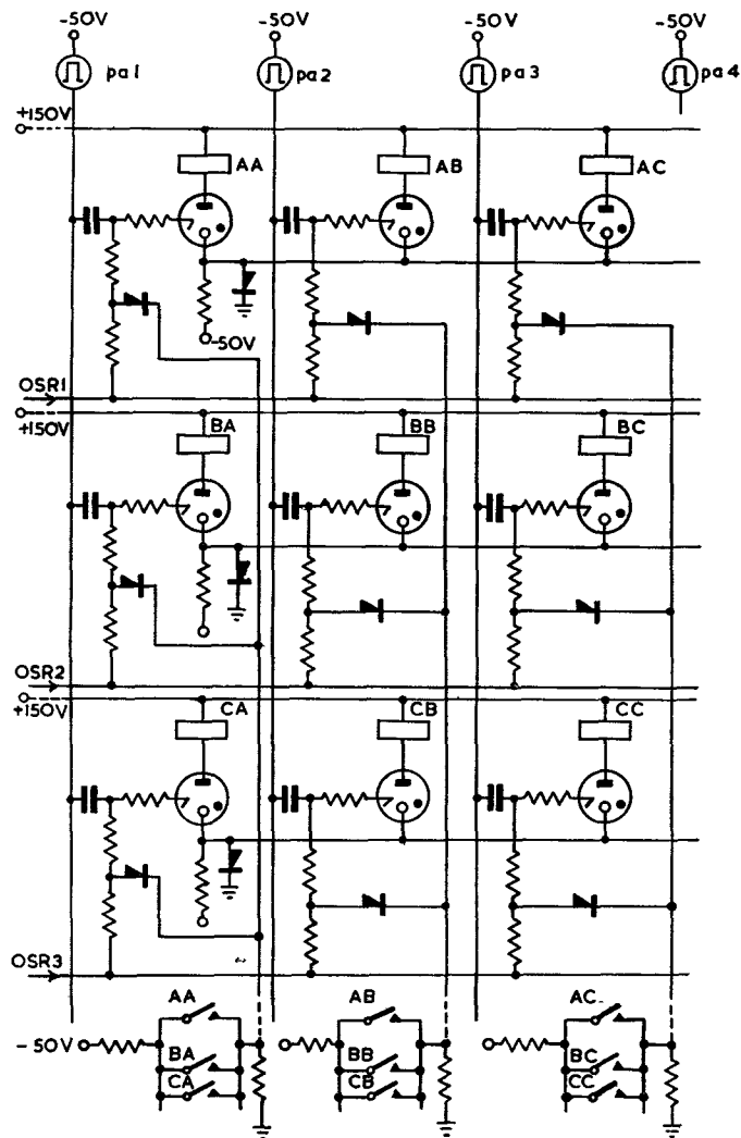
FIG. 7.—PART OF THE LINK SELECTOR.
