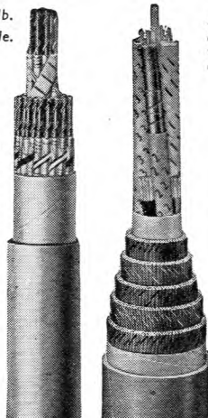
4-tube composite coaxial cable with 18 supervisory pairs and 195 audio-trunk quads.
