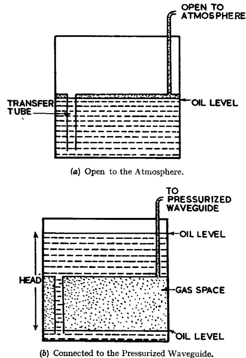
FIG. 1.—PRINCIPLE OF OPERATION OF THE RESERVOIR.
