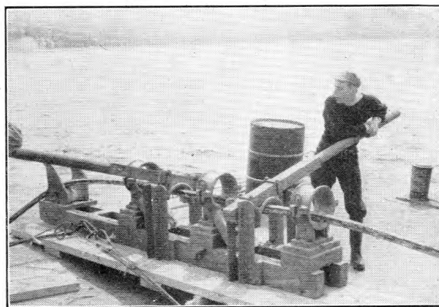
FIG. 16.—THE CABLE-BRAKING DEVICE.
