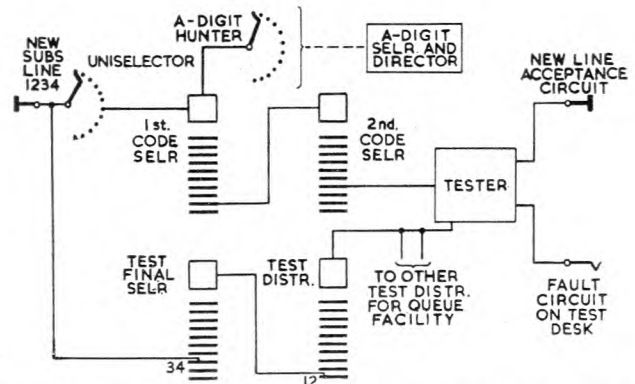
BLOCK SCHEMATIC DIAGRAM SHOWING THE ARRANGEMENT OF THE TESTER AT A DIRECTOR EXCHANGE.
