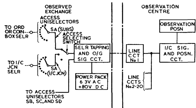
FIG. 1.—BLOCK SCHEMATIC DIAGRAM OF THE SYSTEM.
