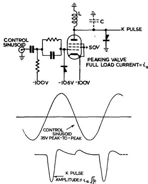
FIG. 16.—K-PULSE PEAKING CIRCUIT.
