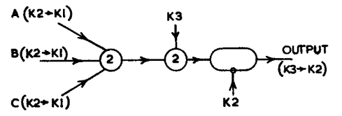
FIG. 24.—LOGICAL "CARRY" CIRCUIT.
