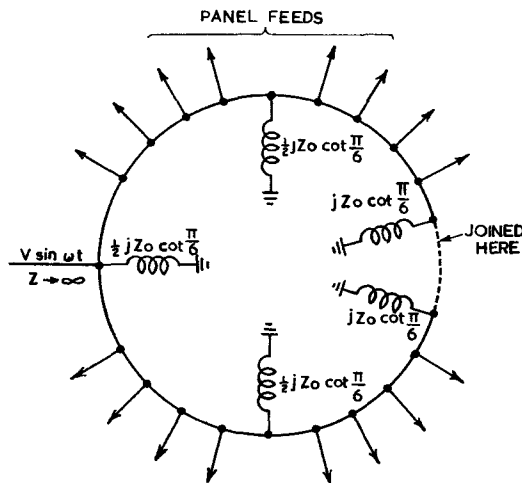
FIG. 20.—MOSAIC'S RING MAIN.
