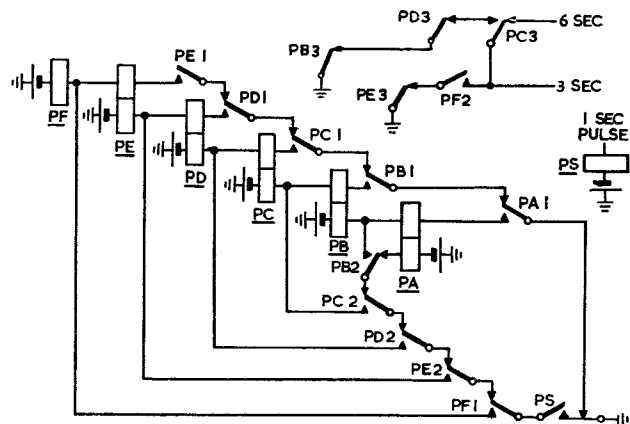
FIG. 4.—GENERATION OF 3-SEC AND 6-SEC PULSES.
