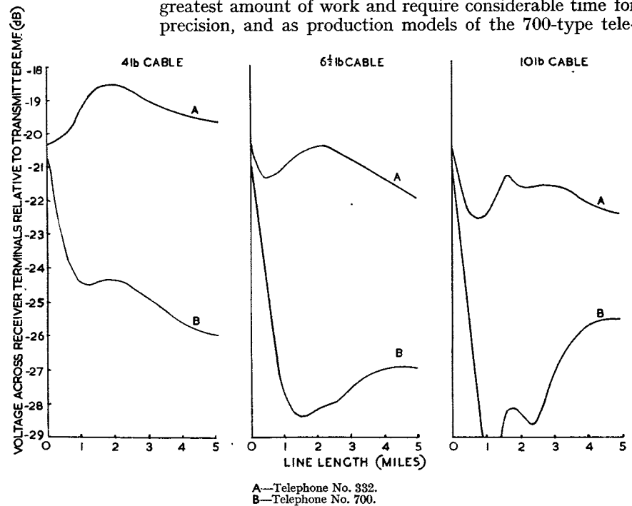
FIG. 13.—SIDE-TONE RESPONSE OF TELEPHONES NO. 332 AND NO. 700.
