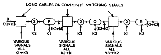
FIG. 14.—LOGICAL K-PULSE SWITCHES.
