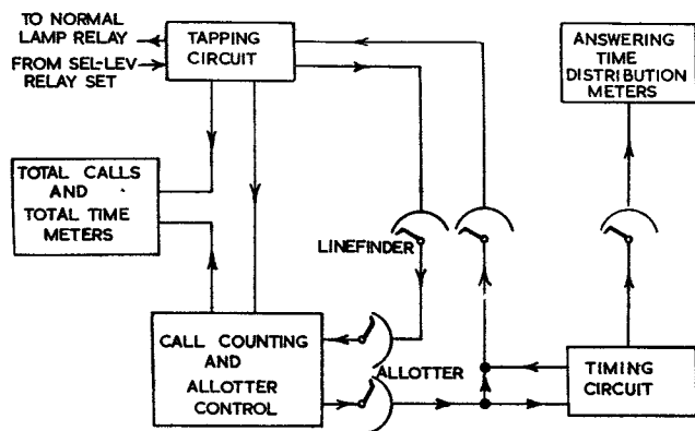
FIG. 1.—BLOCK SCHEMATIC DIAGRAM OF THE EQUIPMENT.
