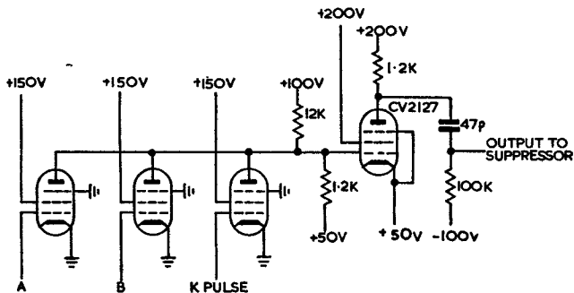
FIG. 23.—TRIGGER-SWITCHING "AND" GATE.
