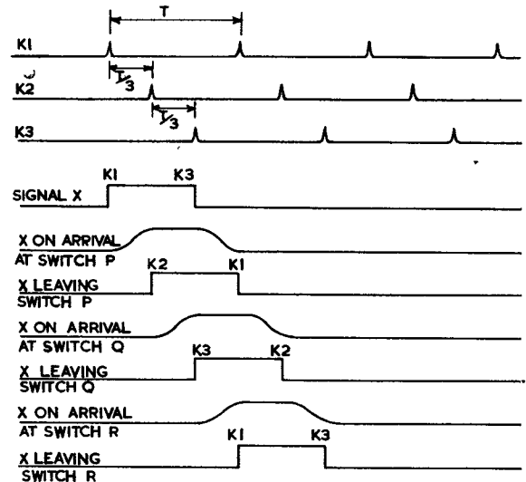
FIG. 13.—PROGRESSIVE TIMING OF SIGNAL PULSE X.
