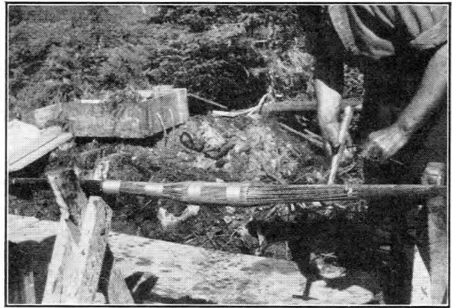
FIG. 20.—COMPLETING A SPLICE.
