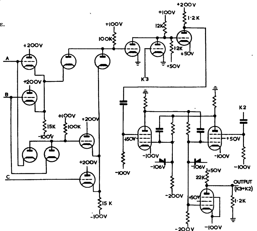
FIG. 26.—PRACTICAL "CARRY" CIRCUIT.
