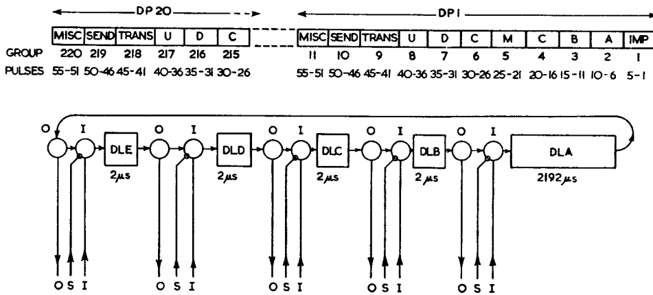
FIG. 3.—A COMPLETE STORAGE SYSTEM.
