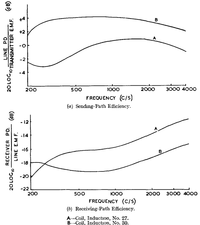
FIG. 10.—SENDING AND RECEIVING CHARACTERISTICS OF COILS, INDUCTION, NO. 27 AND NO. 30.
