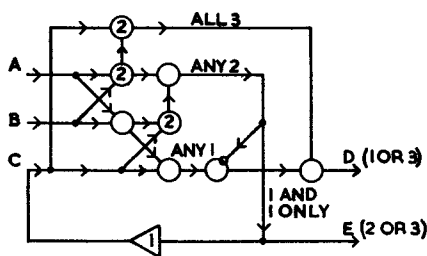
FIG. 27.—LOGICAL "ADDER."
