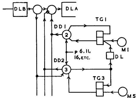
FIG. 5.—INCOMING DIGIT DISTRIBUTION.
