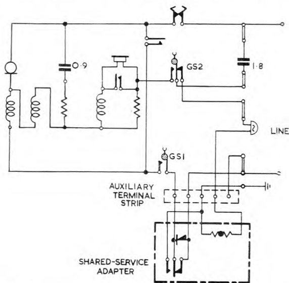
FIG. 18.—TELEPHONE NO. 704, WITH SHARED-SERVICE ADAPTOR.
