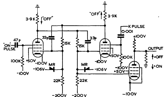
FIG. 21.—BINARY TRIGGER.
