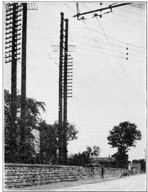
FIG. 6.—HIGH-VOLTAGE POWER CROSSING WHERE ACCIDENT OCCURRED IN 1914.
