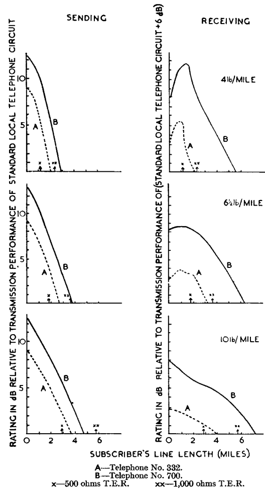
FIG. 15.—TRANSMISSION PERFORMANCE RATINGS OF TELEPHONES NO. 332 AND NO. 700.
