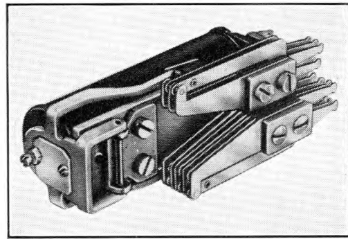
(c) Strowger Horizontal Relay (A.T.M. Co.).
