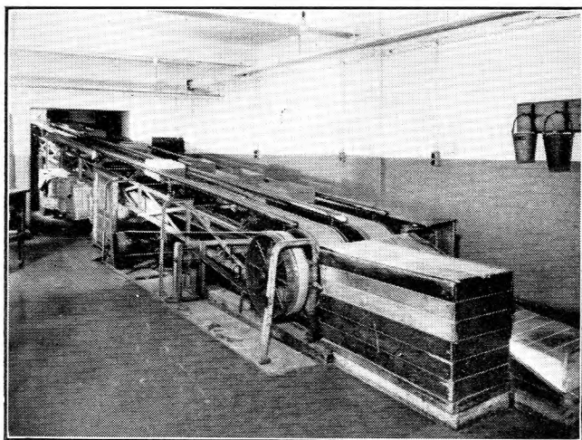
FIG. 1.—THE FIRST CONVEYOR BELT IN THE BRITISH POST OFFICE (WITH GUARDS REMOVED).
