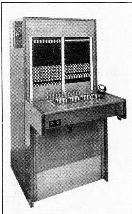
FIG. 18.—MODERN LAMP-SIGNALLING SWITCHBOARD (P.M.B.X. No. 1A).
