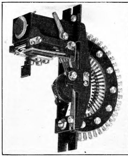
(b) An Early Type of 25-Point Unisector (A.T.E. Co.).
