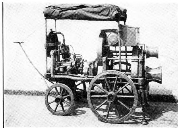
FIG. 10.—EARLY POWER-DRIVEN WINCH.
