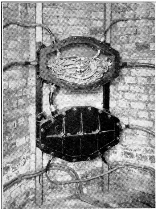
FIG. 12.—AN EARLY CABLE DISTRIBUTION HEAD.
