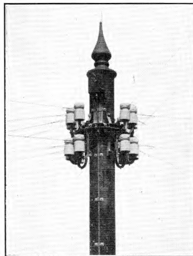
FIG. 5.—THE TOP OF A RING-TYPE DISTRIBUTION POLE.
