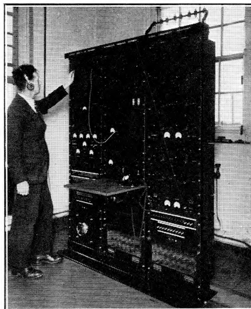
FIG. 5.—SHORT-WAVE TELEPHONY RECEIVER AT BALDOCK RADIO STATION.
