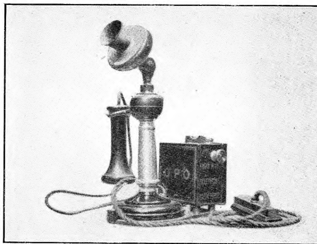
FIG. 12.—THE FIRST POST OFFICE COIN-COLLECTING BOX, WITH TELEPHONE.
