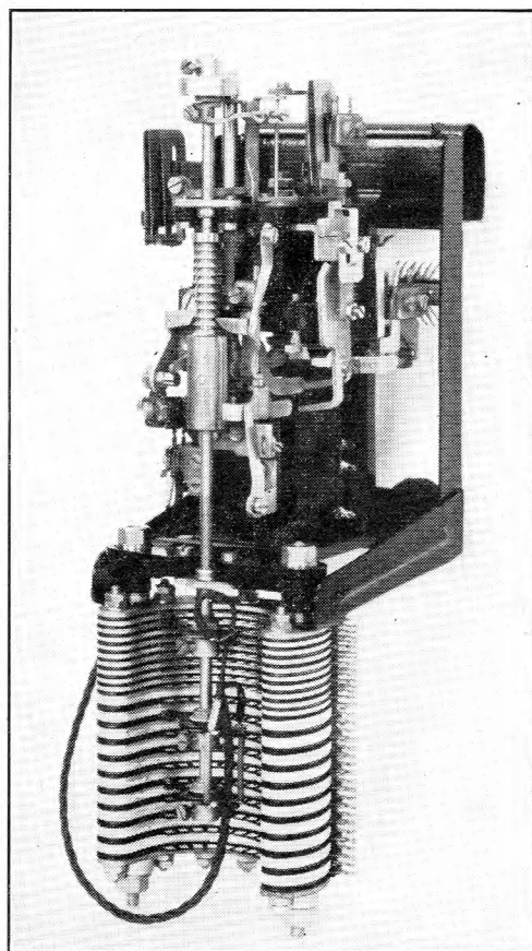
FIG. 5.—AN EARLY TWO-MOTION SWITCH (SIEMENS BROS.).
