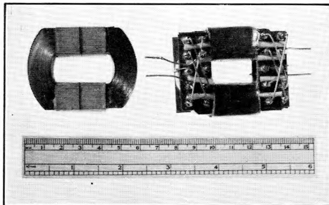
NOTE: The response of the transformer is 1dB down at 40 c/s and 2.5 Mc/s.
