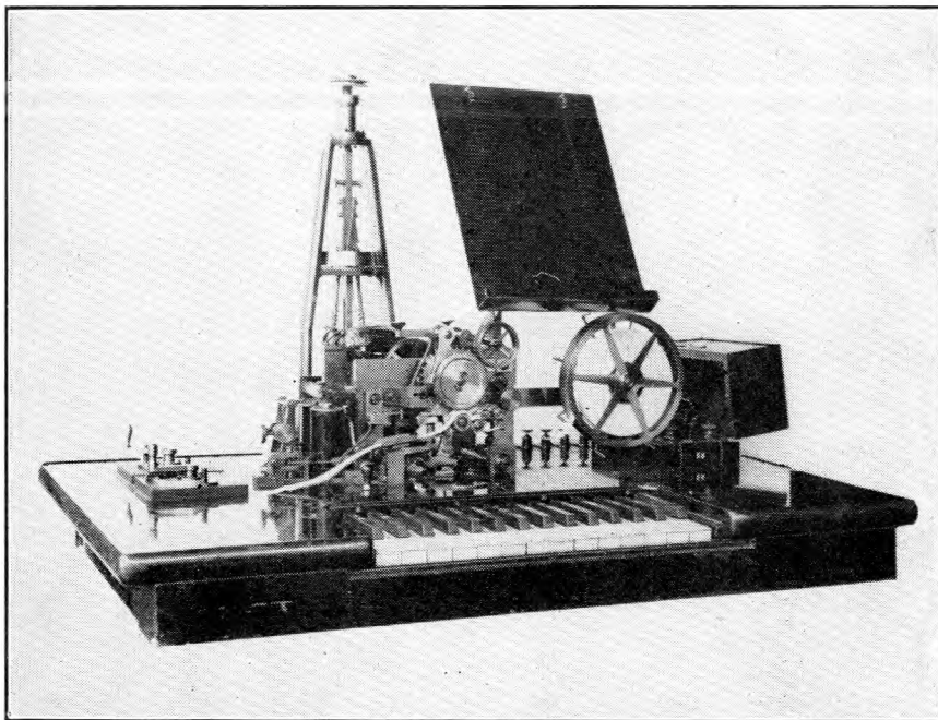
FIG. 1.—THE HUGHES INSTRUMENT.
