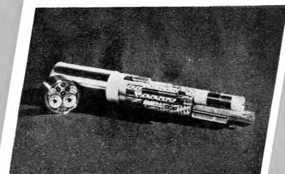
Section of the large tube coaxial cable—London to Birmingham T.V. link, 1949
