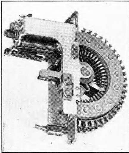
(c) Post Office Unisector No. 1.
