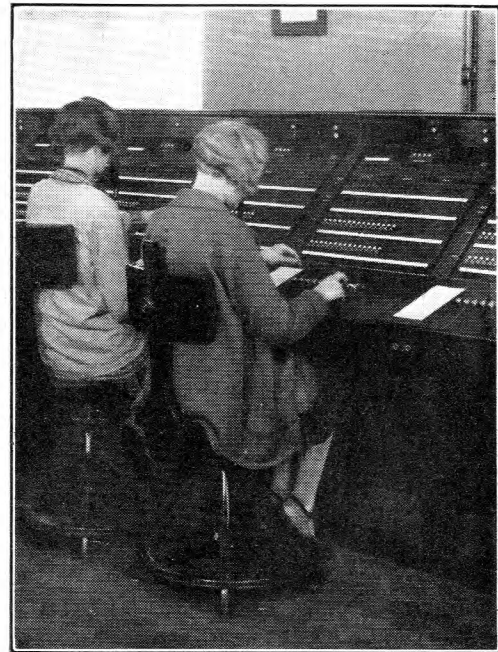
FIG. 9.—CORDLESS B POSITIONS AT A MECHANICAL TANDEM EXCHANGE.
