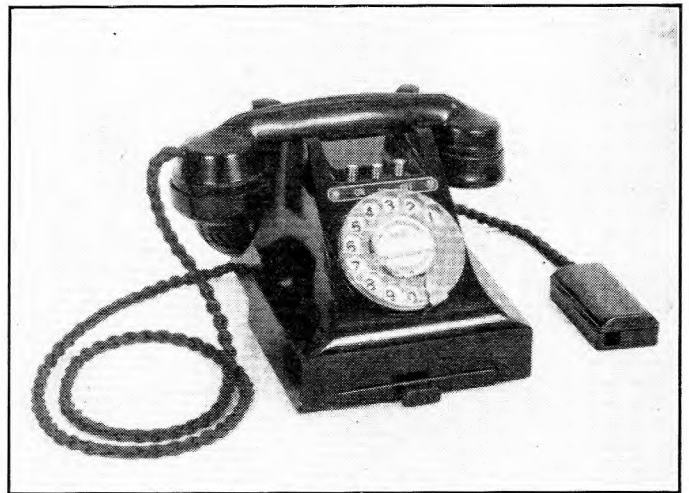
FIG. 9.—TELEPHONE NO. 328.
