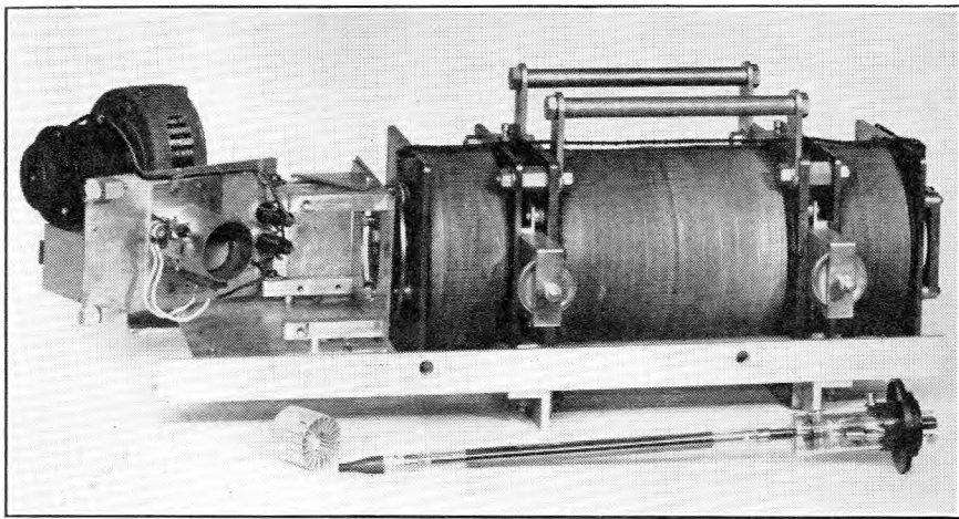
FIG. 14.—TRAVELLING-WAVE AMPLIFIER.
