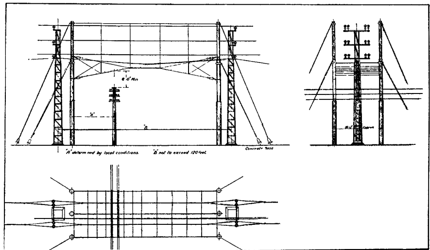
FIG. 16.—AN EARLY FORM OF CRADLE GUARD. (REPRODUCTION OF AN OLD PRINT.)
