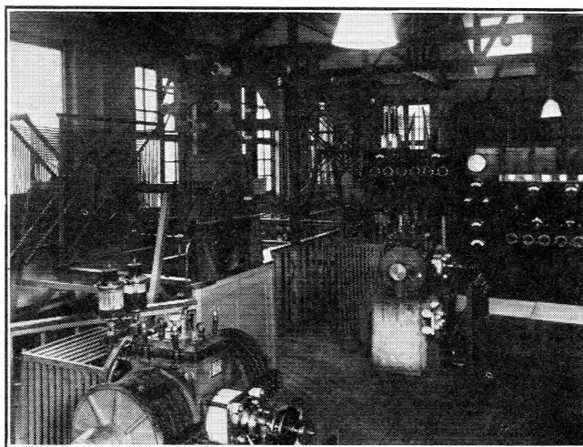
FIG. 1.—NORTHOLT RADIO STATION: POULSEN ARC TRANSMITTER, WITH VALVE TRANSMITTER IN THE BACKGROUND.
