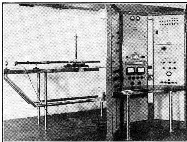
NOTE: The measurement is by a Rayleigh Disk at the centre of the horizontal tube, and observations are made at the table in front of the three racks.
