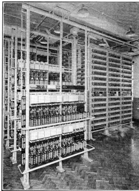
FIG. 6.—SINGLE-SIDED APPARATUS RACKS AT AN EARLY SIEMENS EXCHANGE.
