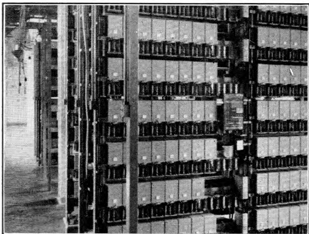
FIG. 13.—TYPICAL INSTALLATION OF 2000-TYPE EQUIPMENT.
