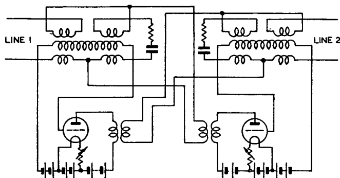
FIG. 3.—DOUBLE REPEATER.
