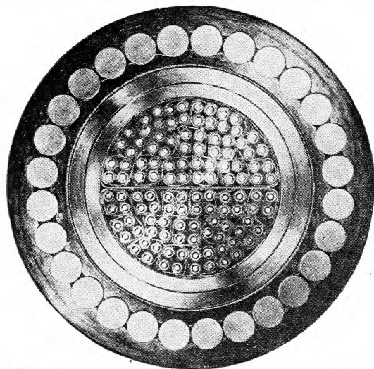
FIG. 6.—CROSS-SECTION OF ANGLO-BELGIAN CABLE OF 1932 (ACTUAL SIZE).
