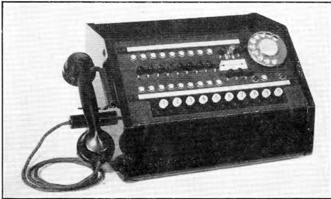
FIG. 20.—CORDLESS SWITCHBOARD USED WITH P.A.B.X. No. 1.
