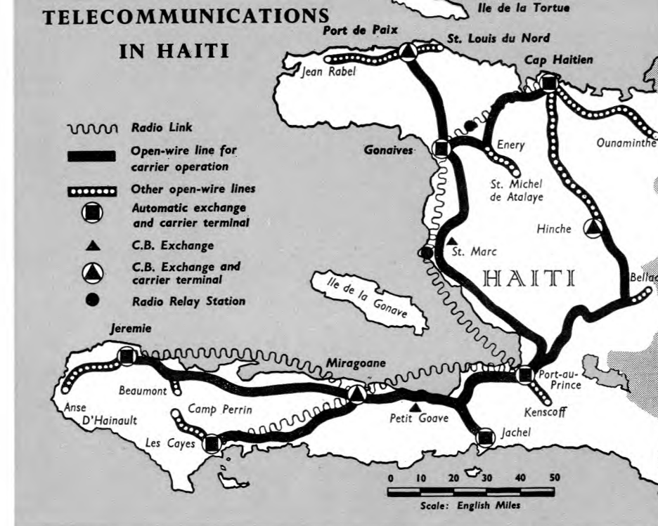
The network of open-wire lines, radio links and exchanges in Haiti. This system is one of the many systems throughout the world for which G.E.C. is responsible for the planning, manufacture and installation.
