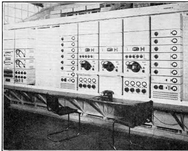
FIG. 7.—GENERAL MONITOR AND CONTROL POSITIONS OF M.U.S.A. RECEIVING SYSTEM.
