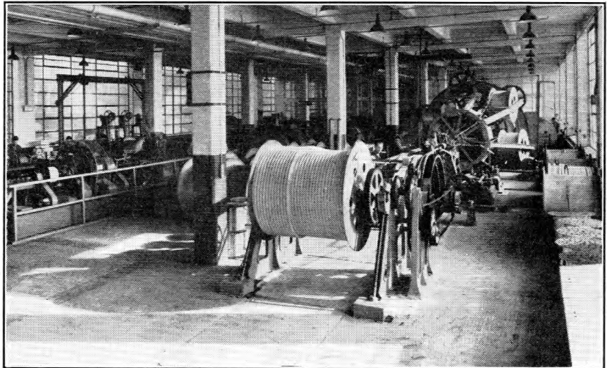
LAYING-UP THE FIRST COAXIAL CABLE, 1935.
