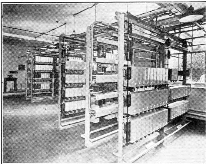
FIG. 21.—TYPICAL 500-LINE INSTALLATION OF P.A.B.X. No. 3.
