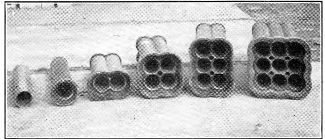
FIG. 4.—SELF-ALIGNING GLAZED EARTHENWARE DUCTS.
