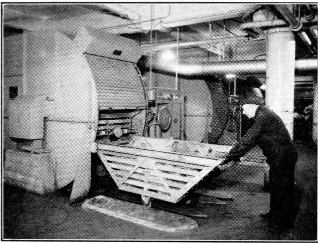
FIG. 8.—BAG-CLEANING MACHINE.
