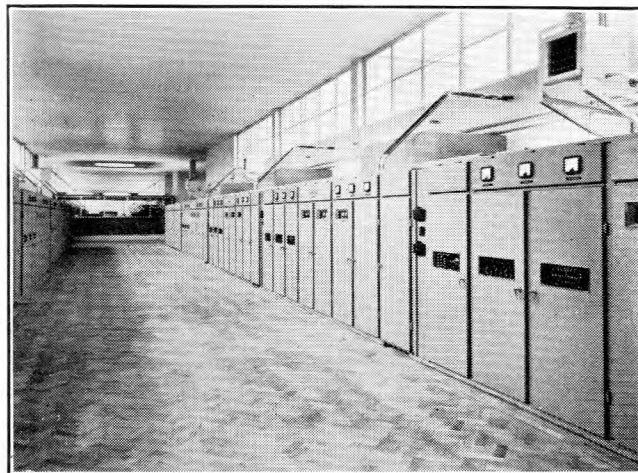
FIG. 10.—TRANSMITTER WING AT THE NEW RUGBY RADIO STATION.
