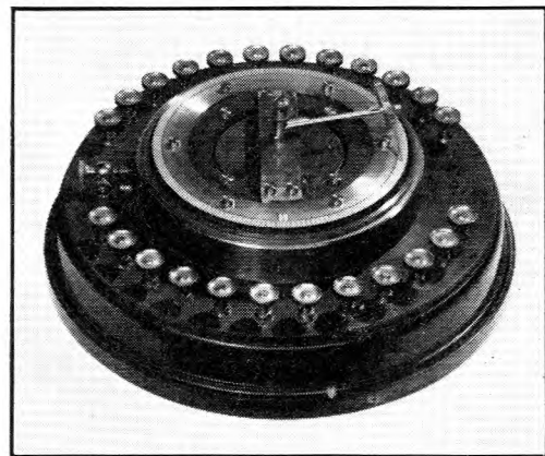
FIG. 1.—DELANEY MULTIPLEX DISTRIBUTOR (1882).
