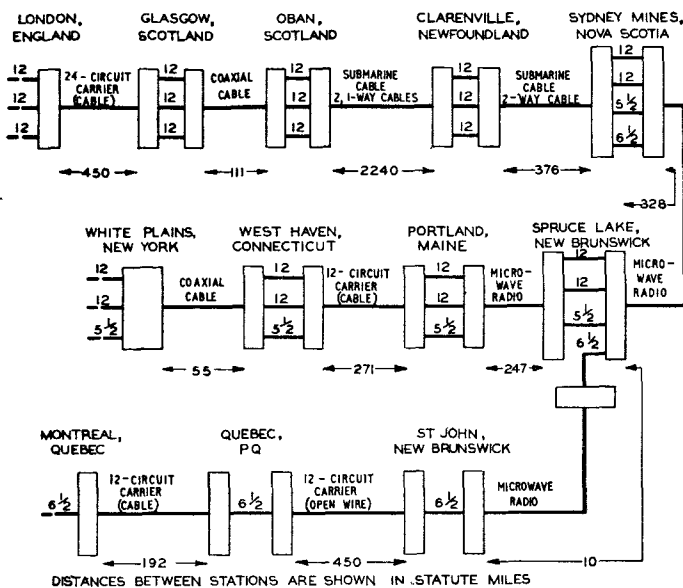
Total distances: London–New York, 4,078 miles; London–Montreal, 4,157 miles. Maintenance circuits, U.S.A.–Canada circuits are not shown. FIG. 2. —FACILITIES USED FOR THE TRANSATLANTIC SUBMARINE TELEPHONE CABLE SYSTEM.
