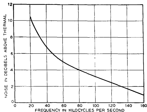
FIG. 21.—REPEATER NOISE.
