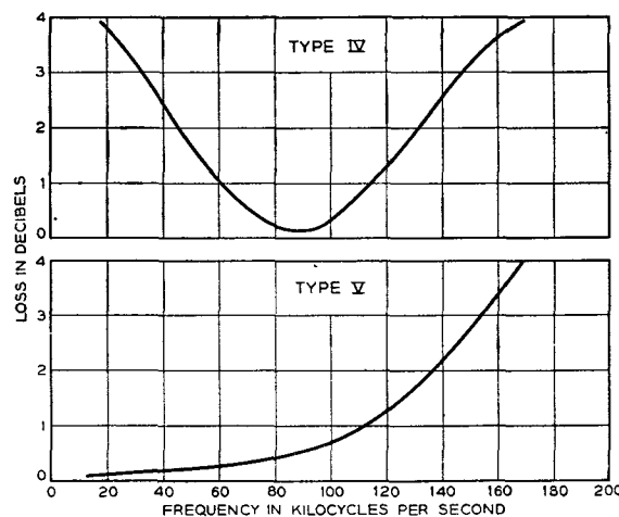
FIG. 23.—EQUALIZER LOSS CHARACTERISTICS.
