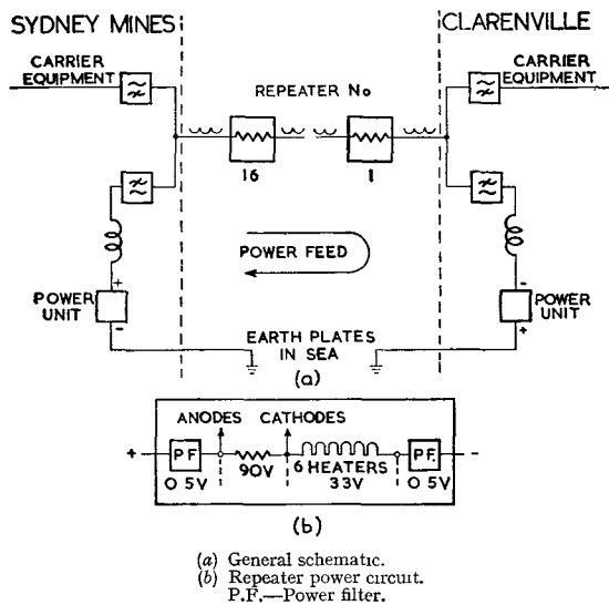
FIG. 6.—POWER-FEEDING ARRANGEMENTS.
