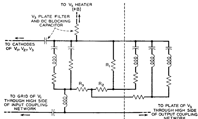
FIG. 8.—BETA NETWORK.
