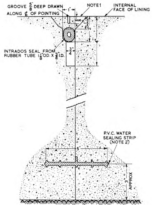
FIG. 6.—DETAILS OF CONSTRUCTION JOINT.
