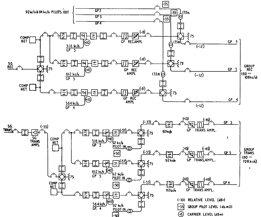
FIG. 3.—BLOCK SCHEMATIC DIAGRAM OF SPECIAL FREQUENCY-TRANSLATING EQUIPMENT.
