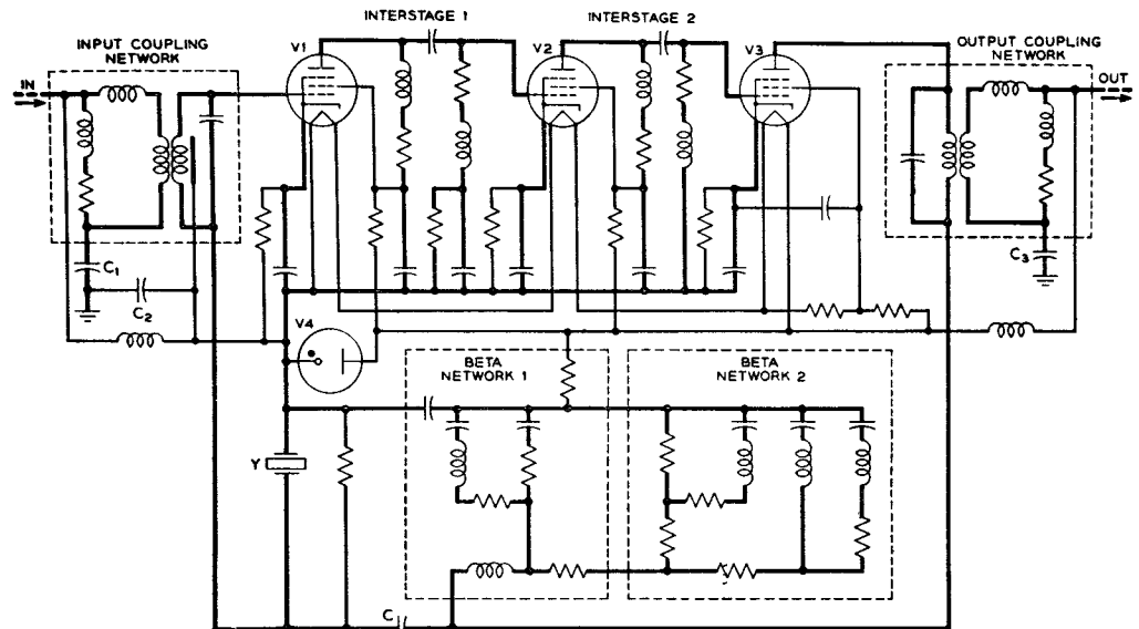
FIG. 1.—SCHEMATIC DIAGRAM OF REPEATER.
