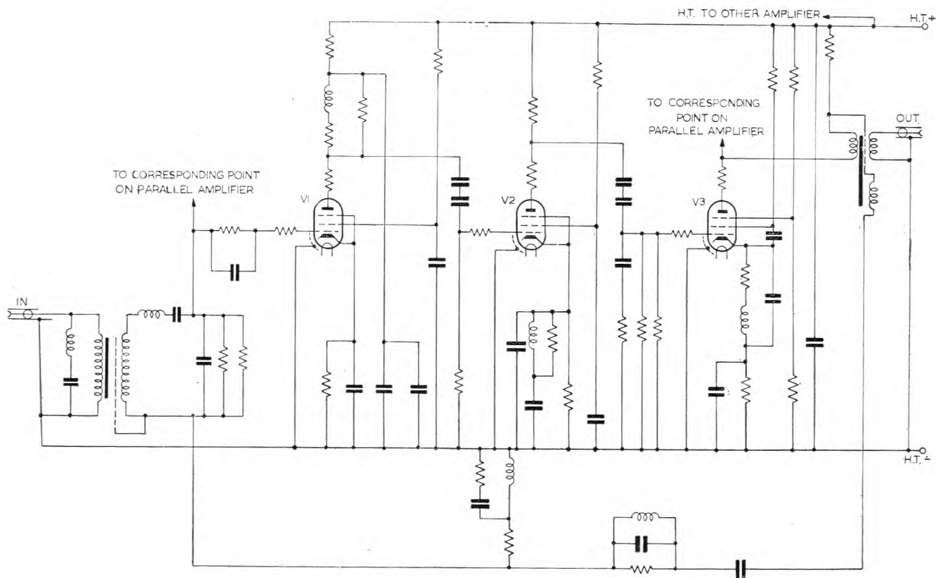
FIG. 3.—AMPLIFIER CIRCUIT.
