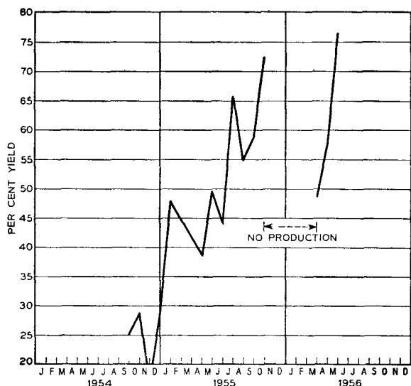
FIG. 6.—PERCENTAGE YIELDS OF MICA CAPACITORS.
