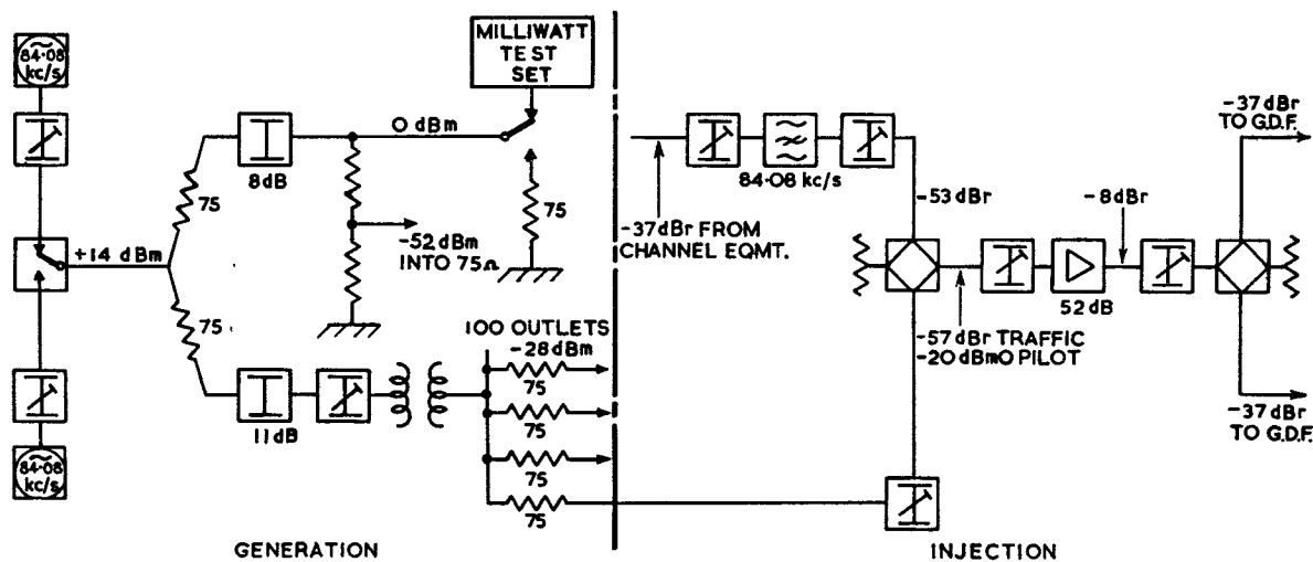
FIG. 1.—GENERATION AND INJECTION OF 84·08-KC/S PILOT SIGNAL.
