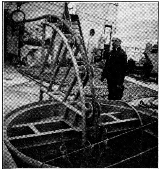
FIG. 7.—NEW ROLLER TRACK CABLE LEADS AT CABLE TANK NO. 1.
