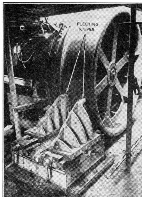
FIG. 4.—FLEETING KNIVES.
