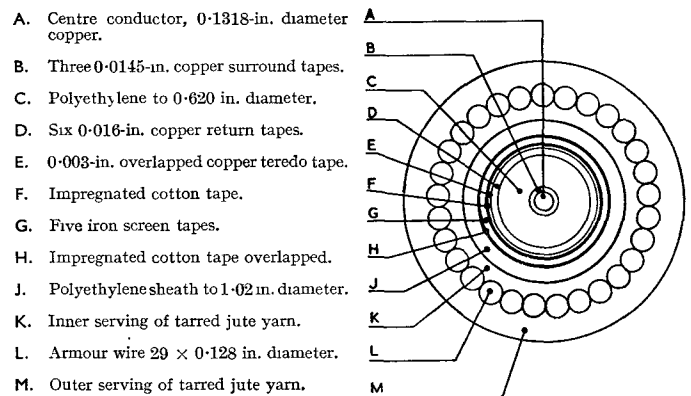
FIG. 3.—CROSS-SECTION OF CABLE ACROSS NEWFOUNDLAND SHOWING MAKE-UP.
