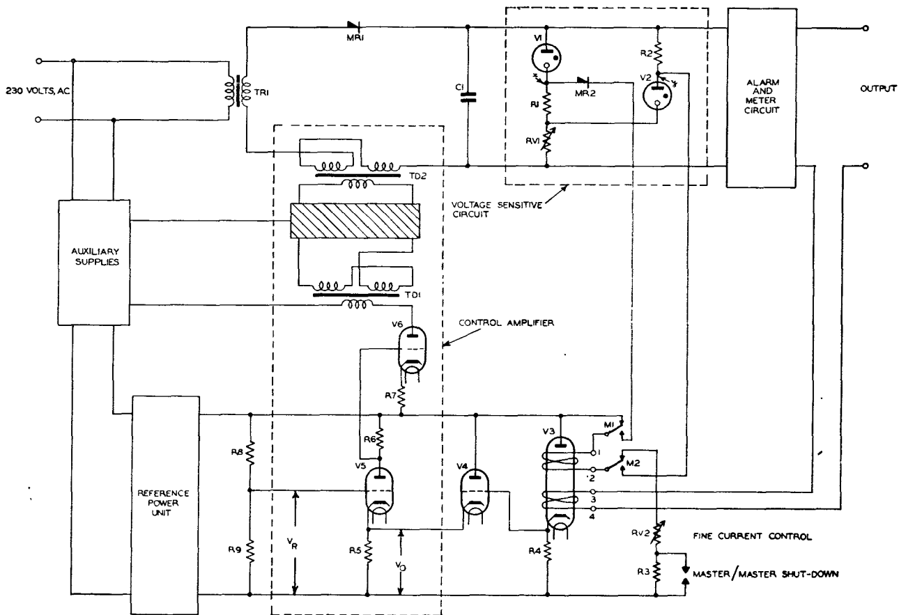
FIG. 5.—SIMPLIFIED SCHEMATIC DIAGRAM OF POWER-FEEDING EQUIPMENT.
