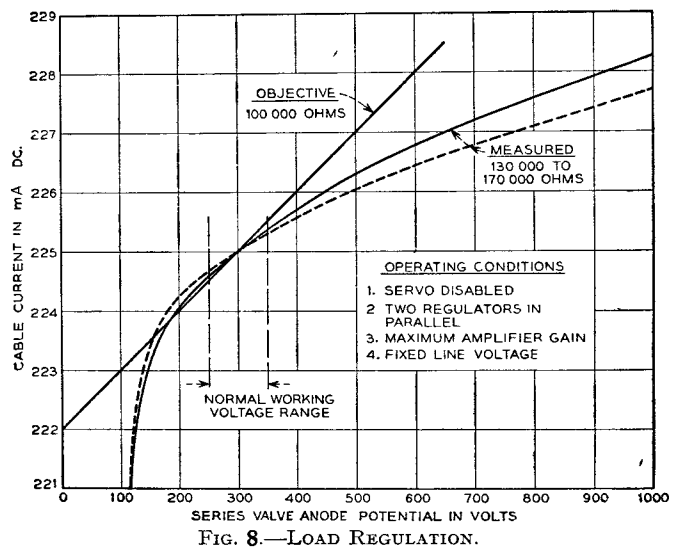
FIG. 8.—LOAD REGULATION.
