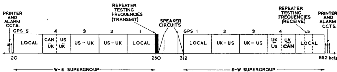
FIG. 5.—FREQUENCY ALLOCATION.
