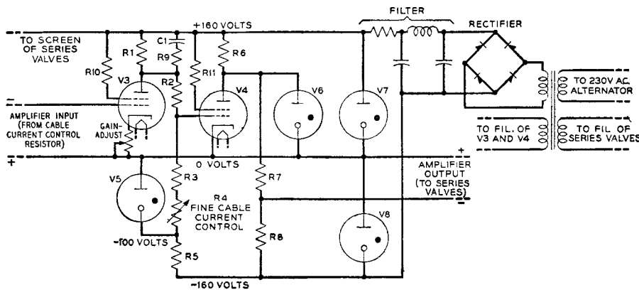
FIG. 5—TWO-STAGE D.C. AMPLIFIER.
