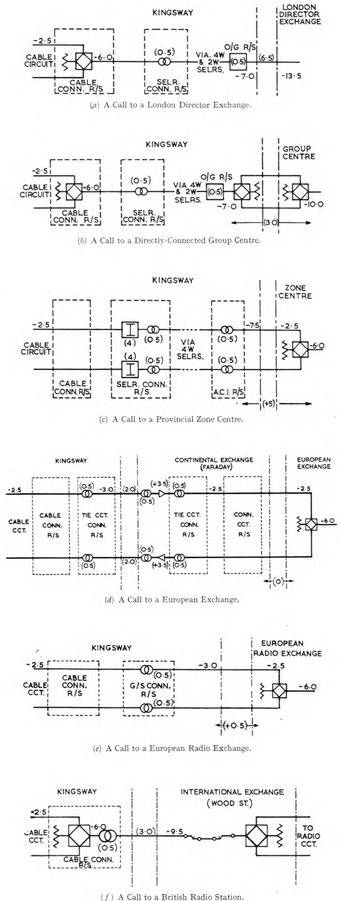
FIG. 4.—TRANSMISSION CONDITIONS ON CALLS FROM NORTH AMERICA.
