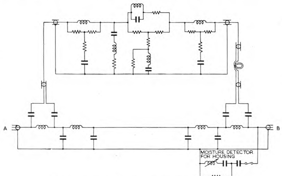
FIG. 7.—SCHEMATIC DIAGRAM OF SUBMERGED EQUALIZER.
