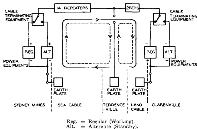
FIG. 2.—CURRENT PATHS ON CLARENVILLE—SYDNEY MINES LINK.
