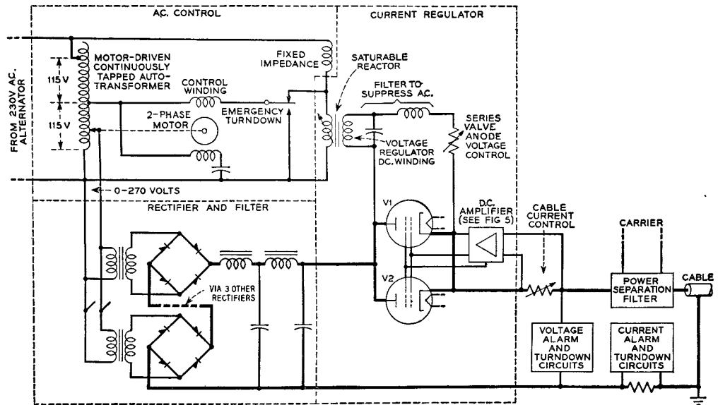
FIG. 2.—SIMPLIFIED CIRCUIT OF THE REGULATING SYSTEM.
