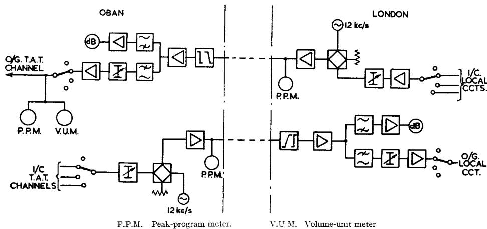
FIG. 20.—BLOCK SCHEMATIC DIAGRAM OF PROGRAM-SWITCHING EQUIPMENT AT LONDON AND OBAN.
