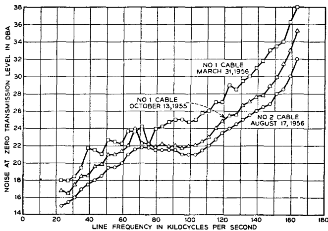
FIG. 16.—CABLE SYSTEM NOISE.
