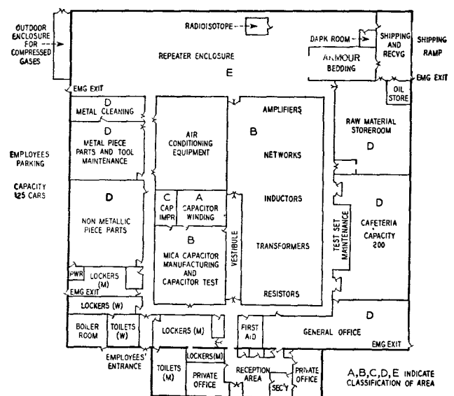
FIG. 1.—PLANT LAYOUT FOR SUBMARINE-CABLE REPEATER SHOP
