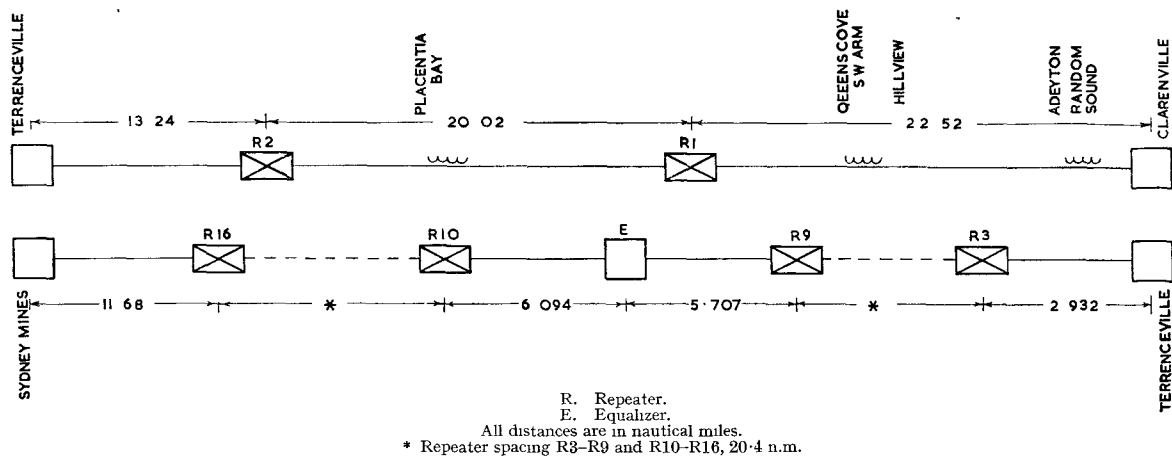
FIG. 2.—STRAIGHT-LINE DIAGRAM OF ROUTE.
