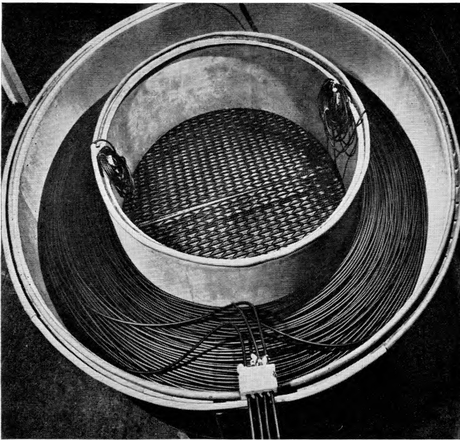
FIG. 5.—SPECIAL WATER TANK OR PAN FOR TESTS ON IMMERSIED CABLE CORE.
