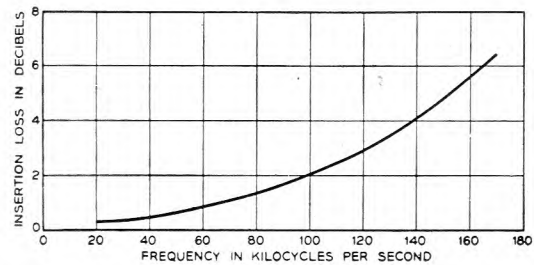
FIG. 7.—TRANSMITTING DEVIATION EQUALIZER: LOSS/FREQUENCY CHARACTERISTIC.
