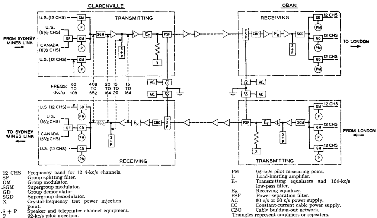
FIG. 2.—NORTH ATLANTIC LINK: BLOCK SCHEMATIC DIAGRAM.
