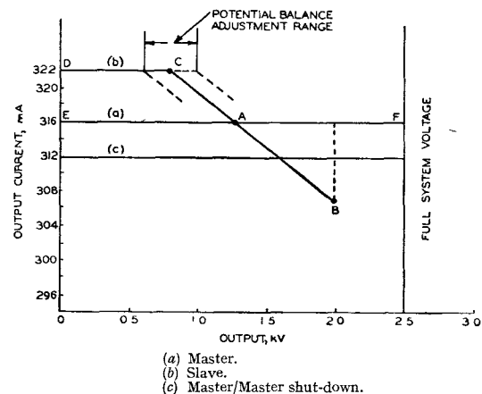
FIG. 1.—OUTPUT-CURRENT/OUTPUT-VOLTAGE CHARACTERISTICS.
