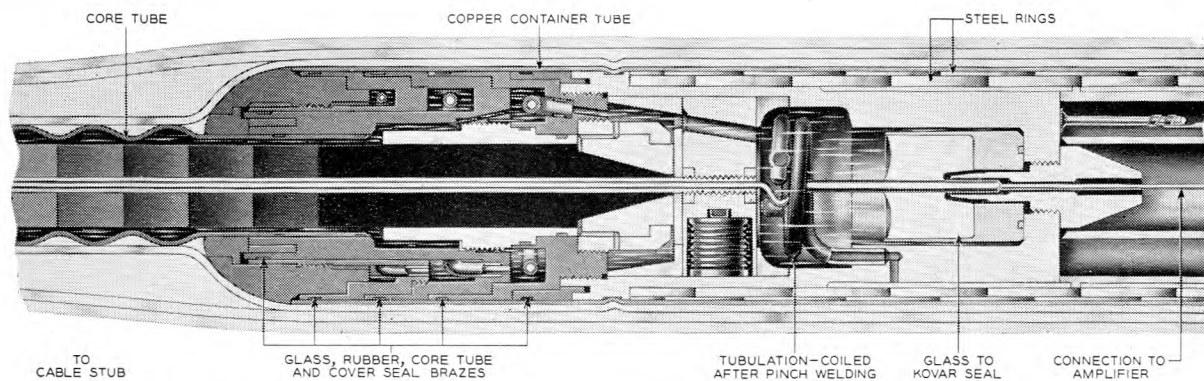
FIG. 3.—SECTIONAL VIEW OF SEAL ASSEMBLY AT EACH END OF REPEATER.
