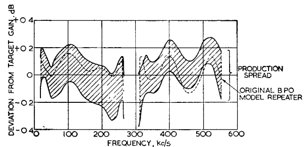
FIG. 17.—REPEATER-GAIN RESPONSE.
