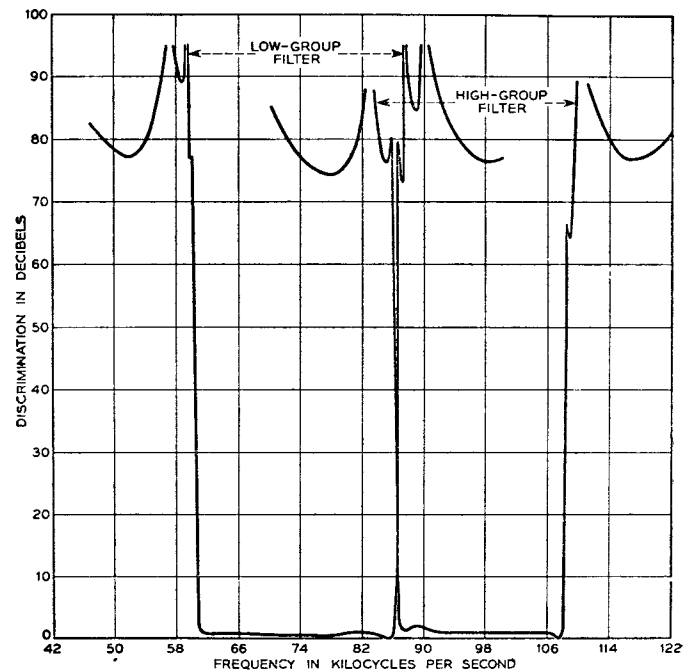
FIG. 11.—SPLITTING FILTERS: LOSS/FREQUENCY CHARACTERISTIC.
