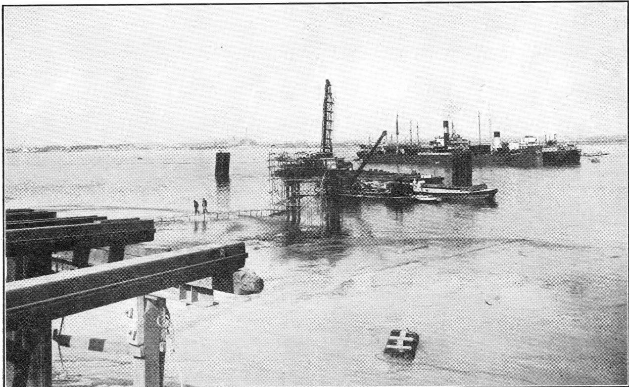
FIG. 1.—VIEW FROM THE SITE, SHOWING NATURE OF FORESHORE ON WHICH THE TANK HOUSE WAS BUILT.
