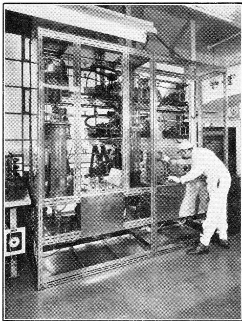
FIG. 4.—EQUIPMENT FOR VACUUM IMPREGNATION OF CAPACITORS
