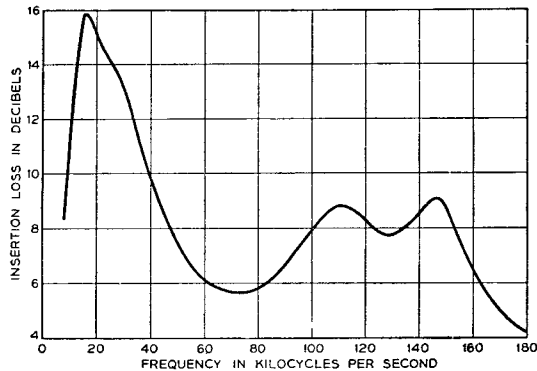
FIG. 9.—RECEIVING FIXED EQUALIZER: LOSS/FREQUENCY CHARACTERISTIC.
