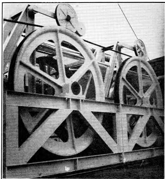
FIG. 10.—AFTER HOLDING-BACK GEAR.
