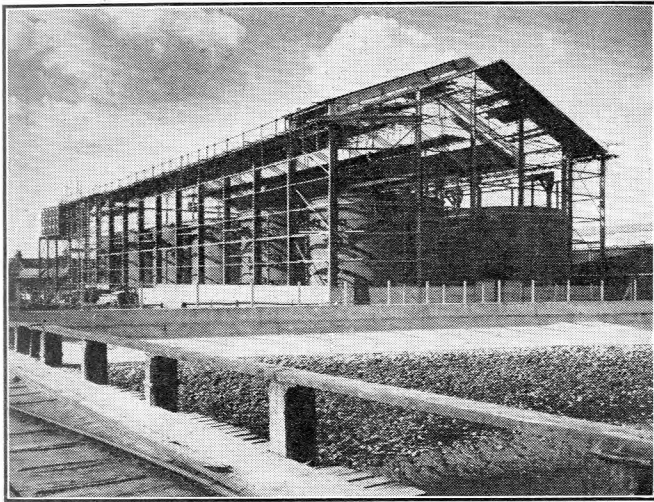
FIG. 2.—THE TANK HOUSE UNDER CONSTRUCTION.
