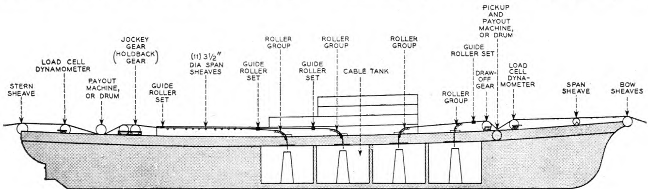
FIG. 10.—SCHEMATIC DIAGRAM OF CABLE GEAR ON H.M.T.S. "MONARCH."
