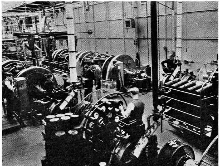
FIG. 6.—VIEW OF SHOP FOR APPLICATION OF CABLE ARMOUR.
