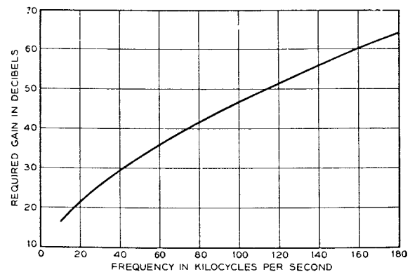
FIG. 2.—REQUIRED INSERTION GAIN.
