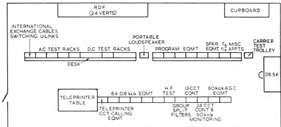
FIG. 19.—LAYOUT OF T.A.T. TEST.
