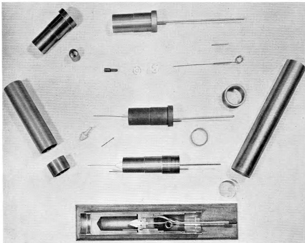
FIG. 4.—COMPONENTS, SUB-ASSEMBLIES, AND SECTIONAL VIEW OF THE GLASS SEAL USED TO CLOSE EACH END OF REPEATER CONTAINER.
