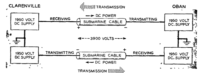
FIG. 1.—CABLE VOLTAGE SUPPLY.
