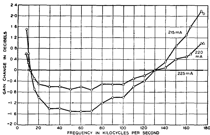
FIG. 15.—EFFECT OF CABLE CURRENT ON SYSTEM GAIN: NO. 1 CABLE.
