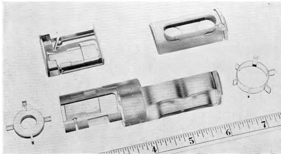
FIG. 2.—REPRESENTATIVE PARTS MACHINED FROM METHYL-METHACRYLATE.
