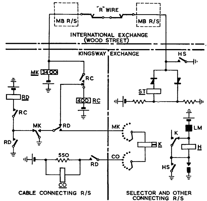
FIG. 5.—FINDER START AND MARKING CIRCUIT ELEMENTS.
