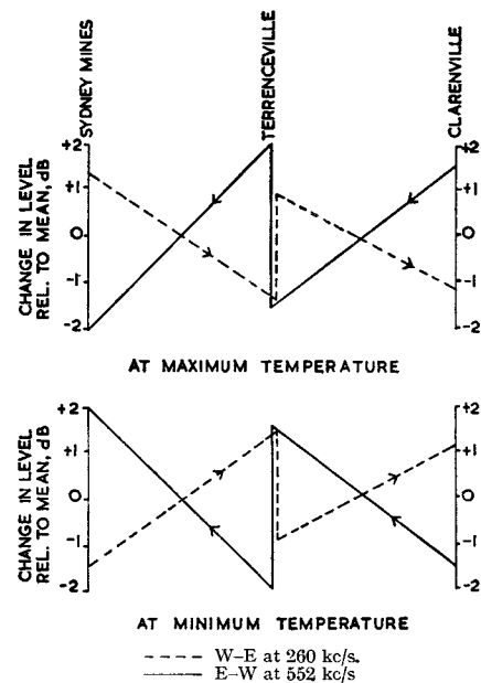
FIG. 10.—DEVIATION FROM MEAN OF TRANSMISSION LEVELS WITH OPTIMUM ADJUSTMENTS OF EQUALIZERS AT SYDNEY MINES, TERRENCEVILLE AND CLARENVILLE.
