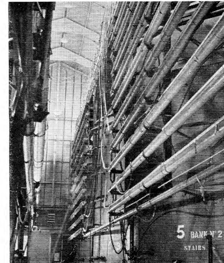
Storage tanks—each of which holds 200 miles of finished cable—showing troughs containing flexible repeaters spliced into the cable.
