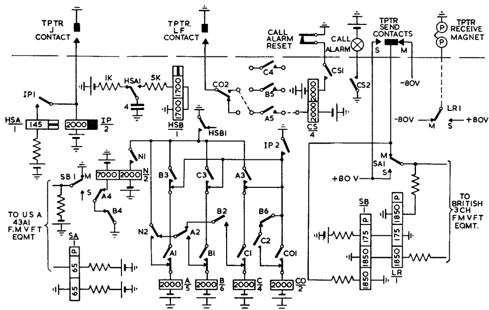
FIG. 16.—SIMPLIFIED SCHEMATIC DIAGRAM OF TELEGRAPH SIGNAL-CONVERSION AND SELECTIVE-CALL RELAY-SET AT OBAN.
