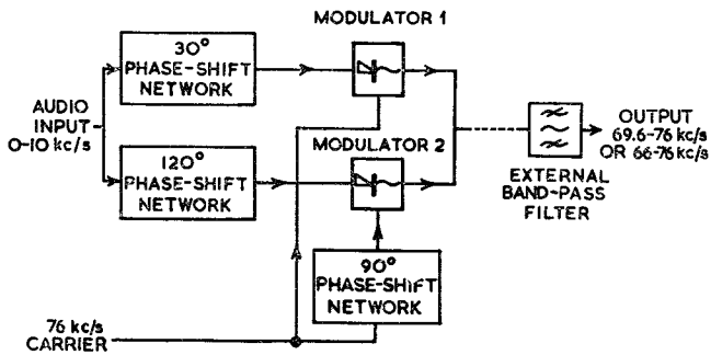
FIG. 8.—BLOCK SCHEMATIC DIAGRAM OF MODULATOR.
