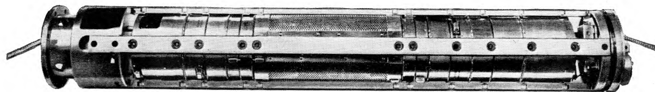
One of 16 repeaters as laid between Clarenville and Sydney Mines shown without sea casing.
