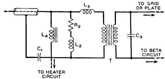
FIG. 4.—COUPLING NETWORK.
