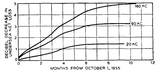
FIG. 14.—CHANGE IN SYSTEM GAIN IN FIRST 11 MONTHS.
