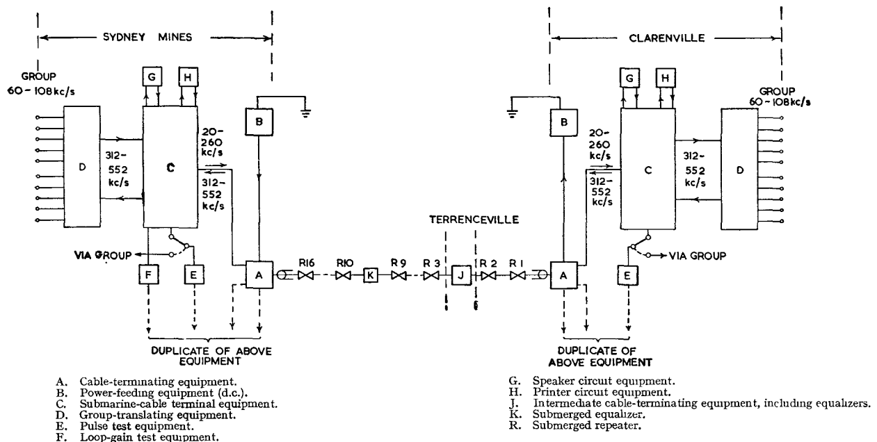
FIG. 7.—ARRANGEMENT OF TERMINAL EQUIPMENT AND REPEATERS.
