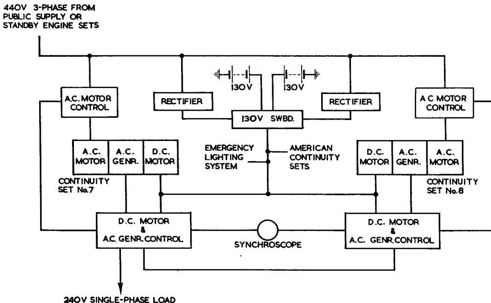
FIG. 14.—BLOCK SCHEMATIC DIAGRAM OF A.C. POWER PLANT FOR INLAND EQUIPMENT AT OBAN/B REPEATER STATION.
