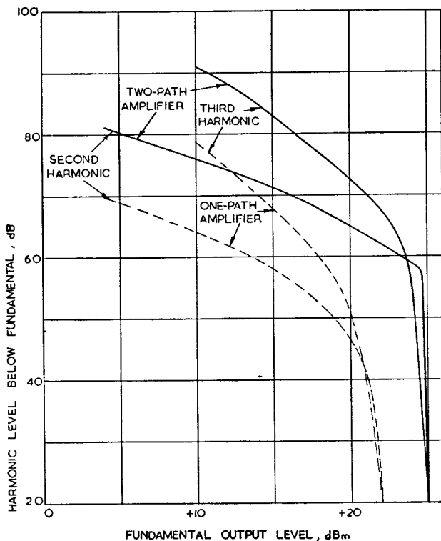
FIG. 14.—AMPLIFIER DISTORTION.
