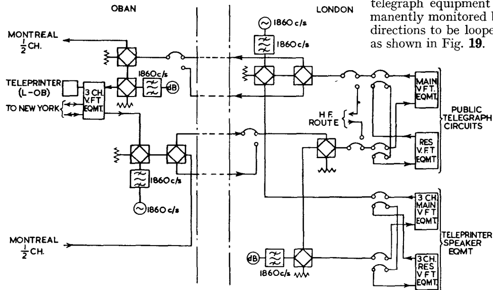
FIG. 19.—BLOCK SCHEMATIC DIAGRAM OF MONITOR AND CHANGE-OVER ARRANGEMENTS FOR V.F. TELEGRAPH CIRCUITS BETWEEN LONDON AND OBAN.
