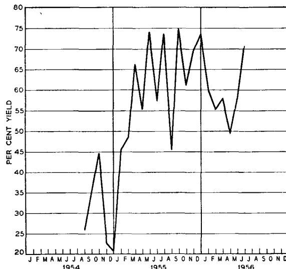
FIG. 5.—PERCENTAGE YIELDS OF PAPER CAPACITORS.
