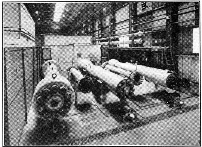
FIG. 9.—PRESSURE-TESTING EQUIPMENT.
