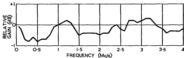
FIG. 17.—TYPICAL OVERALL GAIN/FREQUENCY CHARACTERISTIC.
