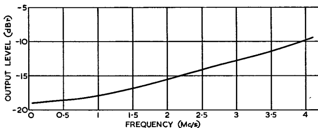
FIG. 4.—TELEPHONY RELATIVE LEVEL AT LINE AMPLIFIER OUTPUT.
