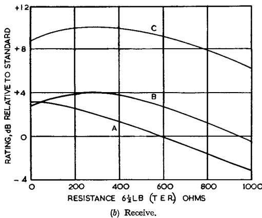
FIG. 2.—TRANSMISSION PERFORMANCE RATINGS (50V BALLAST EXCHANGES).
