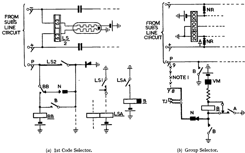
Notes: 1. The strap shown in (b) between U-points 8 and 9 is inserted when the selector is used as a subscriber's 1st selector in a uniselector exchange. 2. Modifications to existing equipment are shown by bold lines.
