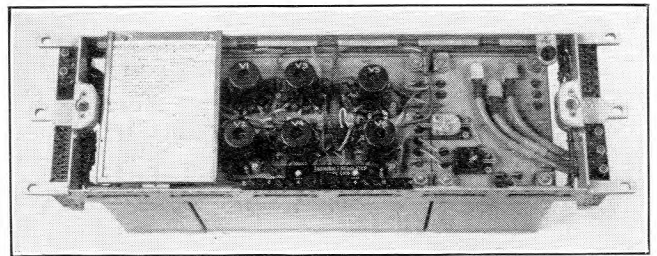
FIG. 6.—LINE AMPLIFIER.
