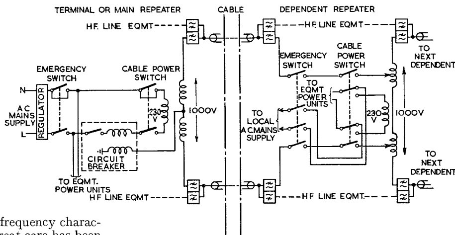
FIG. 9.—POWER-FEEDING CIRCUIT.
