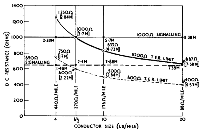
— Limiting condition for new and modified exchanges having a 1,000-ohm signalling limit. - - - Limiting condition for existing exchanges having a 650-ohm signalling limit.
