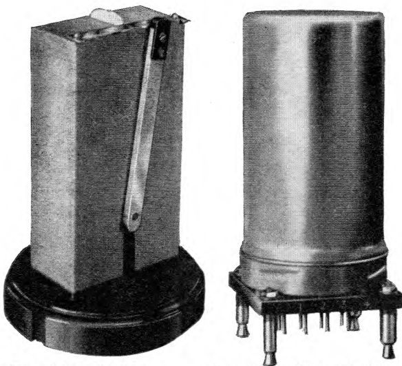
Type 3 Relay on 'Creed' base
