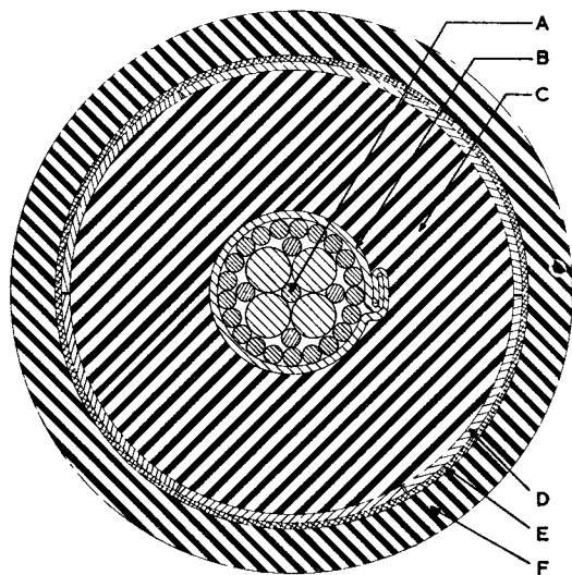
A Torsionally balanced steel strands (26/0.033 in. plus 4/0.080 in). B Longitudinal 15-mil copper tape with box seam. C Polythene to 0.800 in. diameter. D Six 15-mil aluminum tapes. E 10-mil cotton tape impregnated with corrosion inhibitor. F Polythene sheath, of outside diameter 1.02 in.
