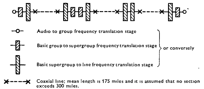
The circuit is 2,500 km (1,560 miles) in length and comprises three audio to-audio links in tandem, each having the circuit formation shown above.
