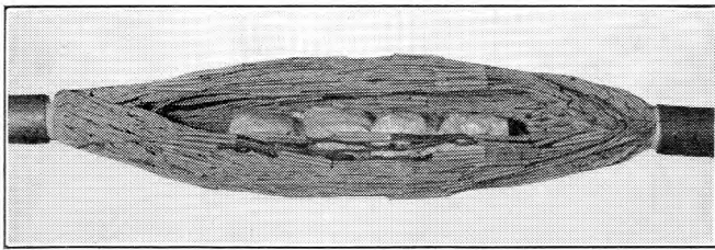
(a) The Coils in Position in the Joint.
