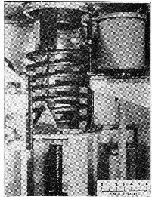
FIG. 9.—VIEW OF R.F. CIRCUIT SHOWING VARIABLE INDUCTOR AND CAPACITOR.
