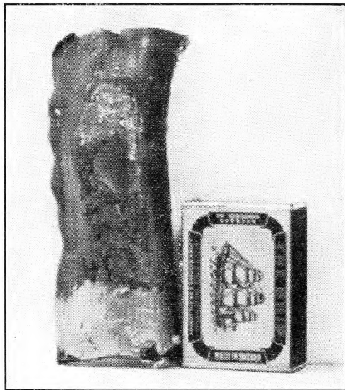
DAMAGE DONE TO CABLE SHEATH BY DORMOUSE.
