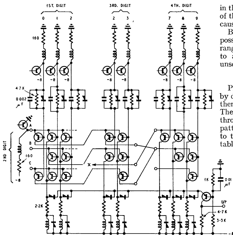
Notes: 1. Numbers exceeding 0A 2,799,999, 1B 1,699,999 and 0C 3,799,999 are redundant. 2. Point a is connected to the collector of the first transistor of the row, which is not shown. FIG. 7.—SCHEMATIC DIAGRAM OF REDUNDANCY TABLE SHOWING PARTS OF THREE MATRICES.
