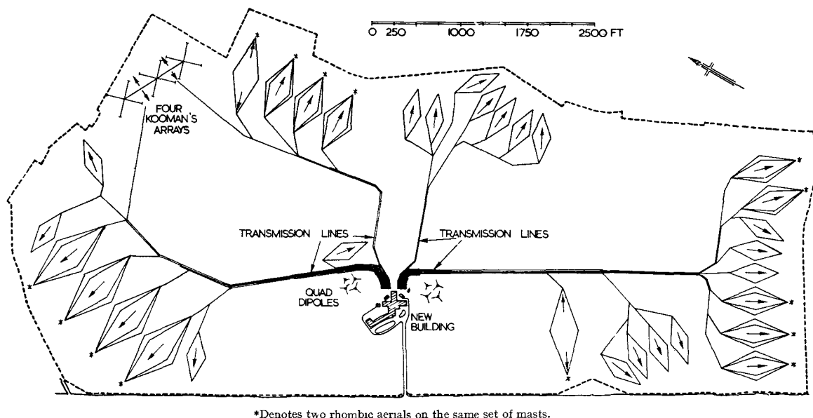
FIG. 3.—SITE PLAN OF THE NEW RUGBY RADIO STATION.
