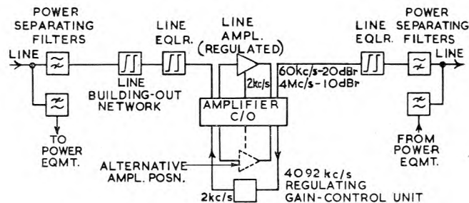
One direction of transmission only is shown; the other is identical.
