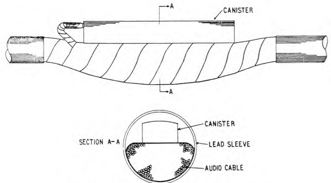
FIG. 3.—CANISTER IN AUDIO-CABLE JOINT.
