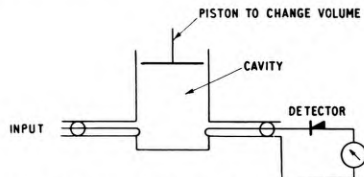
FIG. 2—PRINCIPLE OF CAVITY FREQUENCY-METER
