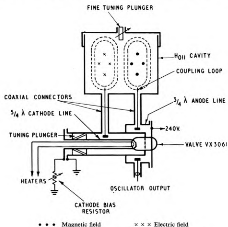
FIG. 2—DIAGRAMMATIC REPRESENTATION OF THE CAVITY-CONTROLLED OSCILLATOR
