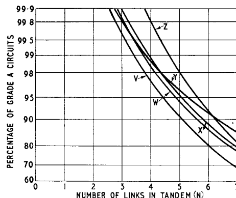
Curve V—Circuits as found during the transmission tests Curve W—Hypothetical circuits in which the average value of bias distortion per link has been reduced from 0.6 per cent marking to zero Curve X—Hypothetical circuits in which the mean value of the fortuitous distortion component of the standard deviation of distortion has been reduced to half its present value Curve Y—Hypothetical circuits in which the mean value of the characteristic distortion component of the standard deviation of distortion has been reduced to half its present value Curve Z—Hypothetical circuits in which the standard deviation of bias distortion has been reduced to half its present value. Grade A Circuits—Those of performance better than that signified by a degree of inherent distortion of 30 per cent ( P = 0.0001 )
