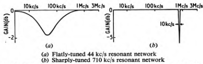
FIG. 6—GAIN/FREQUENCY RESPONSES OF RESONANT NETWORKS
