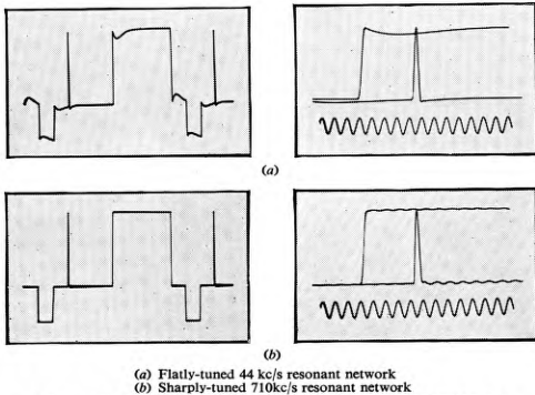
FIG. 7—WAVEFORM RESPONSES OF RESONANT NETWORKS
