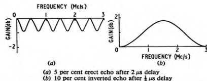
FIG. 8—GAIN/FREQUENCY RESPONSES OF ECHO DISTORTIONS
