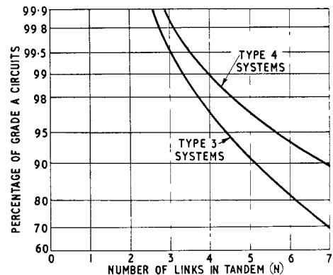
FIG. 7—COMPARISON OF TYPE 3 AND TYPE 4 V.F. TELEGRAPH SYSTEMS
