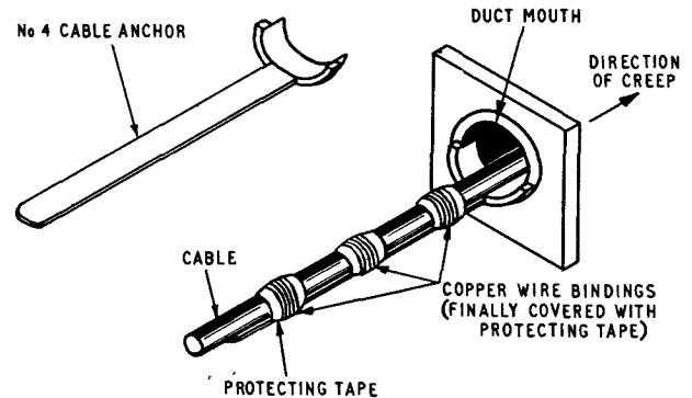
FIG. 4—"SUGAR SHOVEL" TYPE OF ANTI-CREEPAGE DEVICE
