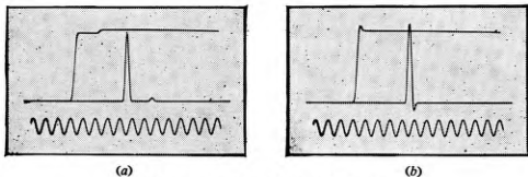
FIG. 9—WAVEFORM RESPONSES OF ECHO DISTORTIONS
