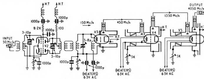
V2—QOV02-6; V3 and V4—CV354; V5—VX3061 FIG. 4—BASIC CIRCUIT OF 50/4,050 Mc/s MULTIPLIER
