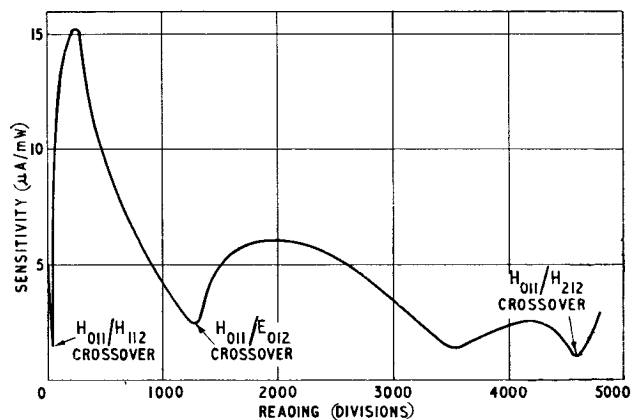
FIG. 8—SENSITIVITY
