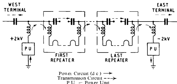
FIG. 2—SUBMARINE-CABLE POWER-FEEDING ARRANGEMENTS (TAT-1)
