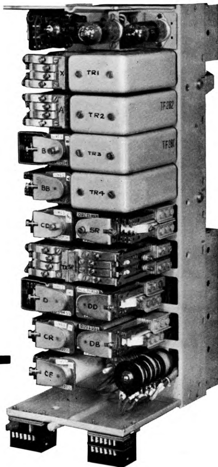
1VF Terminal Relay Set
