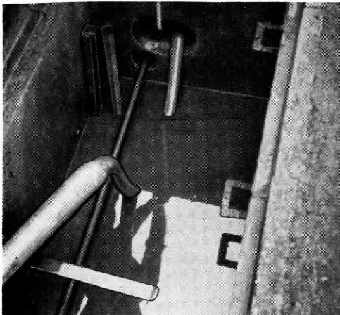
FIG. 8—EFFECT OF CABLE CREEPAGE: SLACK CABLE ACCUMULATED IN JOINTING CHAMBER
