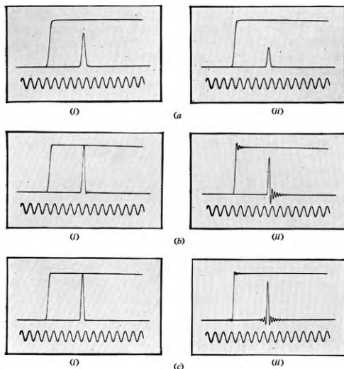
(a) \frac{1}{2} \mu s sine-squared pulse-shaping network (b) 3.2 Mc/s low-pass filter (c) Phase-equalized 3.2 Mc/s low-pass filter
