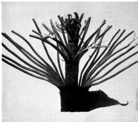
SECTION OF OLD TELEGRAPH CABLE RECOVERED AT TAMWORTH
