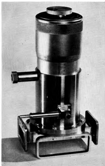
FIG. 1— H_{011} CAVITY FREQUENCY-METER, 3,975–4,275 MC/S
