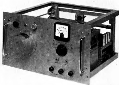
FIG. 3—CAVITY-CONTROLLED MICROWAVE CARRIER SOURCE
