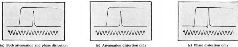
FIG. 12—WAVEFORM RESPONSES OF ATTENUATION AND PHASE DISTORTIONS
