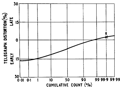
FIG. 1—DISTORTION MEASURED ON A TYPICAL CIRCUIT
