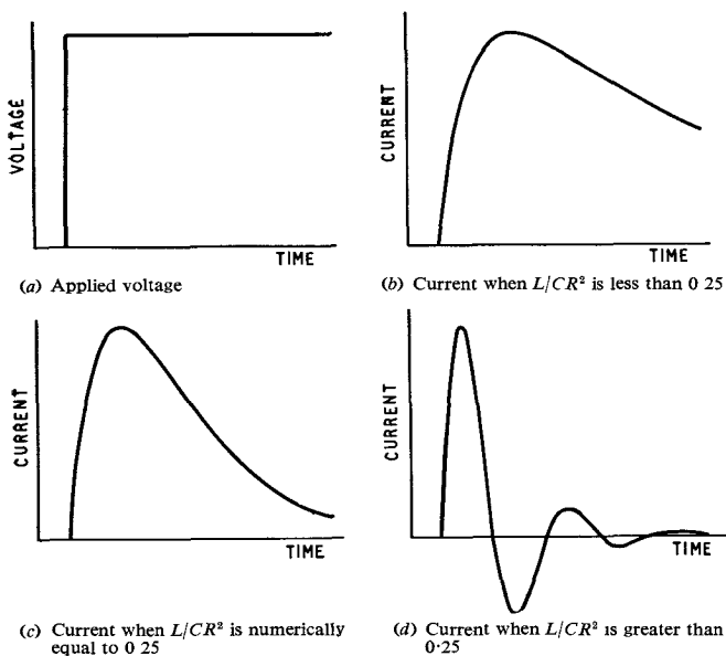
FIG. 1—STEP RESPONSE OF R, L, C CIRCUIT
