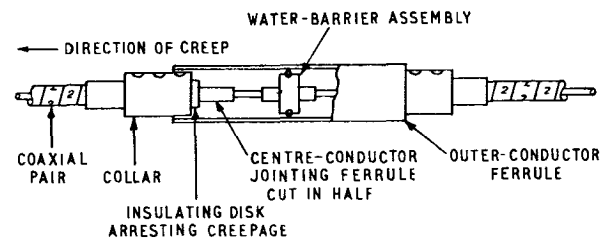
(b) Anti-centre-conductor-creepage device for coaxial cables
