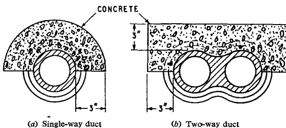
FIG. 3—METHOD OF DAMPING DUCTS
