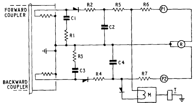
FIG. 3—REFLECTOMETER USING DIRECTIONAL COUPLERS
