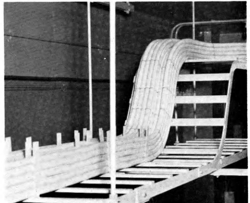
FIG. 3—EXAMPLE OF CABLE CLIPS AND STITCHING
