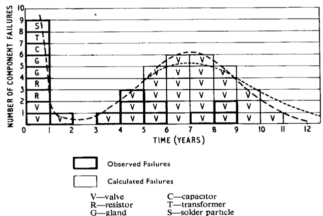
Many examples are known of normal (--- curve) or skewed-normal (--- curve) distributions in time of failures of a single type of component during accelerated life-tests, but little information is available relating to the whole working life of complete batches of a single type of component.
