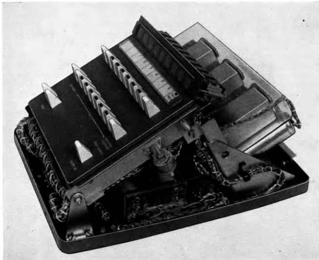
FIG. 2.—CHASSIS OF SWITCHBOARD CLOSED
