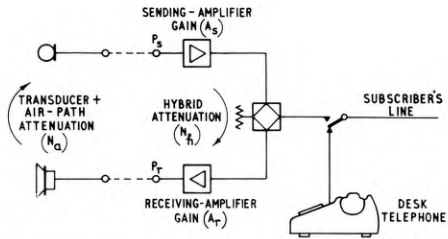
FIG. 2—SCHEMATIC DIAGRAM OF A LOUDSPEAKING TELEPHONE
