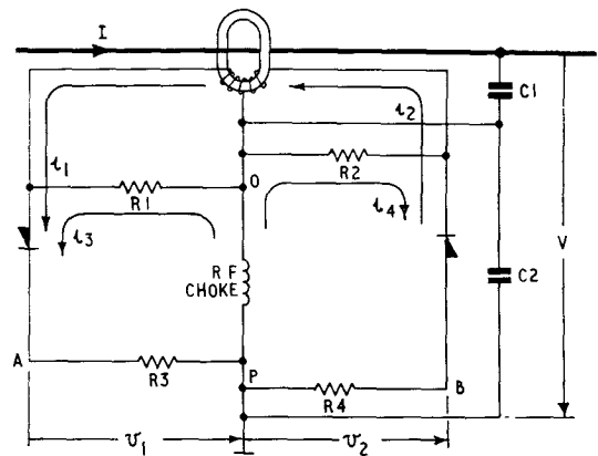
FIG. 4—REFLECTOMETER USING LINE CURRENT AND VOLTAGE COUPLING
