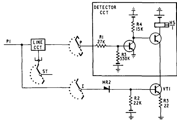
FIG 8—THE INHIBIT CIRCUIT TO PREVENT SWITCHING TO A POSITIVE-BATTERY METER PULSE
