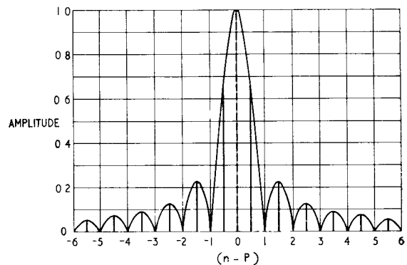
FIG. 3—ENVELOPE OF BEAT-FREQUENCY SPECTRA
