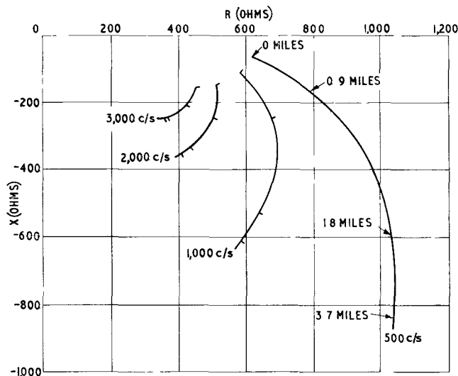
FIG. 10.—CHANGE OF BALANCE IMPEDANCE WITH LENGTH OF SUBSCRIBER'S LINE AND WITH FREQUENCY For 50-volt exchange and 6\frac{1}{2} lb/mile conductors
