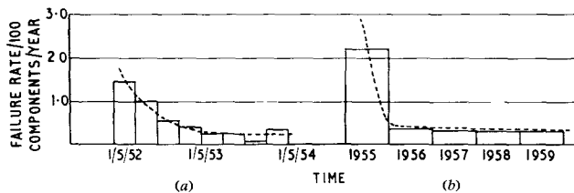
(a) 20 db video amplifiers (b) Experimental electronic director, Richmond exchange FIG. 3—FAILURES PER 100 COMPONENTS PER YEAR
