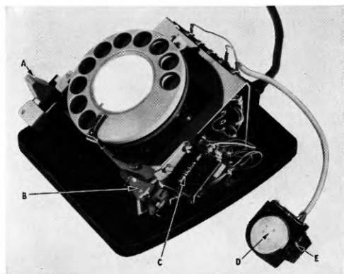
A = Volume control. B = ON/OFF key. C = Relay K. D = Microphone. E = Indicator lamp.
