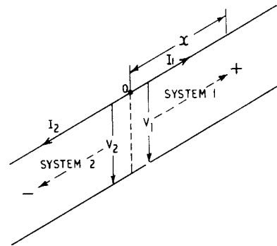
FIG. 1.—TRANSMISSION LINE CARRYING TWO OPPOSITELY-TRAVELLING ELECTROMAGNETIC-WAVE SYSTEMS
