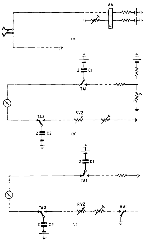
FIG 1—ELEMENTS OF NEW DIAL-TEST CIRCUIT
