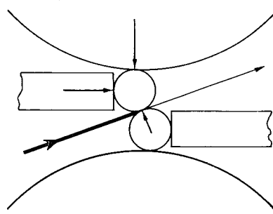
FIG. 2—INCLINED-ROLL METHOD OF SUPPORTING WORK ROLLS
