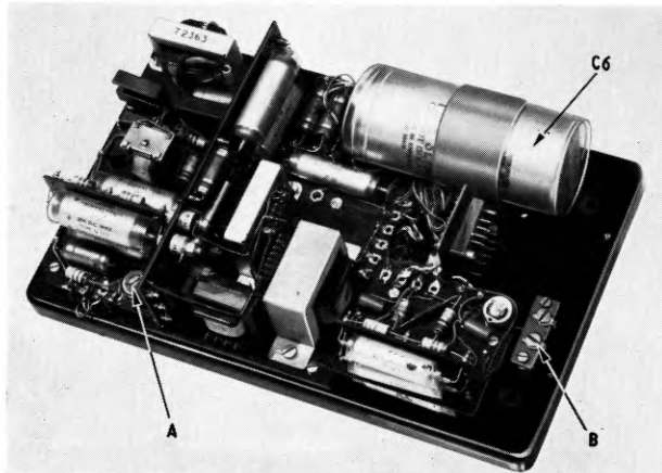
(a) Complete Amplifier
