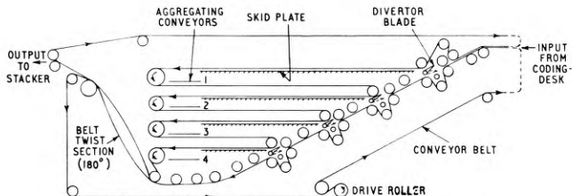
FIG. 4—EXPLANATORY DIAGRAM OF PRIMARY CONVEYOR
