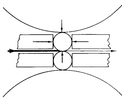
FIG. 1—WORK ROLLS SUPPORTED BETWEEN FOUR BEARING PADS
