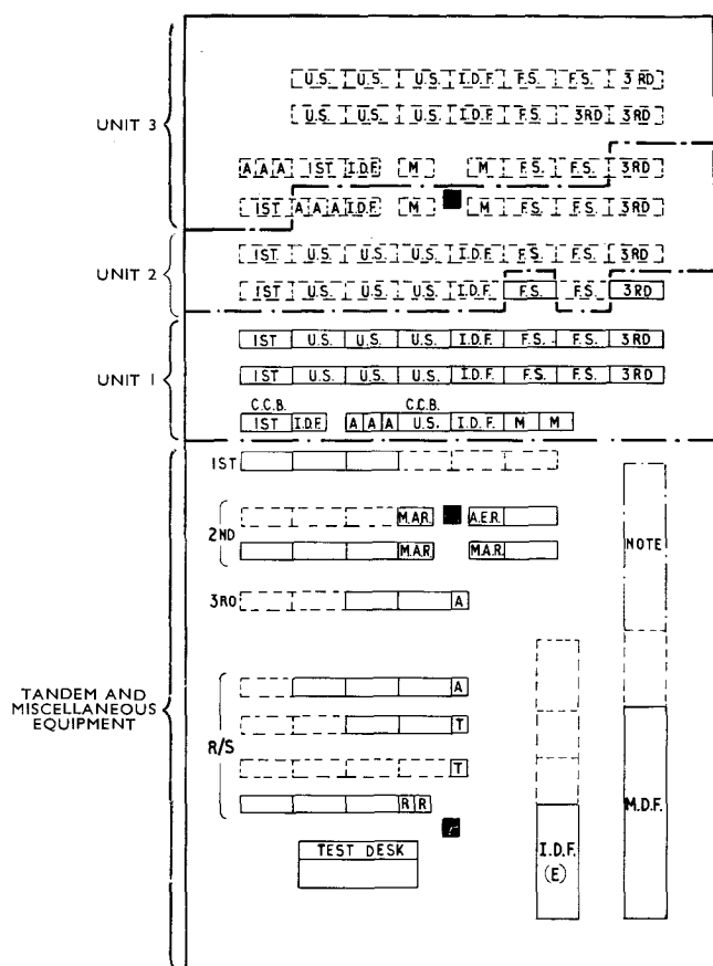
Legend: — Equipment provided initially - - - Additional equipment Note: This extension of the M.D.F. will enable it to serve all equipment ultimately provided on the exchange site. I.D.F. (E) = Equipment I.D.F. A = Router or traffic-recorder access equipment T = Traffic-recorder control rack R = Router rack M = Meter rack AER = Alarm equipment rack MAR = Miscellaneous apparatus rack C.C.B. = Coin-box equipment
