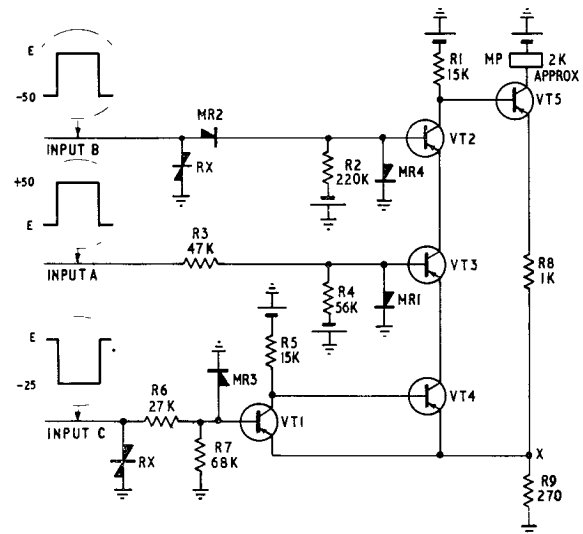
FIG. 7—THE METER-PULSE DETECTION UNIT
