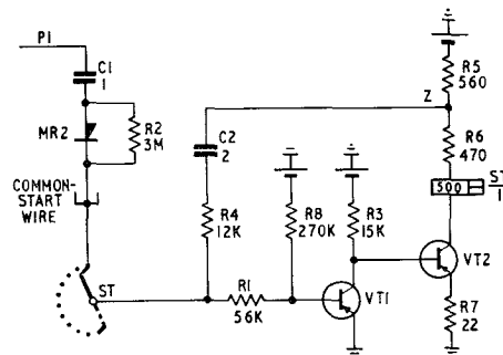
FIG. 5—THE START CIRCUIT
