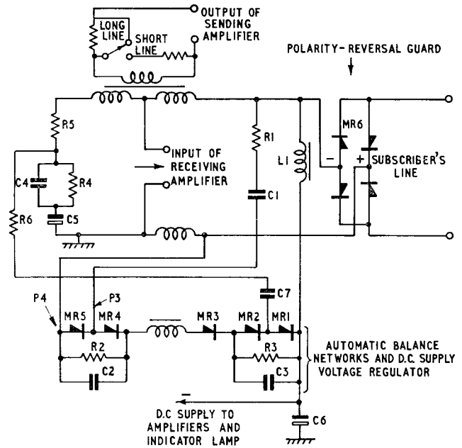
FIG. 9—AUTOMATIC BALANCE-CONTROL UNIT
