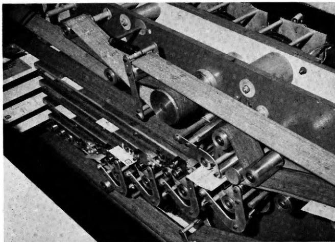
FIG. 3—PRIMARY CONVEYOR
