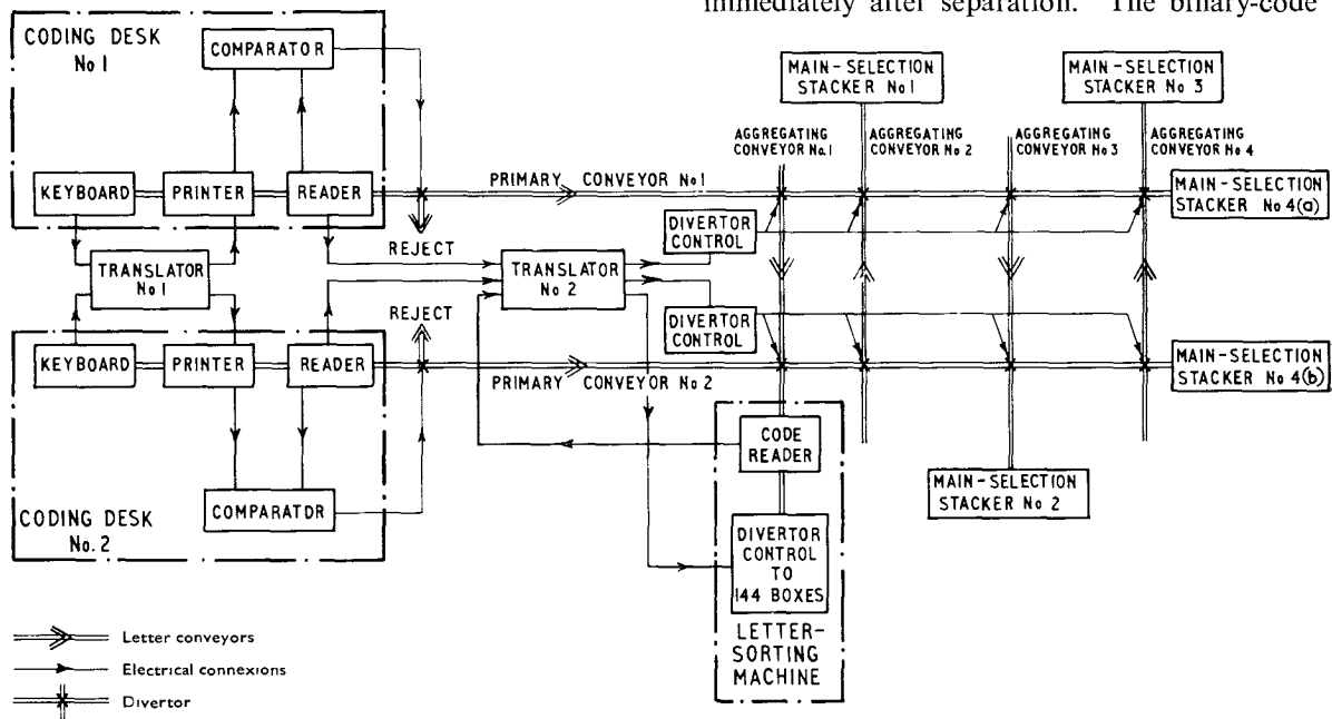
FIG. 2—DIAGRAM OF LUTON SCHEME
