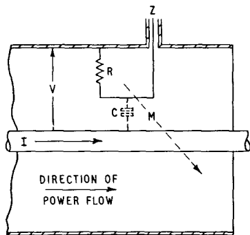
FIG. 2—DIRECTIONAL COUPLER IN A COAXIAL CABLE
