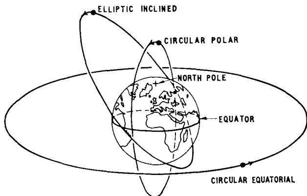
FIG. 1—TYPICAL COMMUNICATION SATELLITE ORBITS
