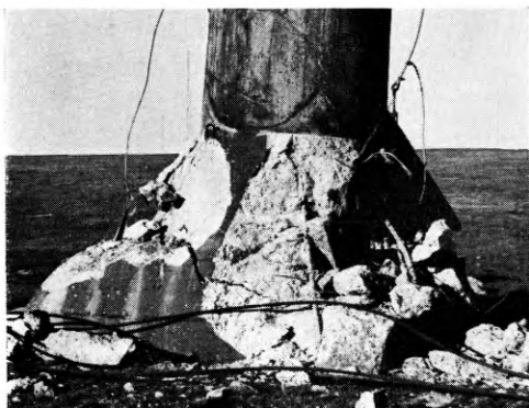
FIG. 4—BASE OF SECOND MAST AFTER FALL
