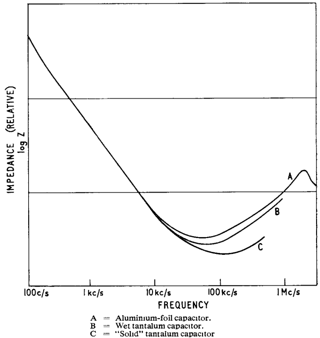
FIG. 9—VARIATION OF IMPEDANCE WITH FREQUENCY
