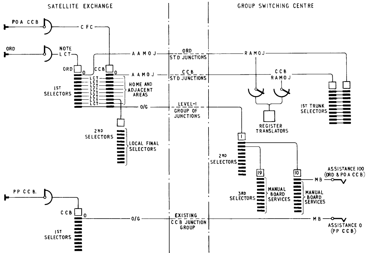
FIG. 5—TRUNKING ARRANGEMENTS AT GROUP-SELECTOR SATELLITE EXCHANGE
