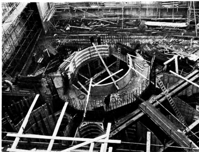
FIG. 2—WORK IN PROGRESS ON TOWER FOUNDATIONS
