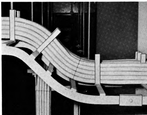
FIG. 1—USE OF CABLE CLIPS
