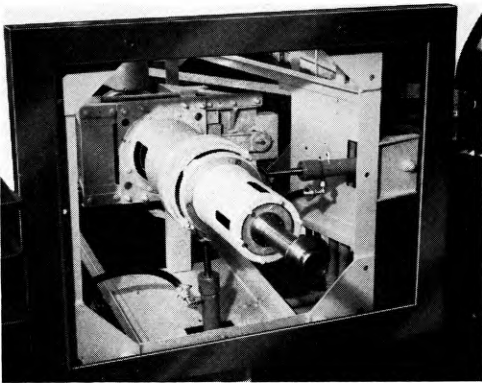
FIG. 5—AERIAL-FEED SCANNING MECHANISM
