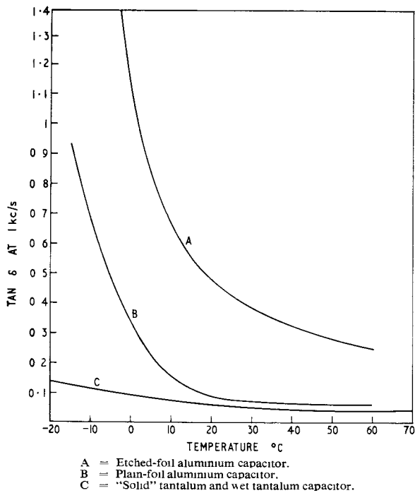
FIG. 8—CHANGE OF TAN \delta WITH TEMPERATURE
