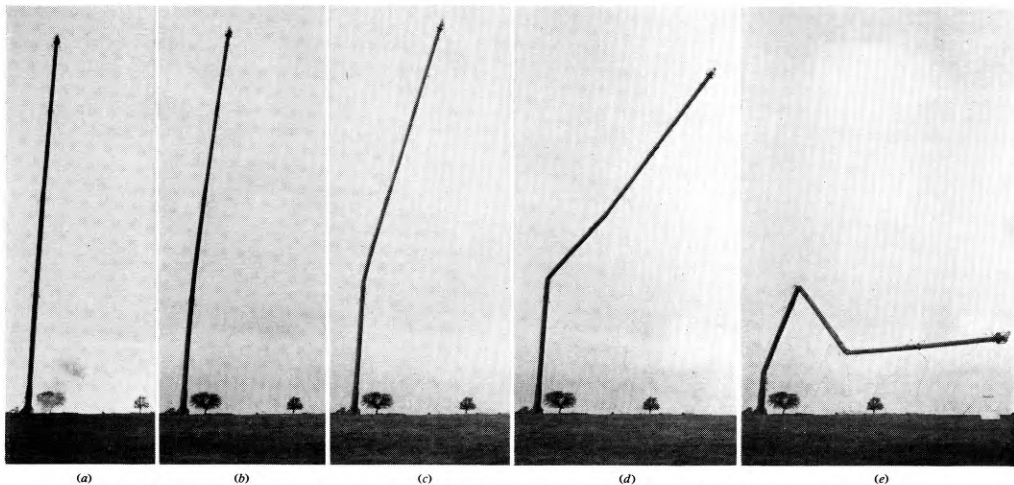
(a) Start of fall, earth surrounding base being blasted; (b) After 3.2 seconds; (c) After 7.3 seconds; (d) After 10.4 seconds; (e) After 12.2 seconds.
