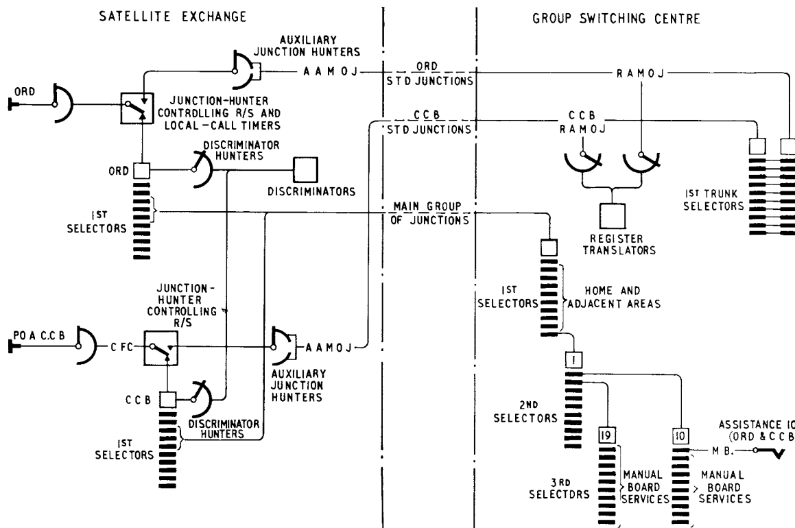
FIG. 4—TRUNKING ARRANGEMENTS AT 2,000-TYPE-DISCRIMINATOR SATELLITE EXCHANGE
