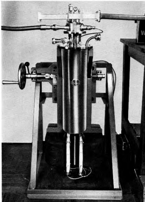
FIG. 9—THE GOONHILLY MASER AMPLIFIER
