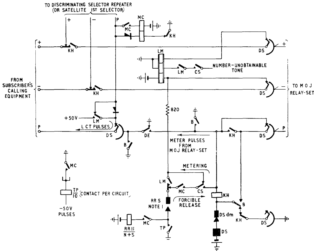
FIG 3—BASIC CIRCUIT OF AUXILIARY JUNCTION-HUNTER AT POSITIVE-BATTERY-METERING EXCHANGES
