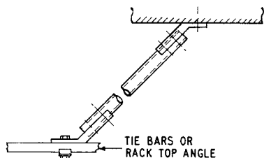
FIG. 7.—TUBULAR STRUT FOR APPARATUS-RACK SUPPORT
