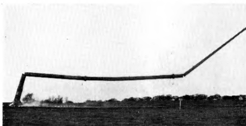
FIG. 5—THIRD MAST JUST BEFORE HITTING GROUND
