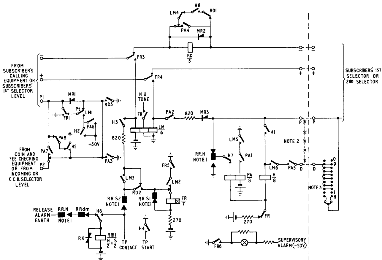
FIG. 2—CIRCUIT OF LOCAL-CALL TIMER
