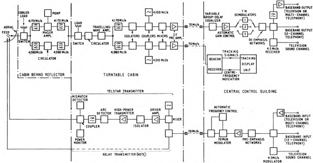
FIG. 6—SIMPLIFIED BLOCK-SCHEMATIC DIAGRAM OF THE GOONHILLY GROUND-STATION TRANSMISSION EQUIPMENT
