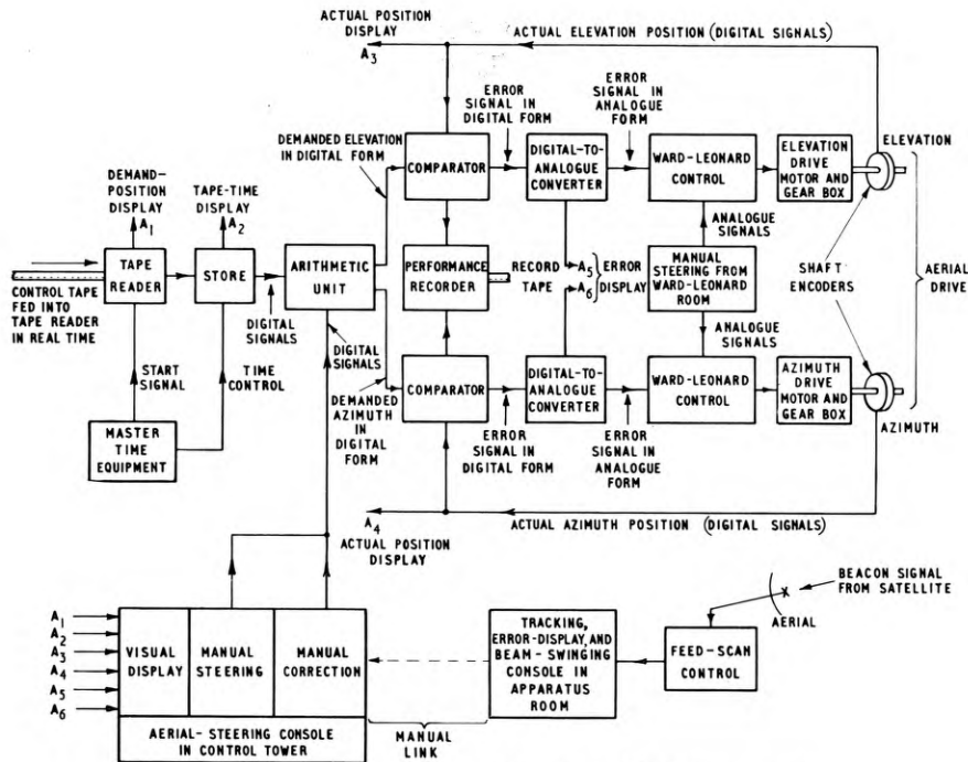
FIG. 3—SIMPLIFIED BLGCK-SCHEMATIC DIAGRAM OF THE AERIAL-STEERING SYSTEM
