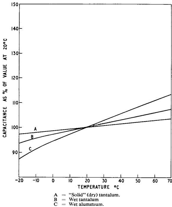
FIG. 7—CHANGE OF CAPACITANCE WITH TEMPERATURE
