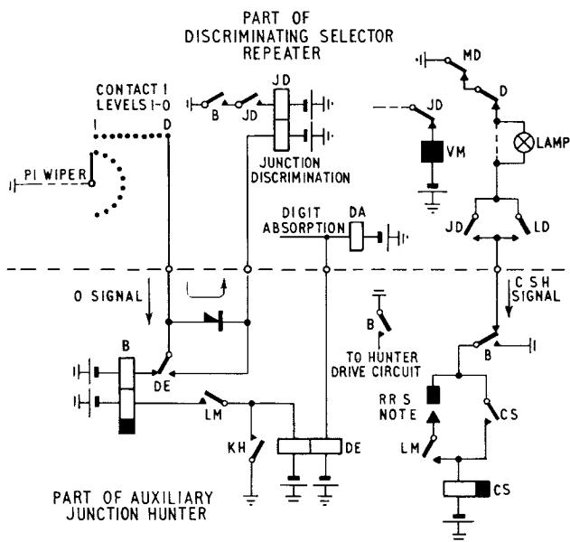
FIG. 2.—METHOD OF OBTAINING LEVEL 0 DISCRIMINATION AND CALLED-SUBSCRIBER-HELD SIGNAL FROM D.S.R.
