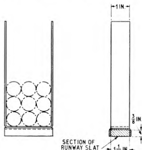
FIG. 2—SKETCH OF CABLE CLIP
