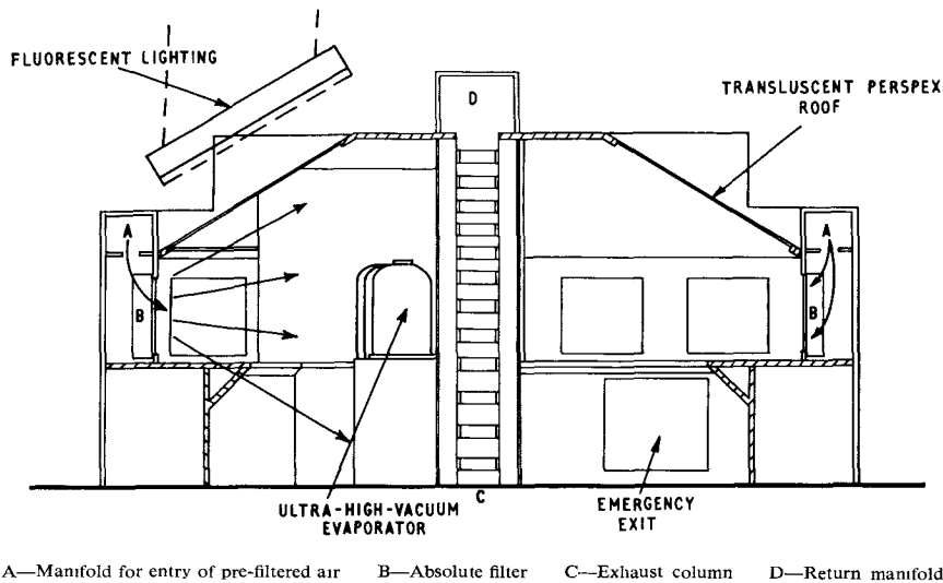
FIG. 6—CROSS-SECTION OF CLEAN ROOM
