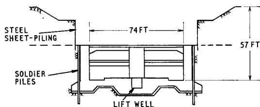
FIG. 2—CROSS-SECTION OF STATION EXCAVATION NORTH-SOUTH
