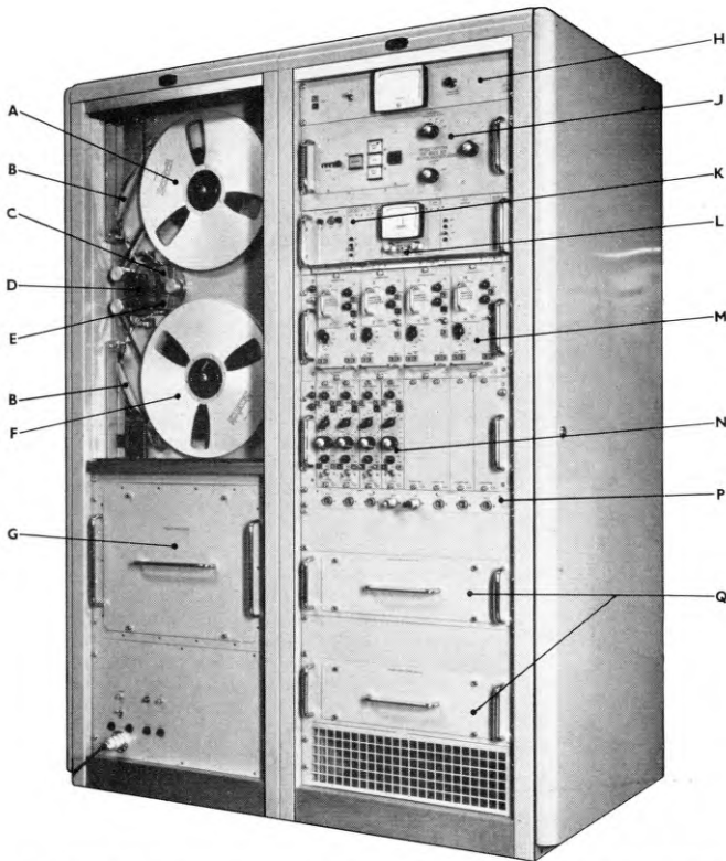
A—Feed spool B—Tape sensing arms C—Recording heads D—Capstan E—Replaying heads F—Take-up spool G—Speed-lock power amplifier H—A.C./D.C. testmeter J—Tape-deck control unit K—Speed-lock replay unit L—Speed-lock control unit M—Four f.m. replay units N—Four f.m. record units P—Input and output sockets Q—Power-supply units
