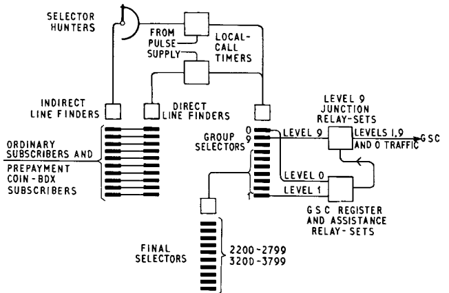
FIG. 3—SIMPLIFIED DIAGRAM OF U.A.X. No. 14 (1,200-LINE MULTIPLE S.T.D. TRUNKING ARRANGEMENTS WITH DIGIT-ABSORPTION ON 1st GROUP SELECTORS)
