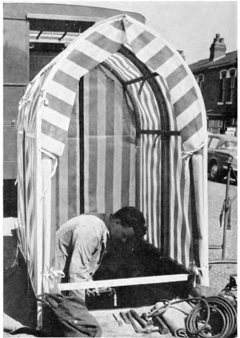
(b) Jointers' Tent No. 3
