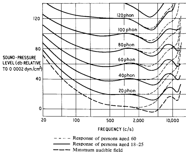
FIG. 8—EQUAL-LOUDNESS CONTOURS
