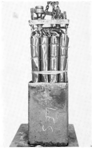
FIG. 5—TYPICAL CASE WITH COIL ASSEMBLY BEING REMOVED
