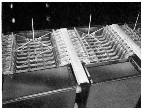
FIG. 2—EBONITE BOX (CAPACITY 2,600 Ah PLATED TO 1,800 Ah)
