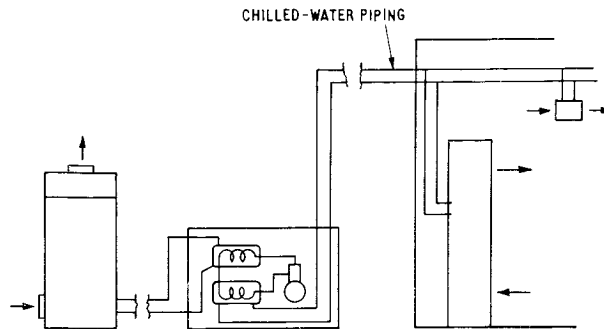
(b) Remote Water-Chiller with Cooling Tower serving Fan-Coil Units
