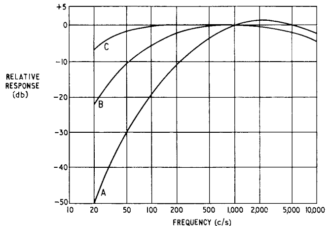
The curves A, B and C are plotted from figures given in B.S.3489 : 1962. FIG. 9—WEIGHTING CURVES FOR SOUND-LEVEL METERS
