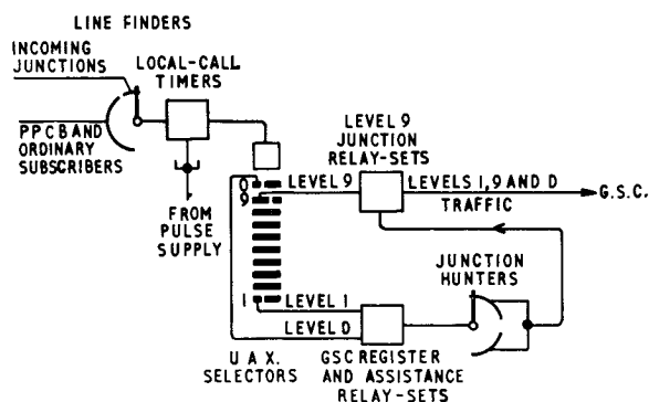
P.P.C.B.—Prepayment coin-box
