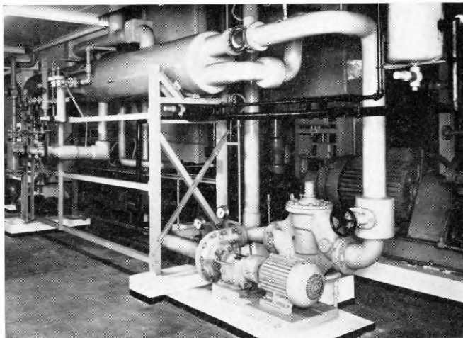
FIG. 3.—SHELL-AND-TUBE WATER CHILLER (EVAPORATER) AND CIRCULATING PUMP
