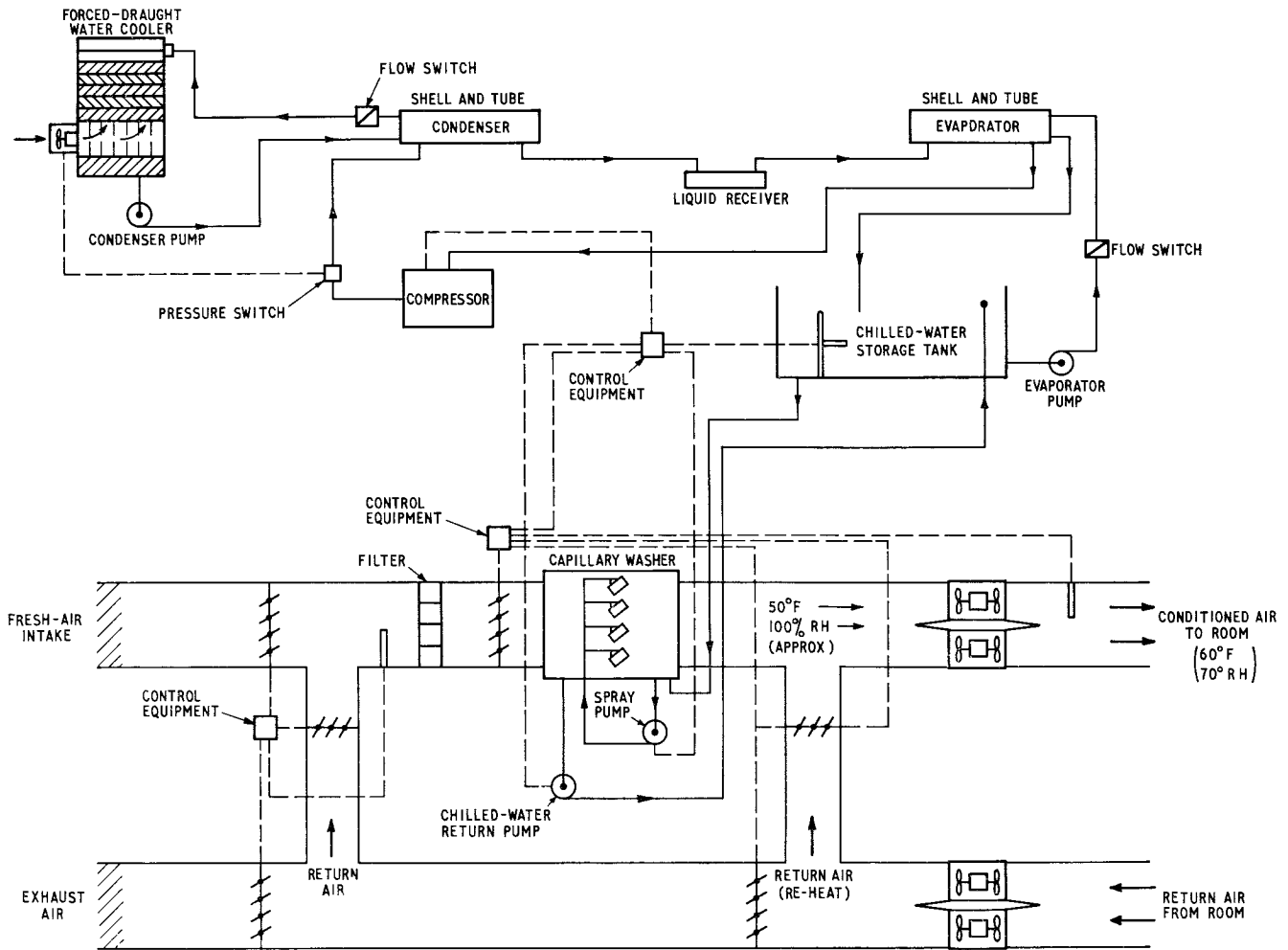
FIG. 4—SIMPLIFIED DIAGRAM OF 70-TON AIR-CONDITIONING SYSTEM
