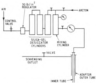
FIG. 9—SCHEMATIC DIAGRAM OF PRESSURE-TESTING ARRANGEMENTS
