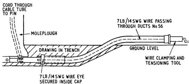
LAYING PLASTIC DUCT BY MOLEPLOUGH
