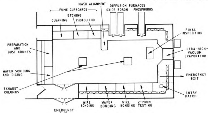
FIG. 2—DETAILED PLAN OF CLEAN AREA
