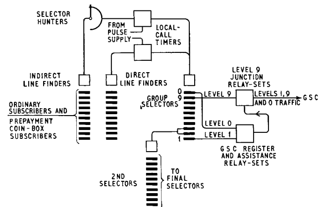
FIG. 4—SIMPLIFIED DIAGRAM OF S.T.D. ARRANGEMENTS AT U.A.X. No. 14 (2,000-LINE MULTIPLE) WITHOUT DIGIT ABSORPTION
