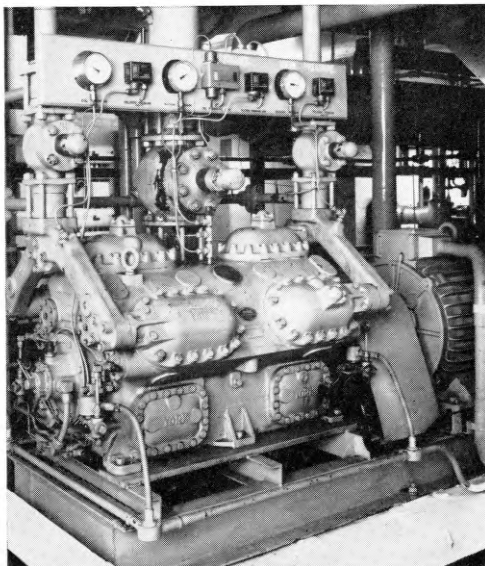
FIG. 2.—TWELVE-CYLINDER SINGLE-STAGE COMPRESSOR
