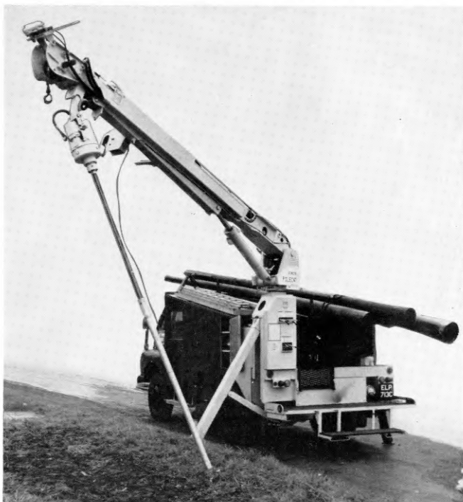
FIG. 2—ADAPTOR FITTED TO DRIVE-SHAFT OF POLE-ERECTION UNIT
