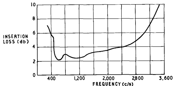
(a) Insertion Loss/Frequency Characteristic
