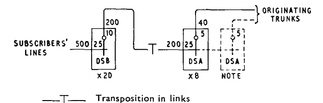
FIG. 5—500-LINE DISTRIBUTOR STAGE OF 5005 SYSTEM
