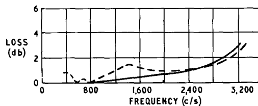
--- Carrier channel — 20 miles of 20 lb/mile cable with standard loading FIG. 1—LOSS/FREQUENCY CHARACTERISTICS OF A TYPICAL CARRIER CHANNEL AND OF 20 MILES OF AUDIO CABLE PAIR WITH STANDARD LOADING
