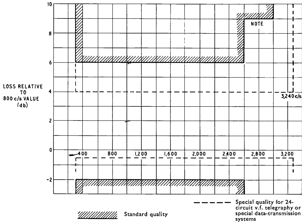
FIG. 13—LIMITS FOR LOSS/FREQUENCY CHARACTERISTICS OF PRIVATE CIRCUITS USED FOR NON-SPEECH APPLICATIONS
