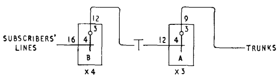
(b) Conventional Method of Showing Link-Trunking Principle. FIG. 4—LINK TRUNKING
