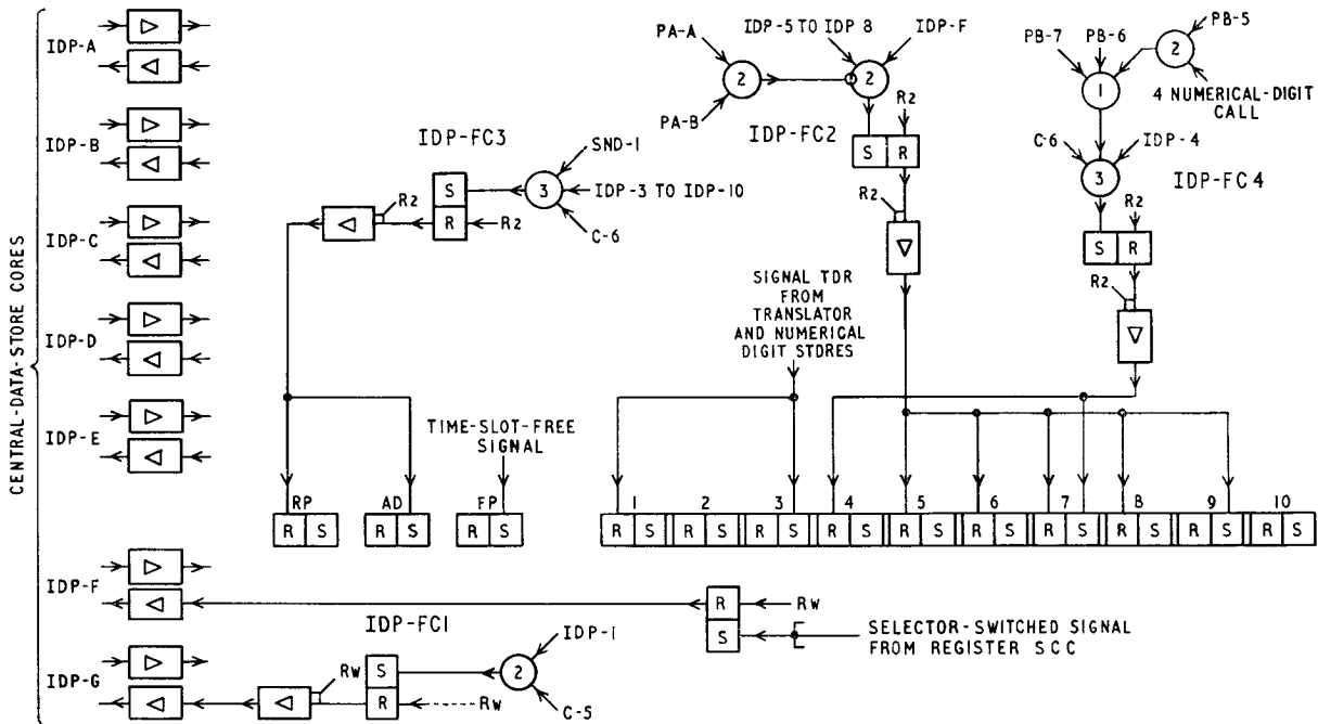
FIG. 27—FUNCTIONAL CIRCUIT OF INTER-DIGITAL-PAUSE COUNTER
