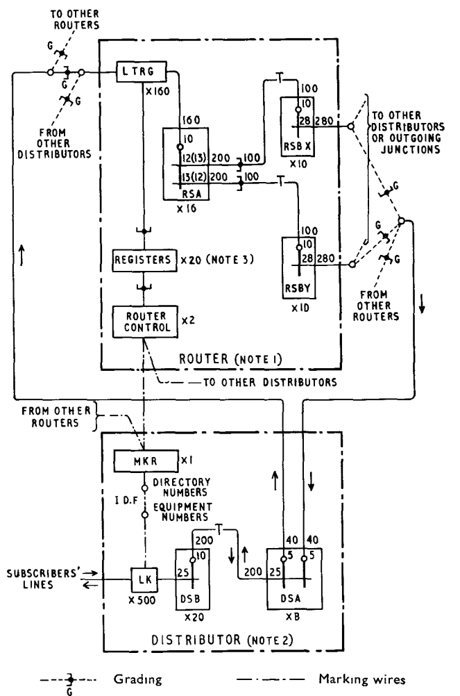
FIG. 6—TRUNKING SCHEME FOR 5005 EXCHANGE OF 500-10,000 LINES SHOWING ROUTERS AND DISTRIBUTORS
