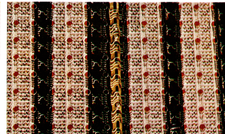
(BOTTOM RIGHT) Frame assembly illustrating the wiring gutters used to accommodate the tape wiring.
