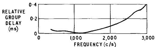
b) Relative Group-Delay/Frequency Characteristic of 15-Mile Junction Consisting Wholly of Loaded Cable
