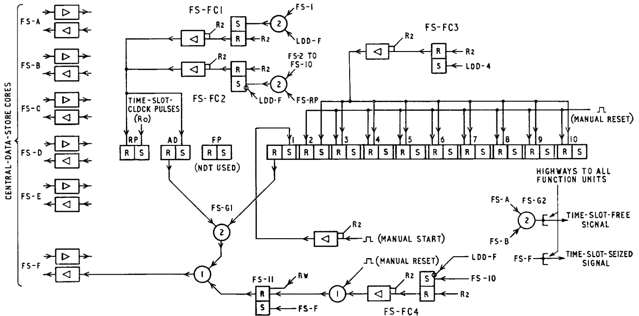
FIG. 18—FUNCTIONAL CIRCUIT OF TIME-SLOT-FREE/TIME-SLOT-SEIZED CONTROL
