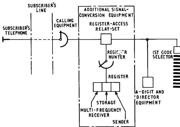
FIG. 2—BASIC TRUNKING
