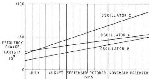
(b) Typical Frequency-Drift Curves
