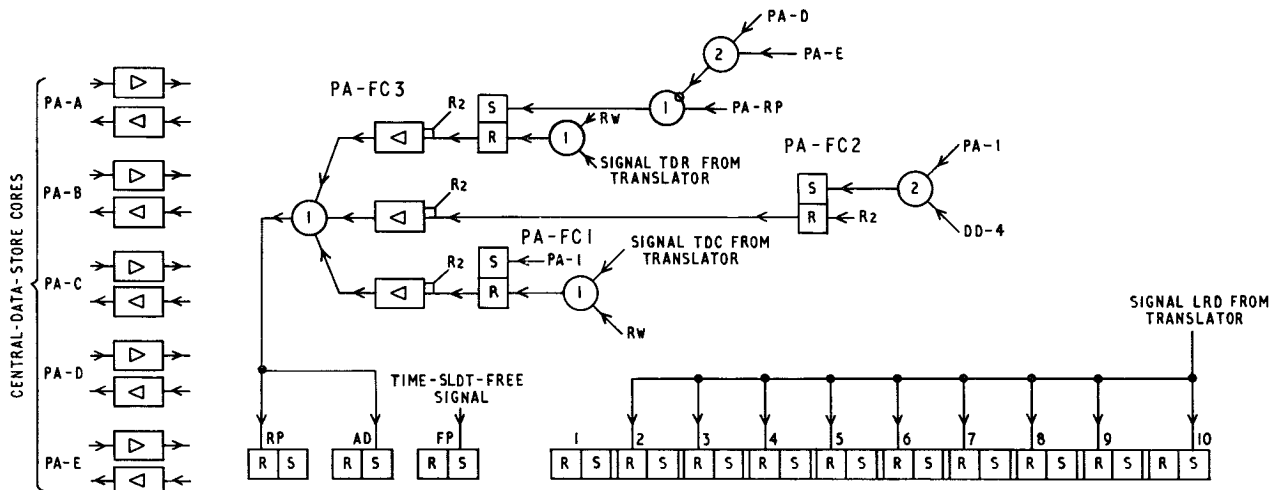
FIG. 28—FUNCTIONAL CIRCUIT OF PROGRAM SWITCH A
