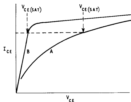
Curve A—Characteristic for a typical mesa transistor with large value of V_{CE(SAT)} Curve B—Characteristic for a typical epitaxial mesa transistor with a smaller value of V_{CE(SAT)}
