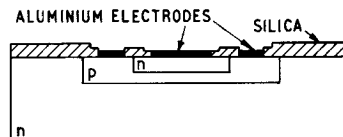
FIG. 4—CROSS-SECTION OF A SILICON PLANAR TRANSISTOR
