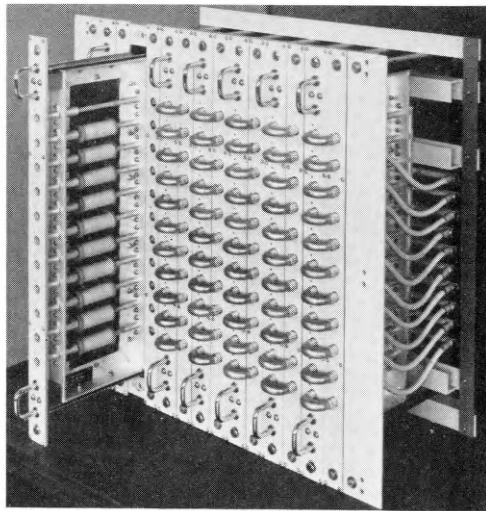
FIG. 3—THE 11 \times 7 COAXIAL MATRIX
