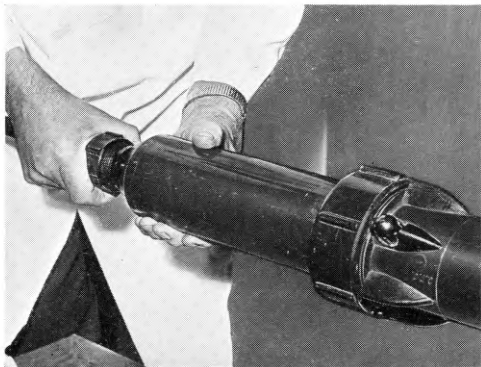
FIG. 3—POLYTHENE SCREW-JOINT
