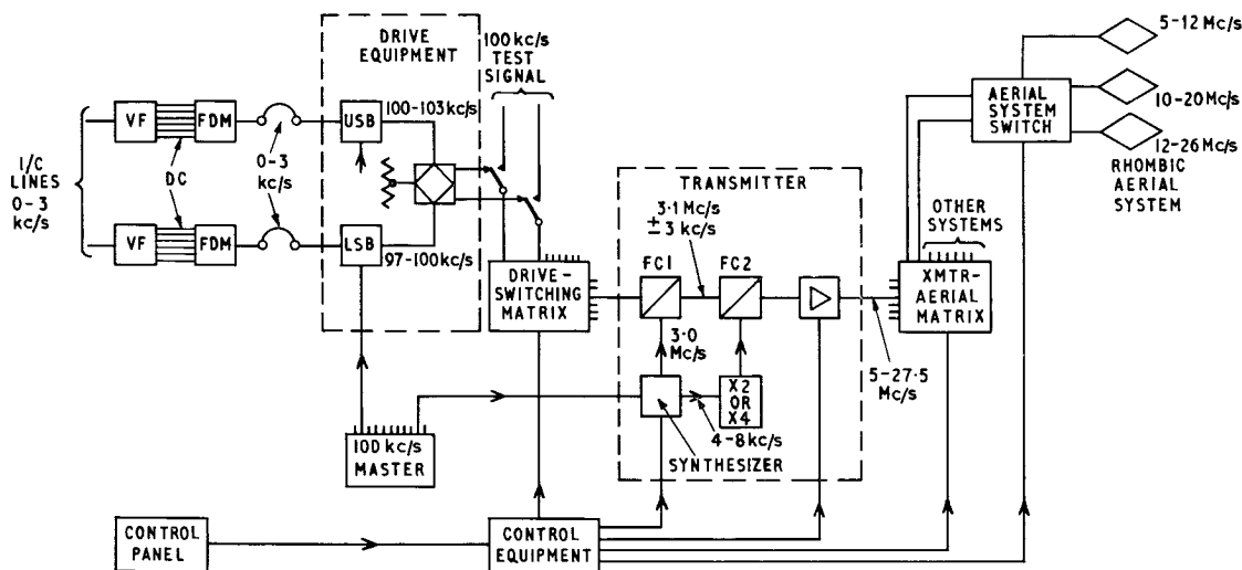
FIG 1 SIMPLIFIED ARRANGEMENT OF CONNEXIONS BETWEEN LINES AND AERIALS
