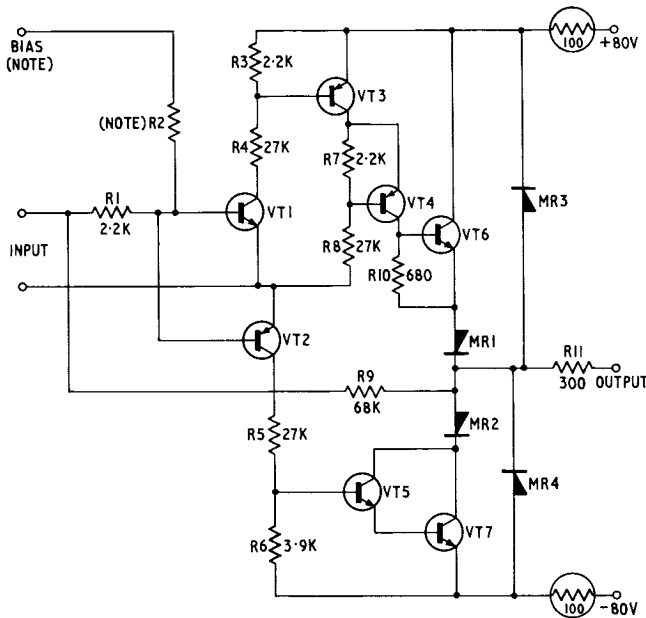
CIRCUIT DIAGRAM OF SEMICONDUCTOR-TYPE RELAY
