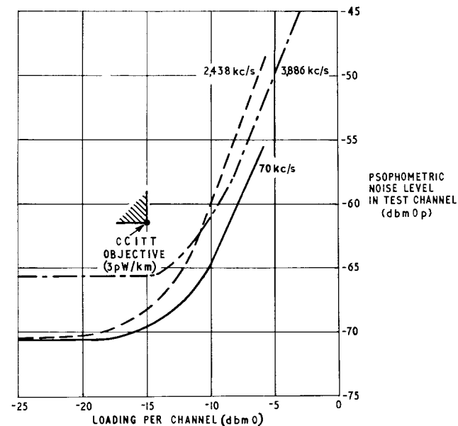
FIG. 9—VARIATION IN NOISE PERFORMANCE WITH TRAFFIC LOADING OF CHANNELS ON COAXIAL-CABLE SYSTEM 150 MILES LONG
