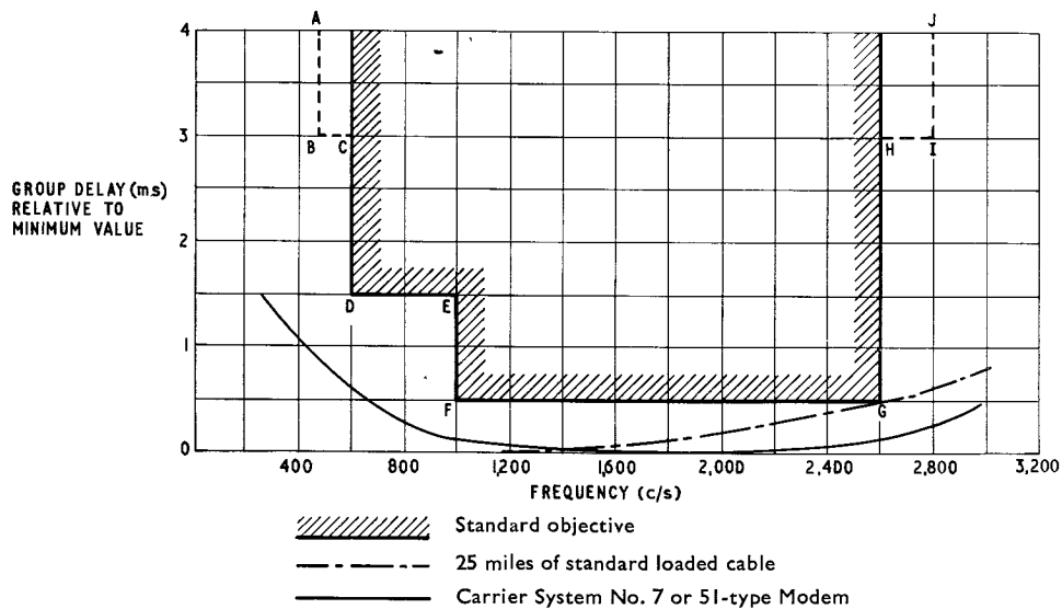
FIG. 14—BRITISH POST OFFICE OBJECTIVE FOR GROUP-DELAY/FREQUENCY CHARACTERISTICS OF PRIVATE CIRCUITS FOR NON-SPEECH APPLICATIONS
