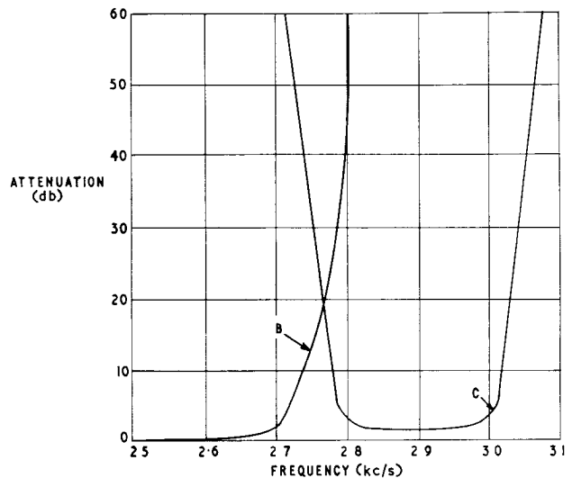
B—Compressed-speech path low-pass filter characteristic. C—Control-channel band-pass filter characteristic. The characteristics B and C relate to the filters designated B and C in Fig. 1.
