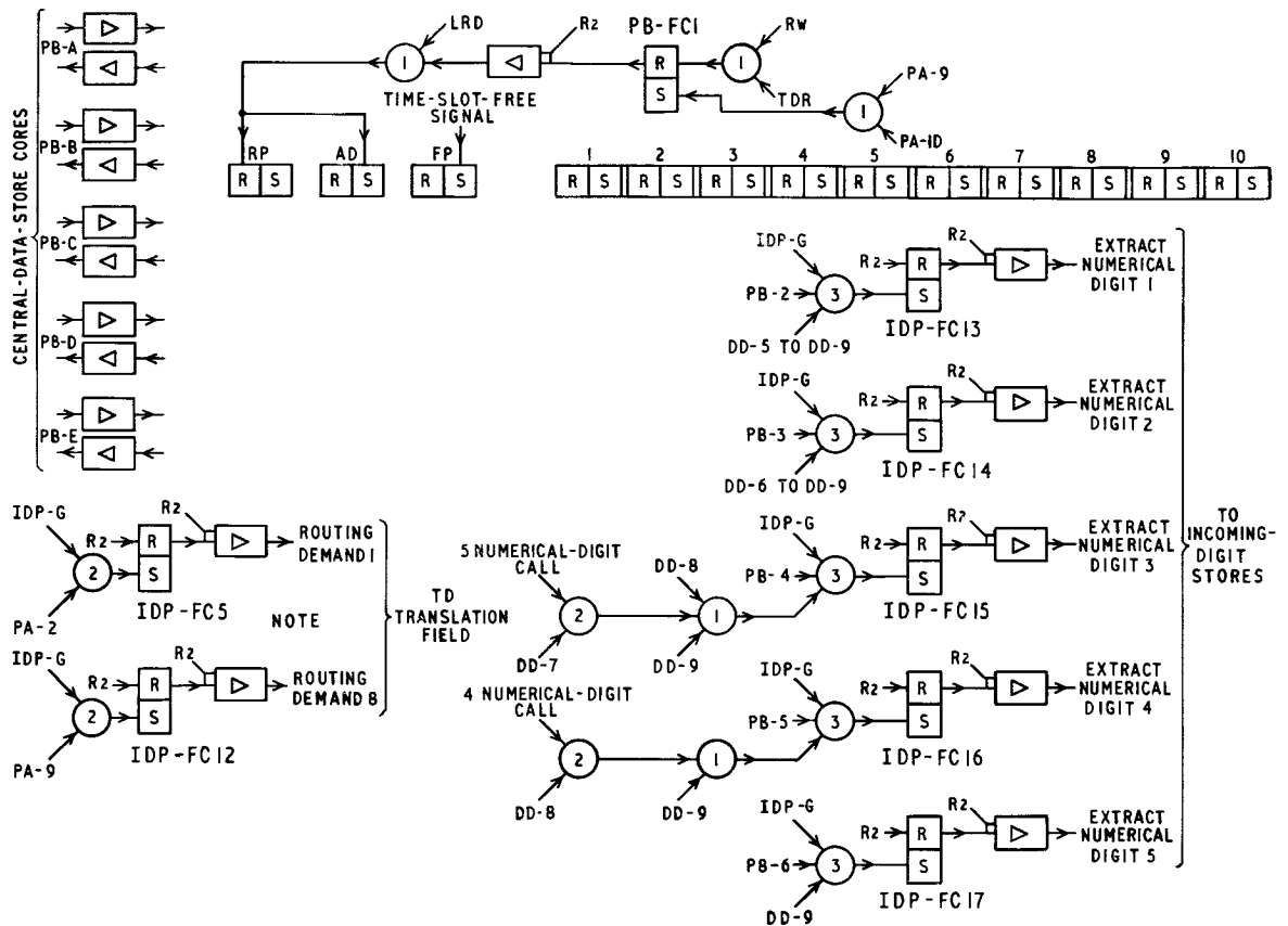
Note: Function control elements IDP-FC6 to IDP-FC11 are similarly connected, using signals PA-3 to PA-8, to produce routing demands 2 to 7, respectively.
