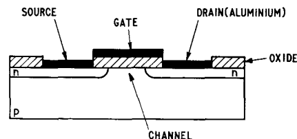
FIG. 5—CROSS-SECTION OF AN INSULATED-GATE FIELD-EFFECT TRANSISTOR (A M.O.S.T.)
