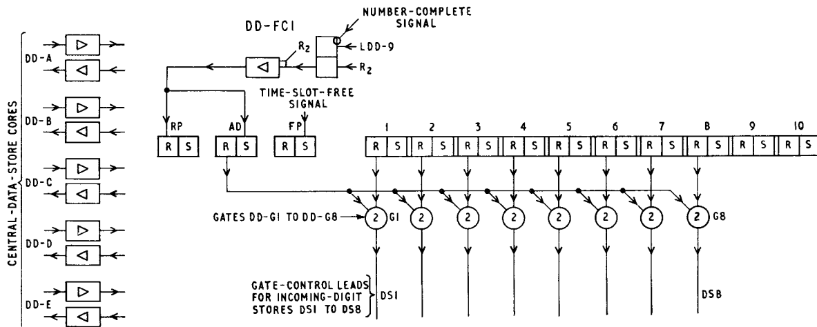
FIG 21—FUNCTIONAL CIRCUIT OF INCOMING-DIGITS DISTRIBUTOR
