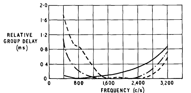
— 20 miles of 20 lb/mile cable with standard loading --- Carrier channel (Frequency-Translating Equipment No. 1A or No. 11A) - - - Carrier channel (Frequency-Translating Equipment No. 80A) FIG. 2—GROUP-DELAY/FREQUENCY CHARACTERISTICS OF TYPICAL CARRIER CHANNELS AND OF 20 MILES OF AUDIO CABLE PAIR WITH STANDARD LOADING
