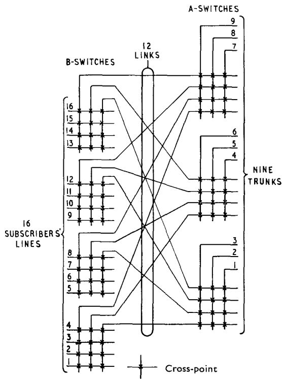
(a) Principle of Link Trunking.
