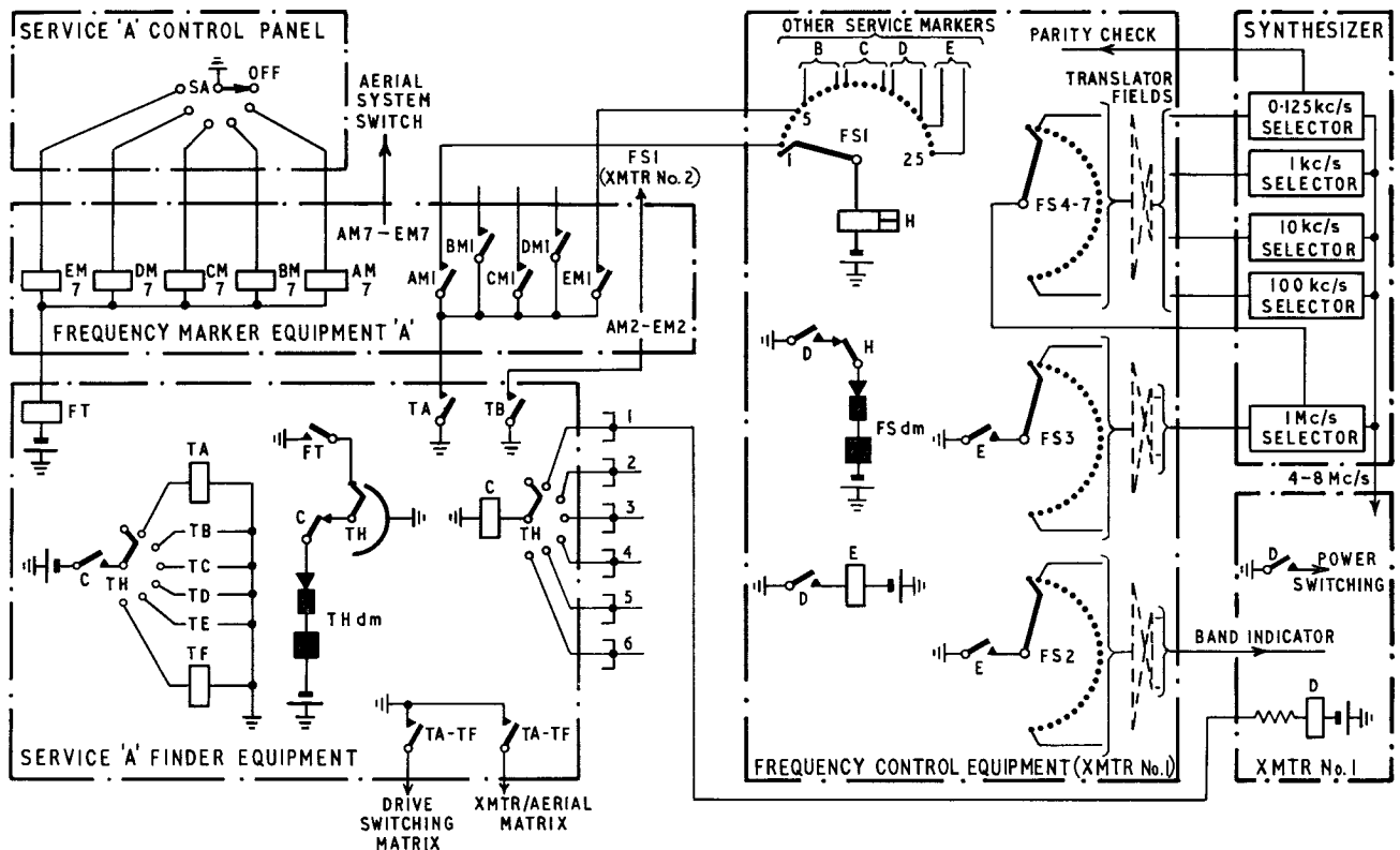
FIG. 2—CONTROL CIRCUIT
