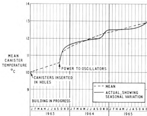
(a) Mean Temperature inside the Canisters
