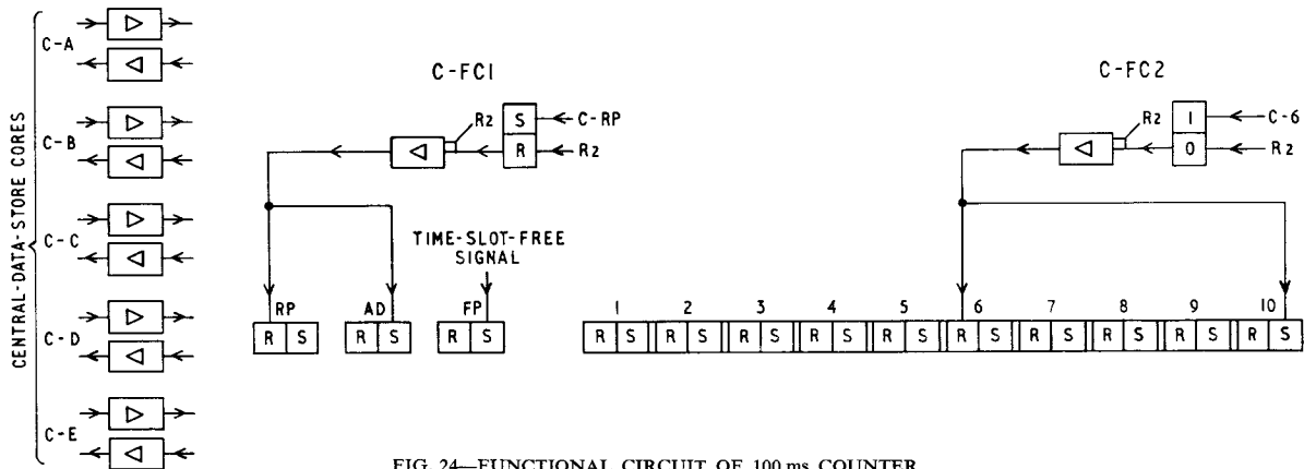
FIG. 24—FUNCTIONAL CIRCUIT OF 100 ms COUNTER
