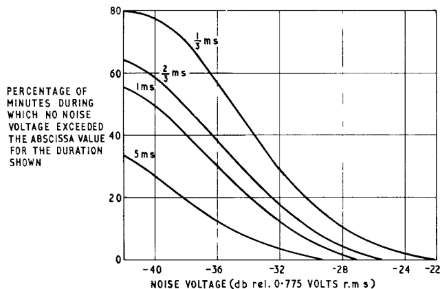
FIG. 10—MEASURED NOISE VOLTAGES ON AUTOMATIC-EXCHANGE CONNEXIONS (2,000-TYPE AND PRE-2,000-TYPE DIRECTOR EXCHANGES)
