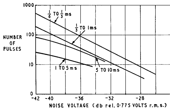
FIG. 11—TOTAL NUMBER OF SHORT PULSES DURING WHICH GIVEN VALUE OF NOISE VOLTAGE WAS EXCEEDED FOR THE DURATION GIVEN
