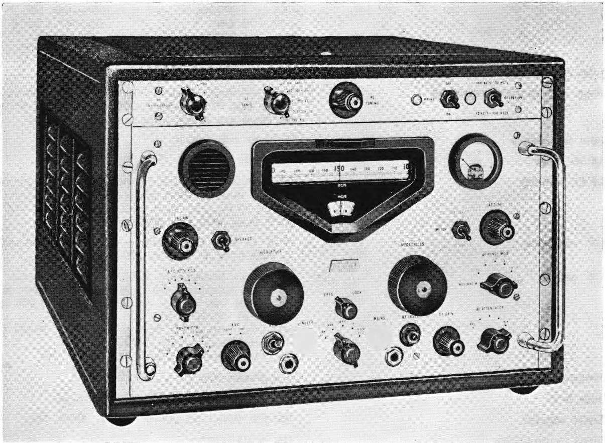
Receiver, radio, 5820-99-999-9292
