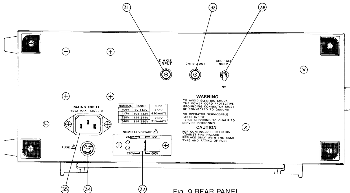
Fig. 9 REAR PANEL
