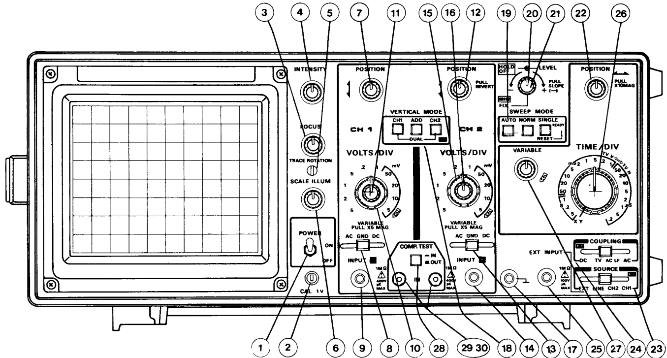
Fig. 8 FRONT PANEL
