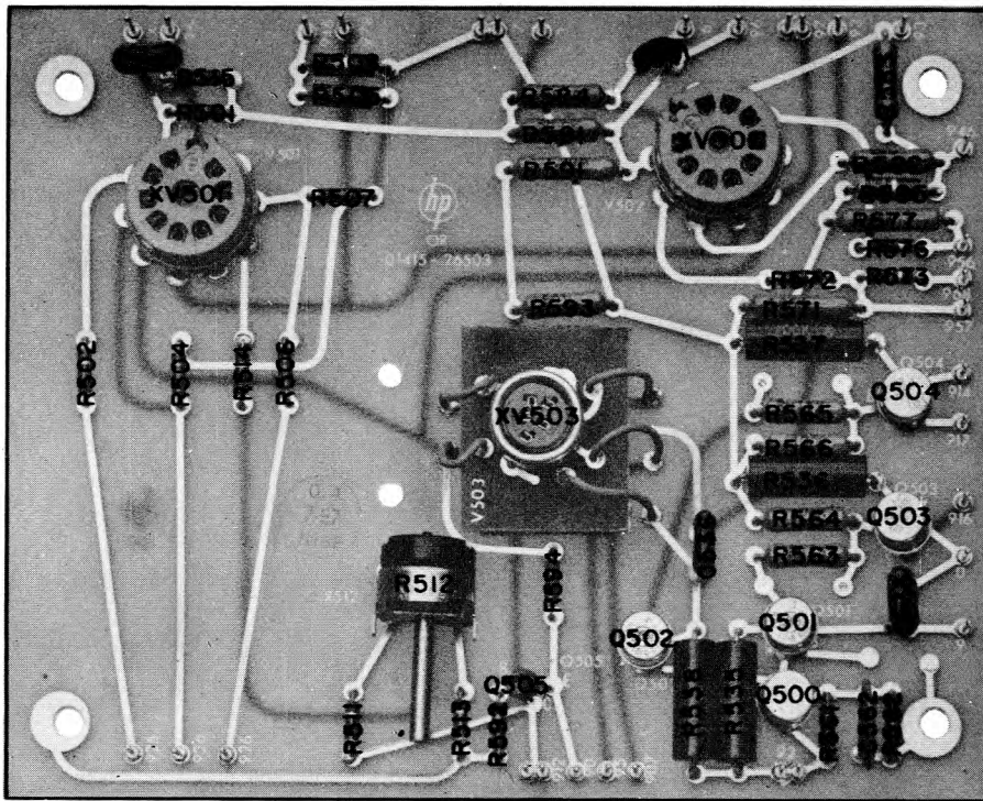
Figure IIA-4. Amplifier Board A5
