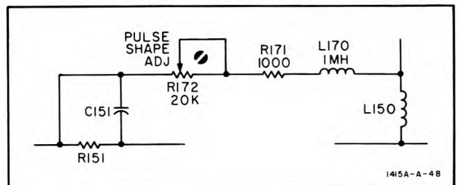
Figure IIA-9. Pulse Shape Adjust Circuit
