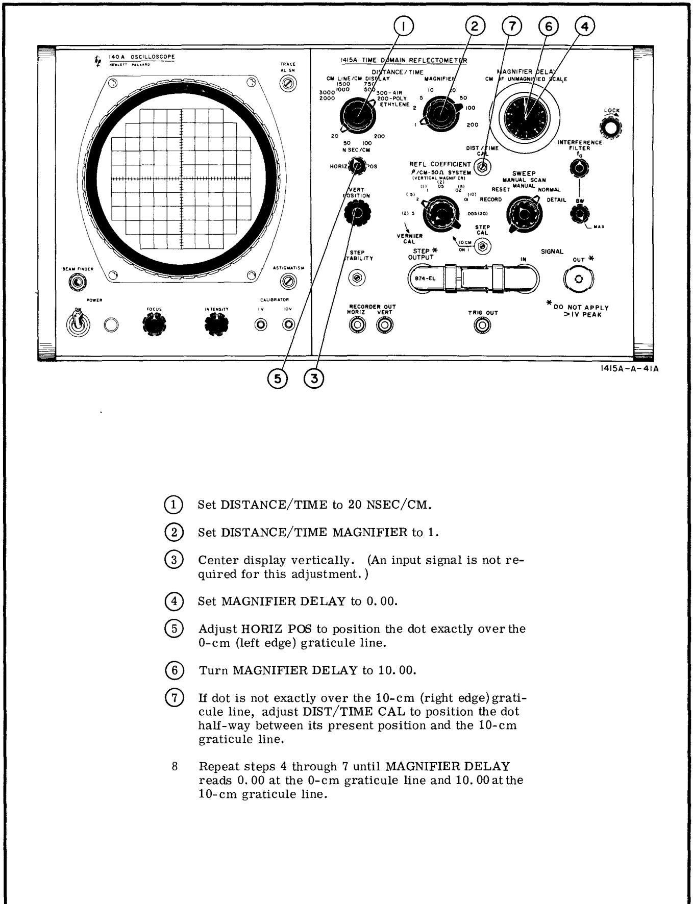
Figure 3-4. Horizontal Calibration
