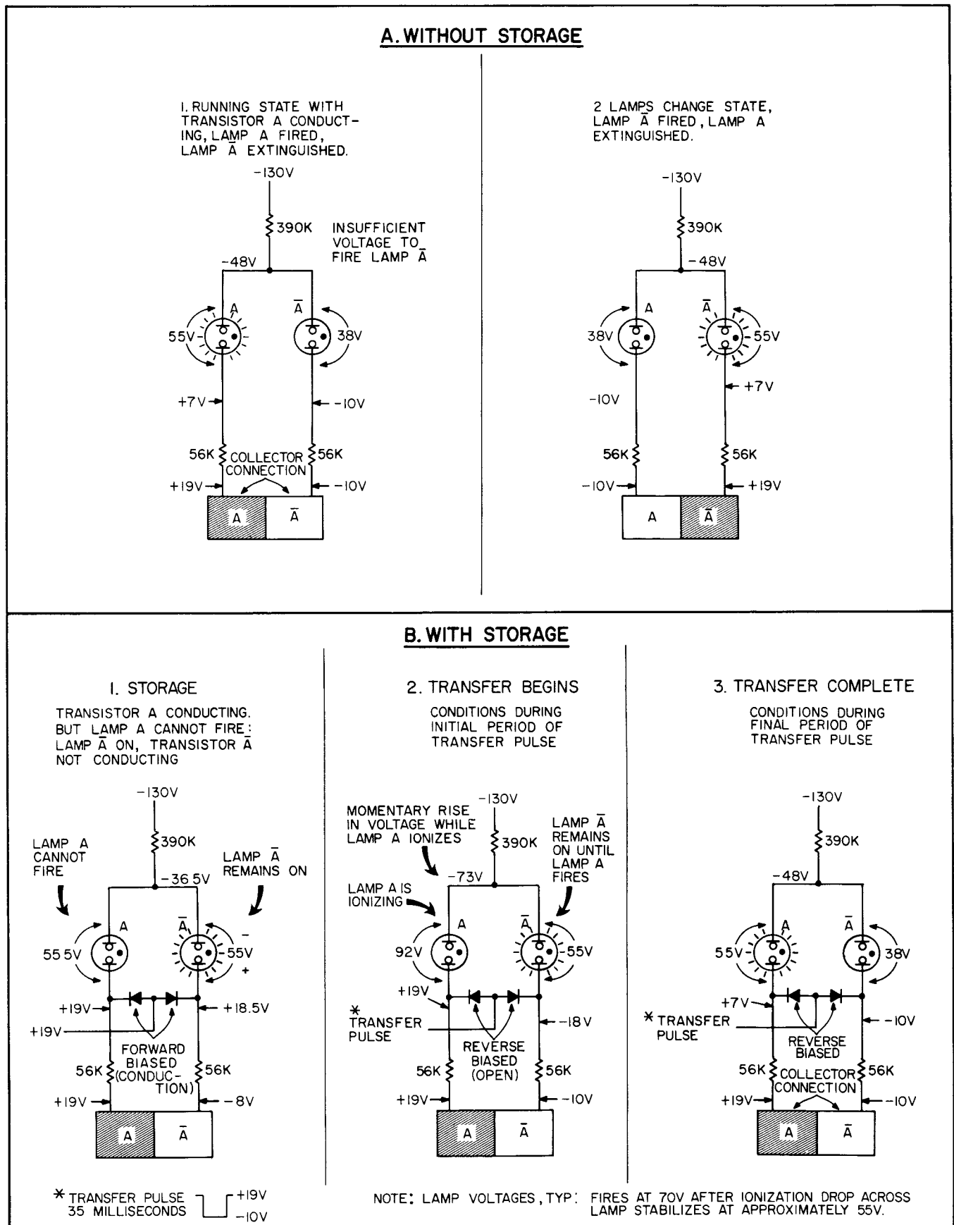
Figure 2-8. Lamp Control
