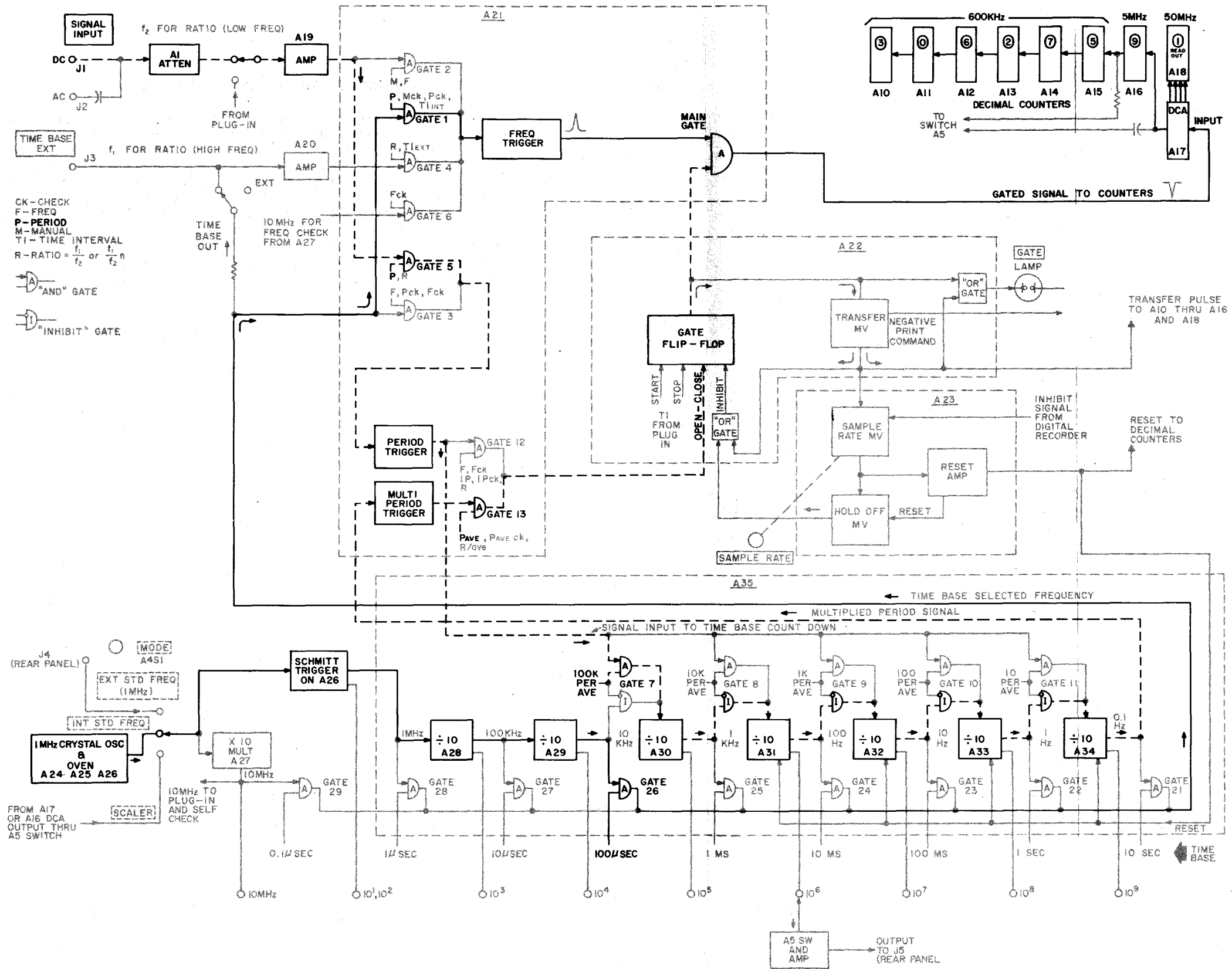
Figure 6-9. Multiple Period Average Measurements
