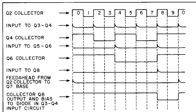
WAVEFORMS
