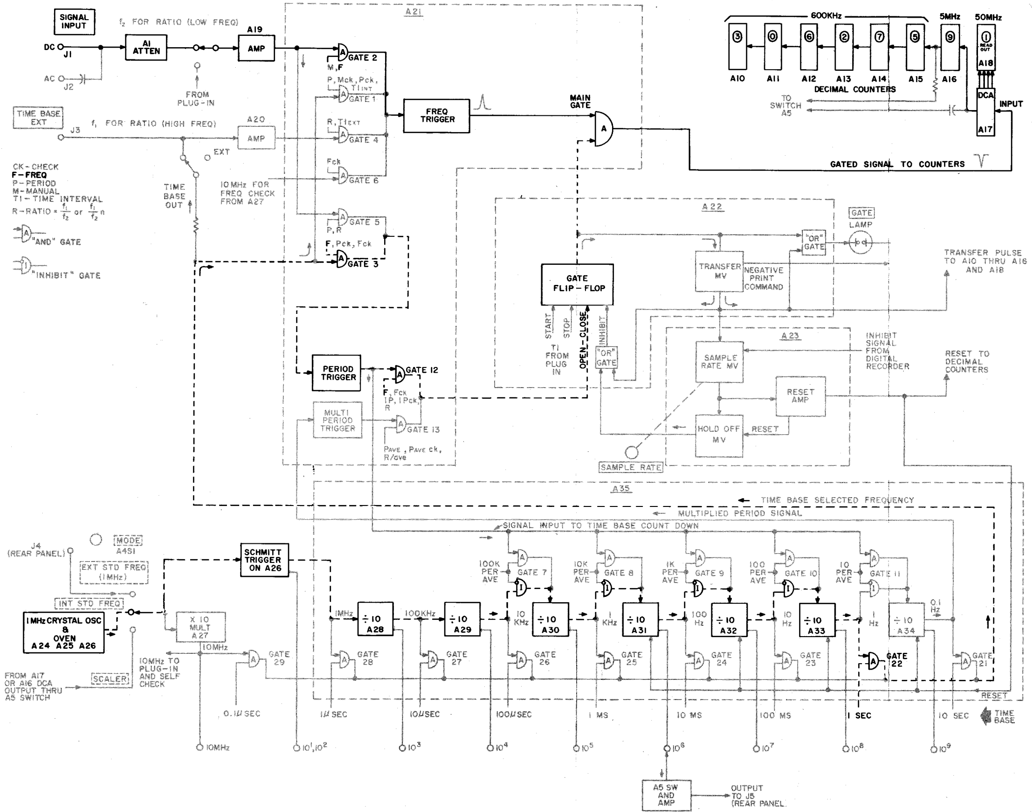
Figure 6-7. Frequency Measurements
