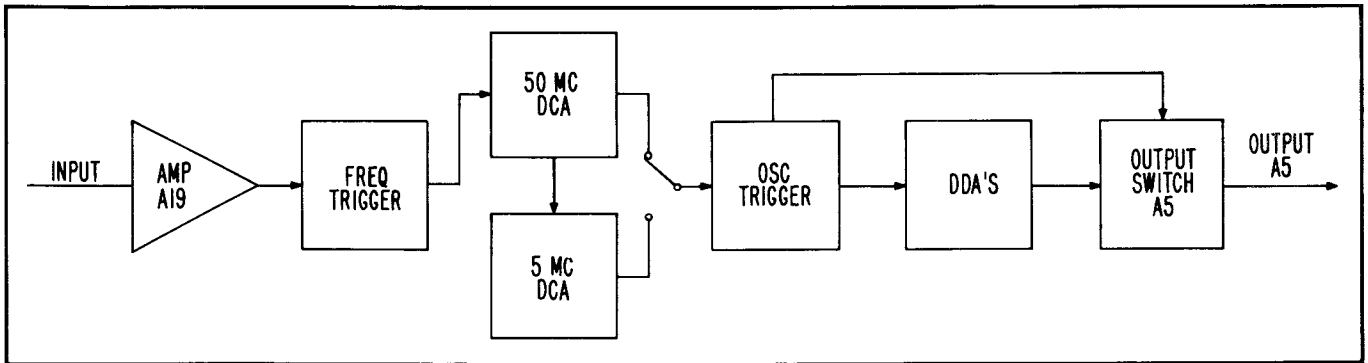
Figure 2-11. Scaler Operation
