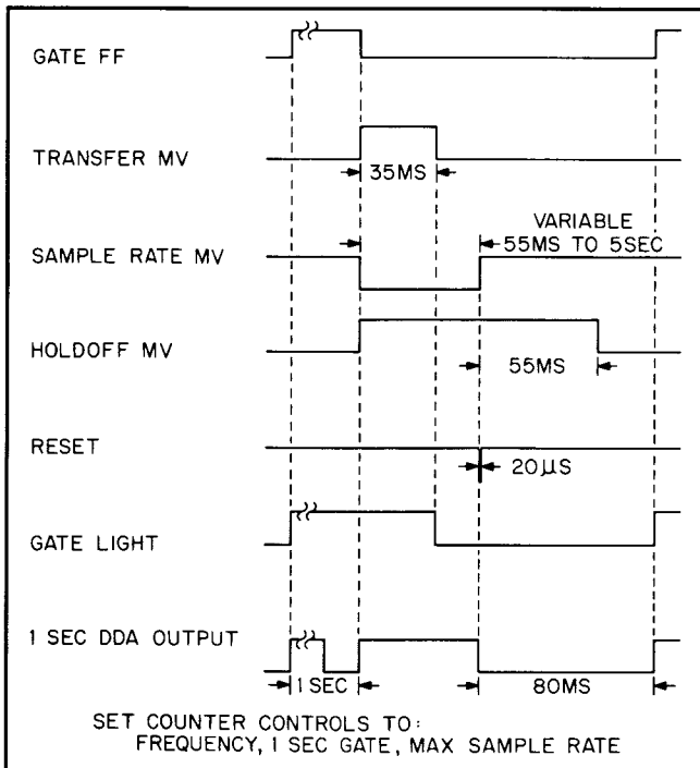
Figure 2-12. Time Sequence
