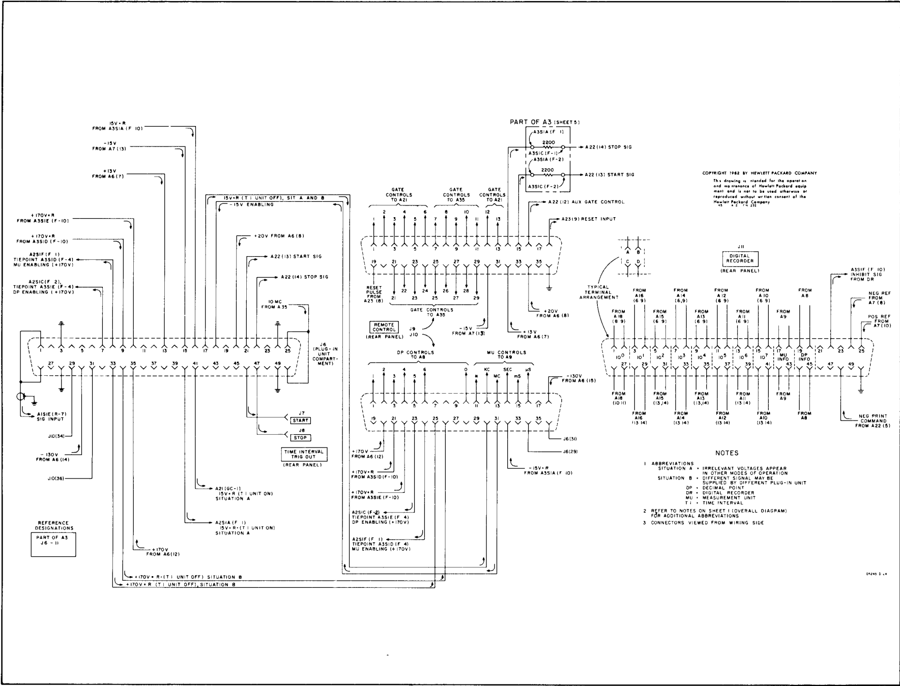
Figure 5-3. Remote Control Wiring and Connectors (Special)
