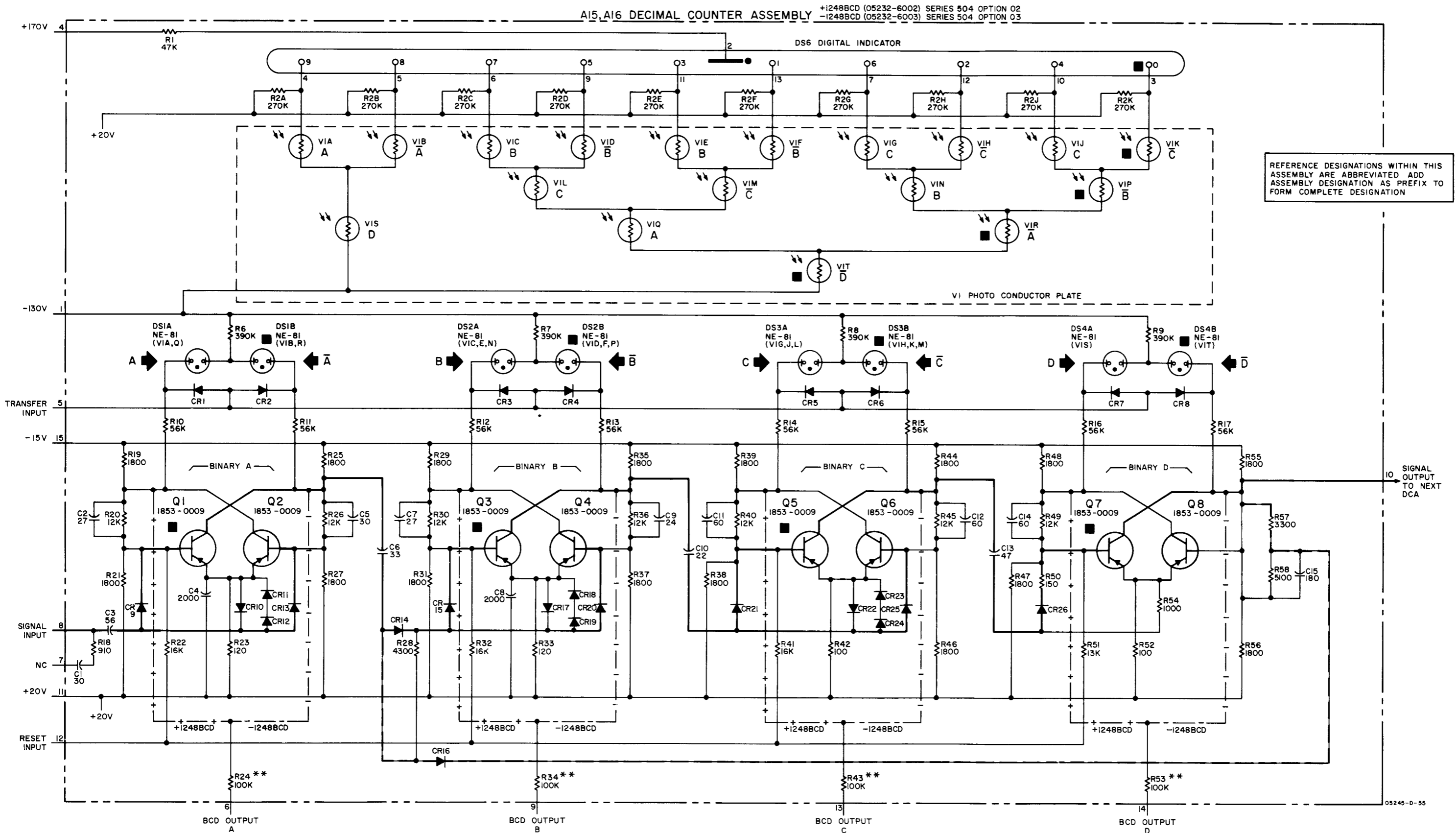
Figure 7-28. A15, A16 Decimal Counter (05232-6002, 6003) Option 02, 03
