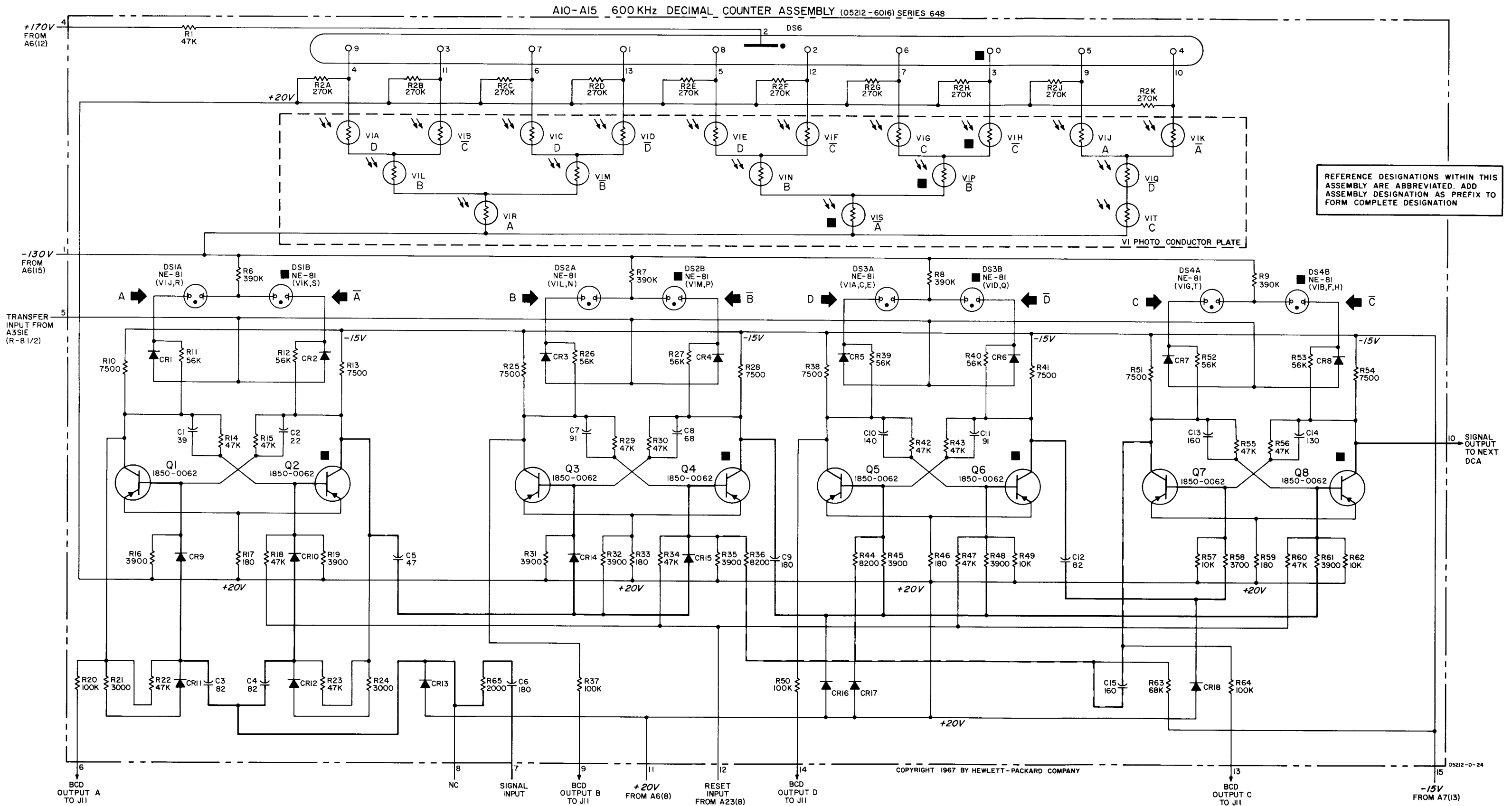
Figure 7-9. A10-A15 Decimal Counter (05212-6016)
