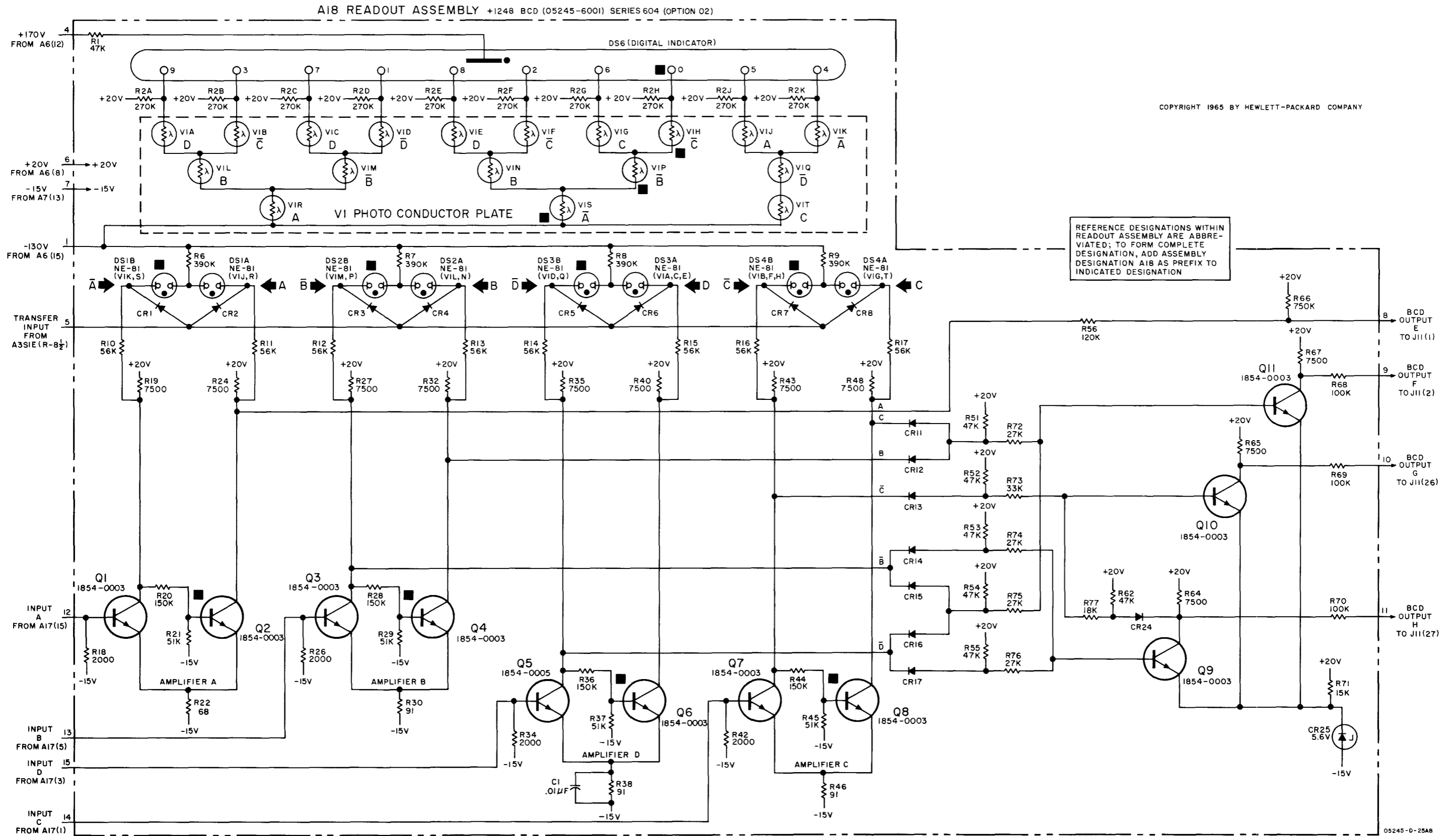
Figure 7-15. A18 Readout (05245-6001) Option 02
