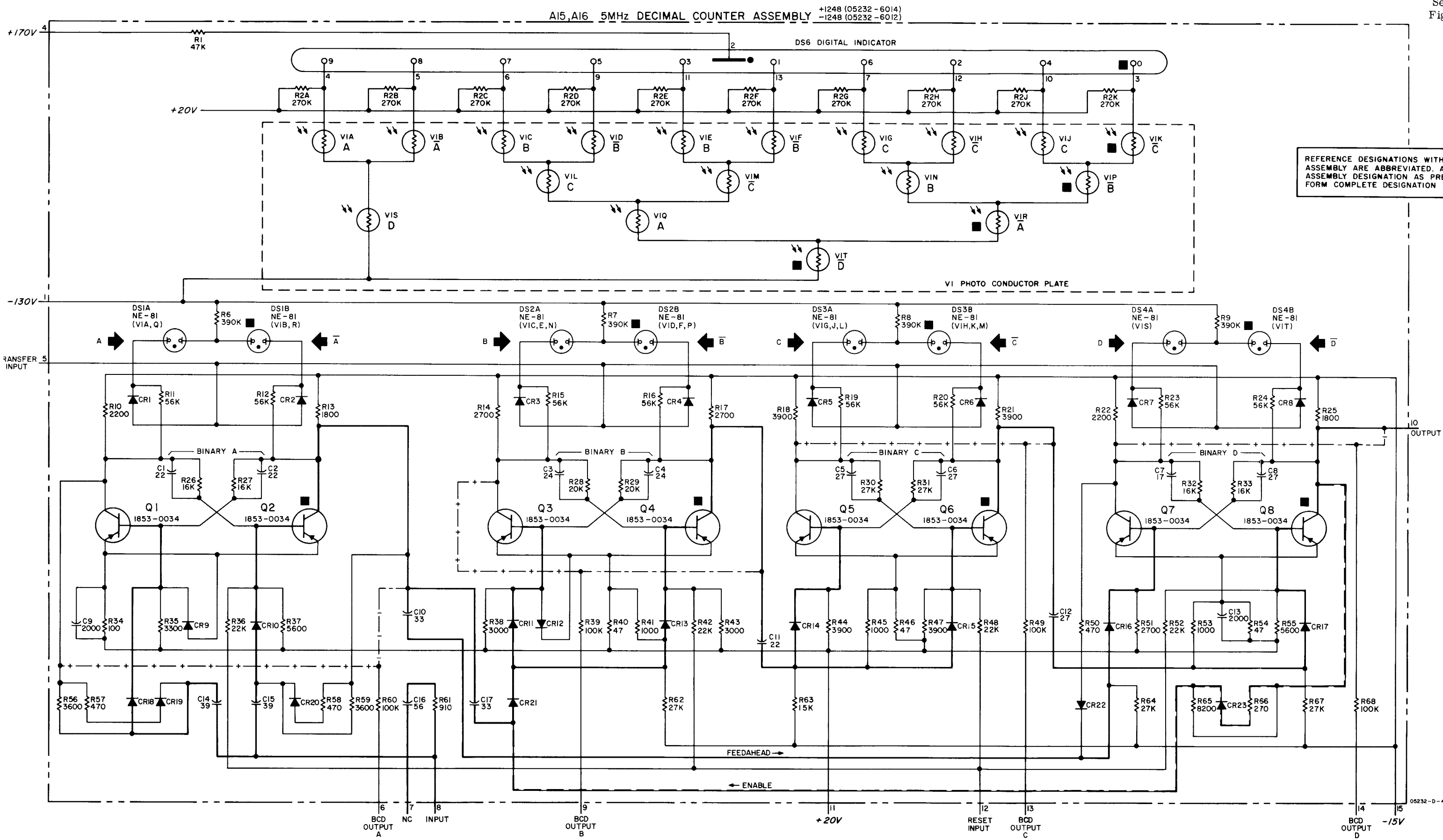
Figure 7-12. A15, A16 Decimal Counter (05232-6014, 6012) Option 02, 03
