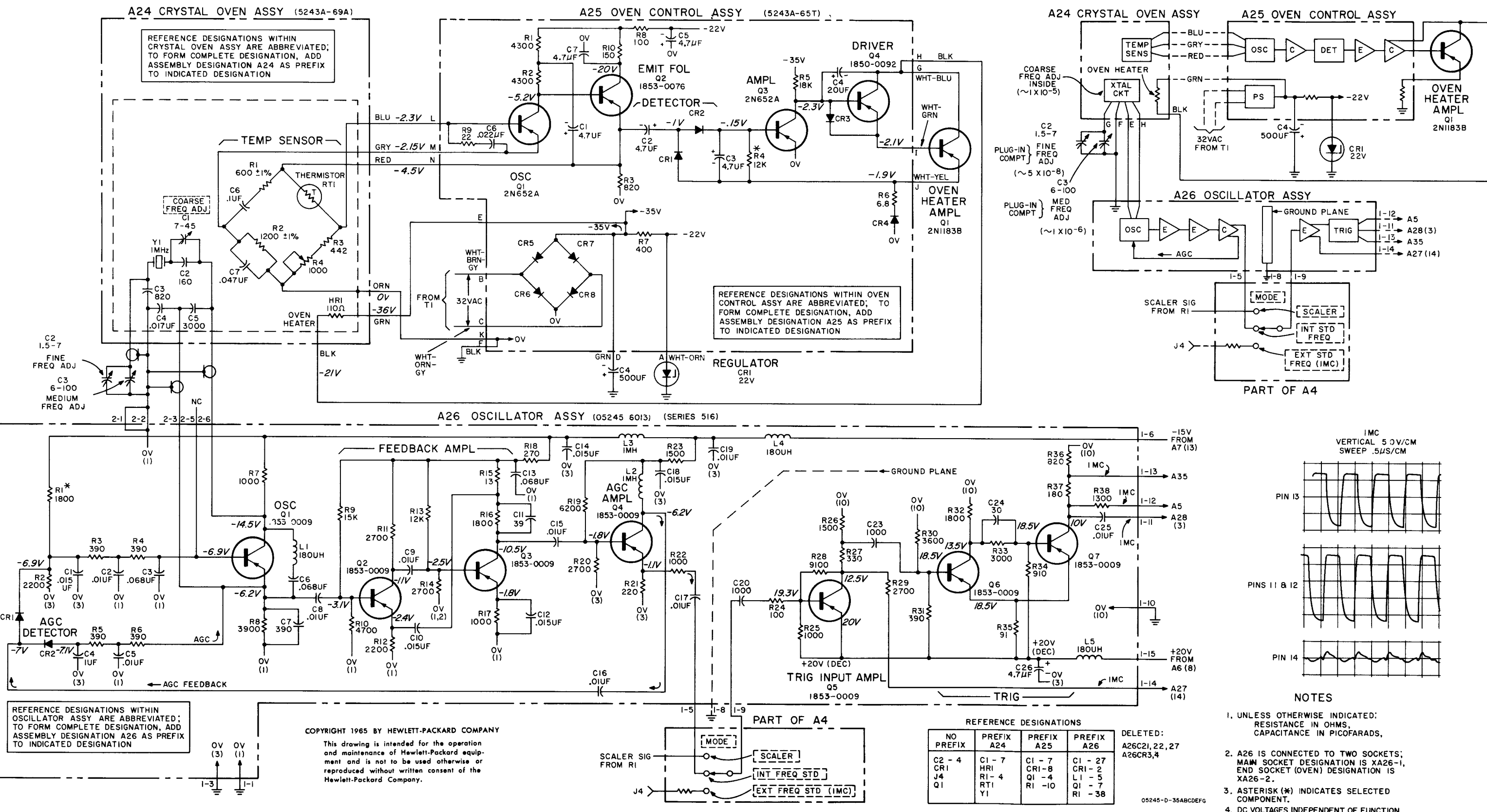
Figure 7-21. A24, A25, A26 Crystal Oven, Oven Control, Oscillator
