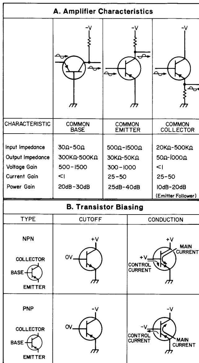
Figure 2-2. Transistor Operation
