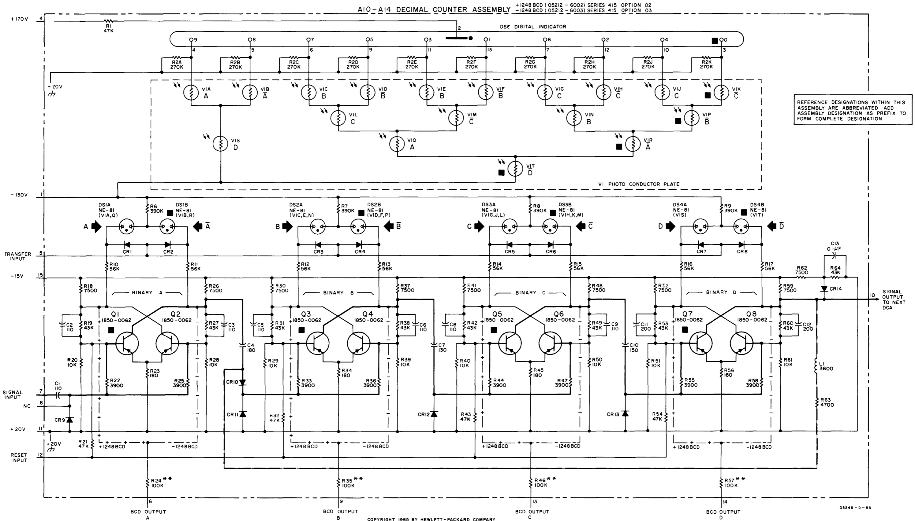
Figure 7-10. A10-A14 Decimal Counter (05212-6002, 6003) Option 02, 03
