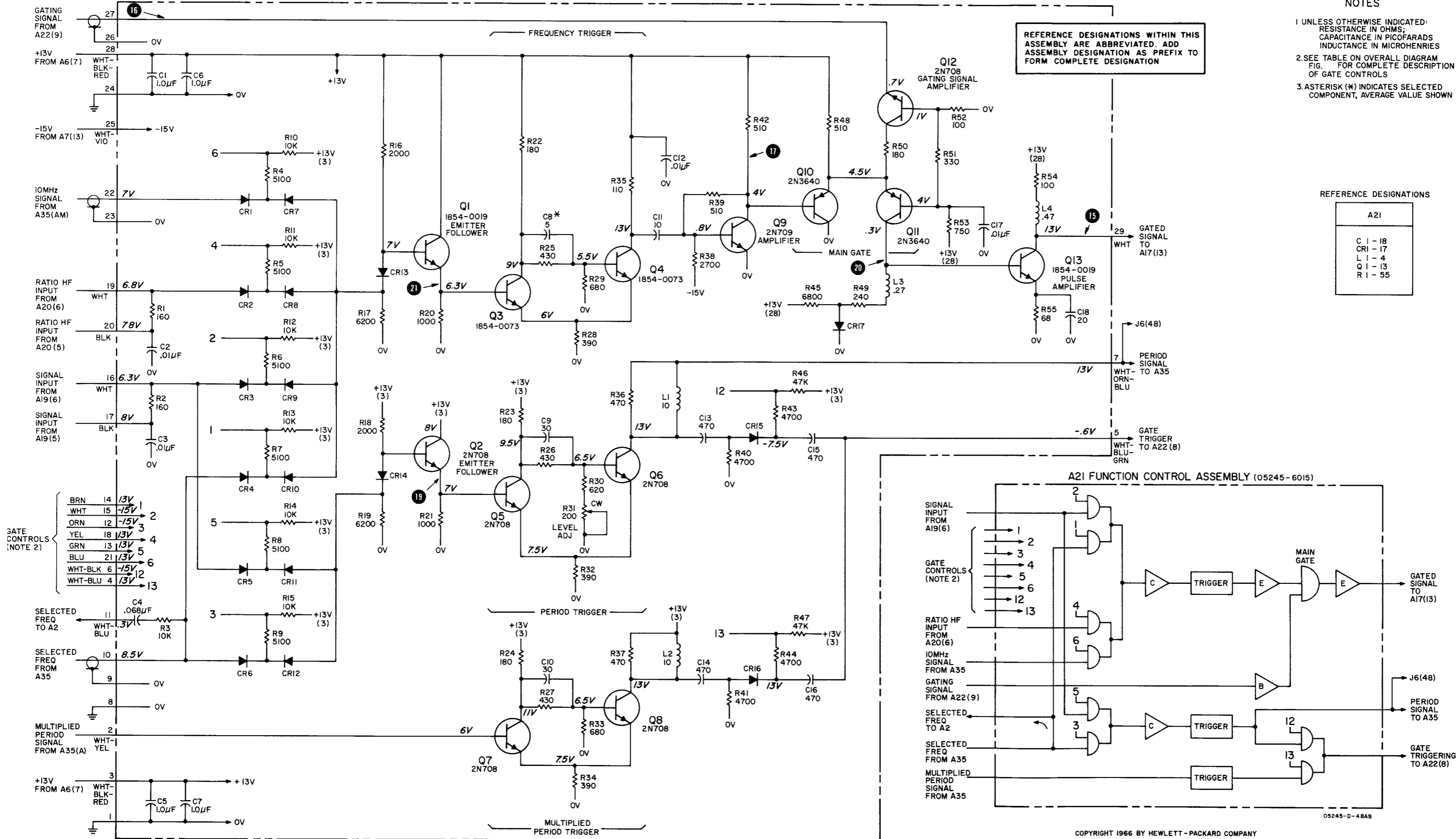
Figure 7-18. A21 Function Control
