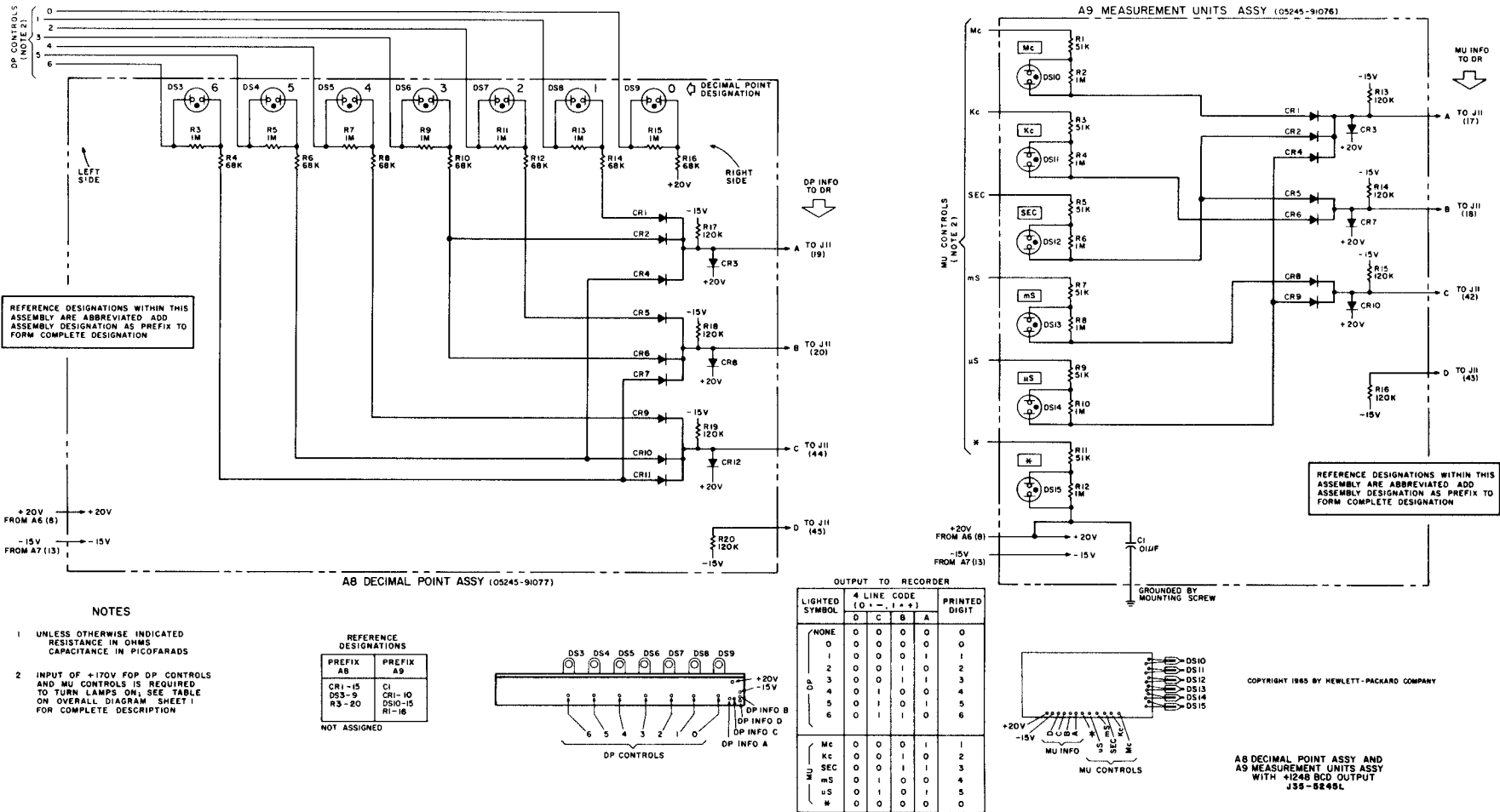
Figure 5-1. DP and MU with +1248 BCD Output (J35-5245L Special)
