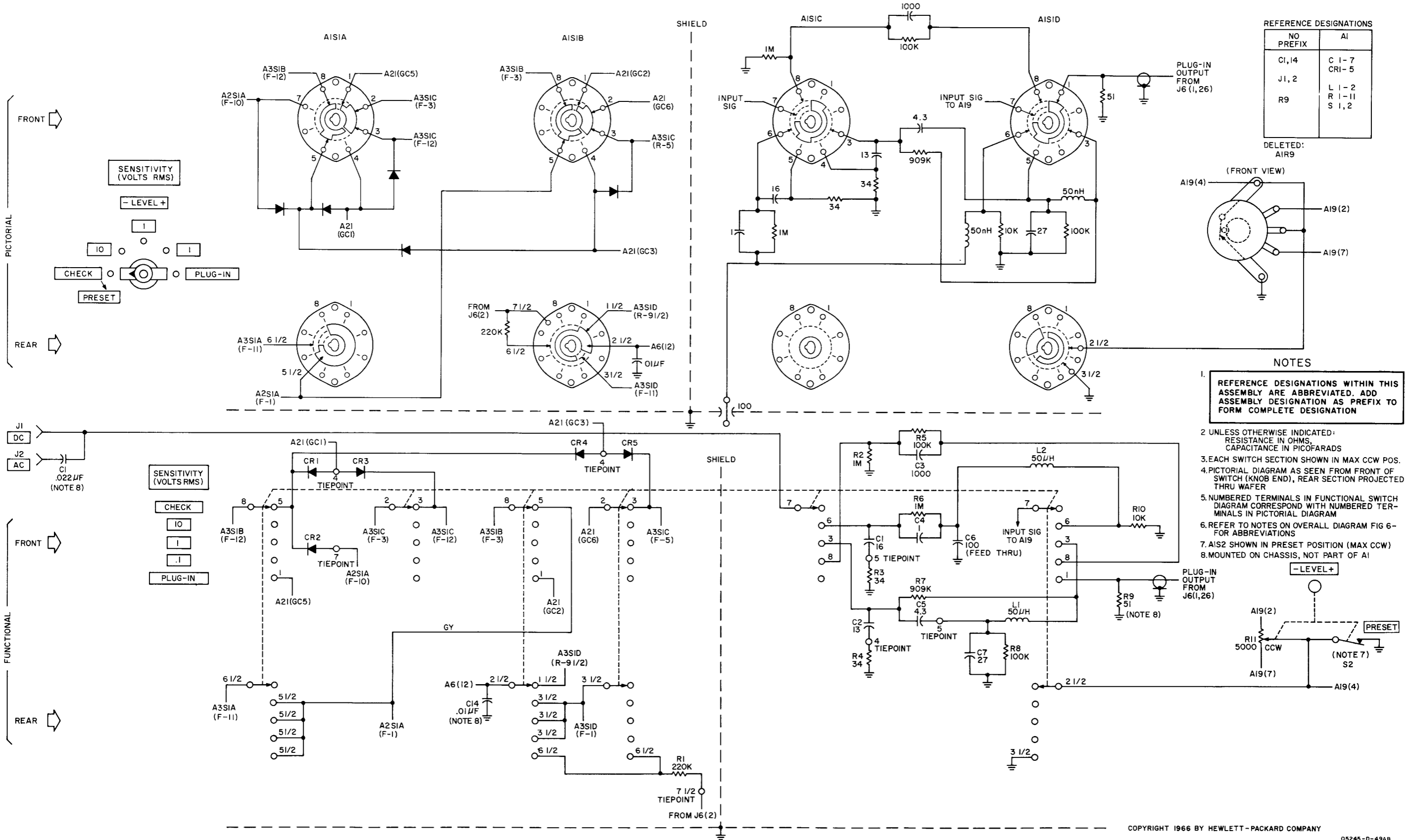
Figure 7-3. AI Input Switch
