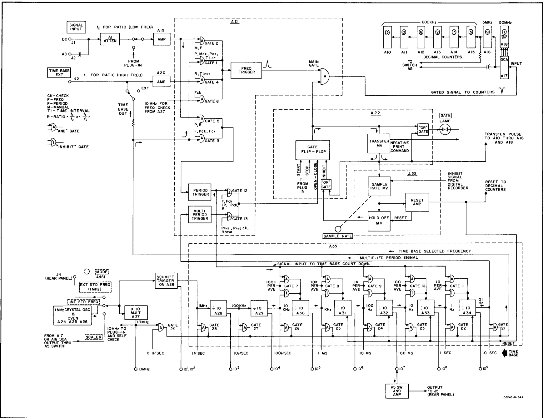
Figure 2-13. Model 5245L Logic Block Diagram
