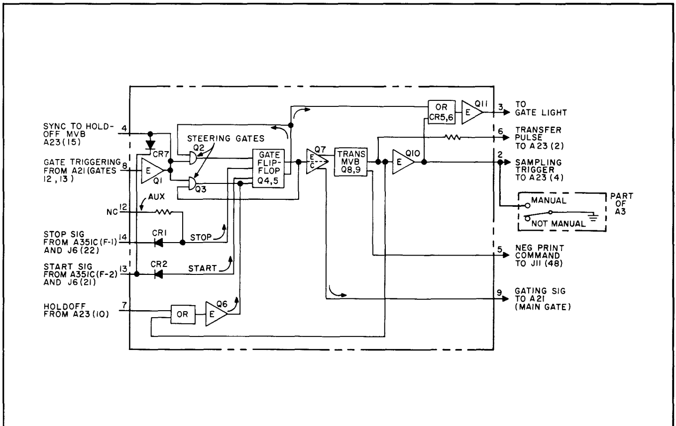
Figure 2-18. Gate Control Block Diagram
