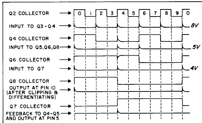
WAVEFORMS
