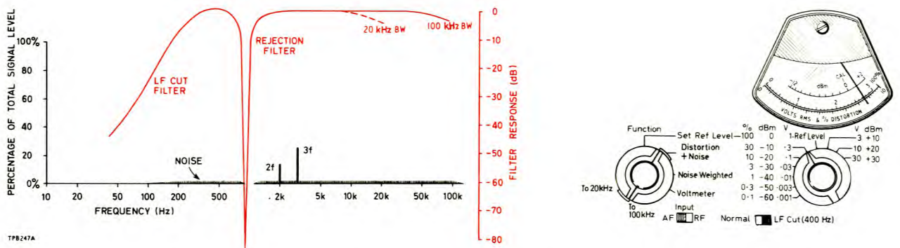
Fig. 2.5 Fundamental rejection with I.f. cut
