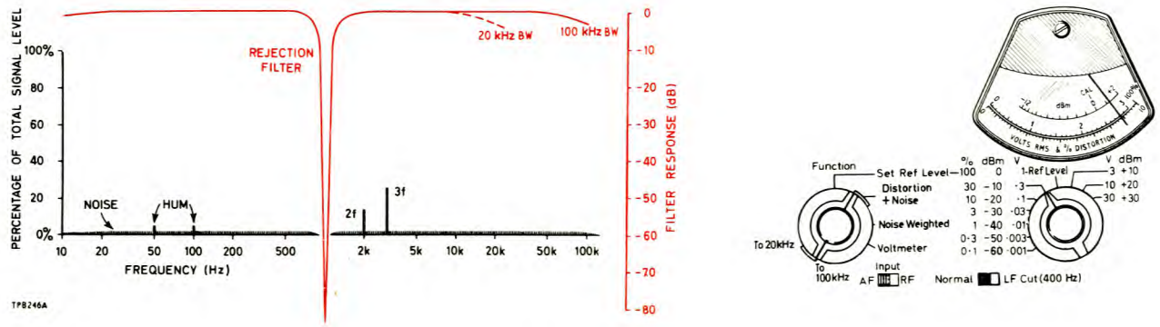
Fig. 2.4 Fundamental rejection
