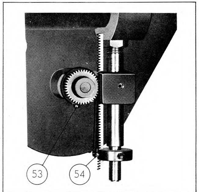
Figure 4-40. Attenuator Drive Loading Spring in Place
