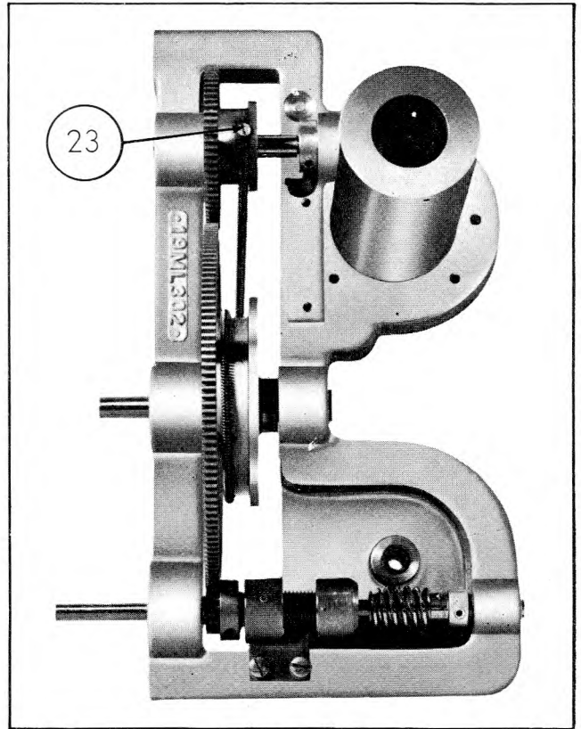
Figure 4-17. Right View of Assembled Drive
