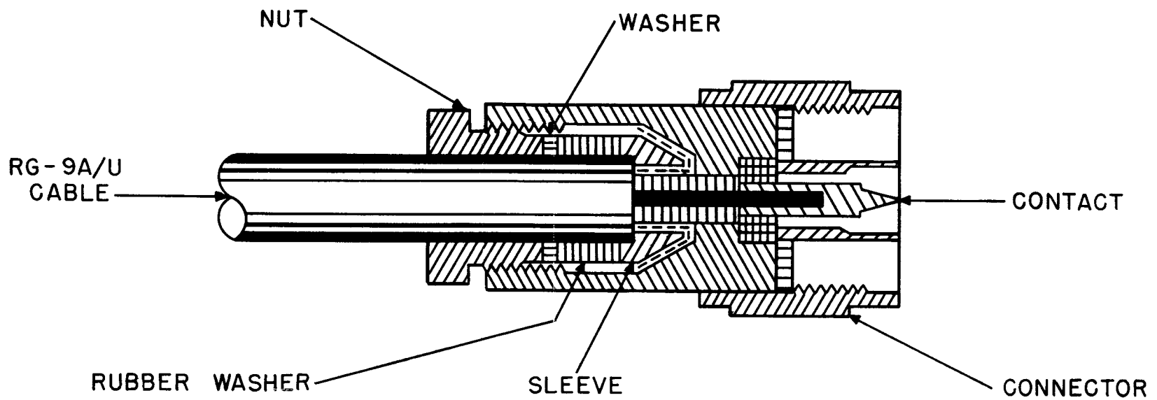
Figure 7-9. RF Cable CG-92B/U (6'), Fabrication Data
