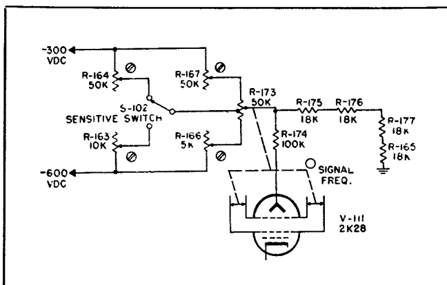
Figure 3-5. Repeller Voltage Tracking Circuit
