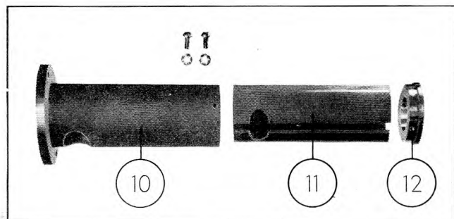
Figure 4-10. Parts Comprising Drive Housing
