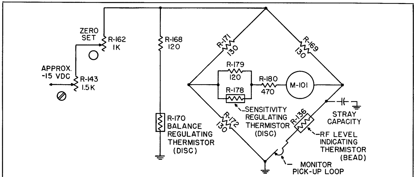
Figure 3-6. Monitor Circuit
