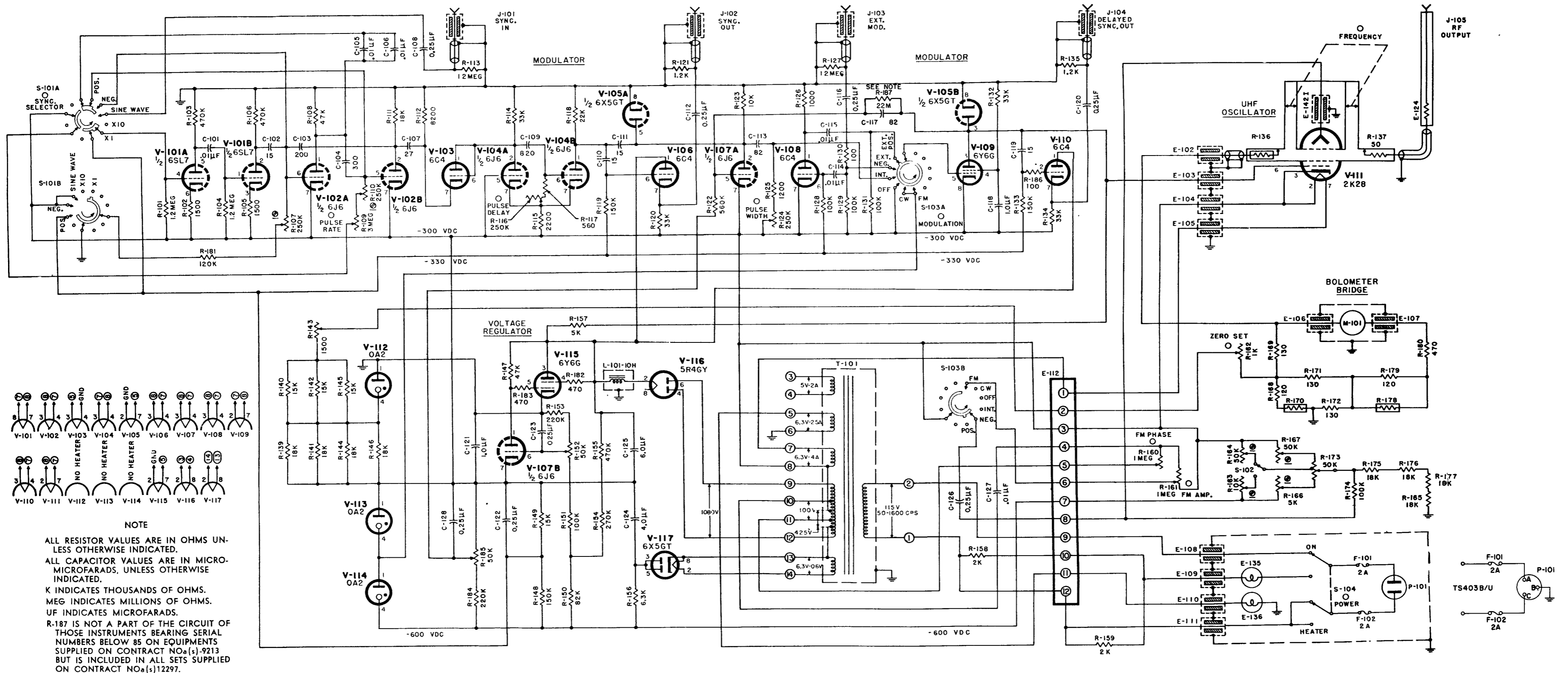
Figure 7-1. Signal Generator TS-403/U, Schematic Diagram
