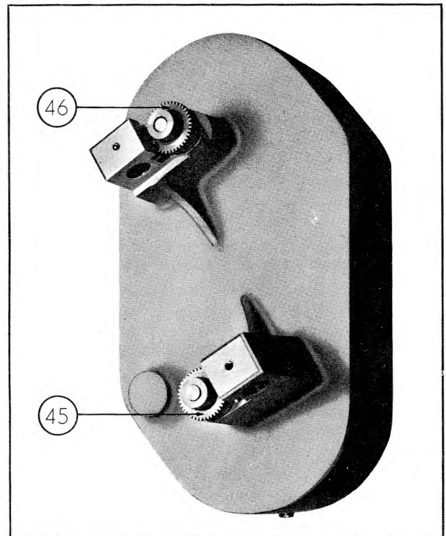
Figure 4-33. Rear View of Attenuator Gear Case
