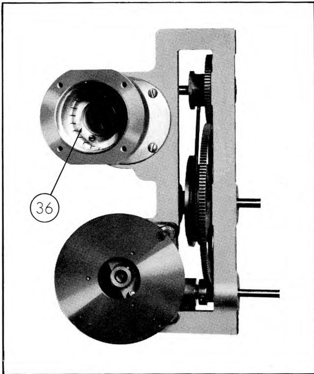
Figure 4-30. Left View of Assembly with Brush in Place
