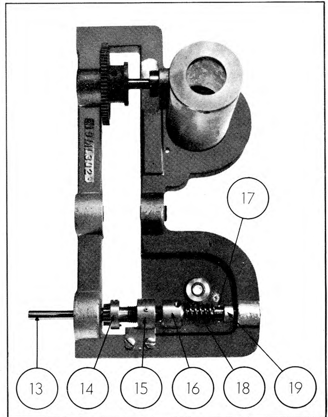
Figure 4-13. Lower Drive System Assembled
