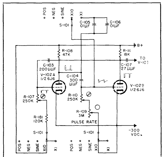
Figure 3-8. Free Running Pulse Rate Multivibrator
