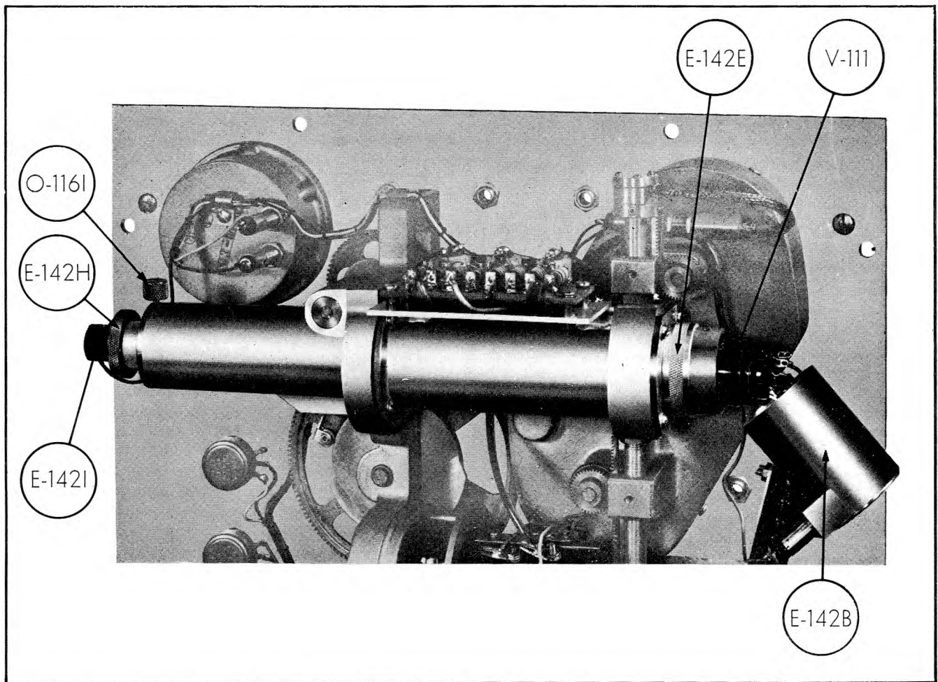
Figure 4-2. Removal of Shield E-142 B
