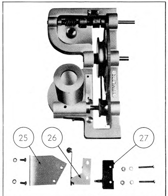
Figure 4-18. Assembly of Sensitive Switch S-102
