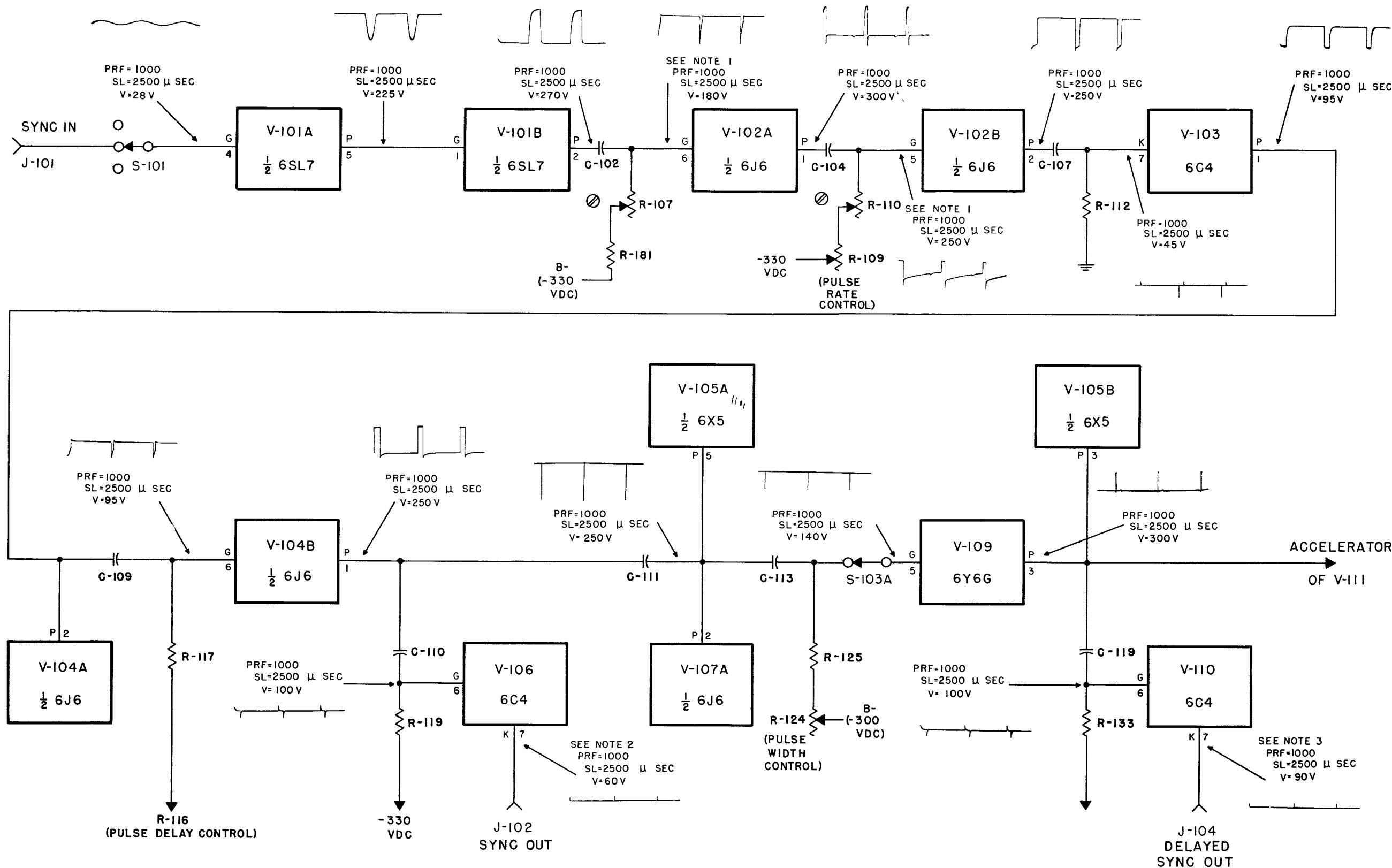
Figure 7-4. Signal Generator TS-403/U, Servicing Block Diagram
