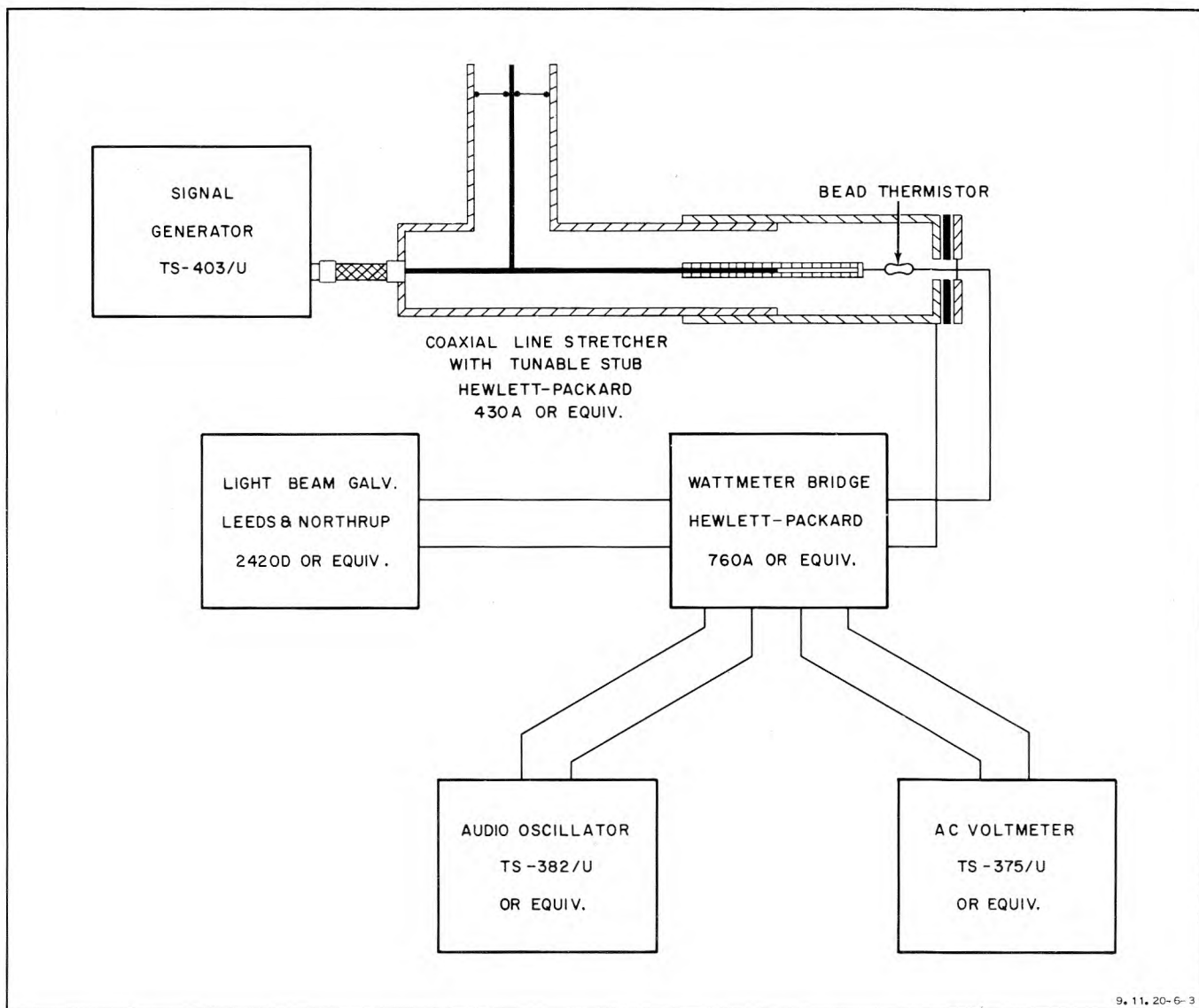
Figure 4-46. Test Set-up for Calibrating Output Attenuator
