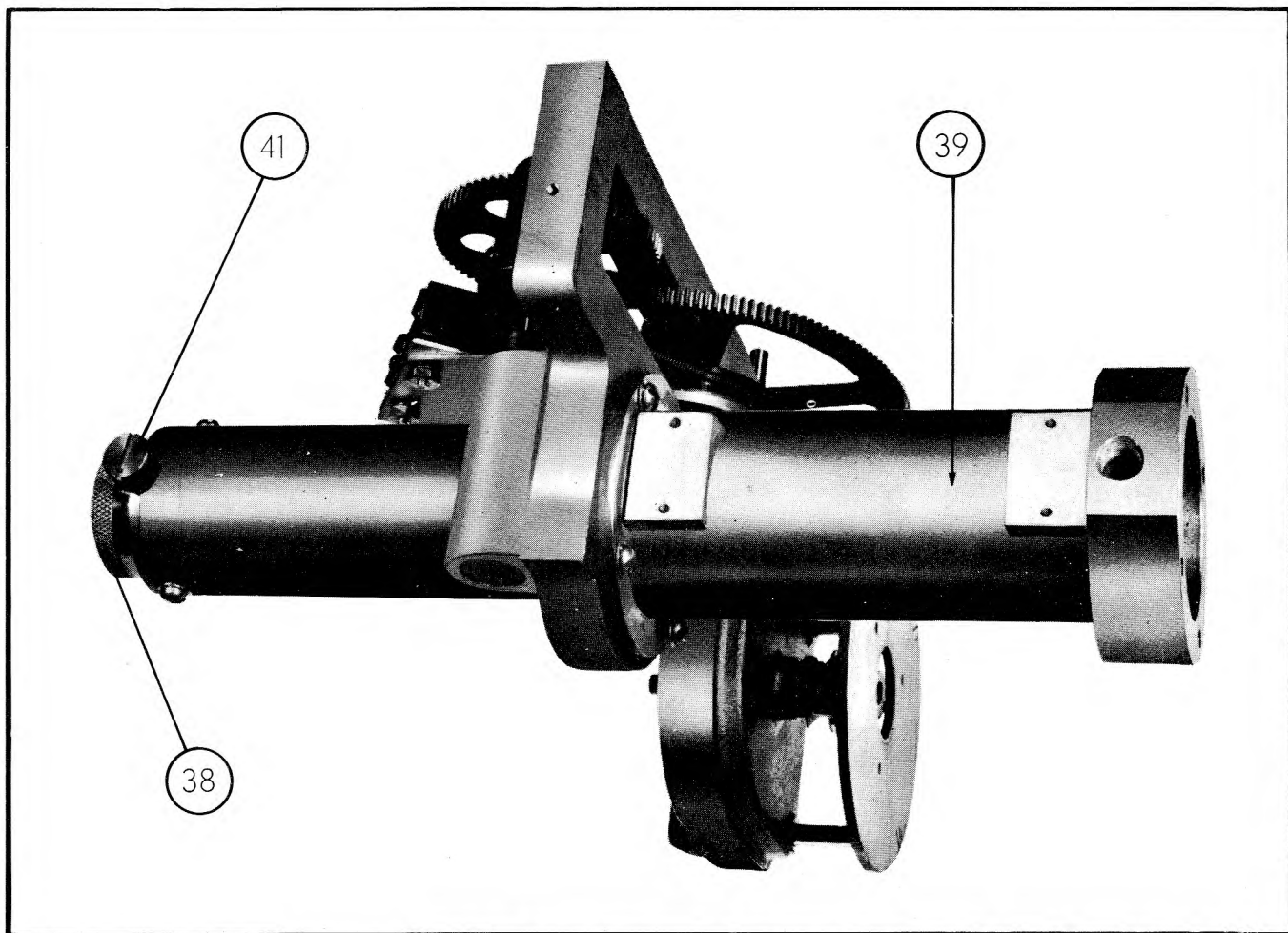
Figure 4-29. Outer Conductor Assembled
