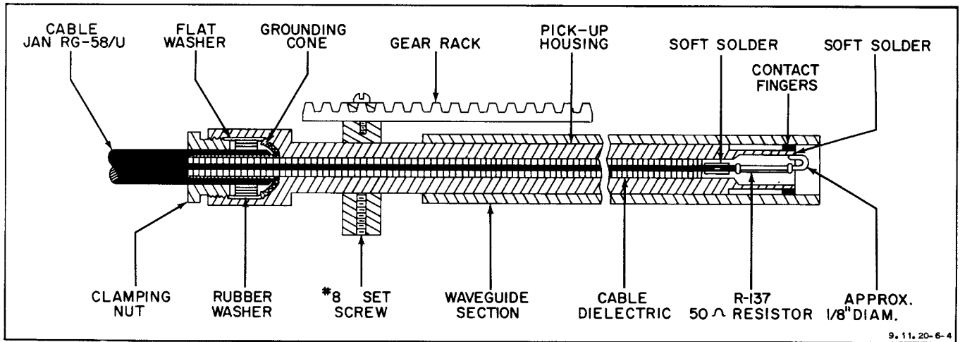
Figure 4-47. Cutaway View of Output RF Probe E-101
