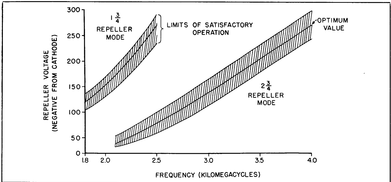
Figure 3-4. Repeller Voltage Characteristics
