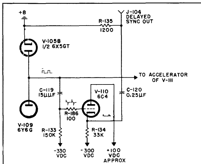
Figure 3-15. Delayed Sync Out Circuit
