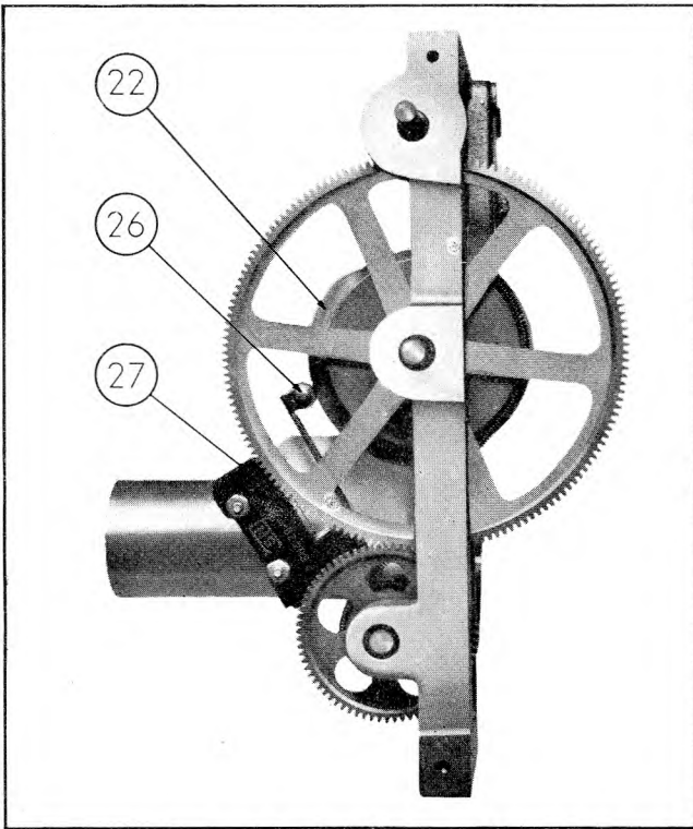
Figure 4-19. Sensitive Switch Mounted on Main Casting
