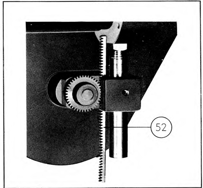
Figure 4-39. Assembly of Attenuator Rack
