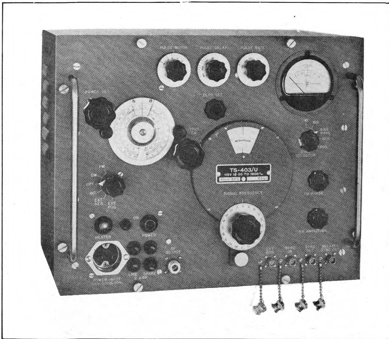
Figure 1-4. Signal Generator TS-403/U, Oblique View
