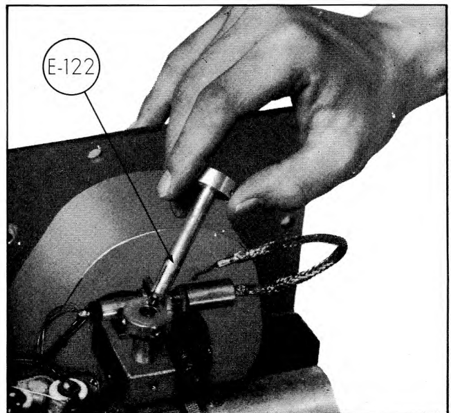
Figure 4-8. Removal of E-122
