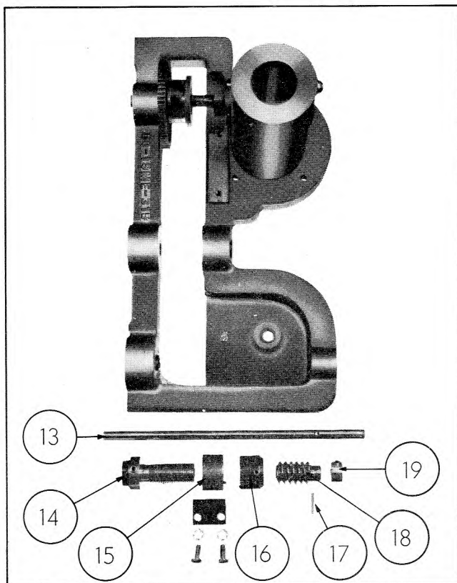
Figure 4-12. Parts Comprising Lower Drive System
