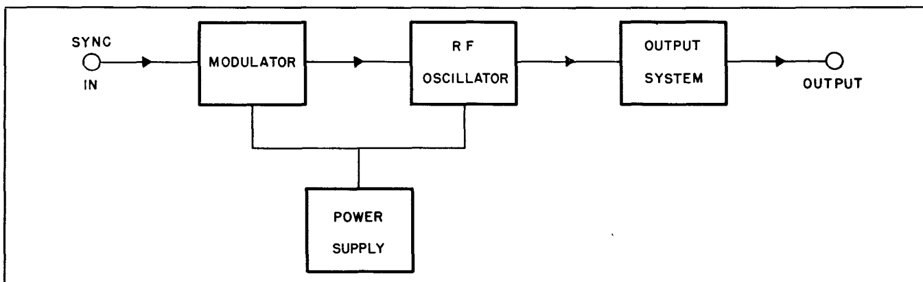
Figure 3-1. Signal Generator TS-403/U, Circuit Block Diagram
