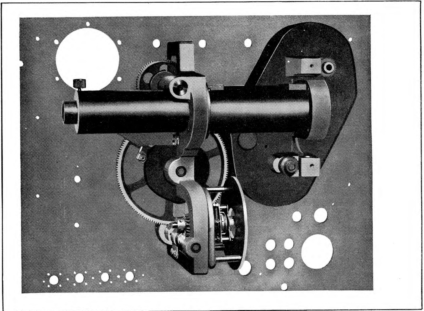
Figure 4-34. Oscillator and Attenuator Assembly Mounted on Panel
