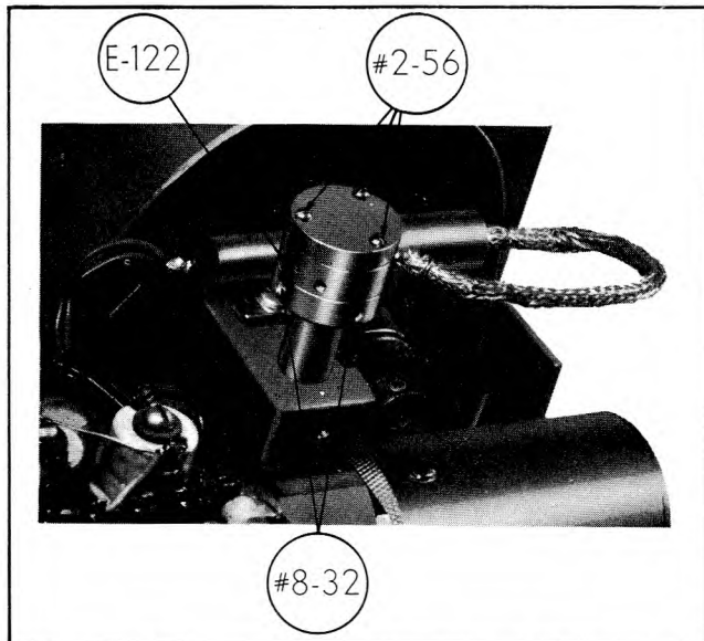
Figure 4-6. Screws Holding RF Probe in Place
