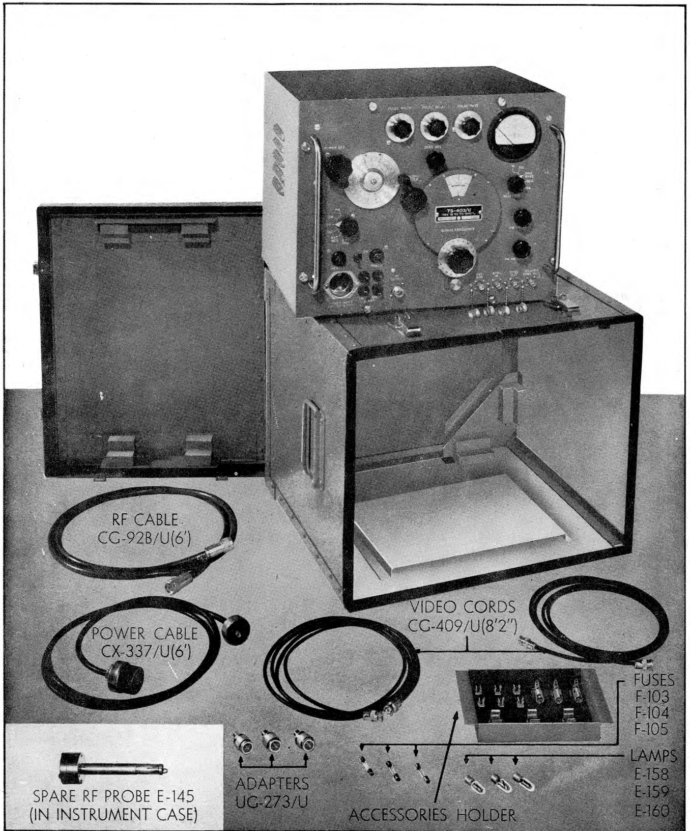
Figure 1-1. Signal Generator TS-403/U, Equipment Supplied
