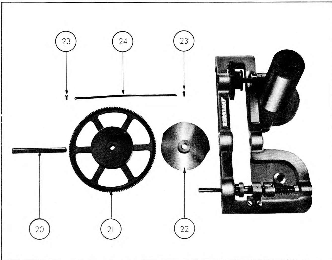
Figure 4-14. Parts Comprising Main Drive System
