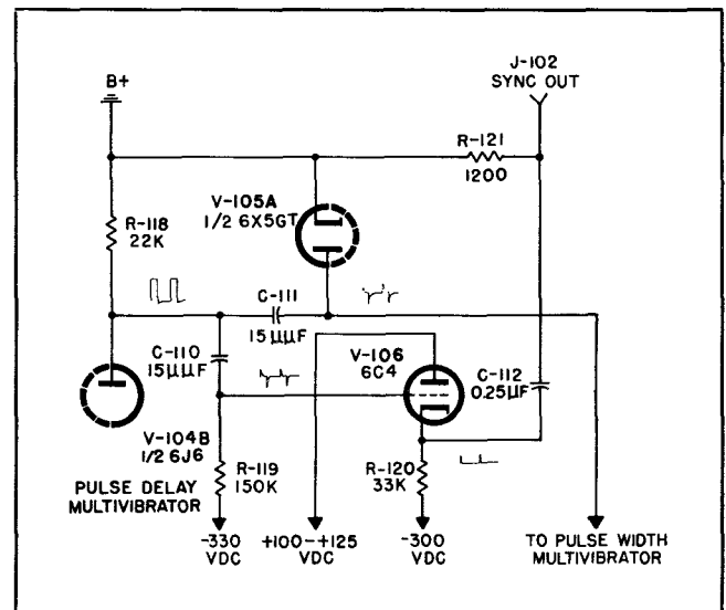
Figure 3-13. Sync. Out Pulse Circuit
