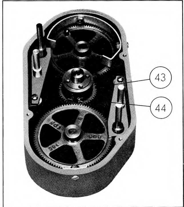
Figure 4-32. Attenuator Gear Case Showing Spring-Loading of Pinion
