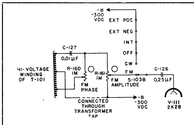
Figure 3-18. Circuit Providing Repeller AC Voltage for FM
