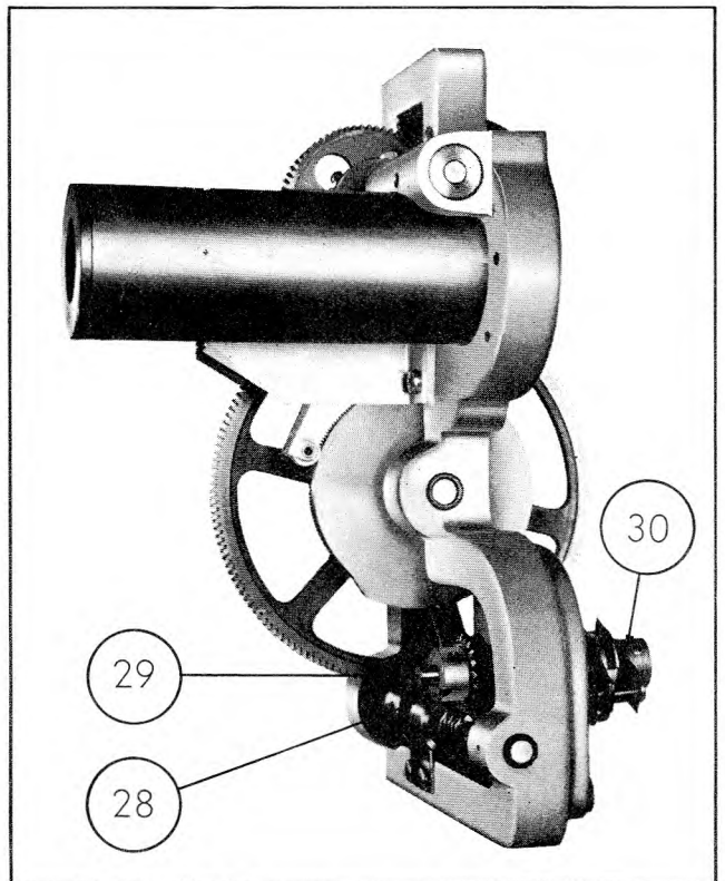
Figure 4-22. Oblique View Showing Potentiometer Drive Assembled
