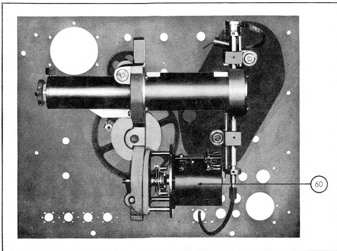
Figure 4-44. Complete Drive System Assembled on Panel
