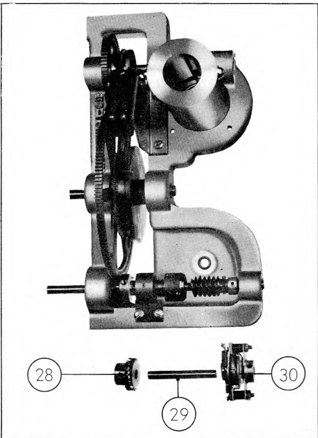
Figure 4-20. Parts Comprising Potentiometer Drive
