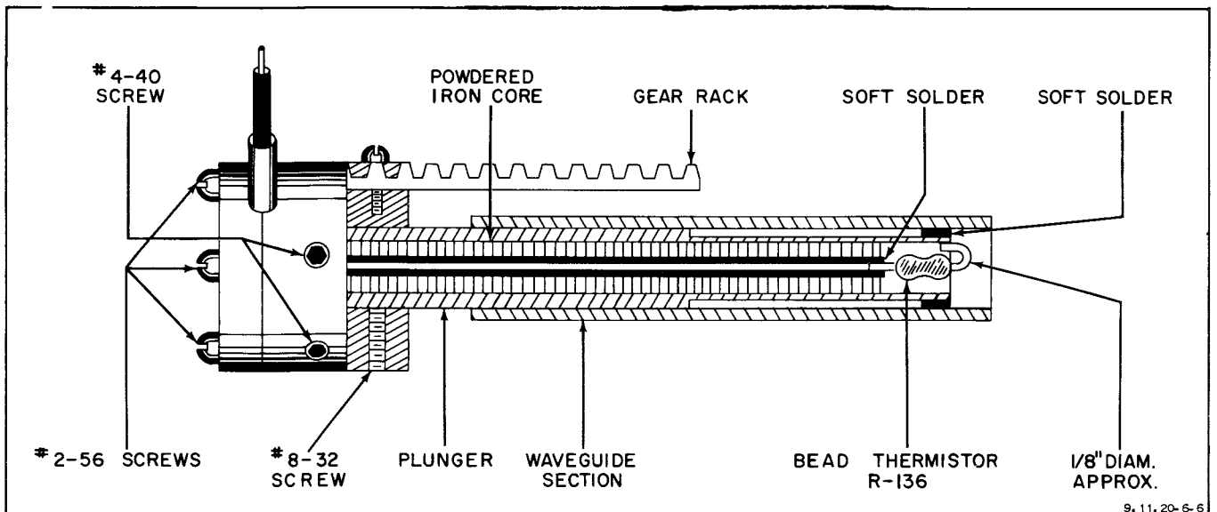
Figure 4-49. Cutaway View of Monitor RF Probe E-122
