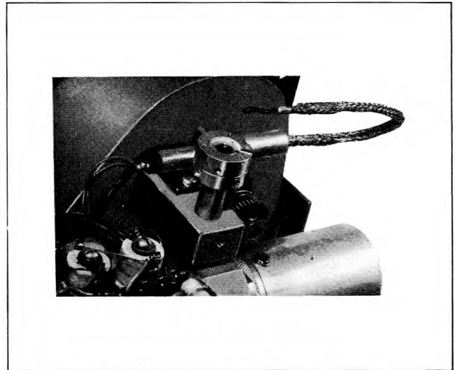
Figure 4-7. Removal of Cap of RF Probe
