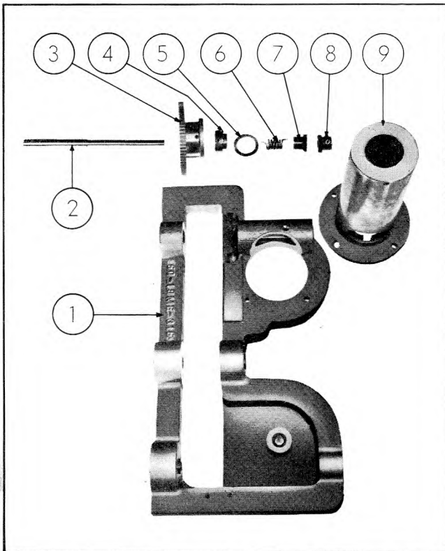
Figure 4-9. Parts Comprising Upper Drive System
