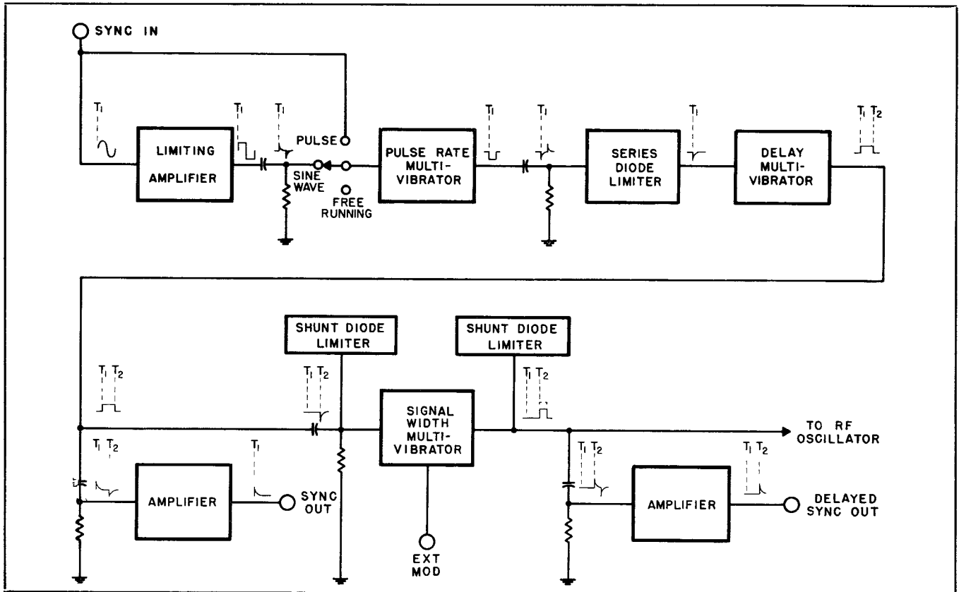
Figure 3-7. Modulator Section Block Diagram
