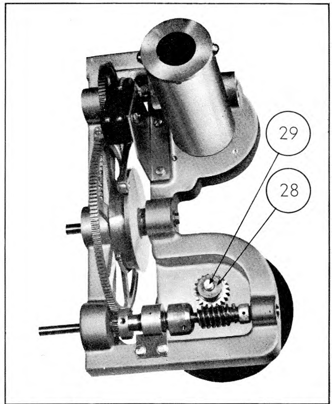
Figure 4-21. Potentiometer Drive Assembled Into Place
