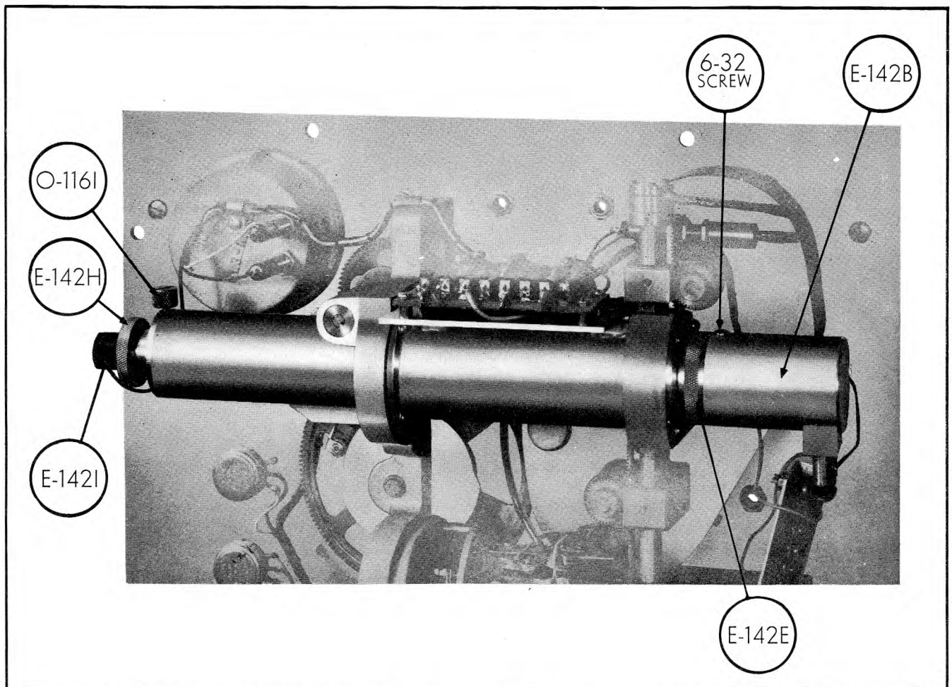
Figure 4-1. Overall View of Oscillator Assembly
