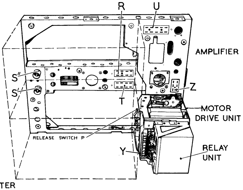
Fig. 3—Main tray.
