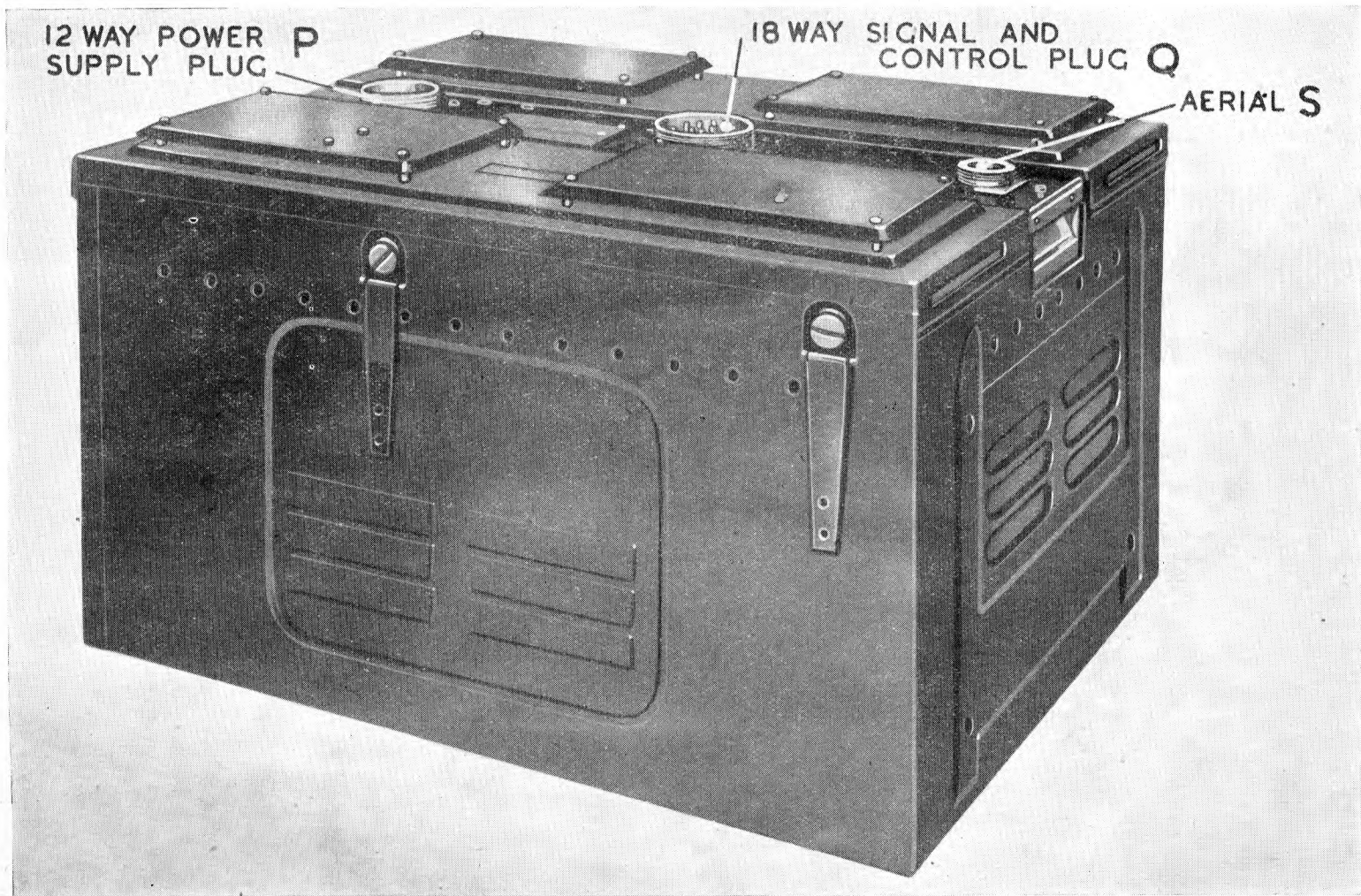
Fig. 1—TR. 1143A—general view.
