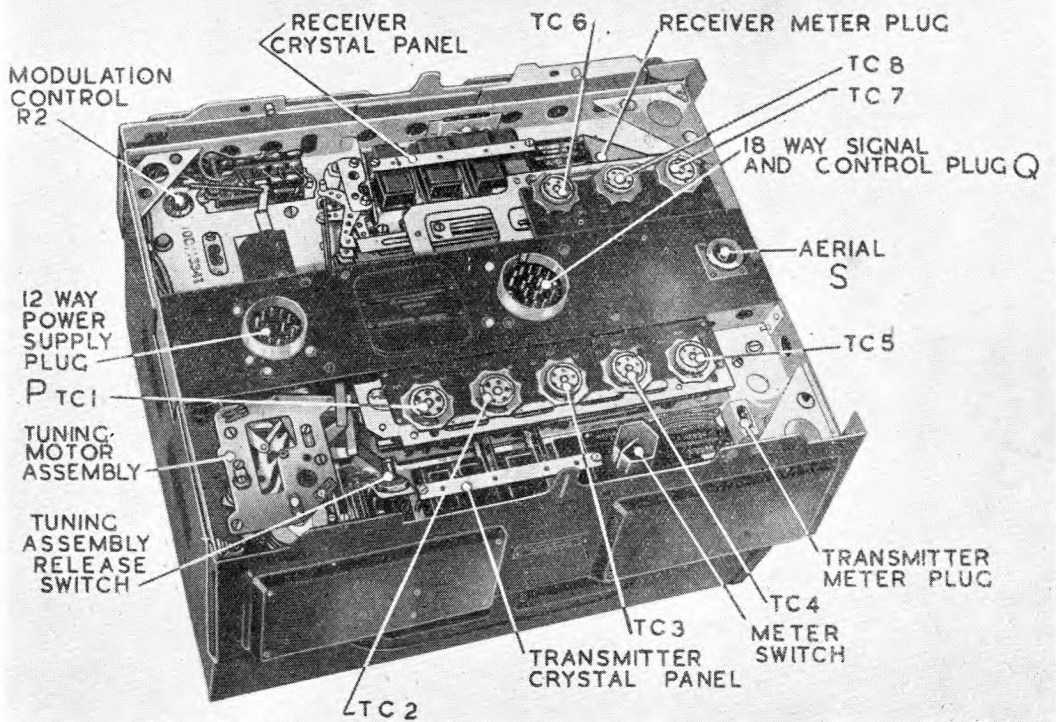
Fig. 2—TR. 1143A—top covers slid back.
