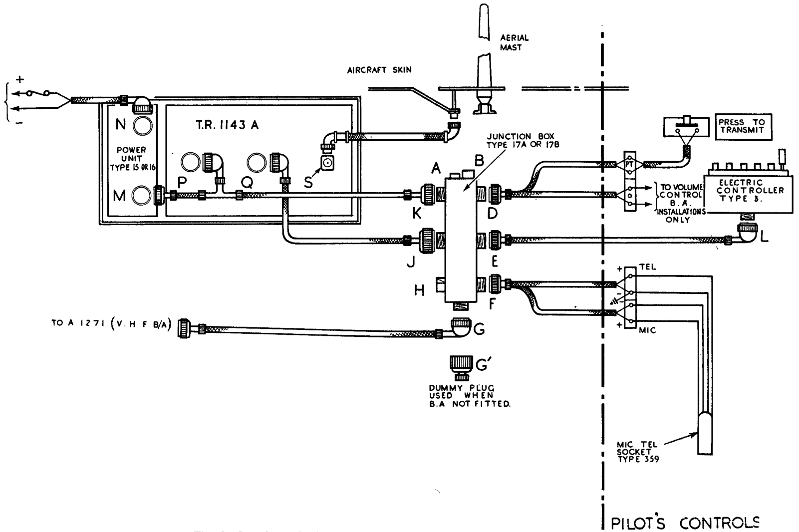
Fig. 6—Standard single-seater installation (showing plug nomenclature).
