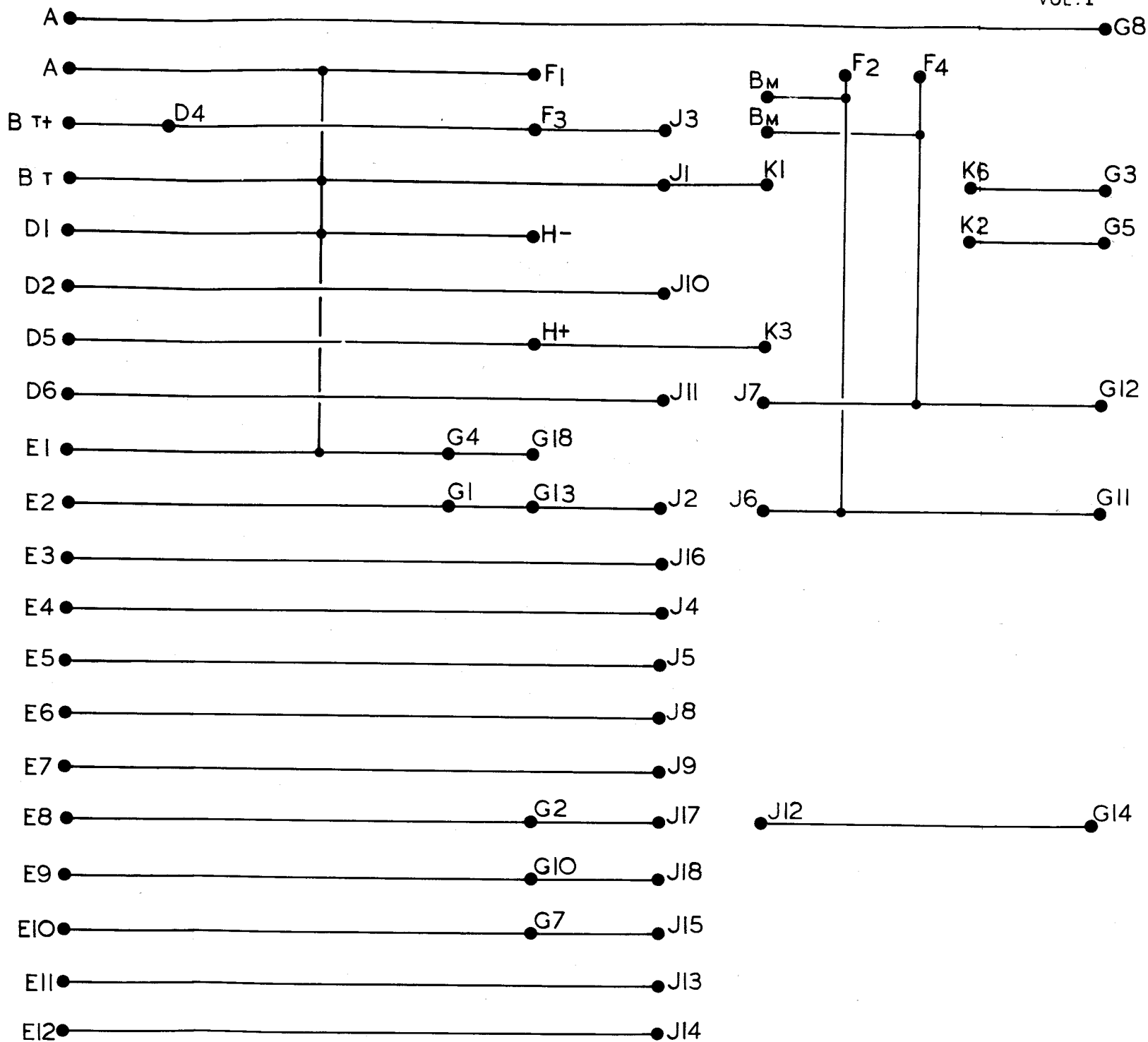
FIG. 29. JUNCTION BOX, TYPE 17A OR 17B, CIRCUIT
