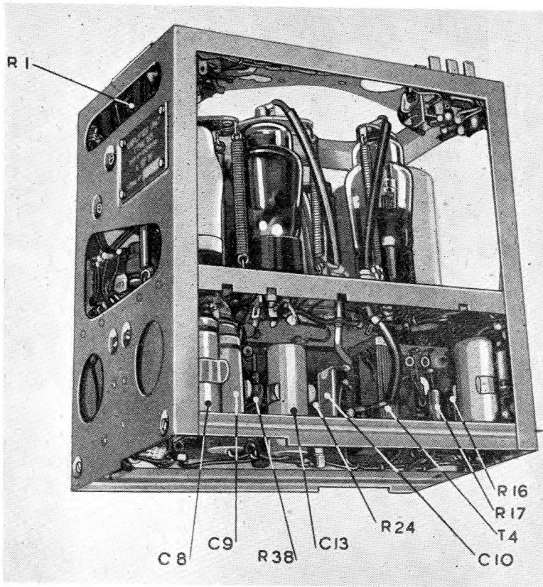
Fig. 11—Amplifier unit—underside.
