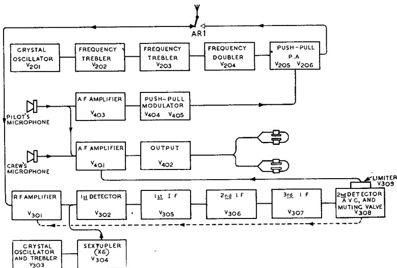
Fig. 4—Block-diagram.
