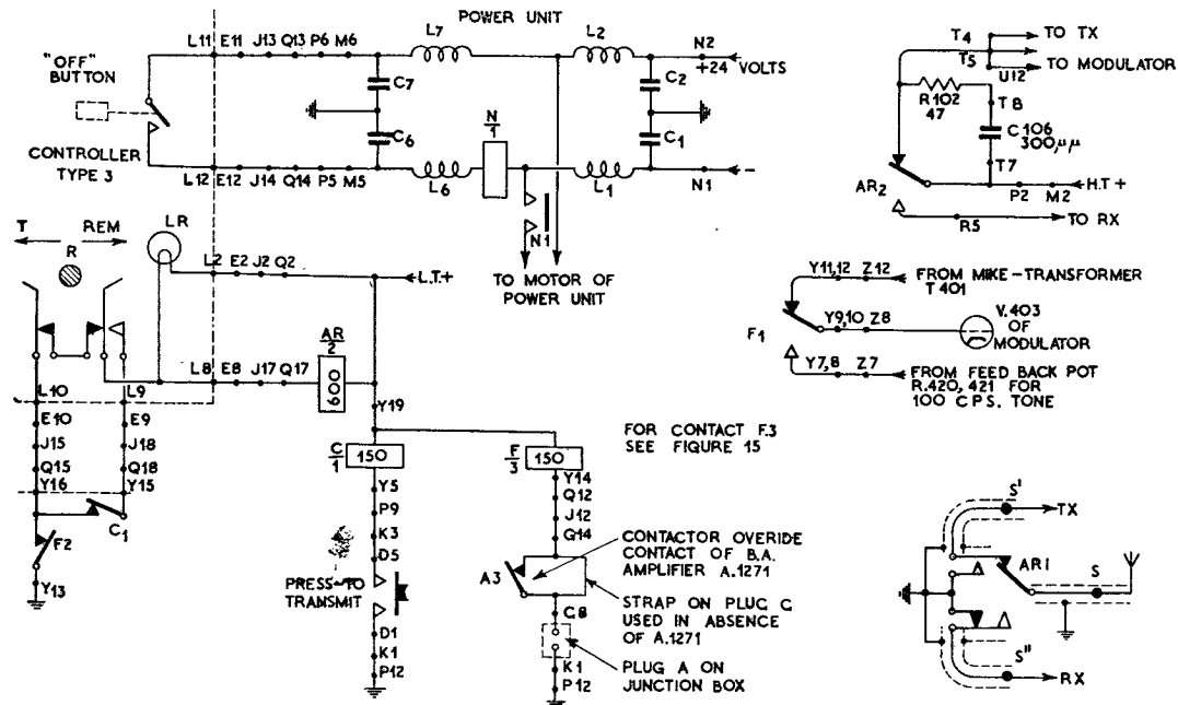
Fig. 14—Control circuits I (on-off, TR and MCW).
