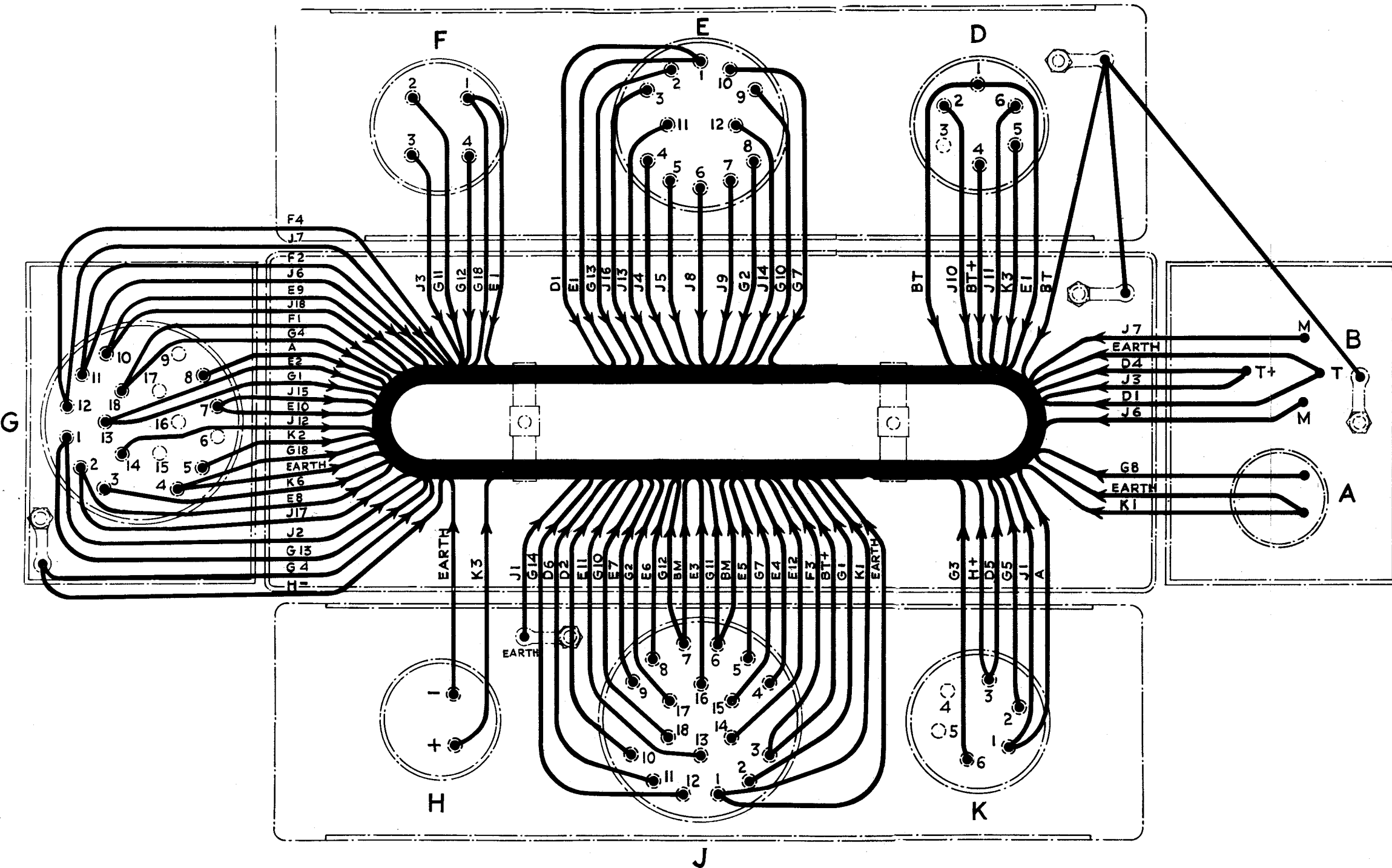
FIG. 30. JUNCTION BOX, TYPE 17B, WIRING DIAGRAM
