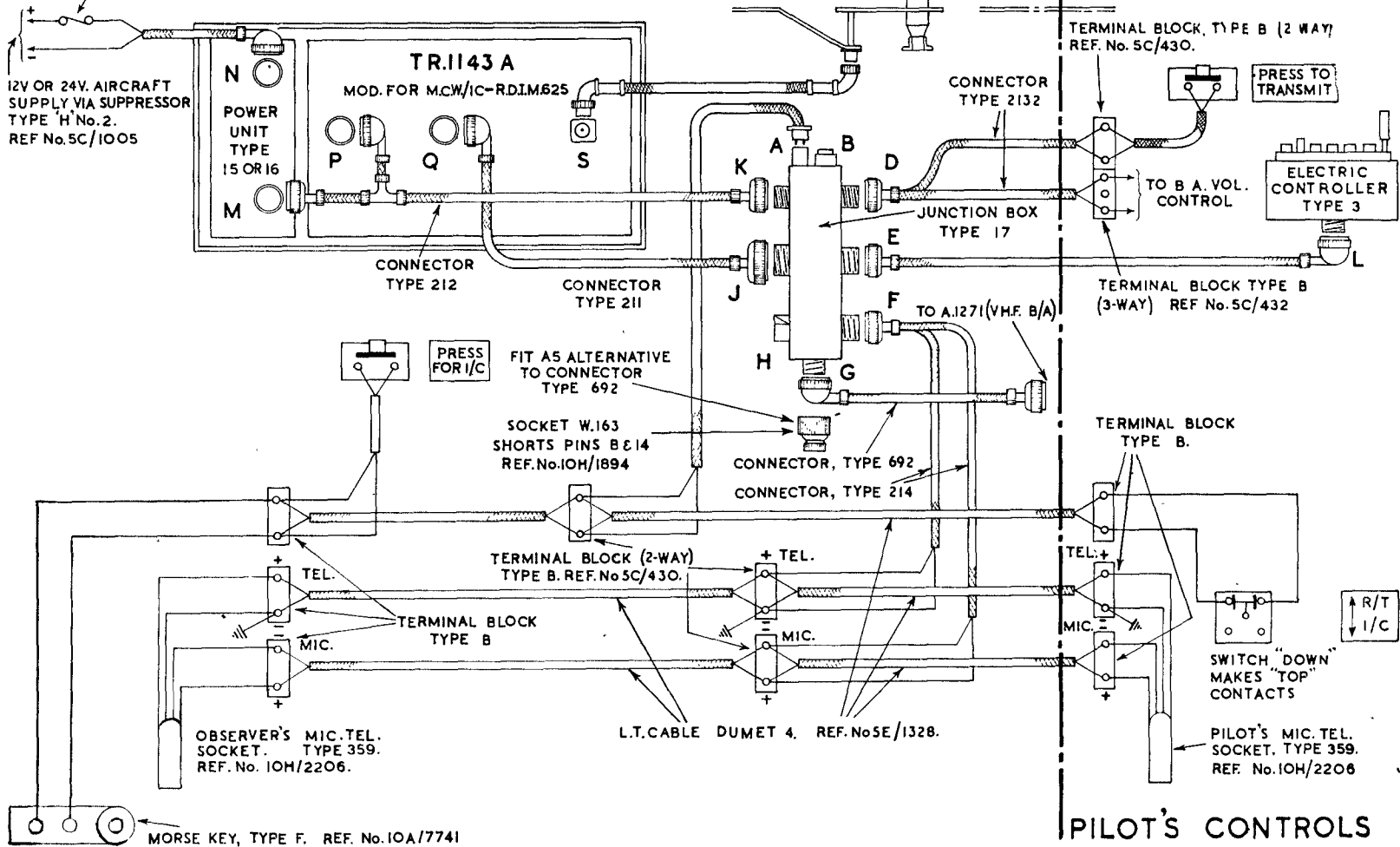
Fig. 9—Pilot-crew installation II.
