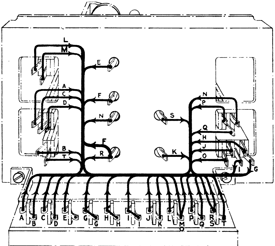
FIG. 28 - WIRING DIAGRAM OF RELAY UNIT
