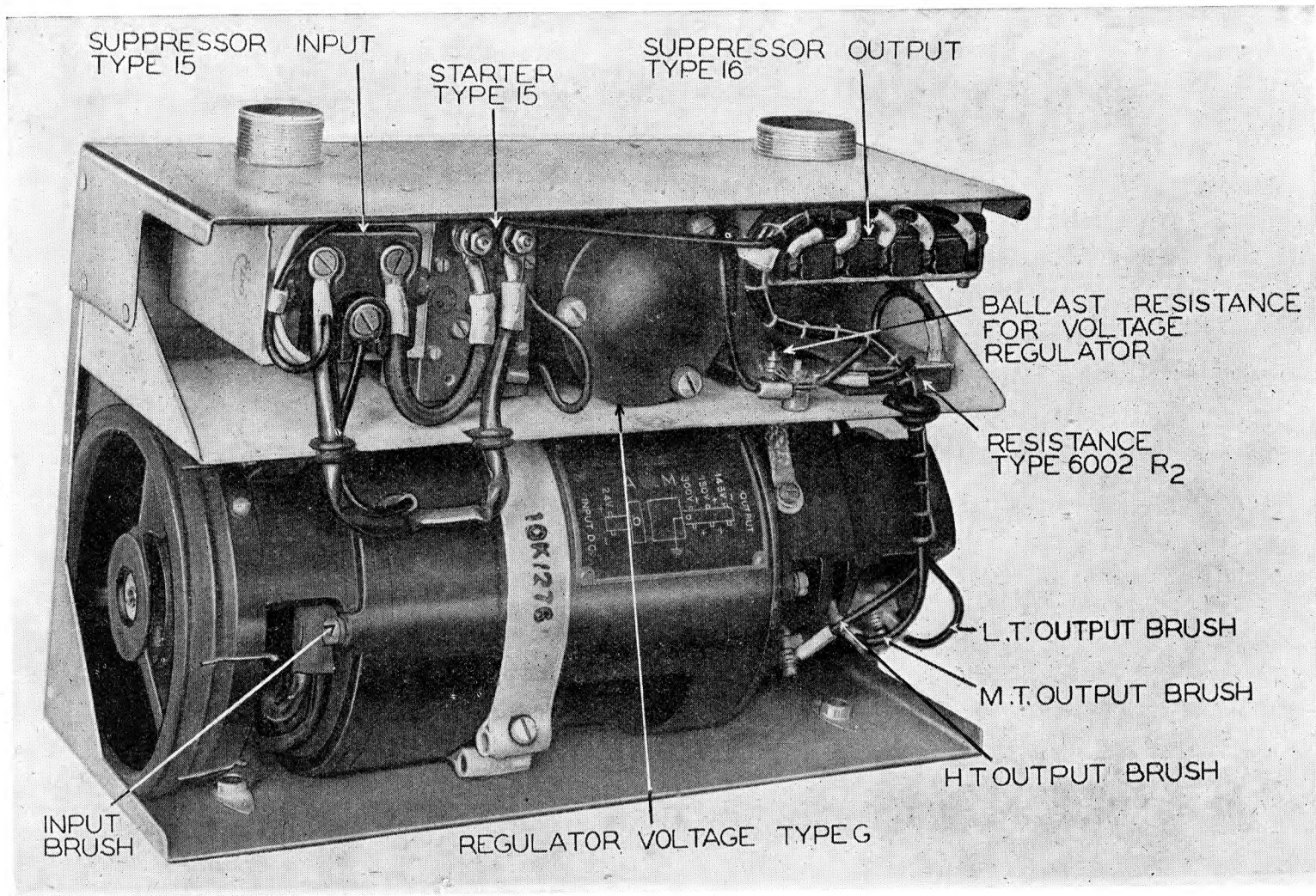
Fig. 34—Power unit, type 16, view with cover removed.
