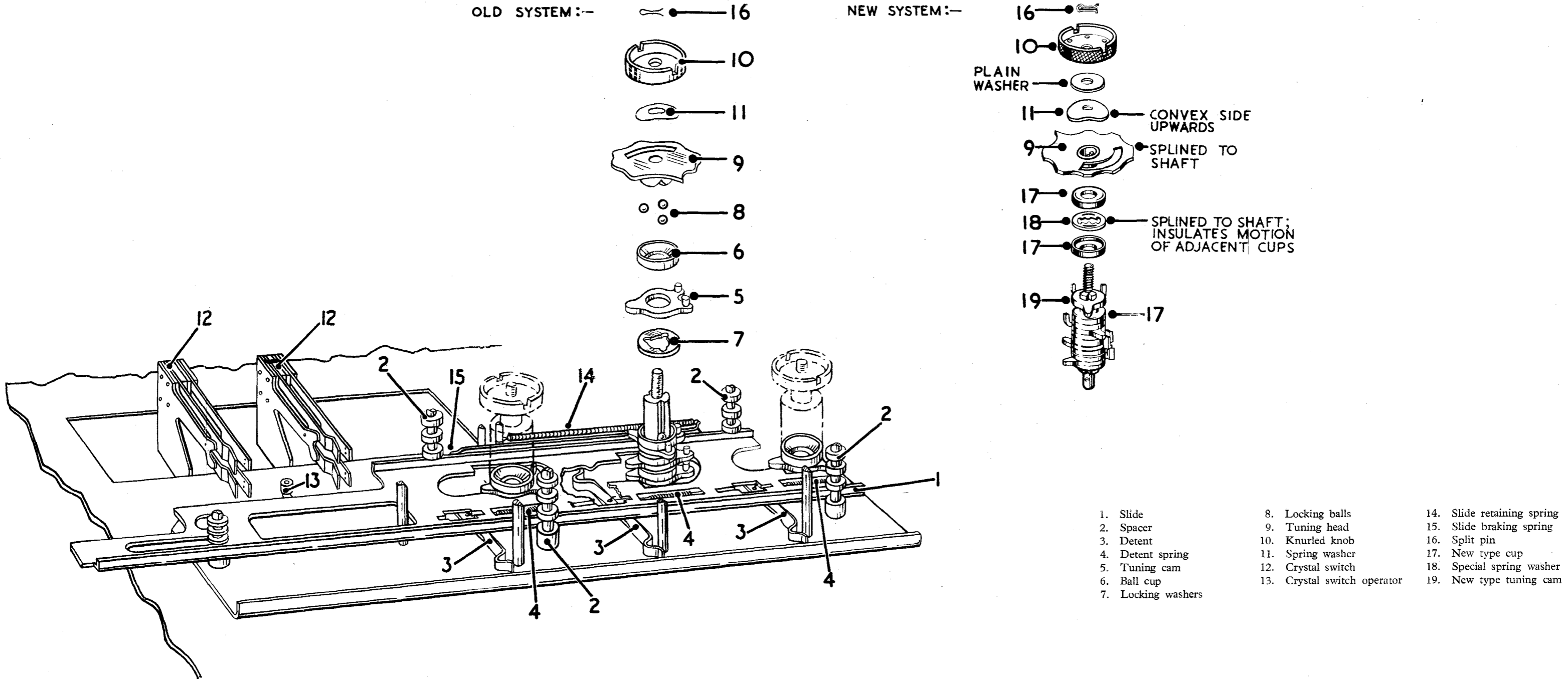
FIG. 24 PERSPECTIVE OF TUNING CAMS
