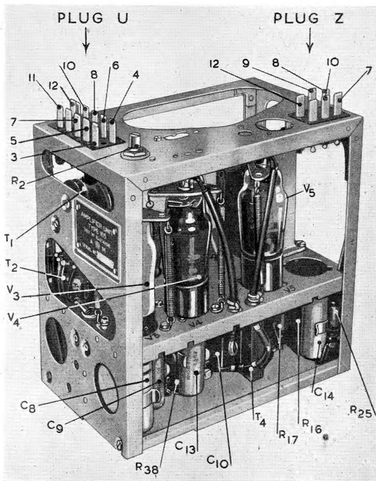
Fig. 10—Amplifier unit type 165.
