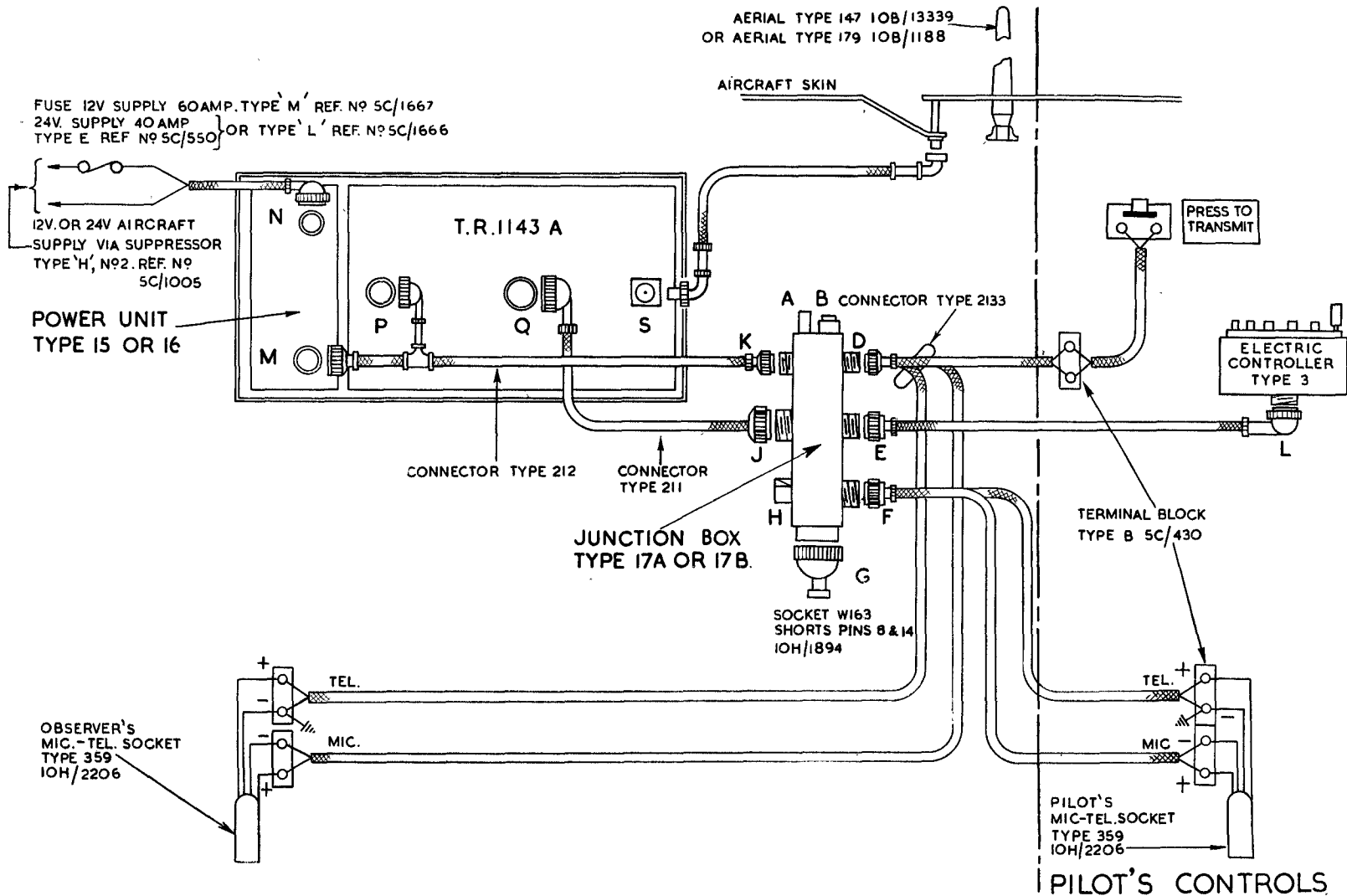
Fig. 8—Pilot-crew installation I.
