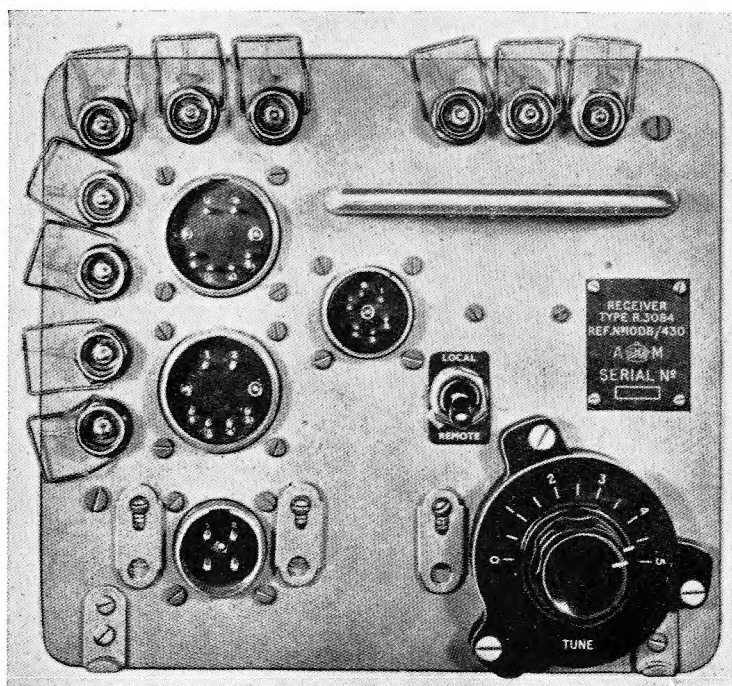
Receiver of A.S.V. Mark II
