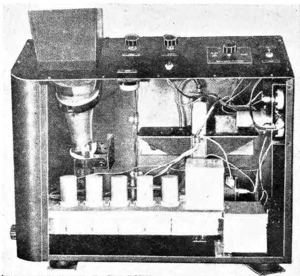
Receiver of A.S.V. Mark I
