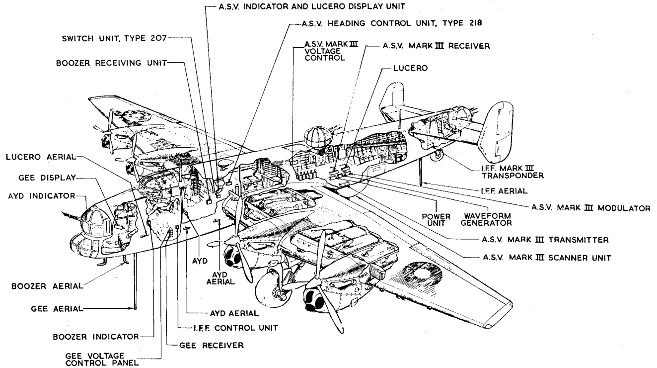
Layout of Radar Equipment in Halifax Mark II
