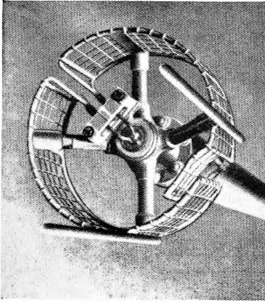
The Bali Broad-Band Round Dipole Aerial
