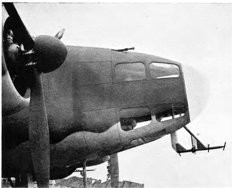
Transmitter Array—Side View
