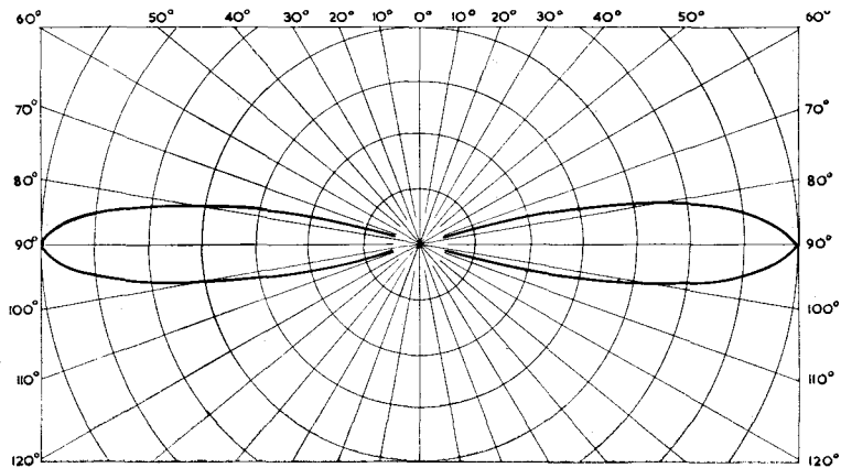
Broadside Aerials
