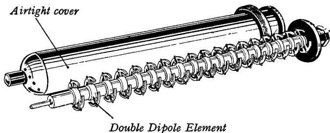
END FIRE ARRAY, COVER REMOVED
