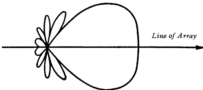
TYPICAL FIELD STRENGTH DIAGRAM
