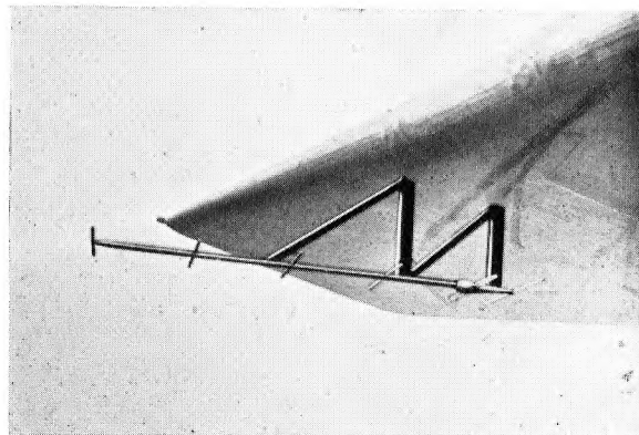
Homing Receiver Aerial
